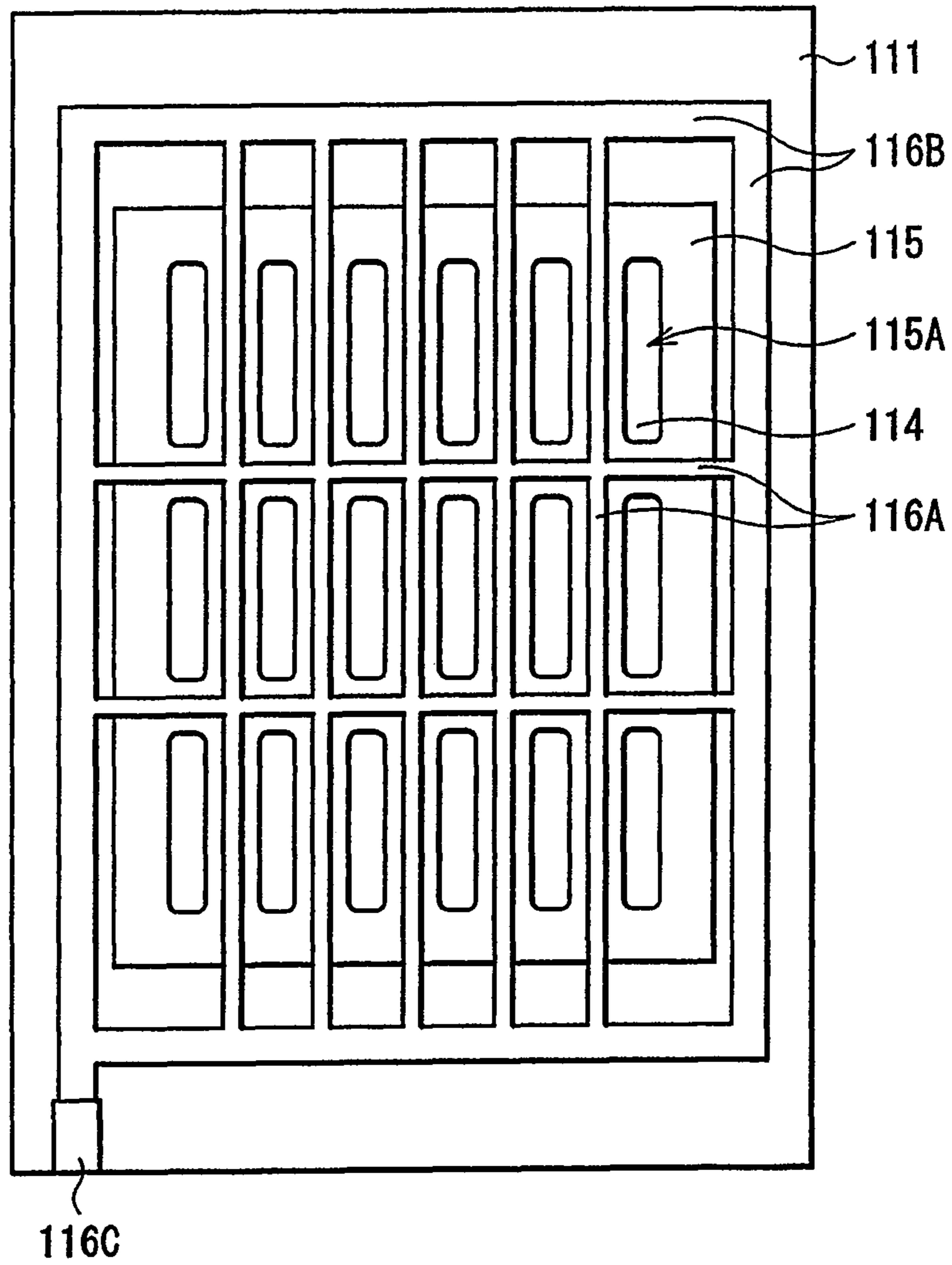
FIG. 3 PRIOR ART
