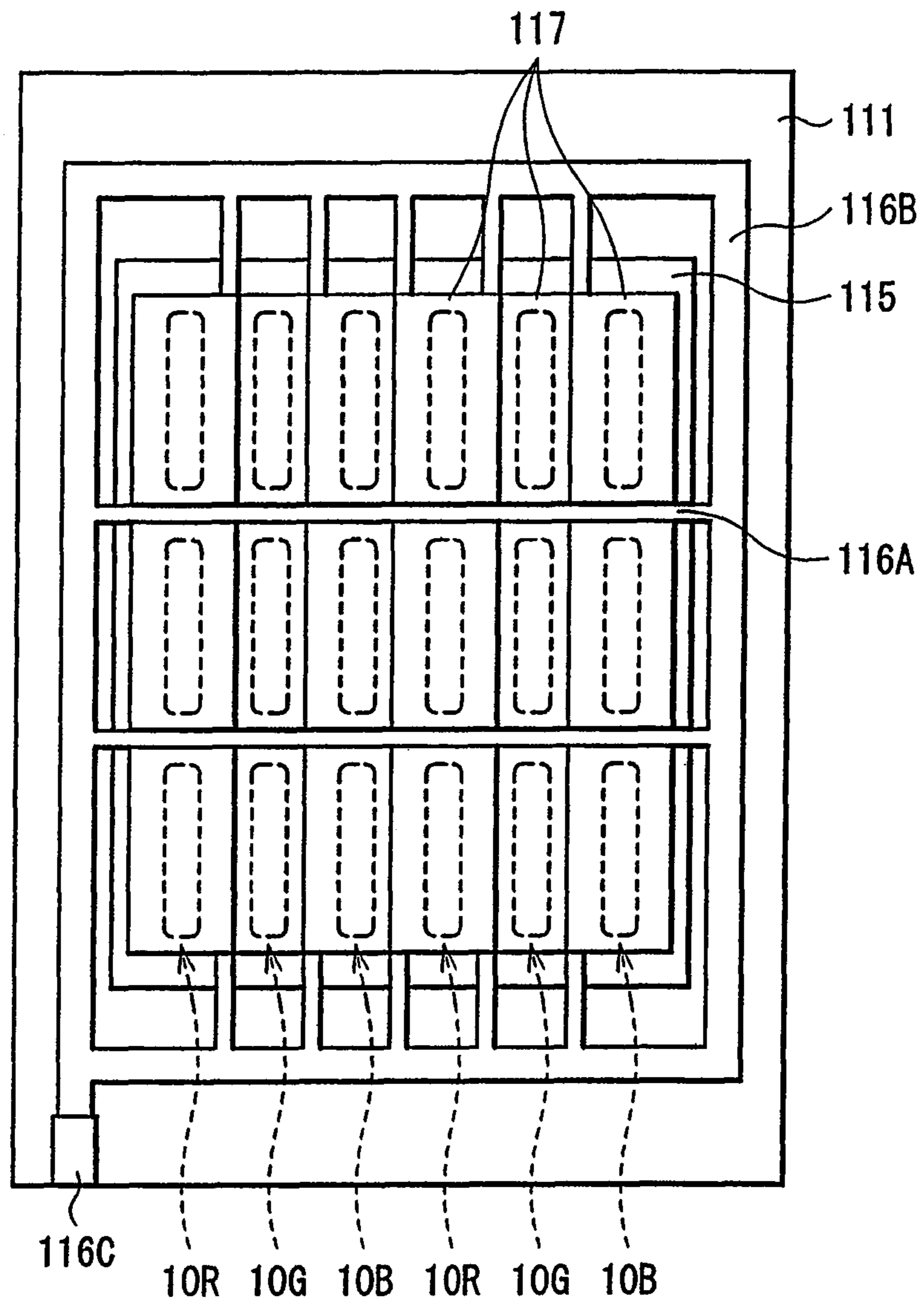
FIG. 6 PRIOR ART
