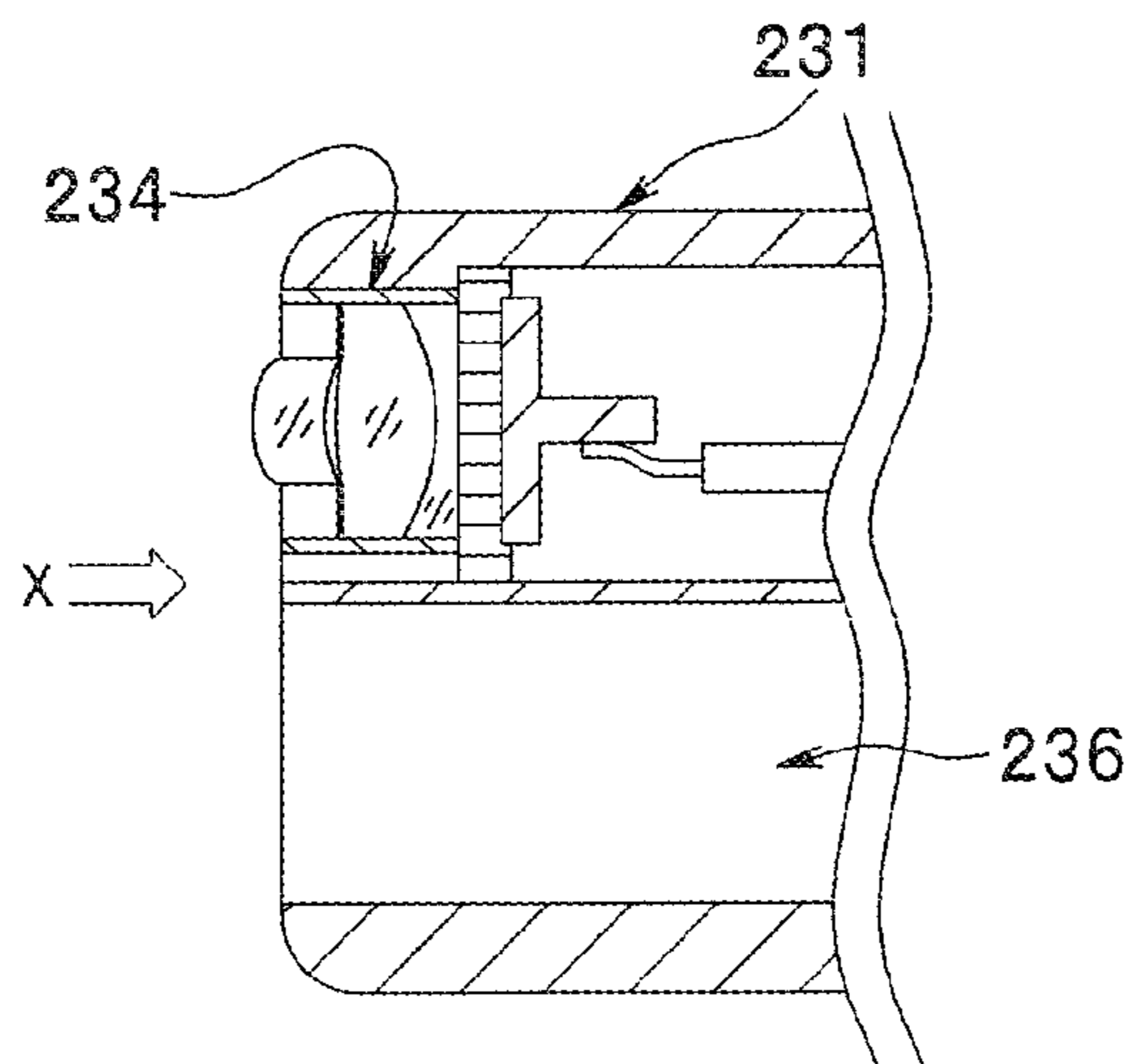
FIG.3 (PRIOR ART)
