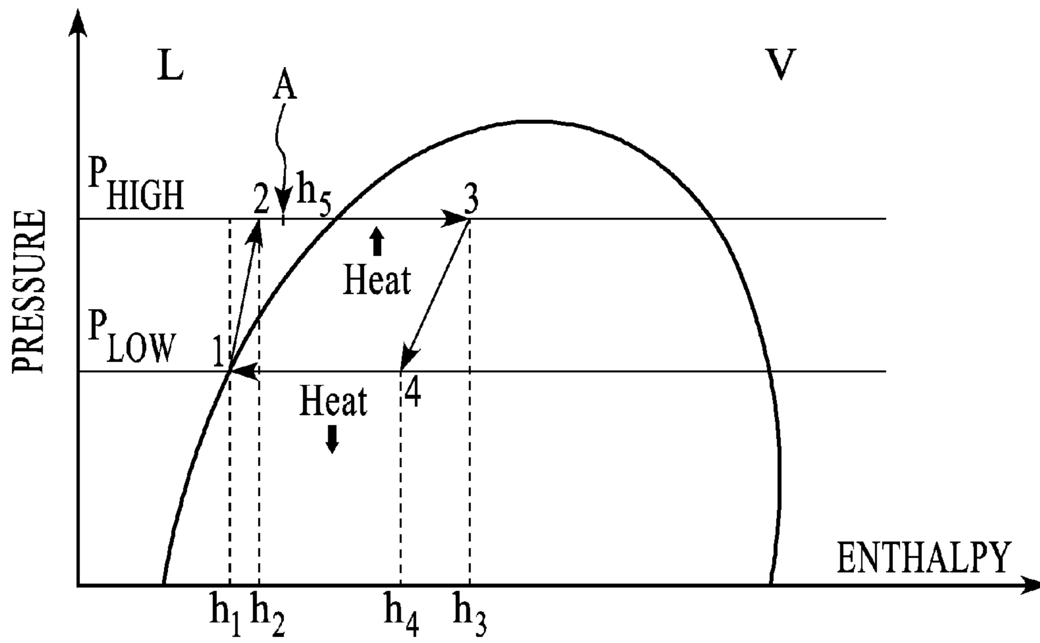
FIG. 2C (PRIOR ART)
