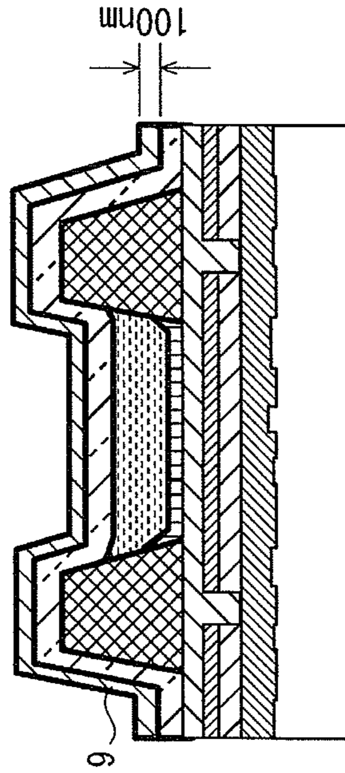
FIG. 23D Form cathode electrode
