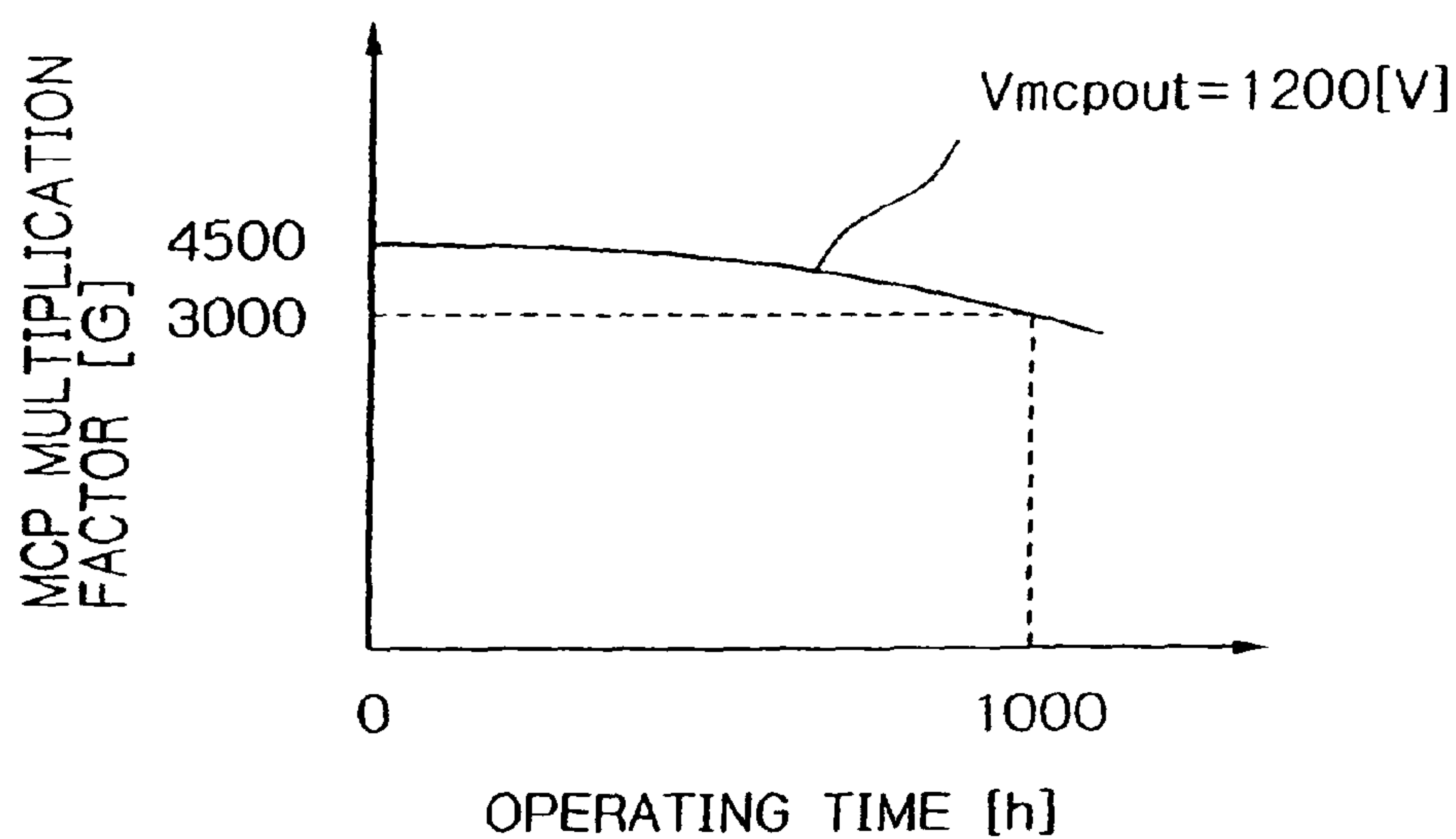
CORRELATION BETWEEN OPERATING TIME AND MCP MULTIPLICATION FACTOR
