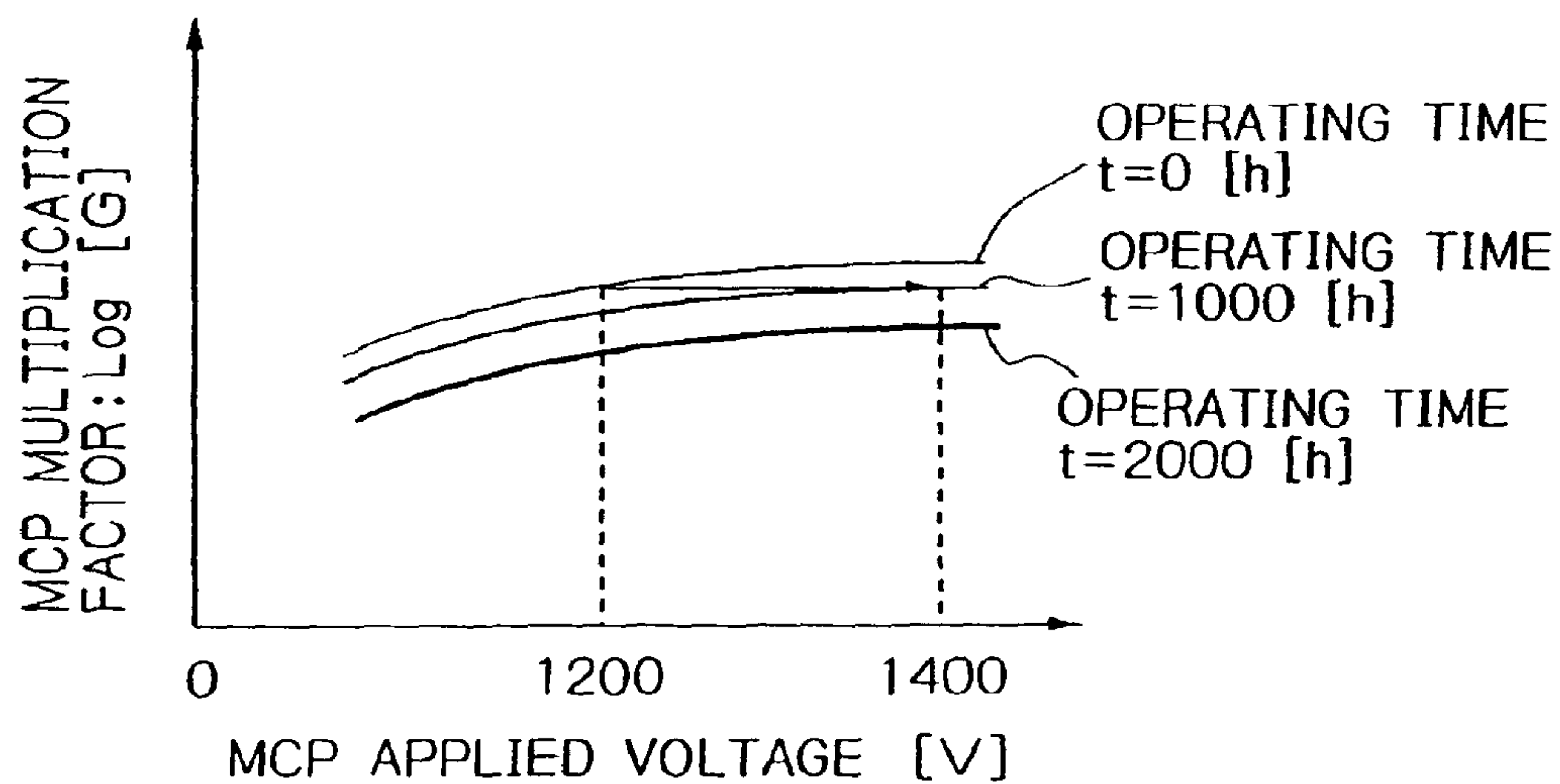
CORRELATION BETWEEN MCP APPLIED VOLTAGE AND MCP MULTIPLICATION FACTOR
