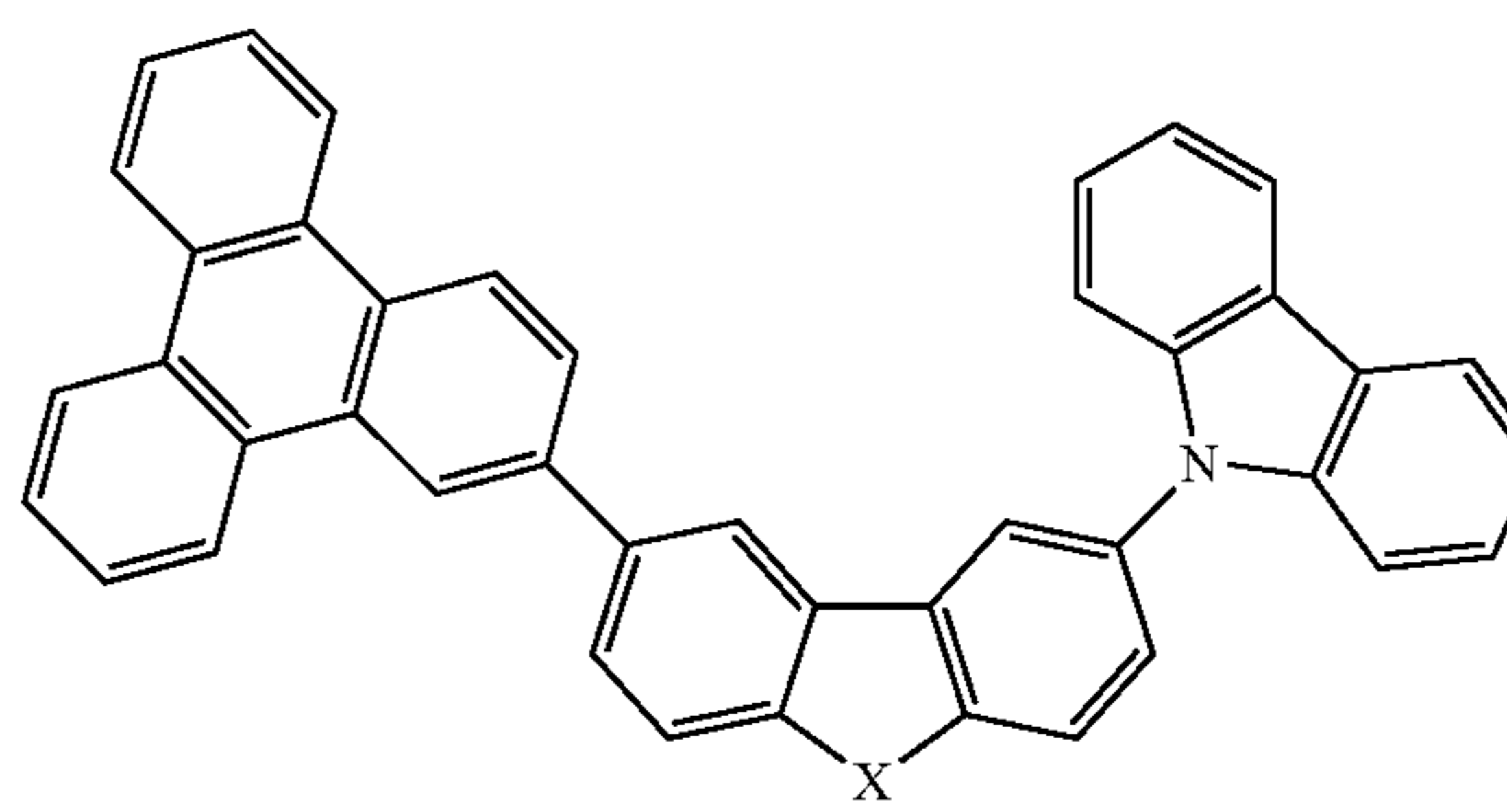
Compound 15
