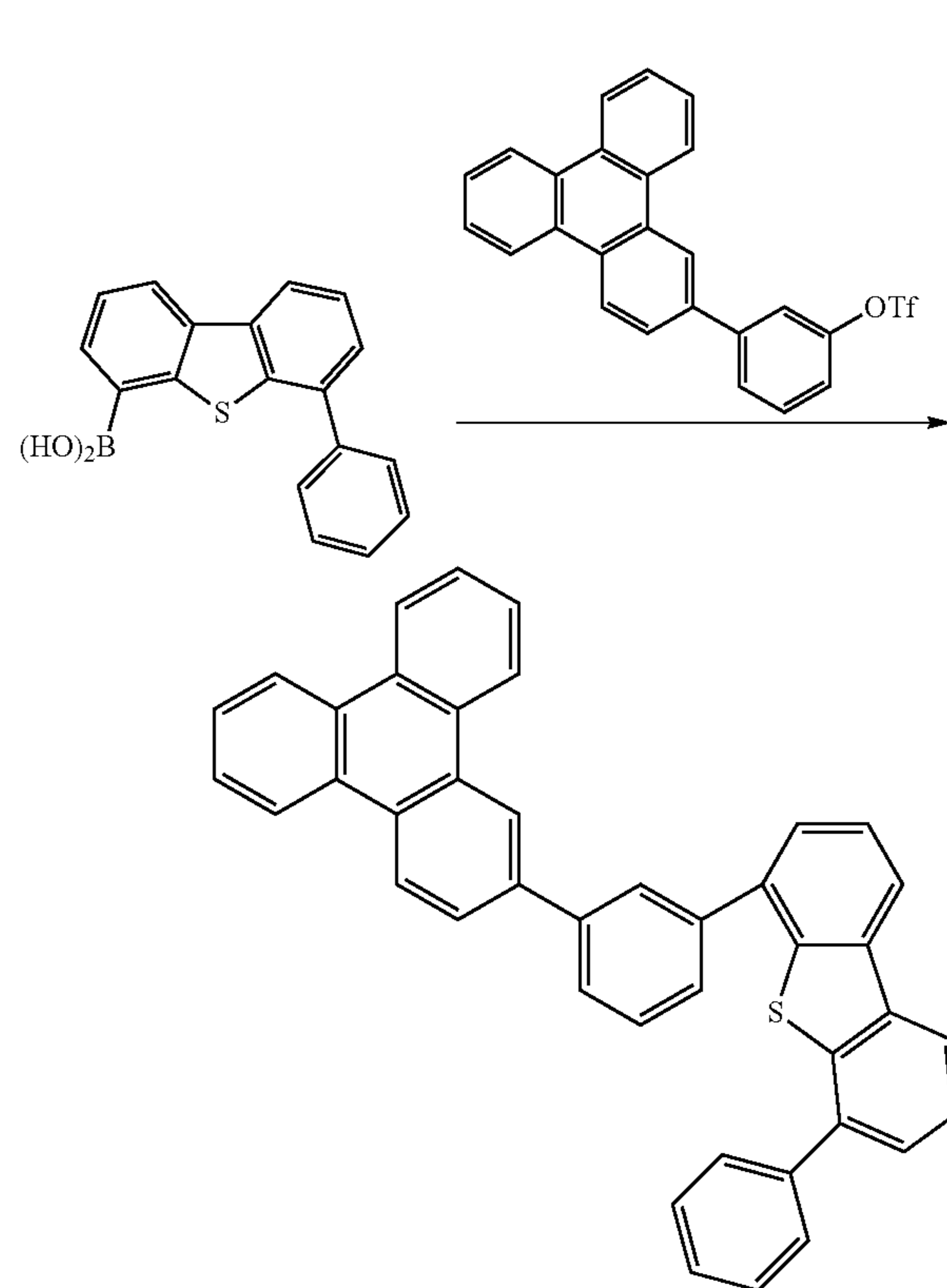
Compound 23S
