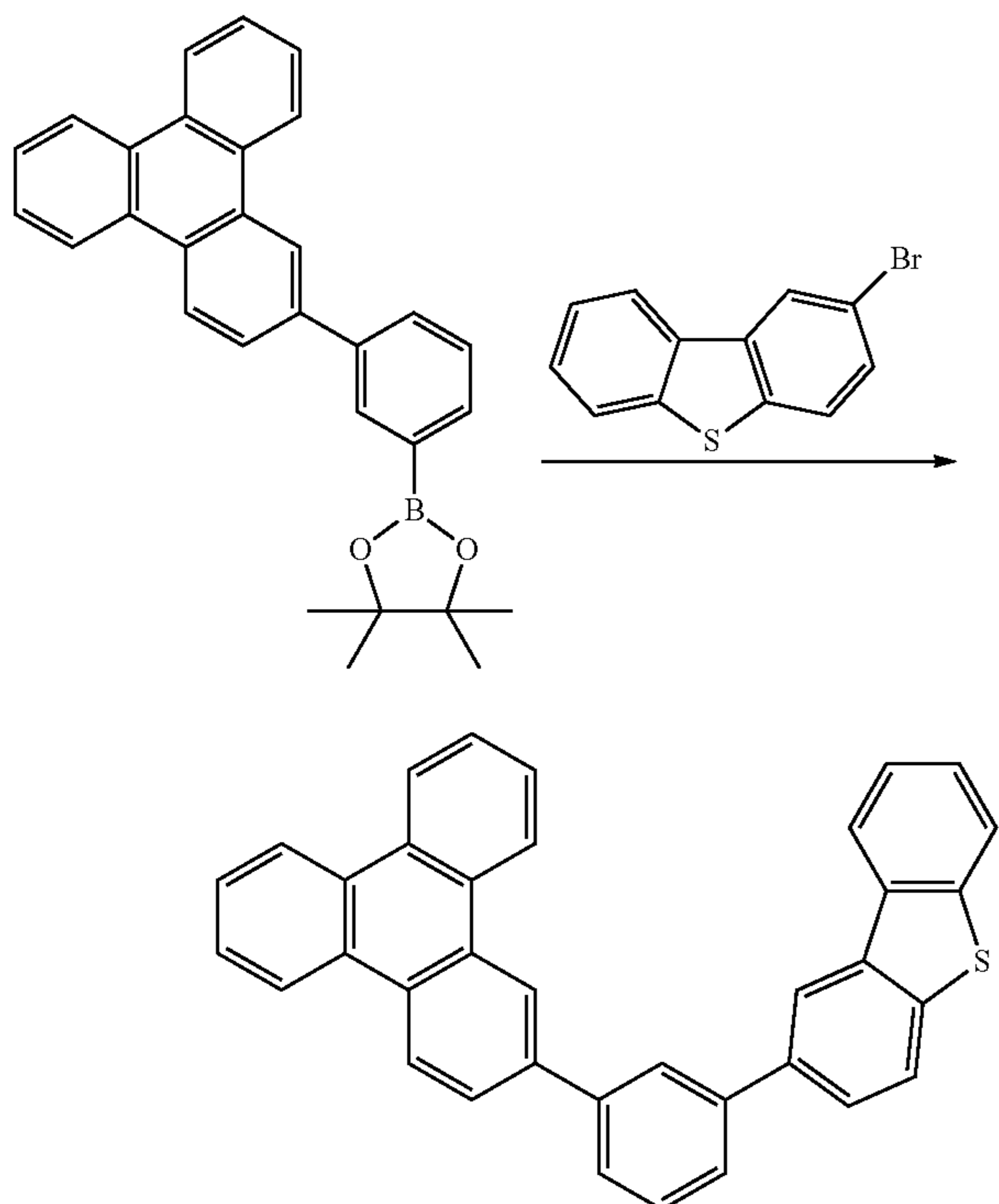
Compound 20S
