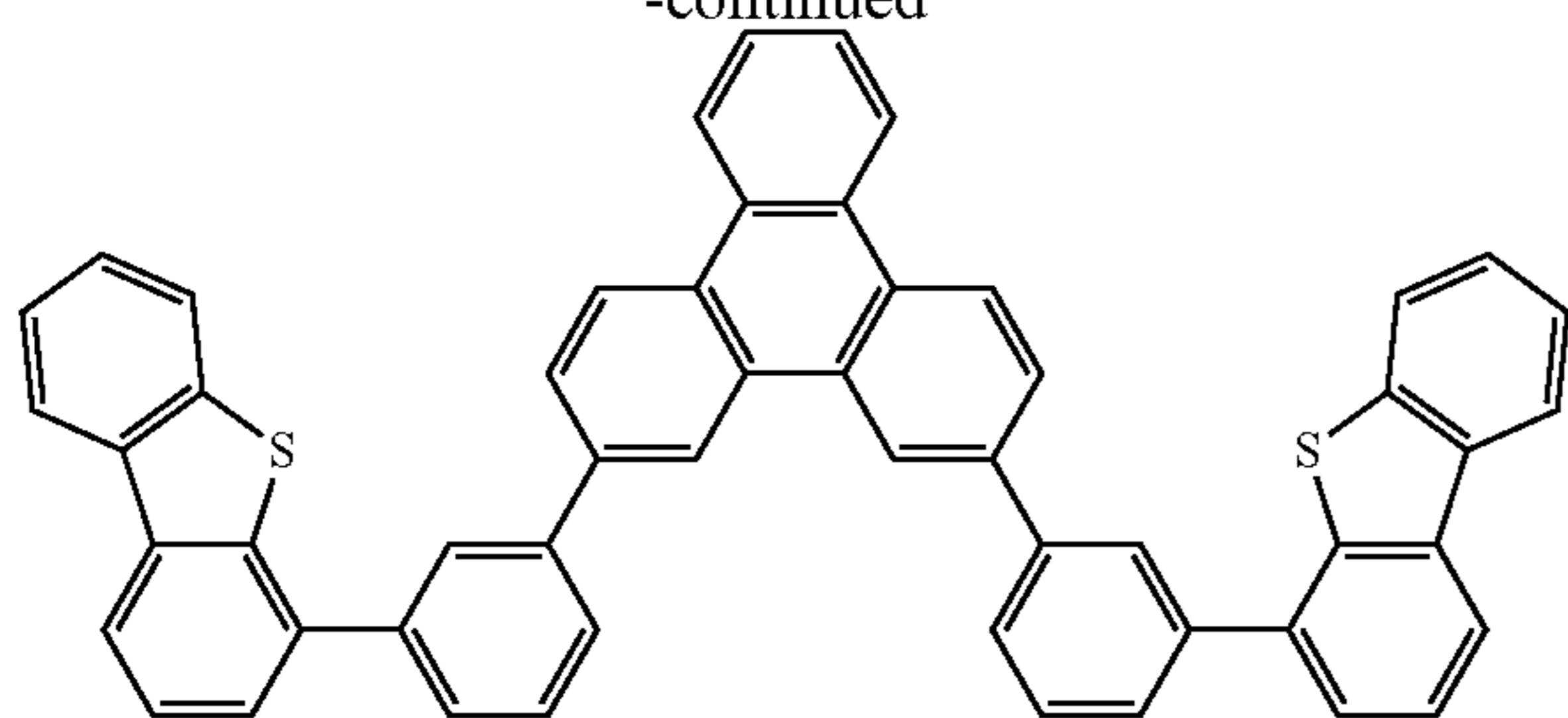
Compound 4S
