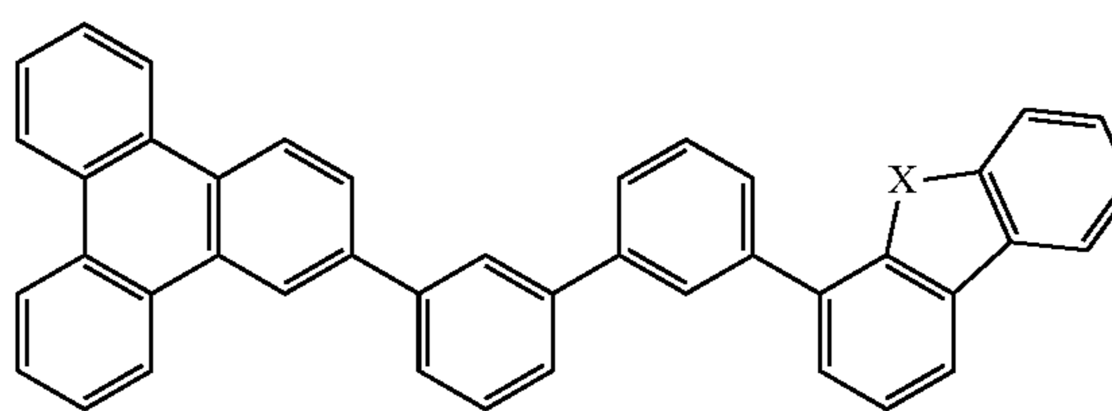
Compound 9
