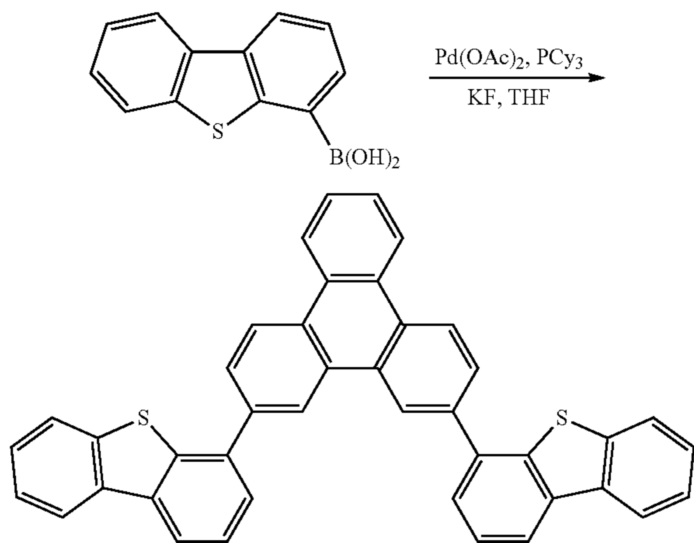
Compound 10S
