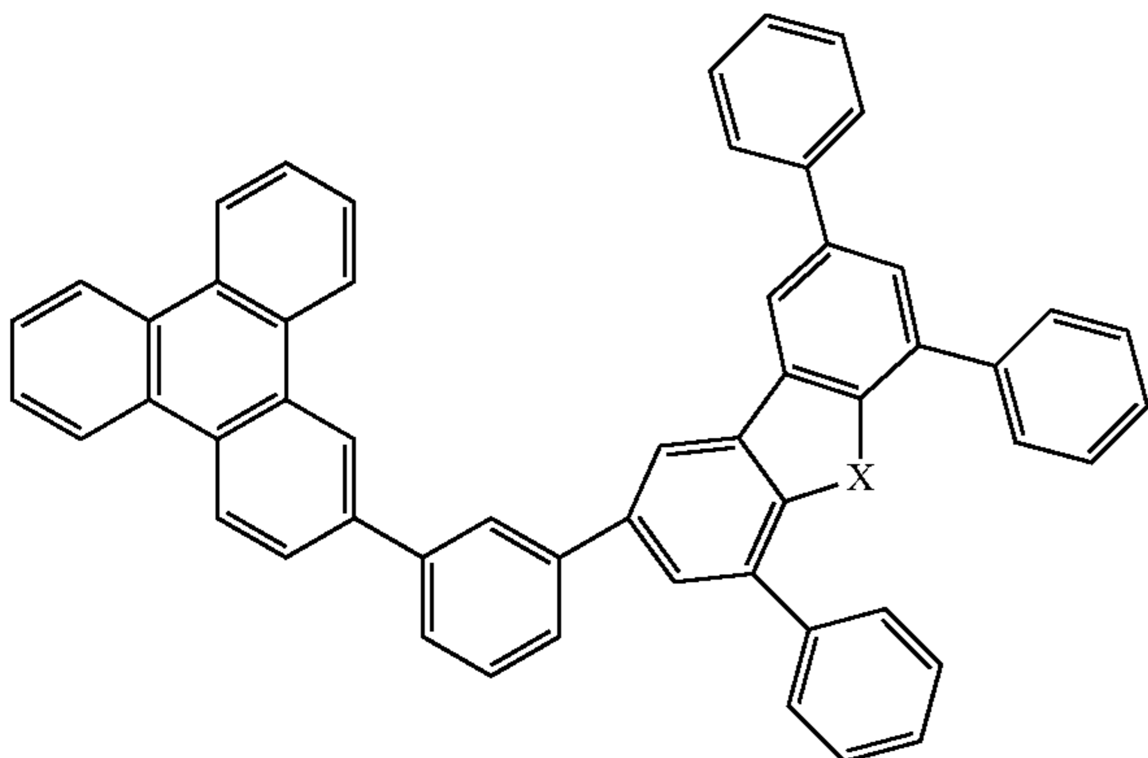
Compound 36
