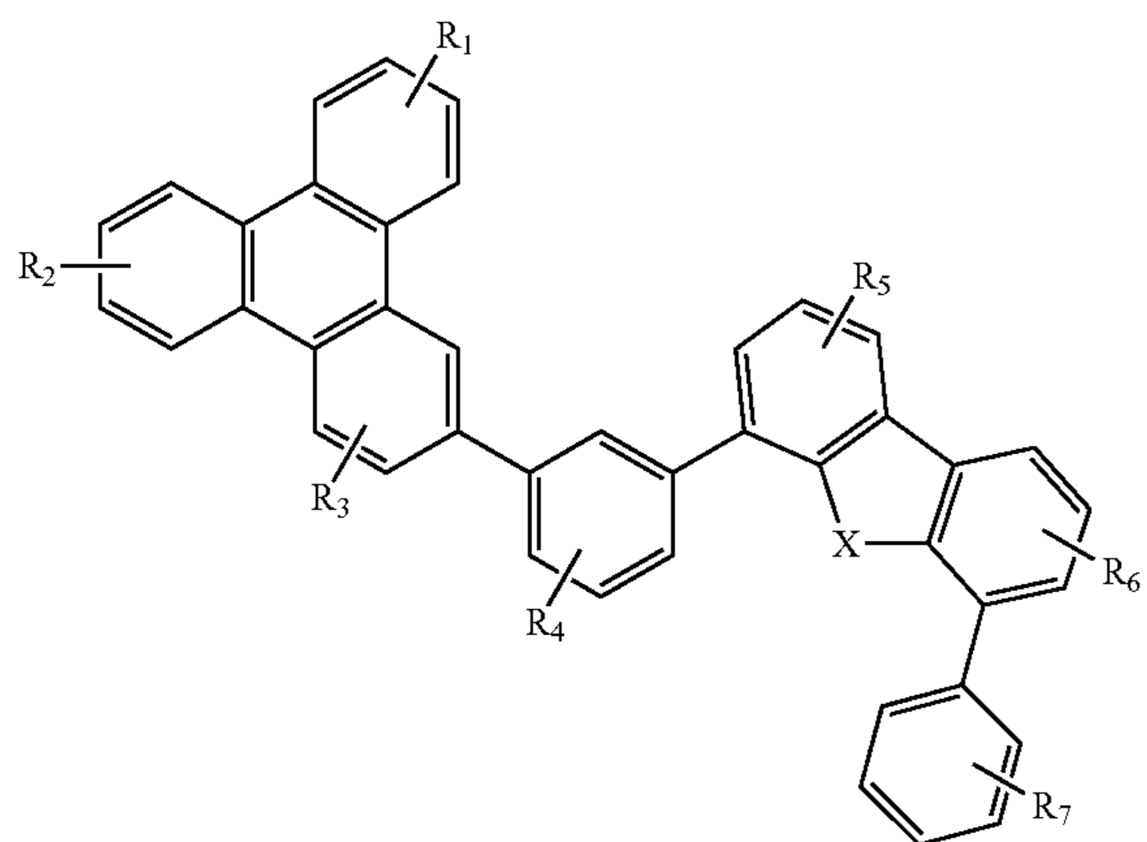
Compound 23 G
