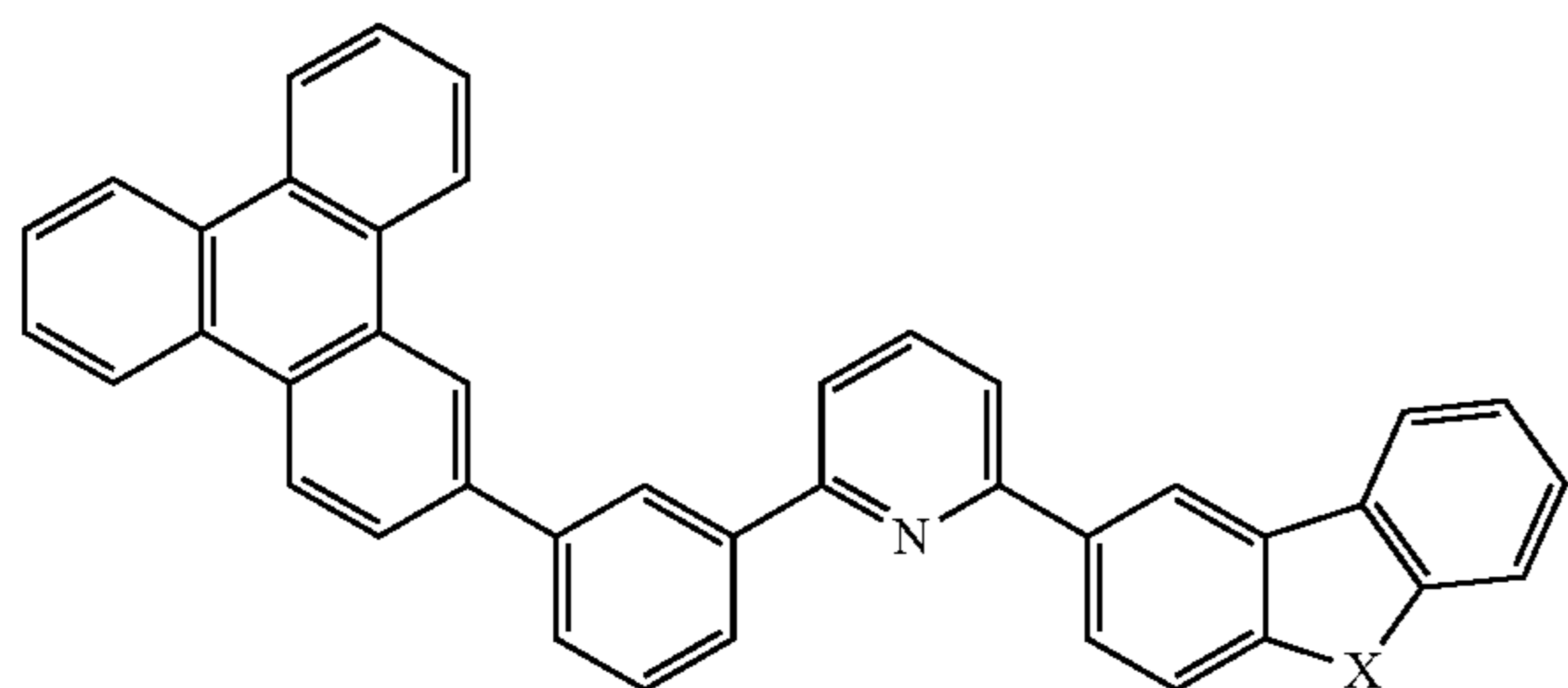
Compound 44
