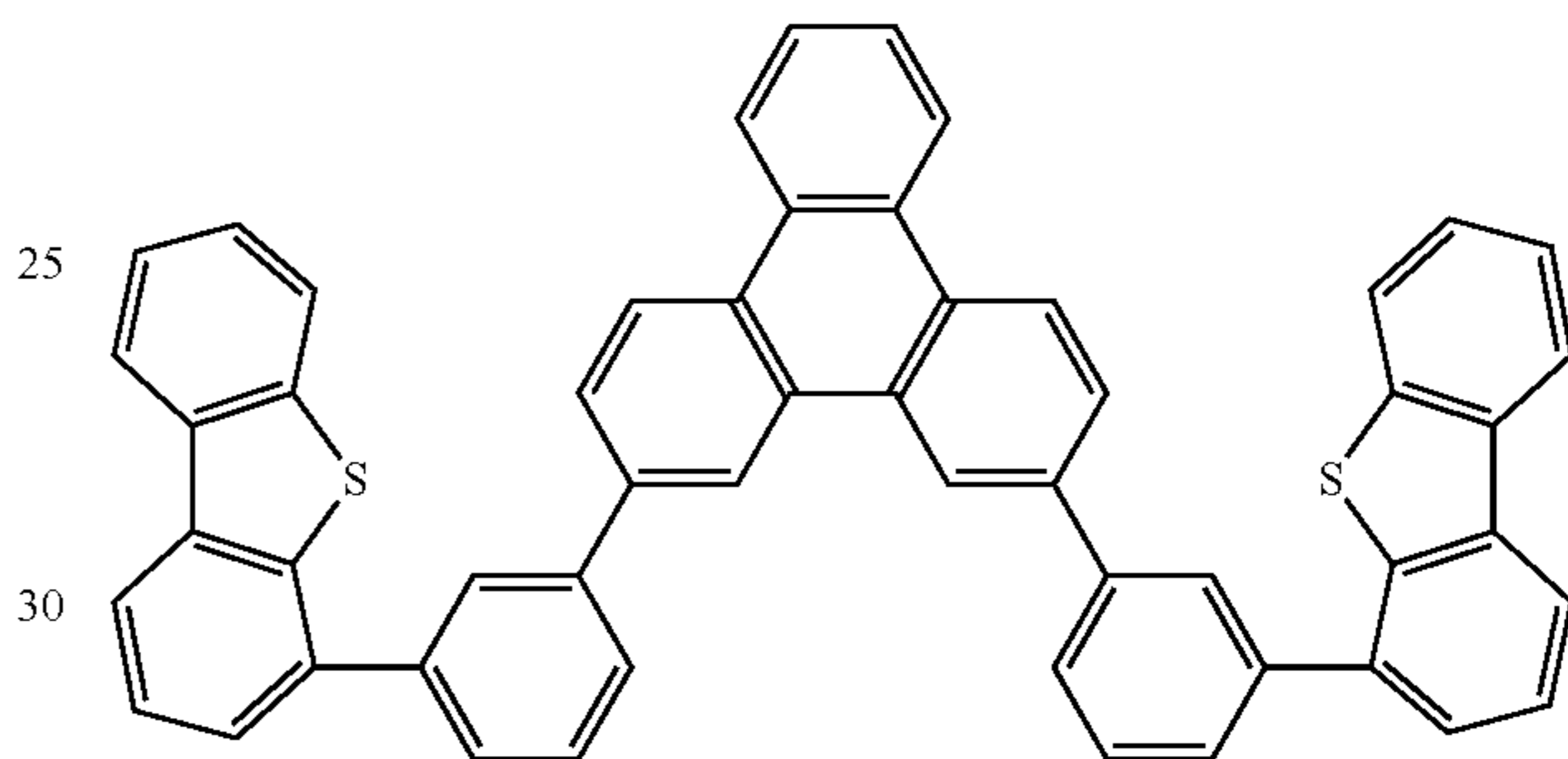
Compound 4'
