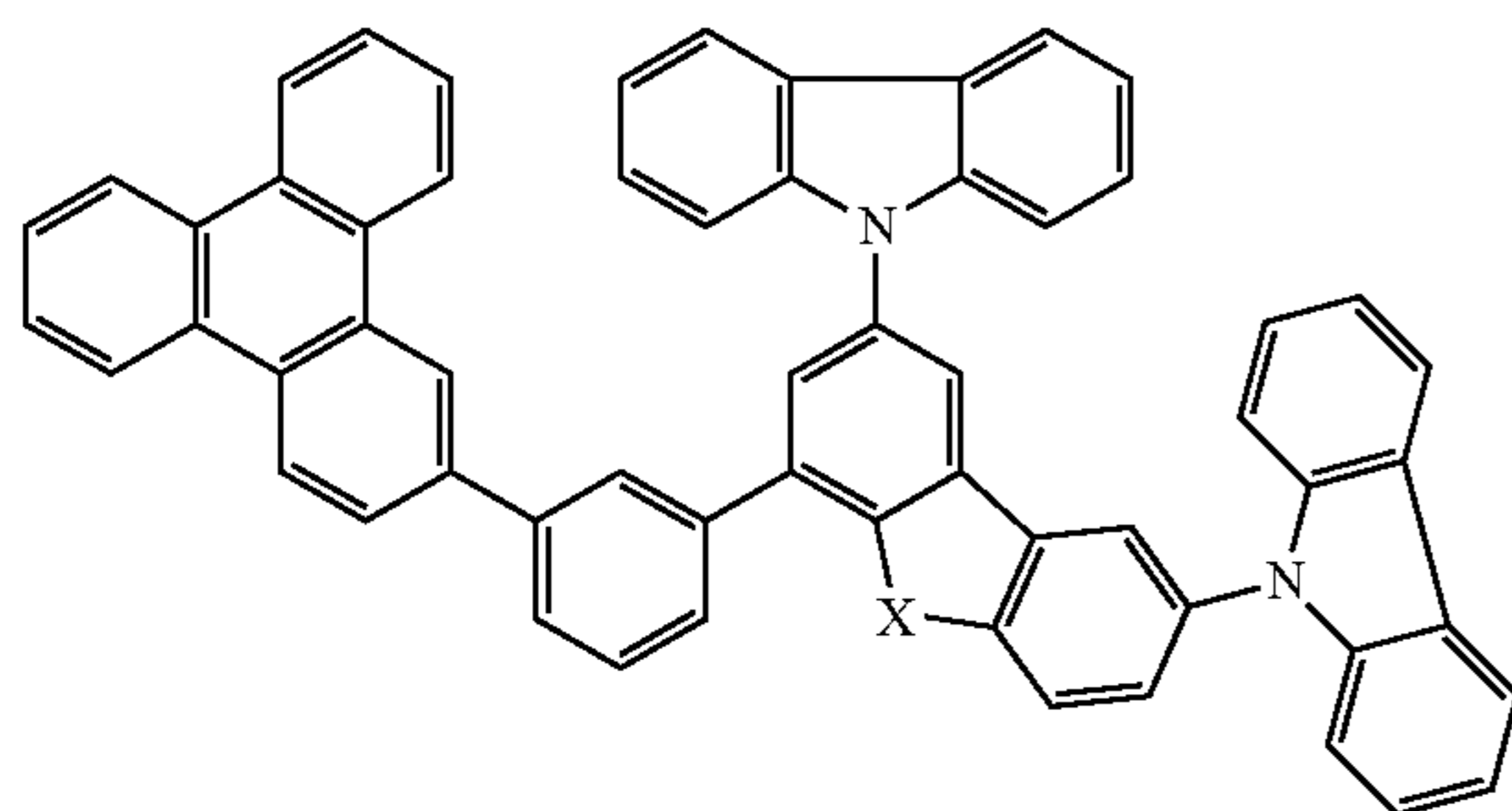
Compound 27
