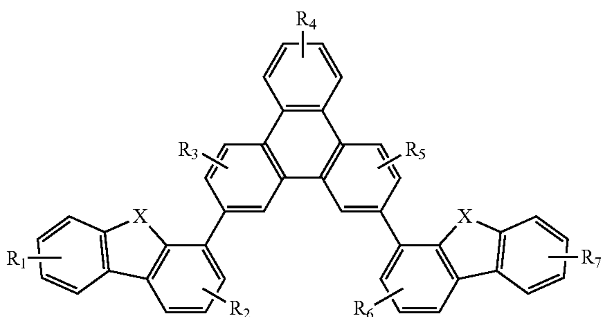
Compound 15G
