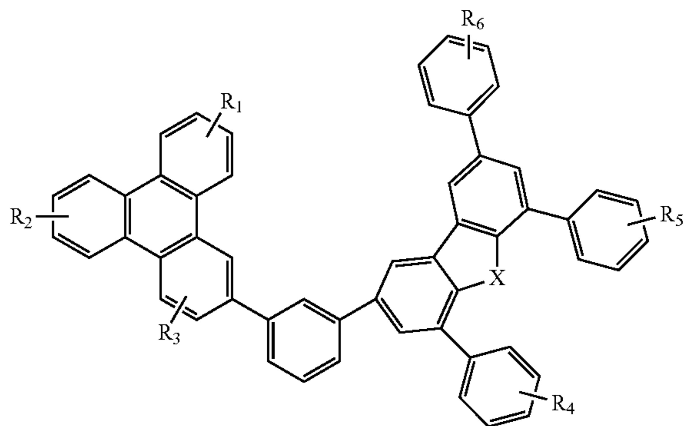
Compound 37G
