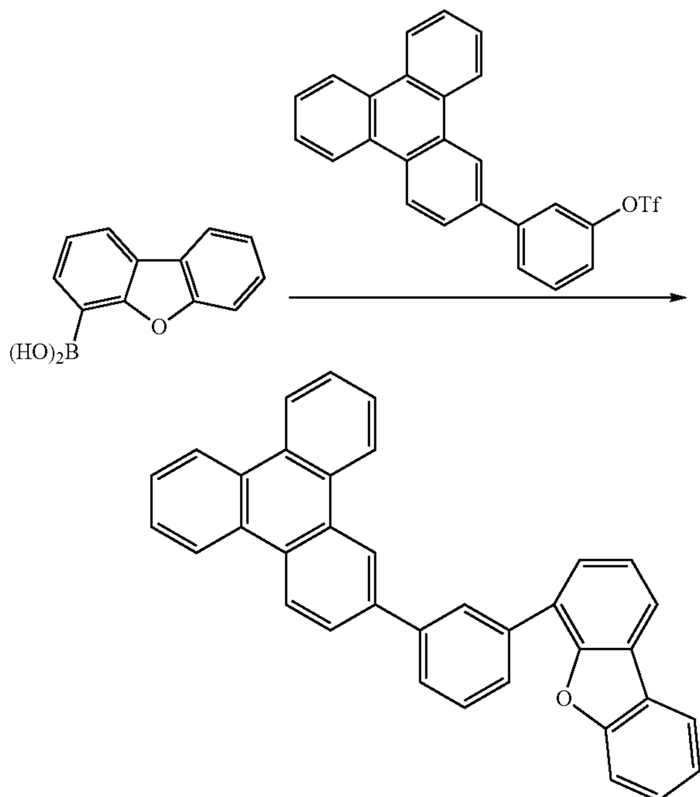
Compound 20
