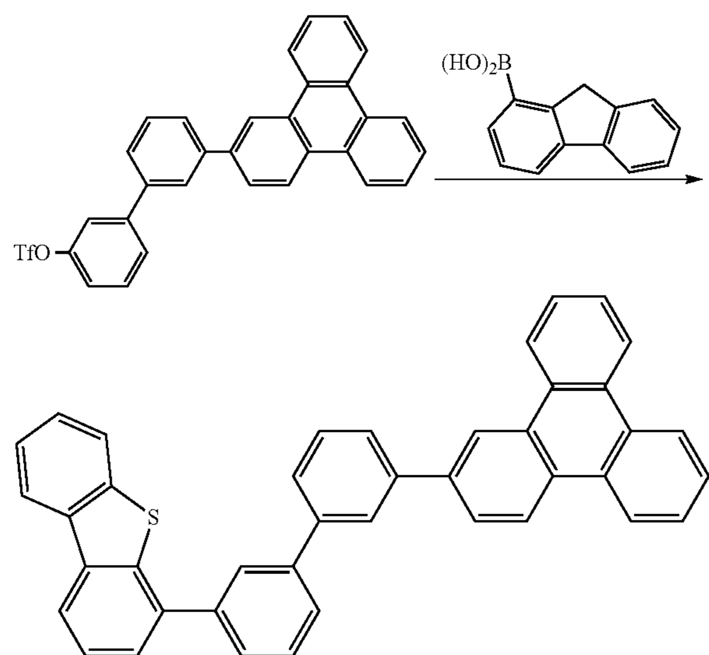
Compound 9S
