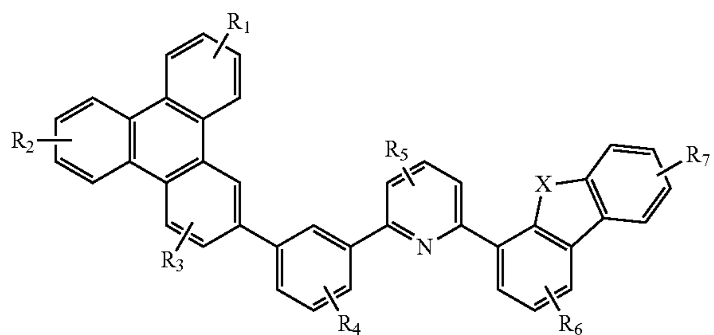
Compound 21 G
