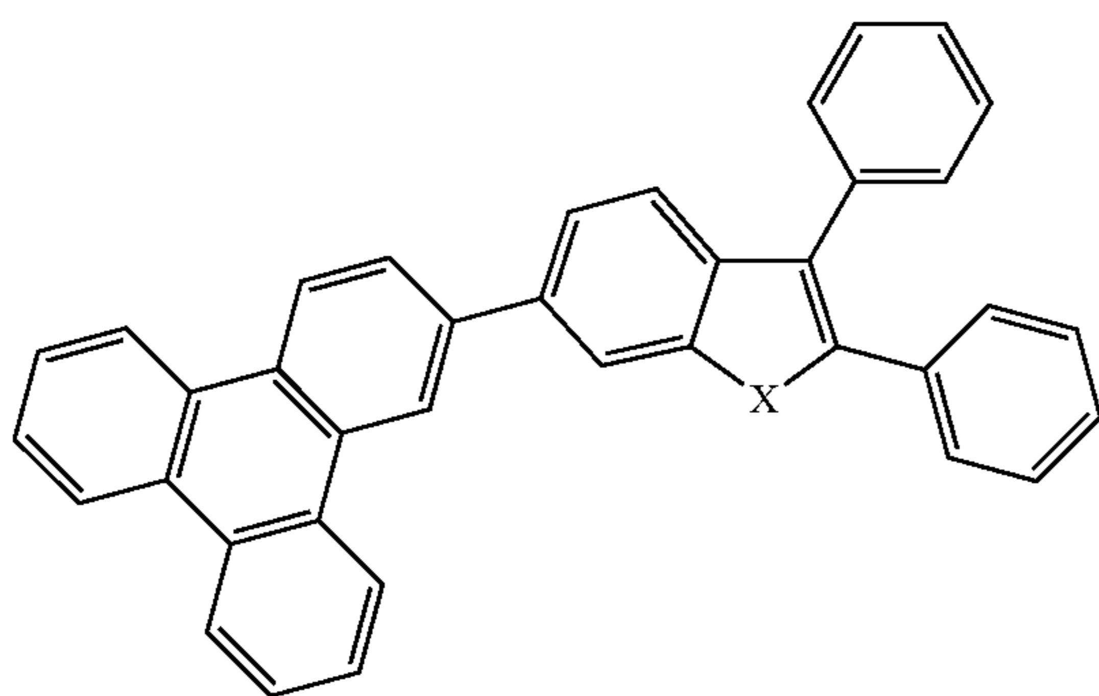
Compound 17
