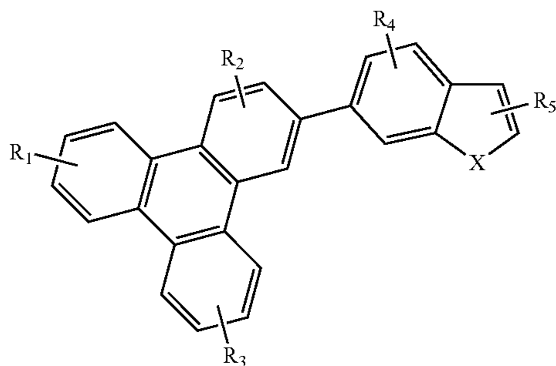
Compound 17G
