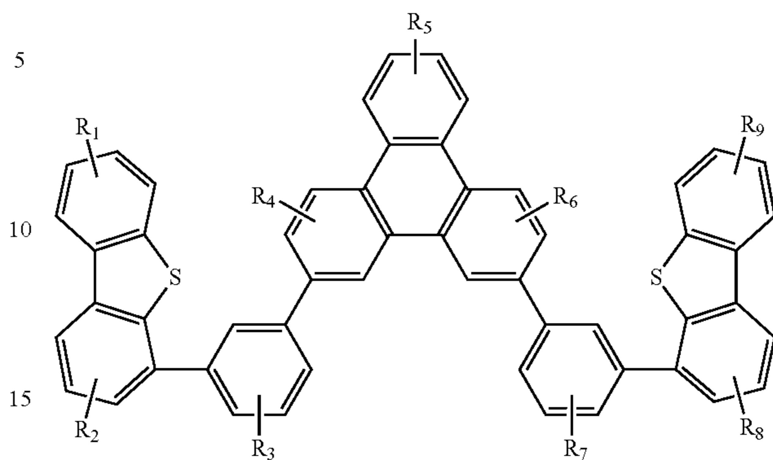
Compound 4'G
