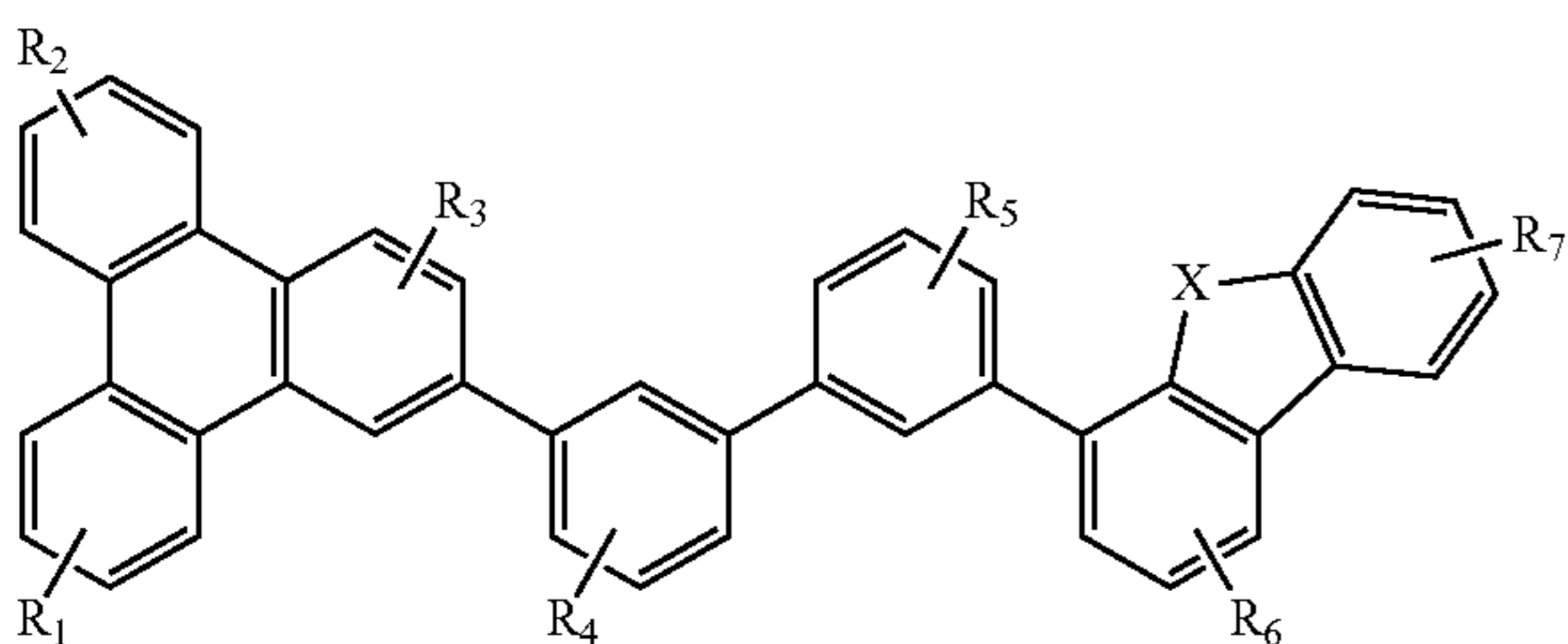
Compound 10G
