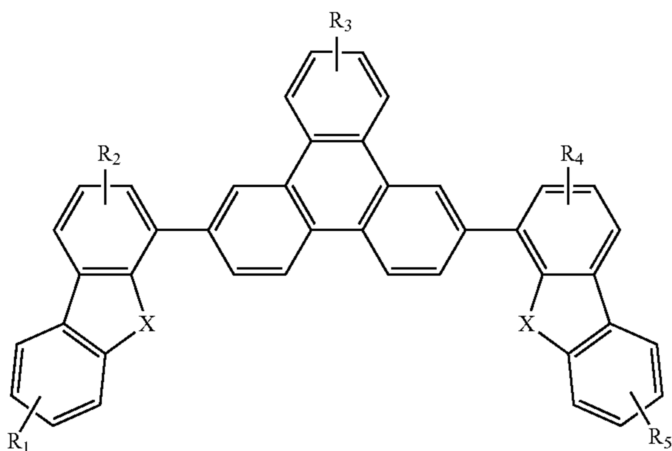
Compound 19 G
