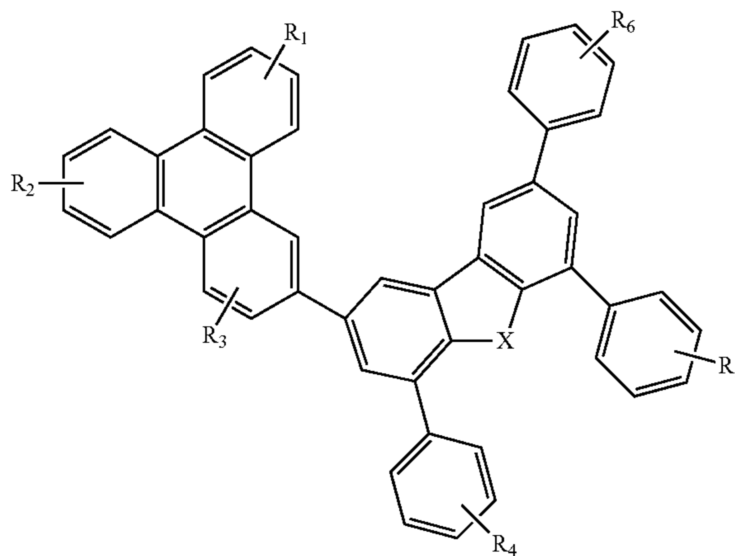
Compound 36G
