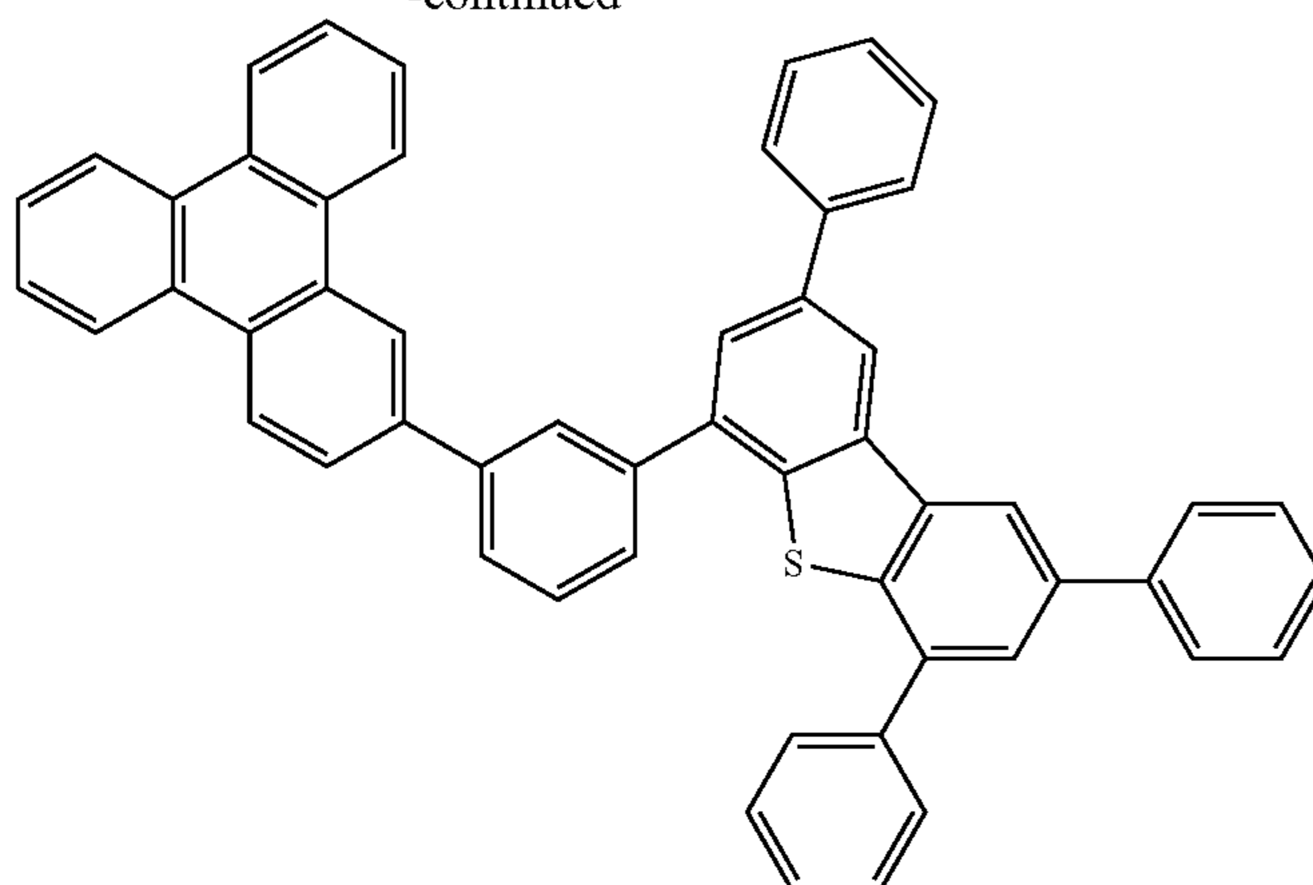
Compound 25S
