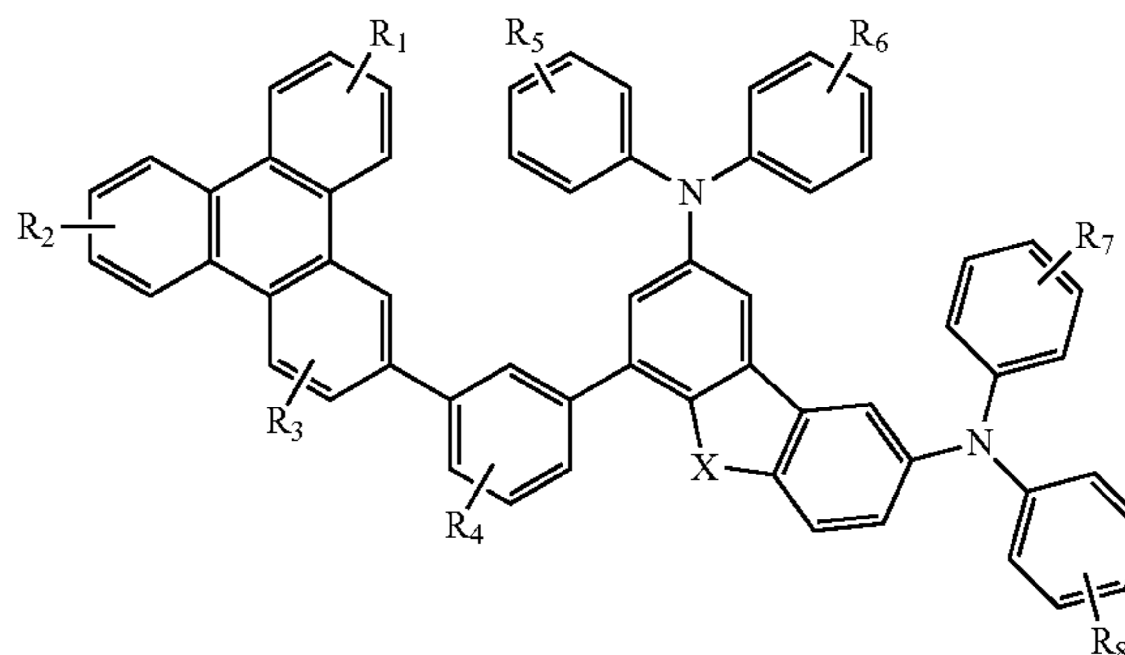
Compound 28G
