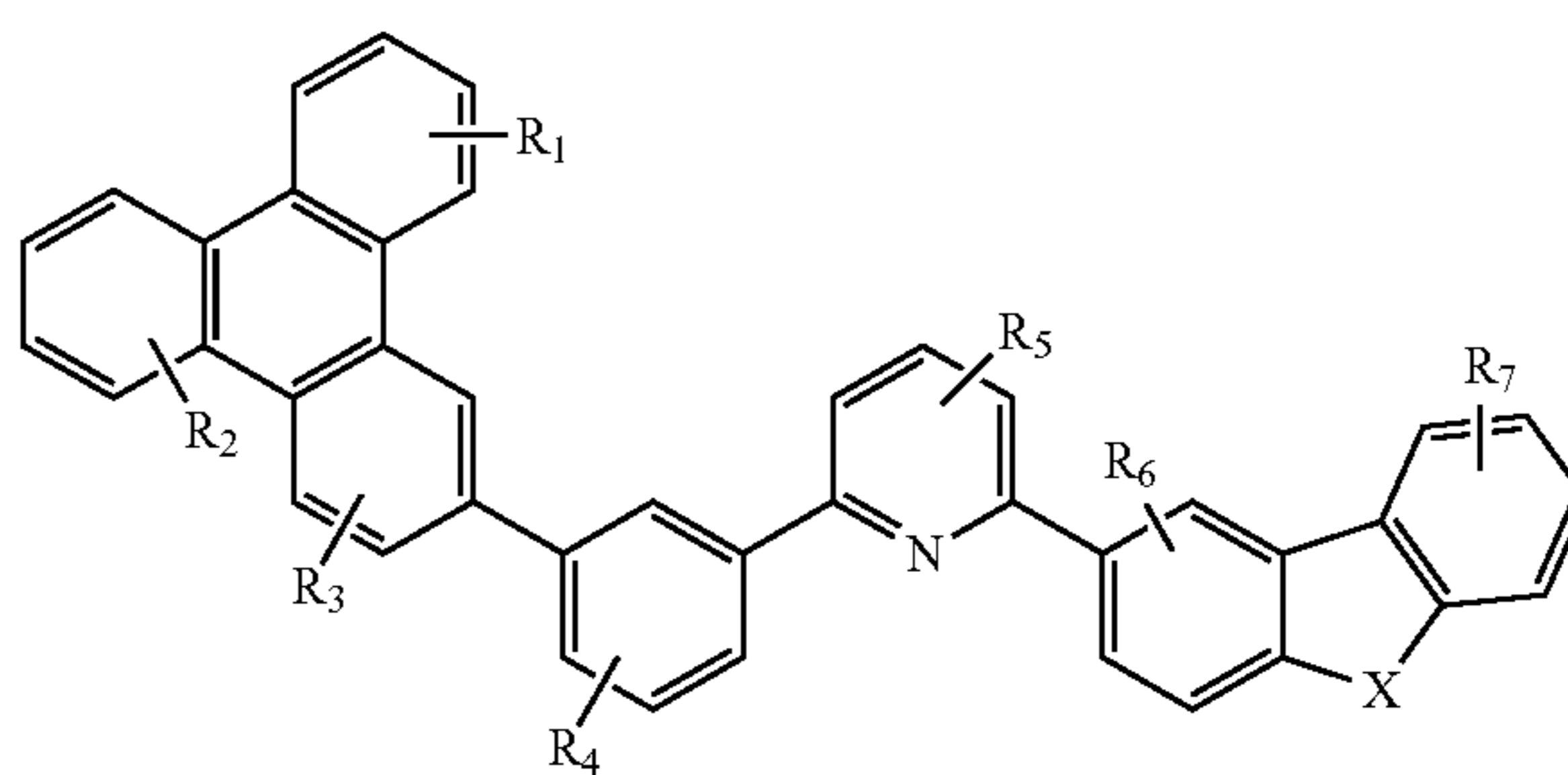
Compound 44G
