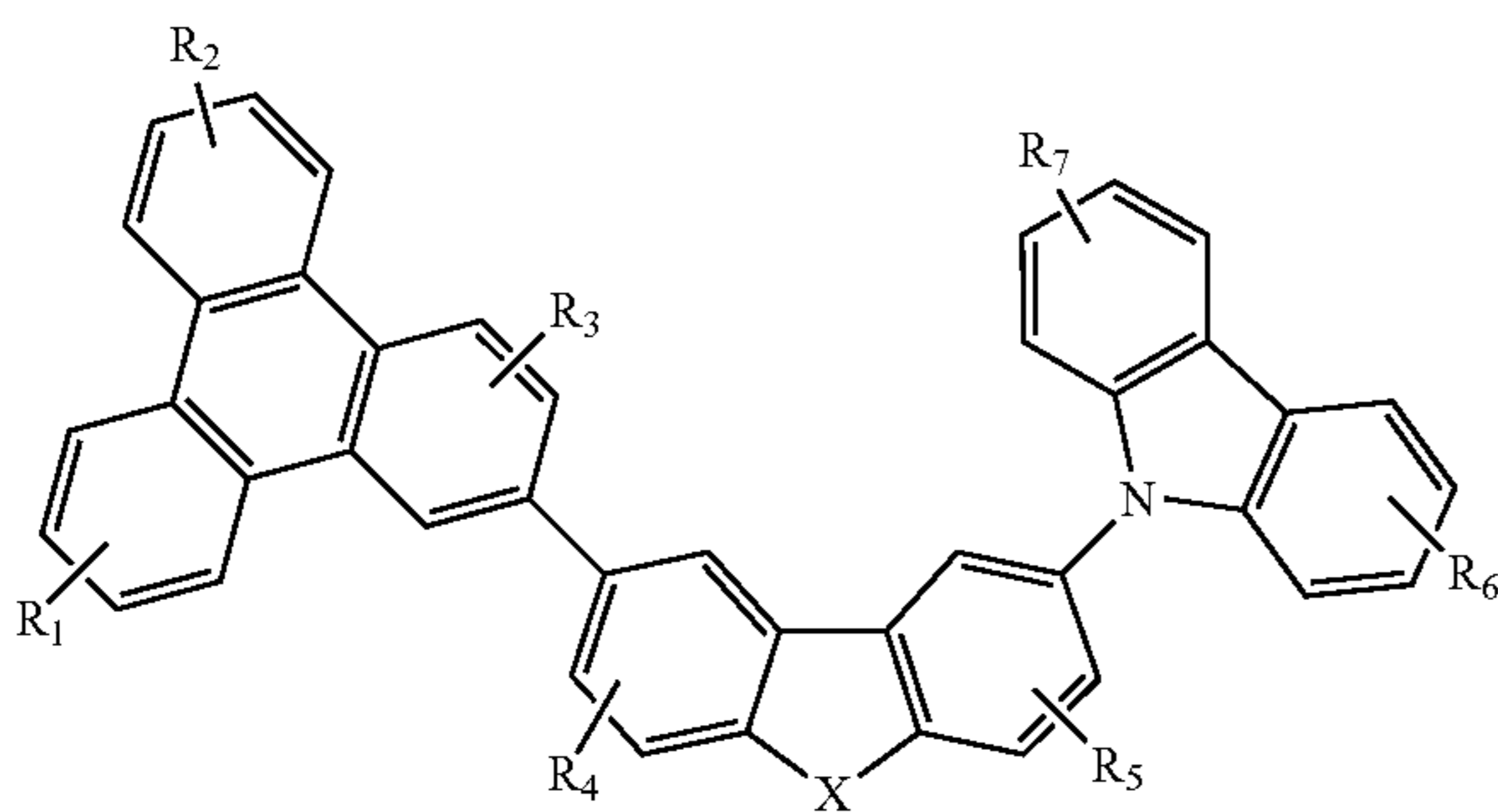
Compound 19 G
