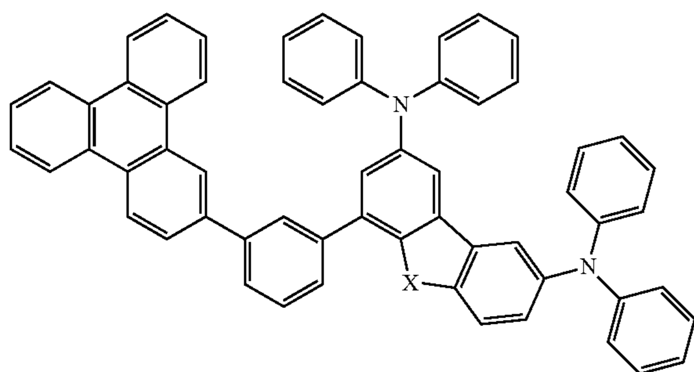
Compound 28
