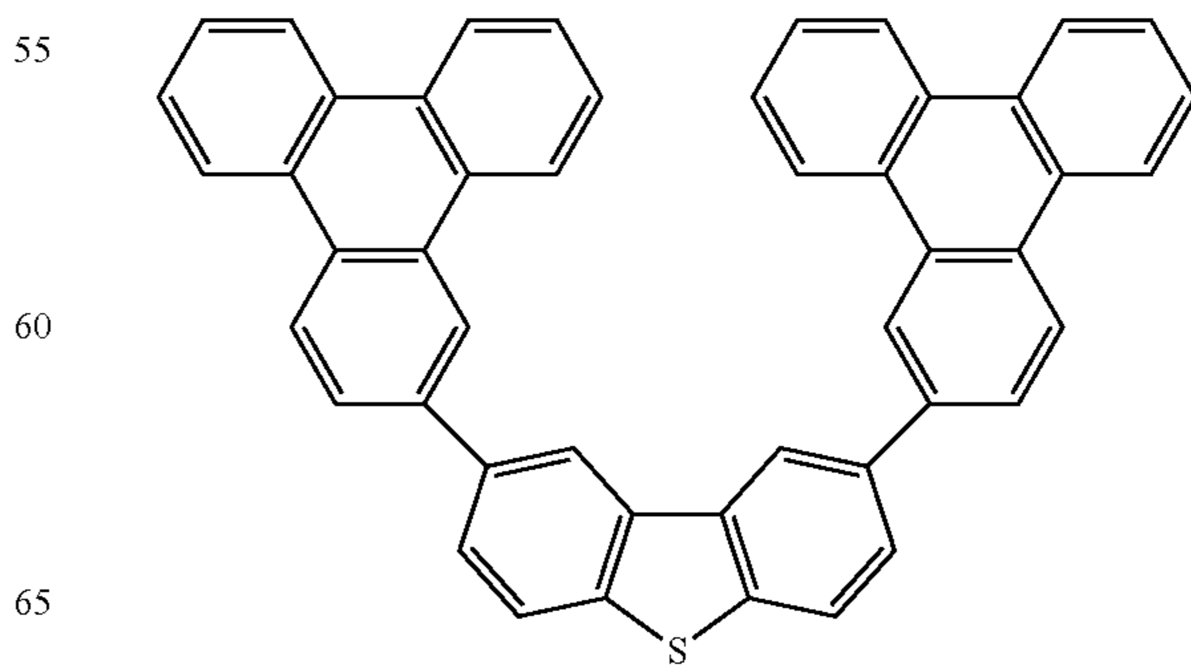
Compound 5'
