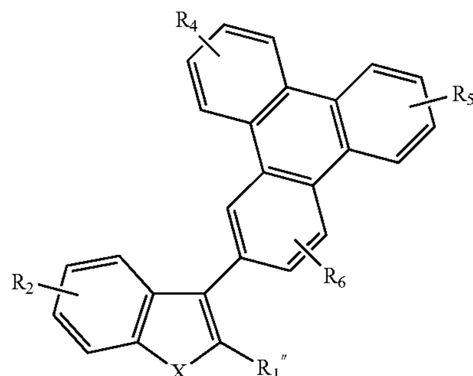
Compound 13G 5
