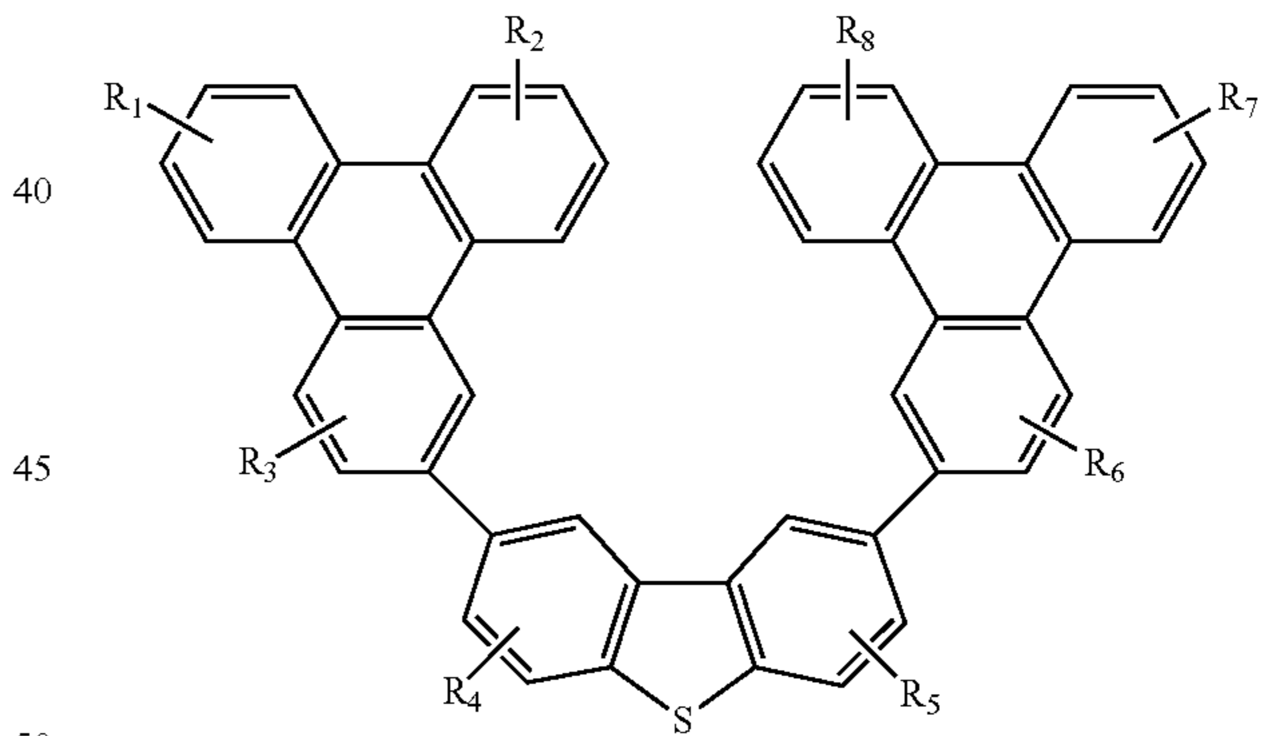
Compound 5'G
