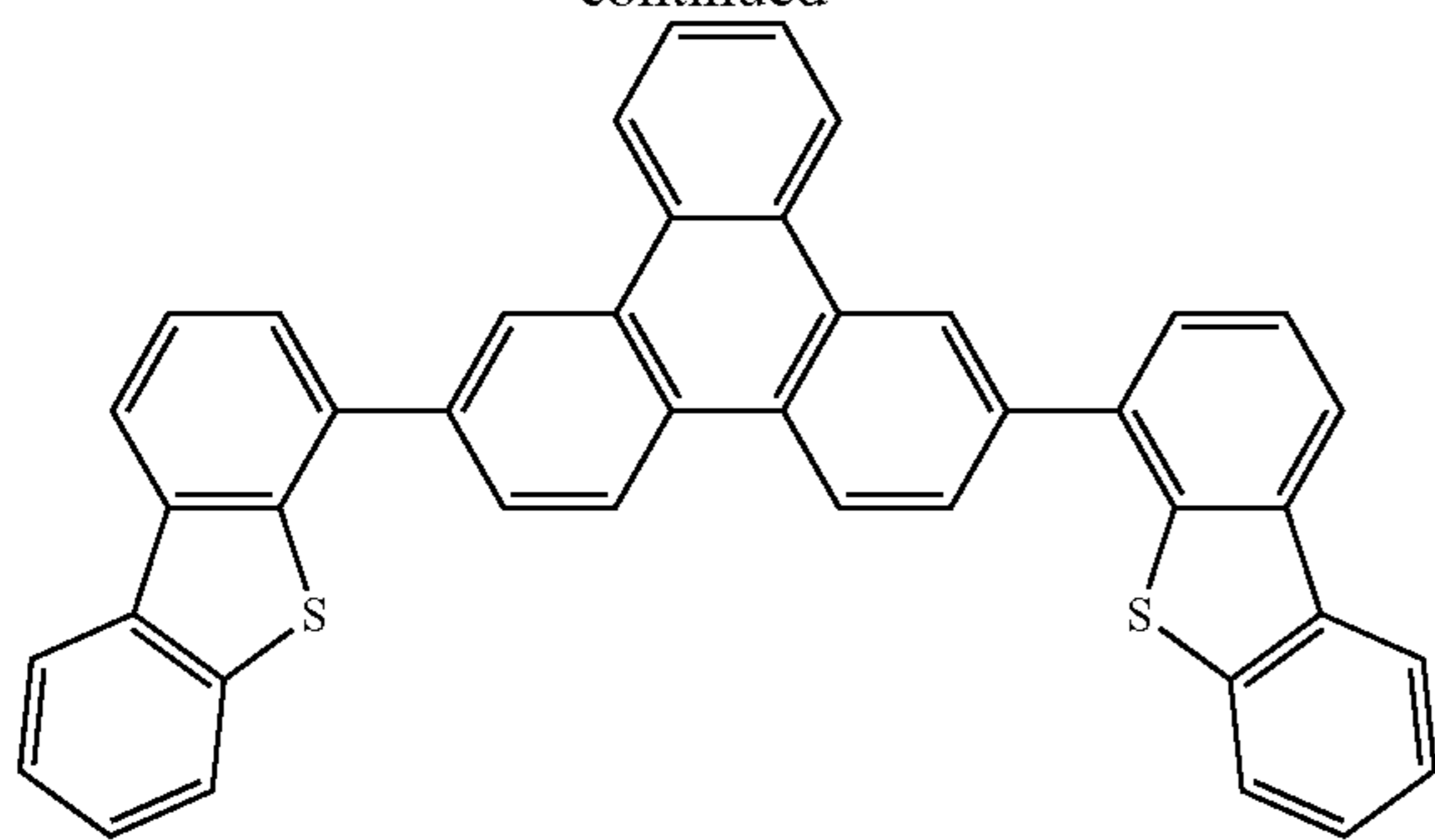
Compound 19S
