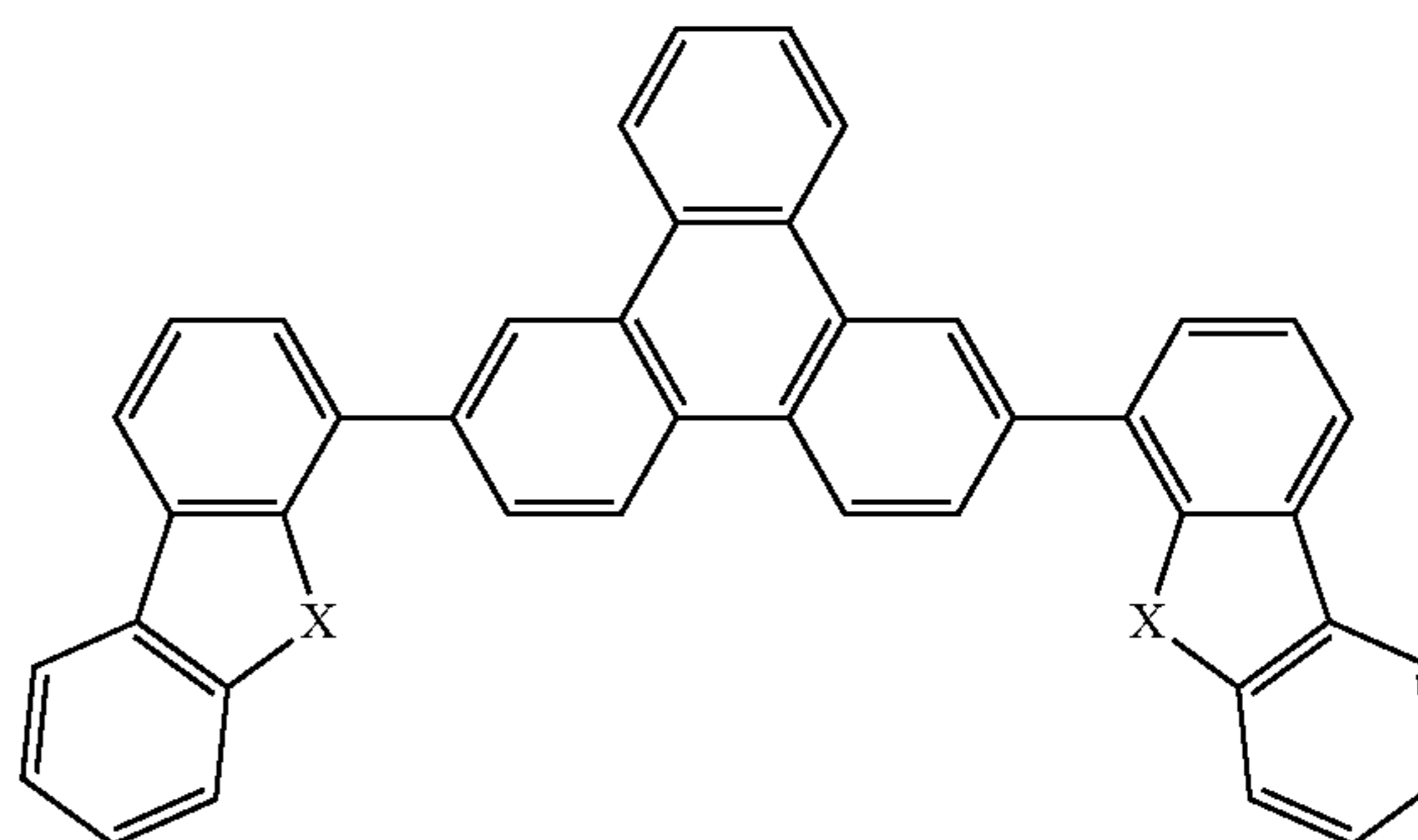
Compound 19
