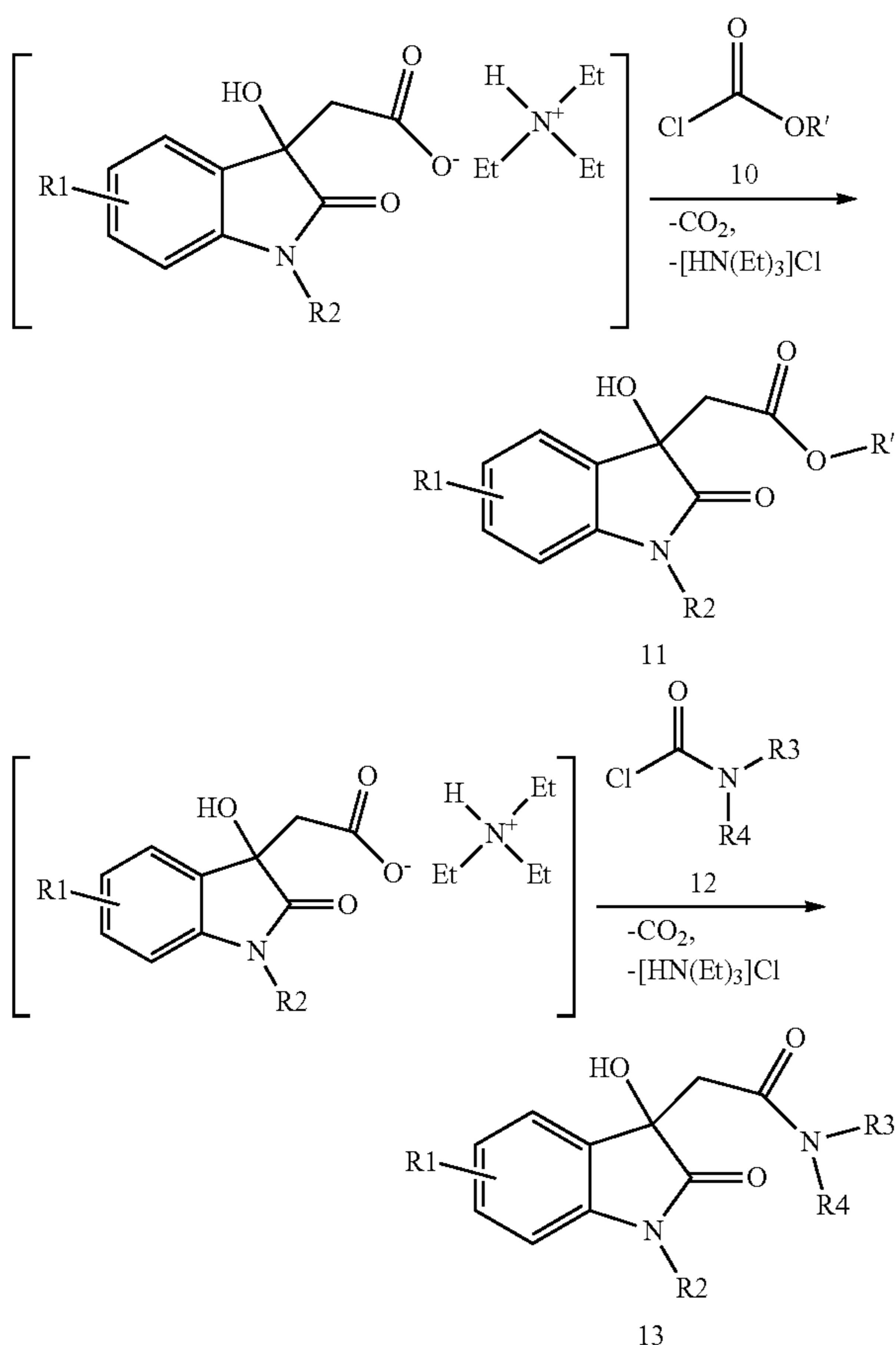
Scheme 7: Synthesis of esters 11 and amides 13 or 9
