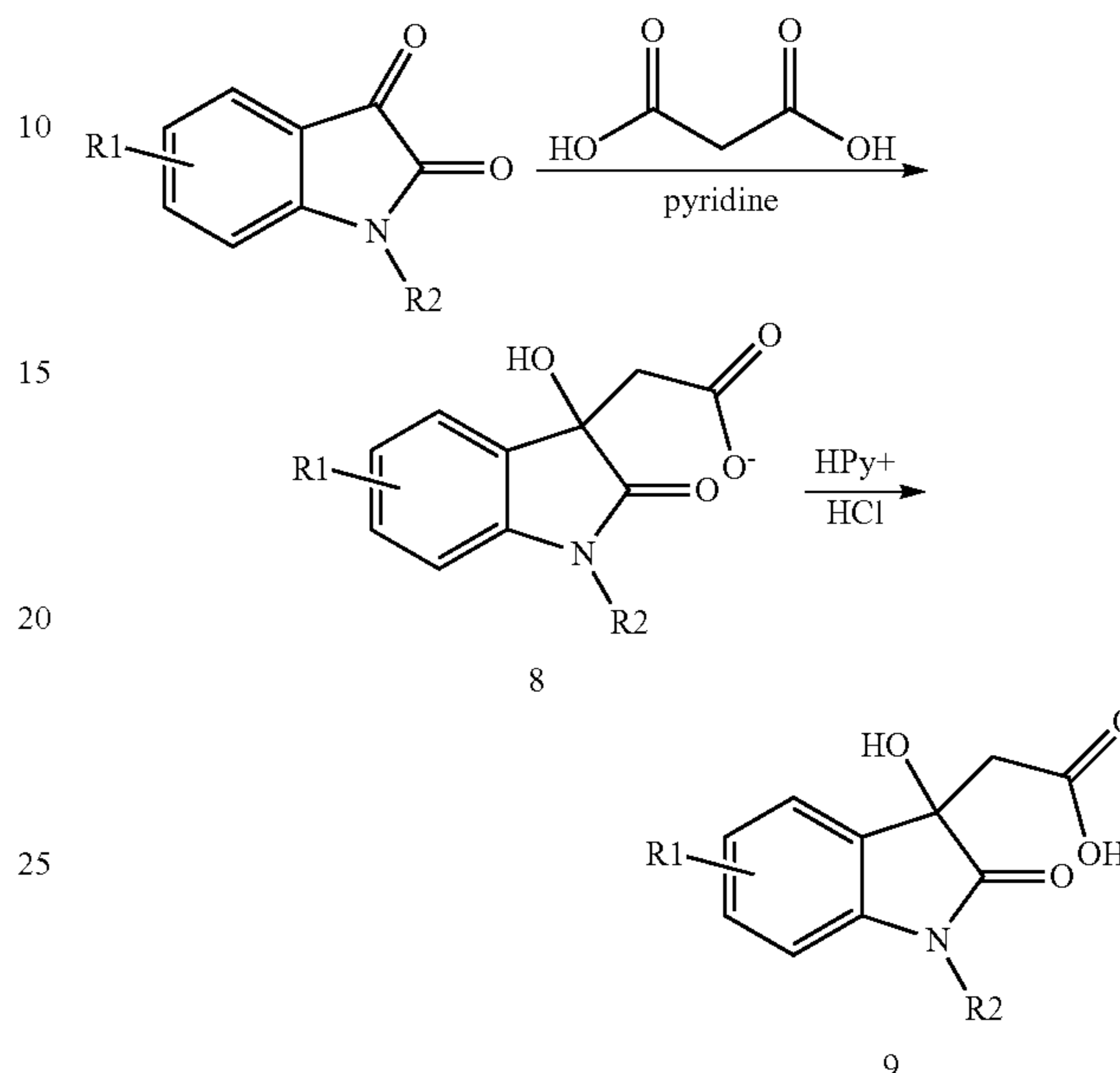
Scheme 6: Condensation of isatin with malonic acid in pyridine (R1 = hydrogen or lower alkyl)
