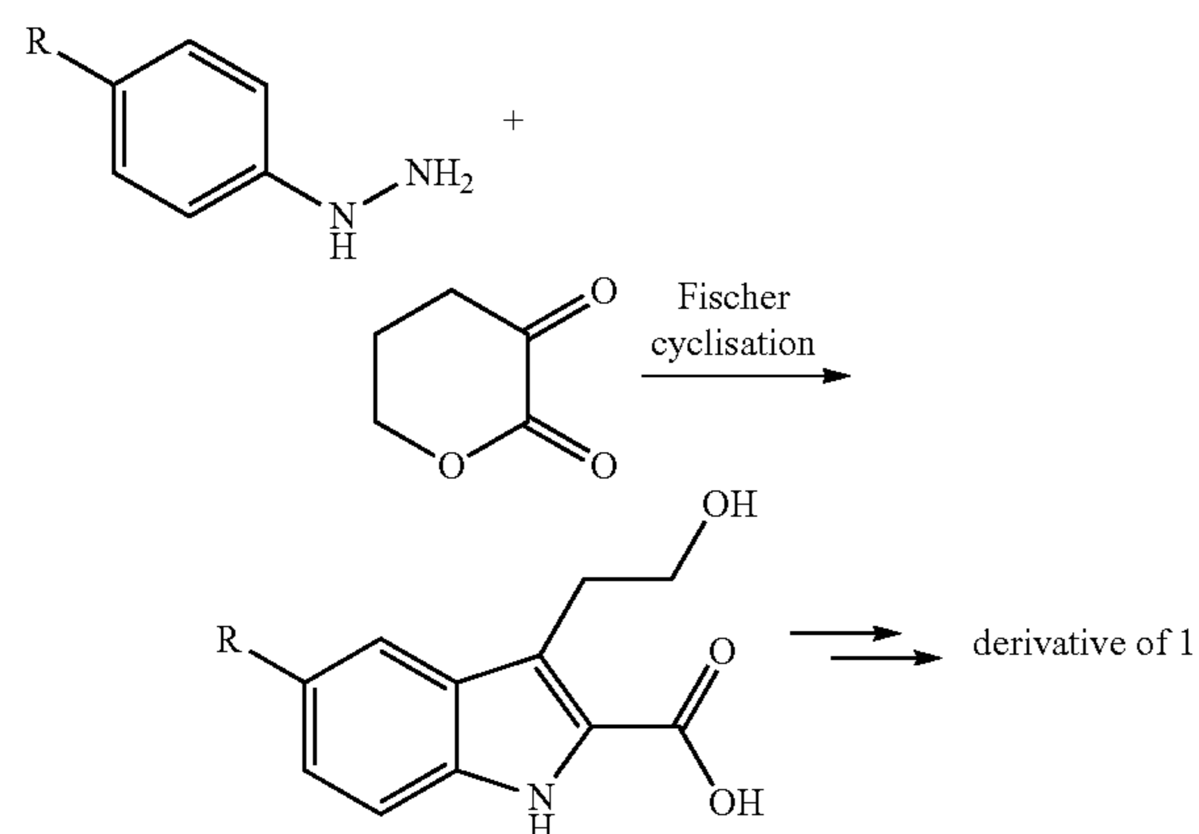
Scheme 3: Alternative Carbonyl compounds for the Fischer cyclisation
