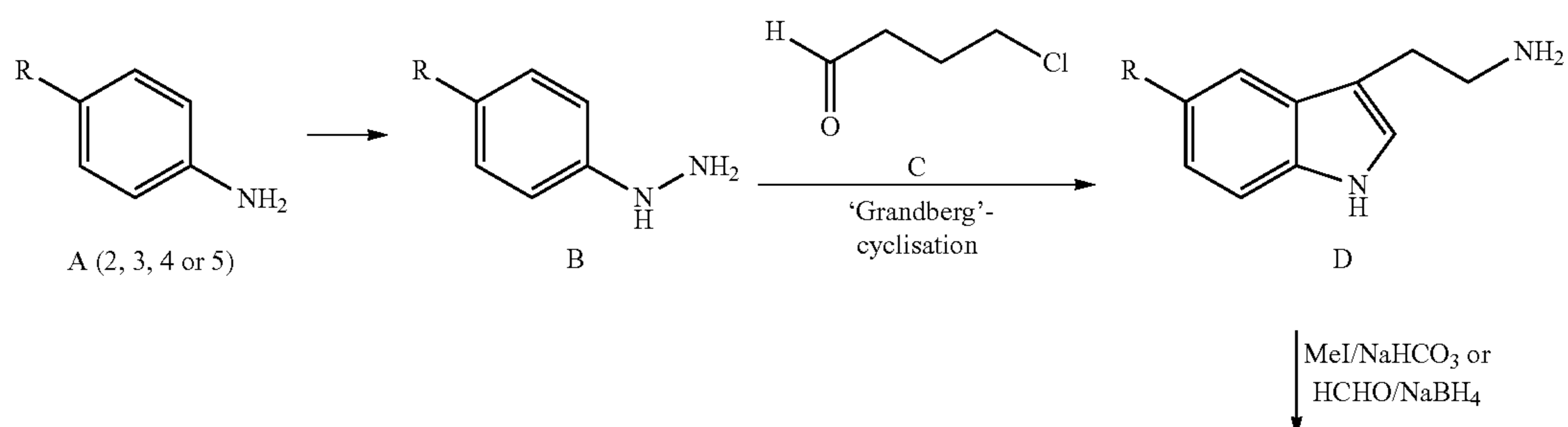
Scheme 2. Synthesis of tryptanes from their aniline precursors
