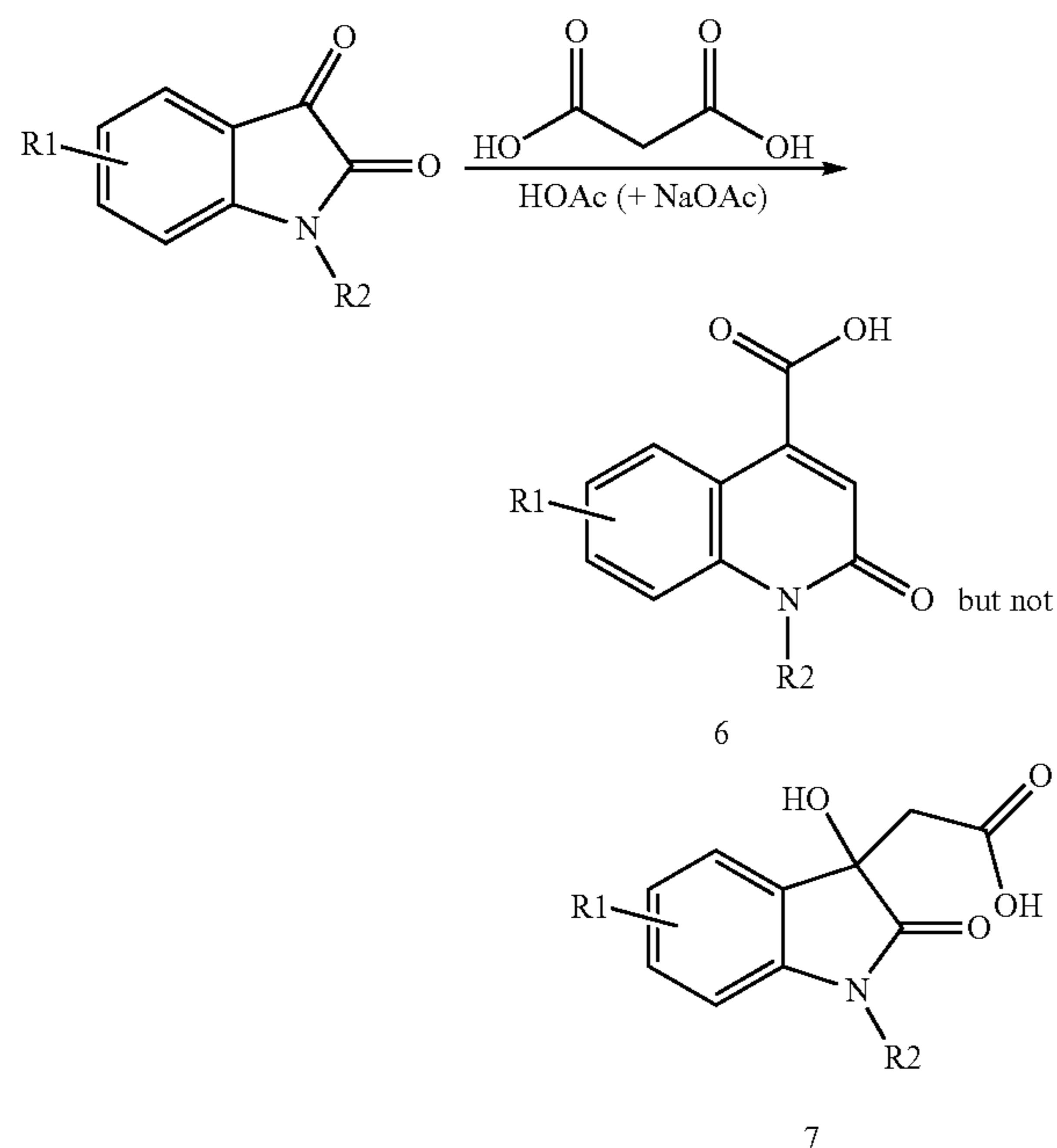
Scheme 5: Condensation of isatin with malonic acid in acetic acid
