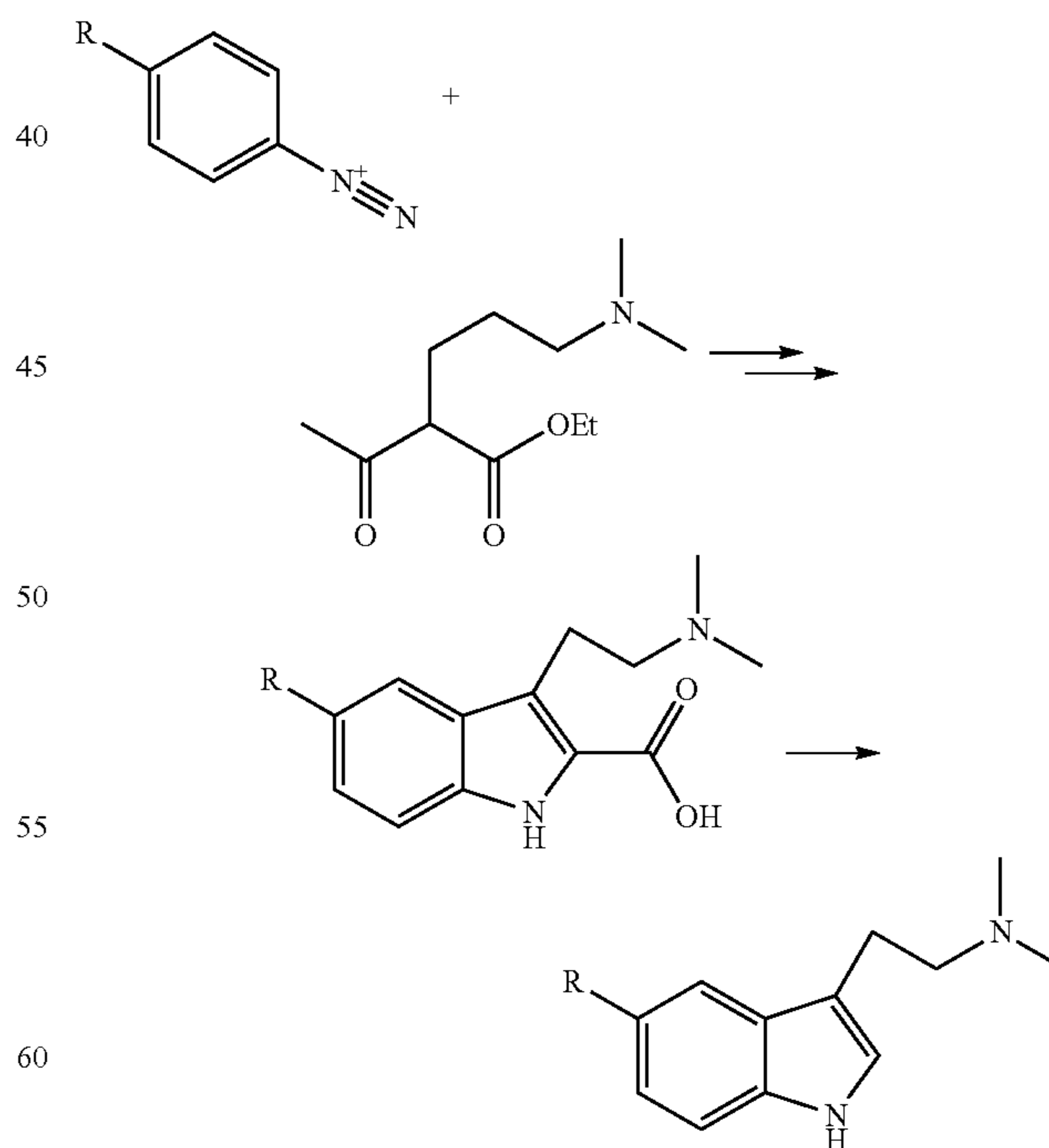
Scheme 4: Alternative to the preparation of a phenyl hydrazine (synthesis of the N,N-dimethylpropyl-malonic acid ethyl ester is inconvenient)
