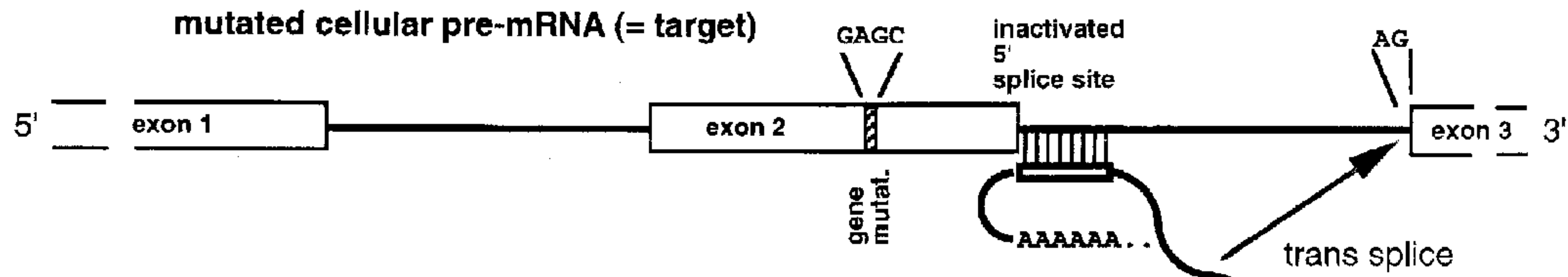
repair pre-mRNA (with the first exons) and with a potent 5' splice site
