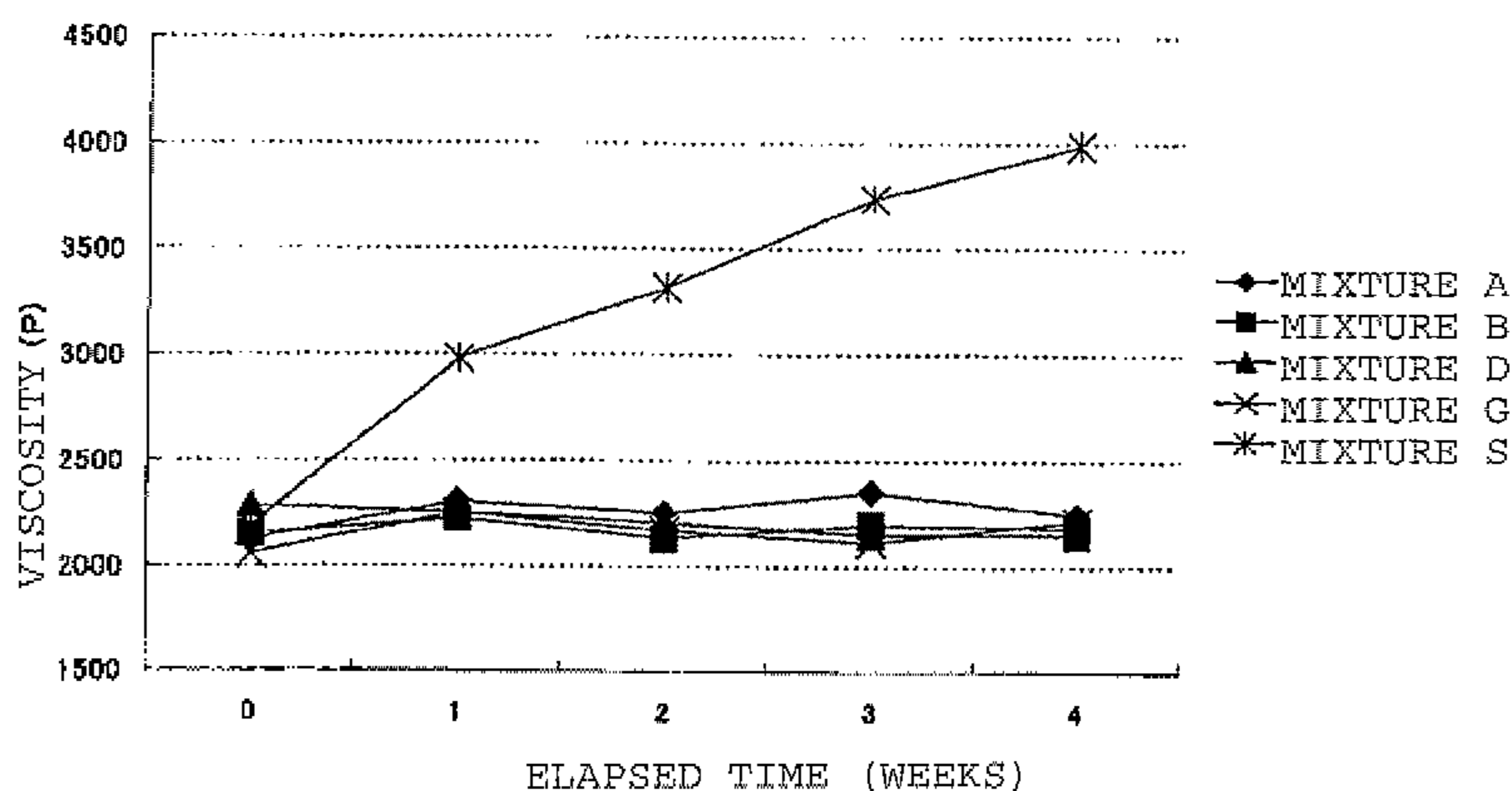
FIGURE 1 CHANGES IN E-TYPE VISCOSITY OVER TIME
