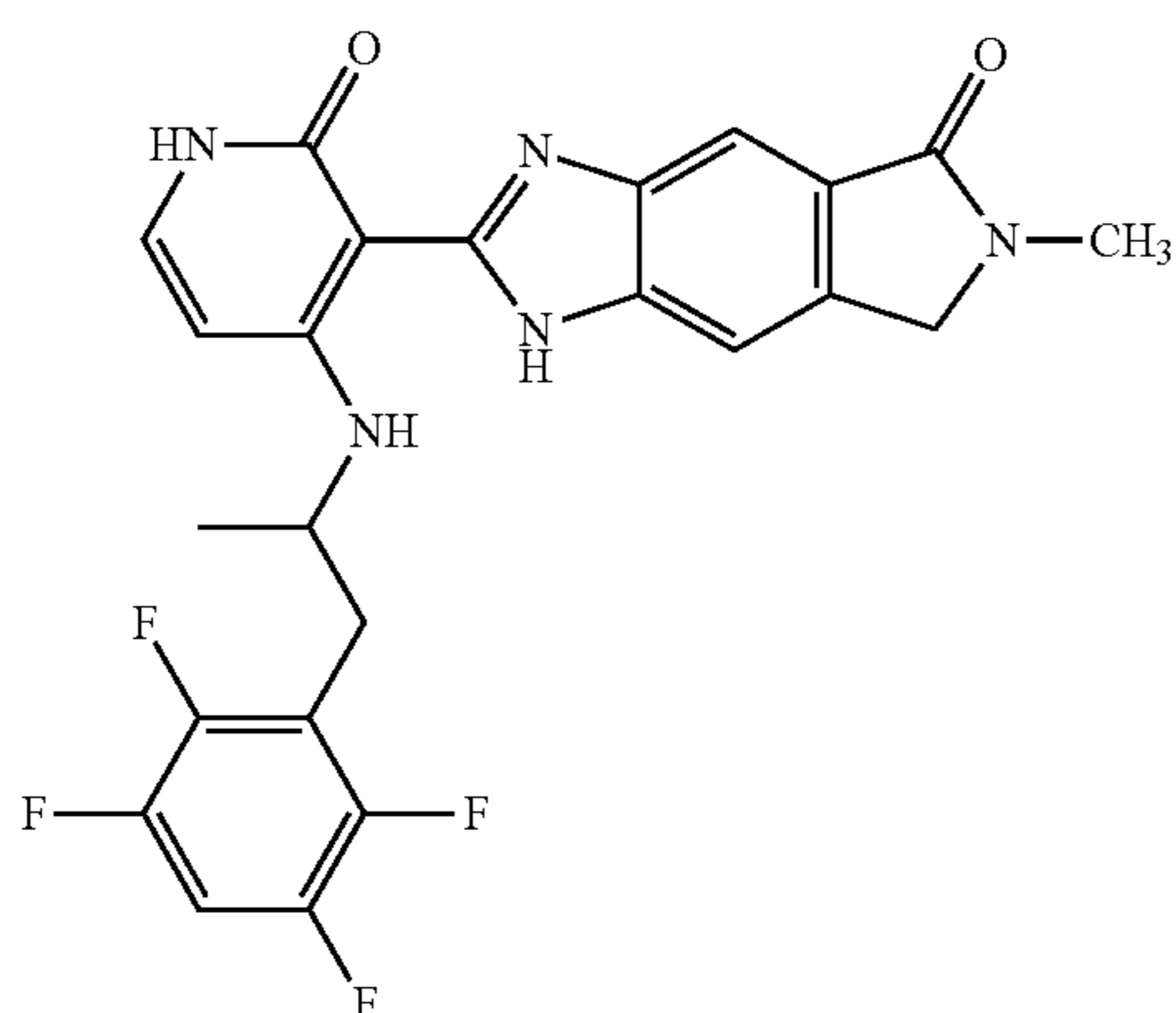
Compound 42
