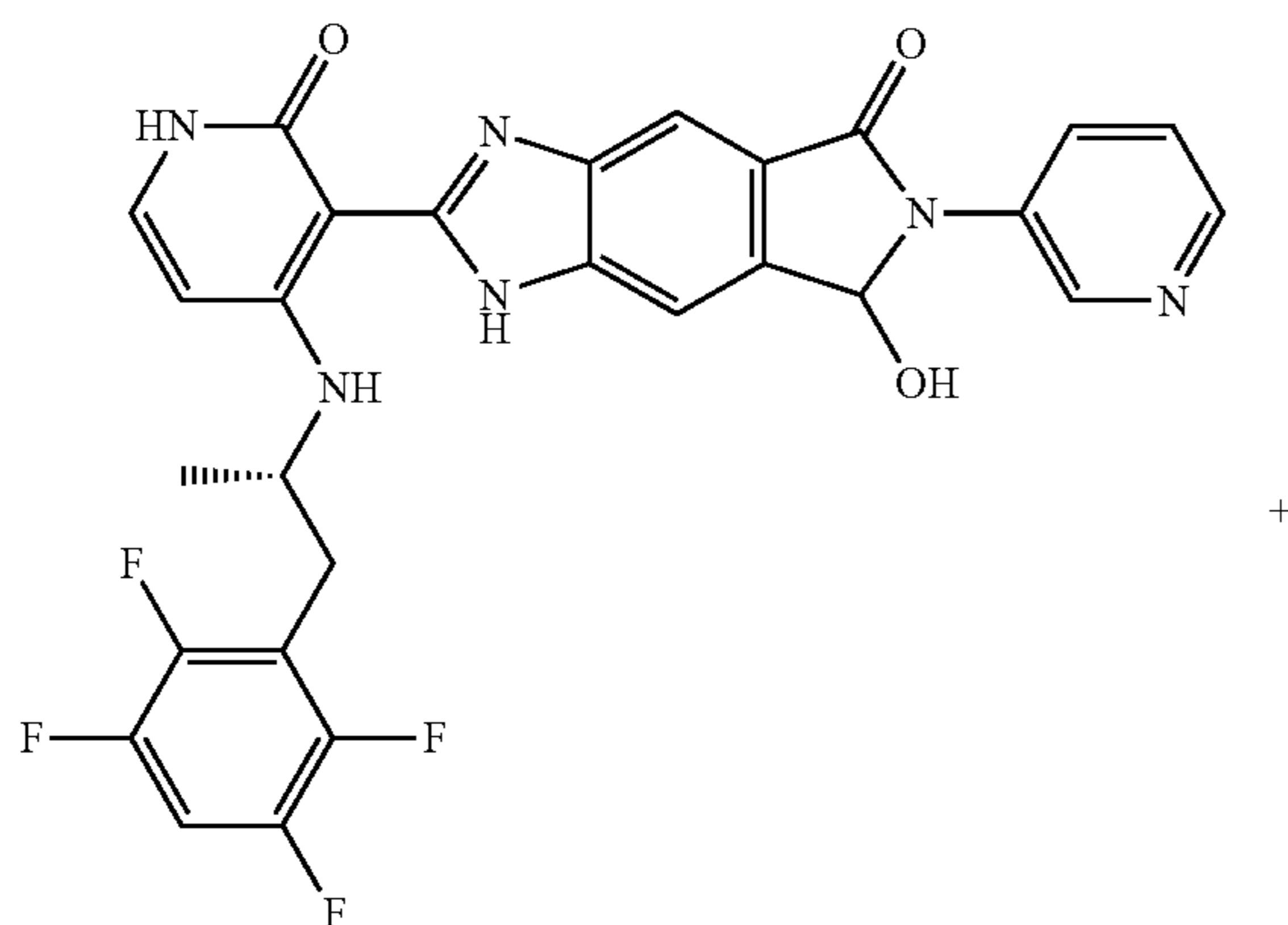
Compound 13
