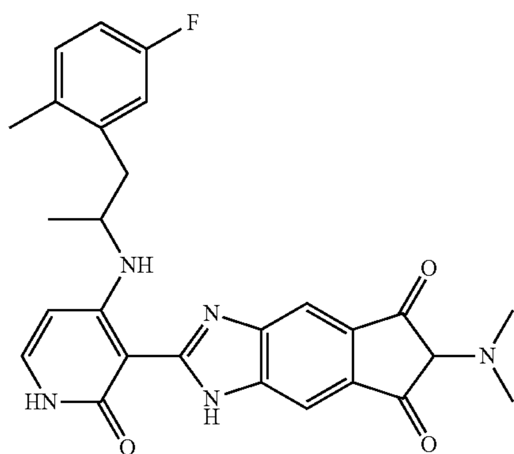
Compound 38
