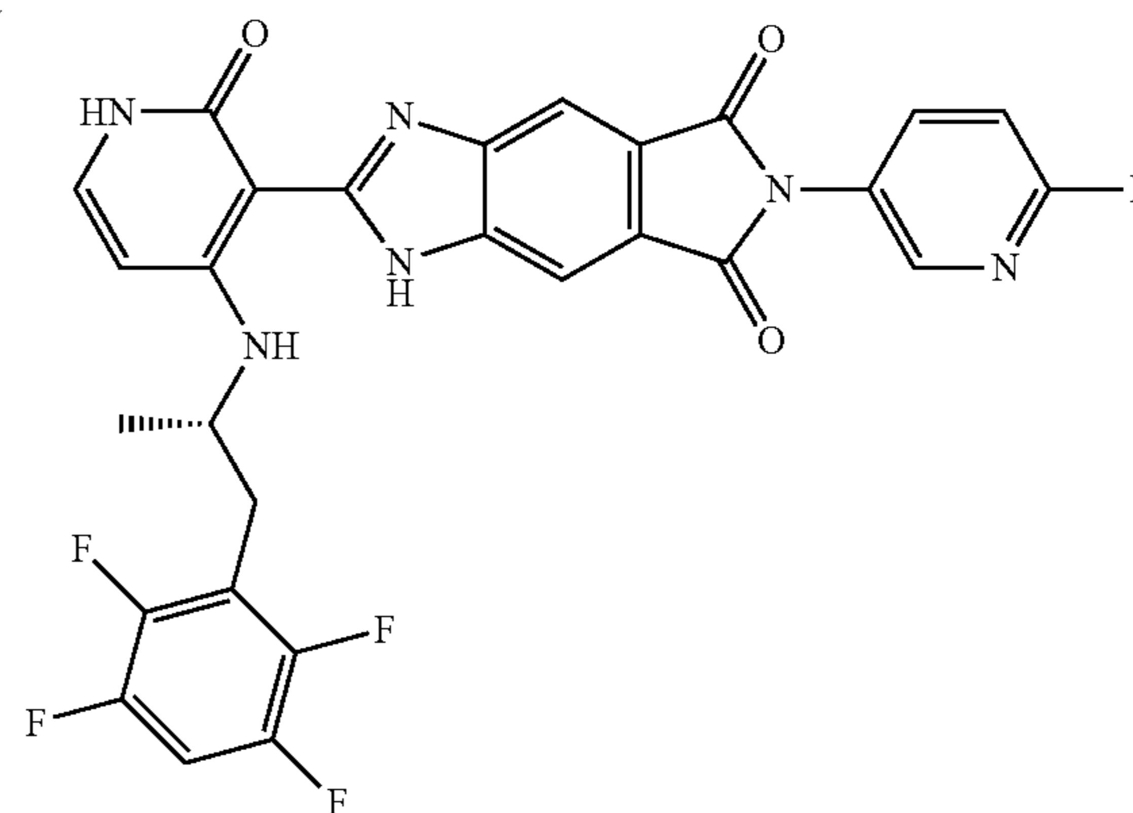
Compound 15
