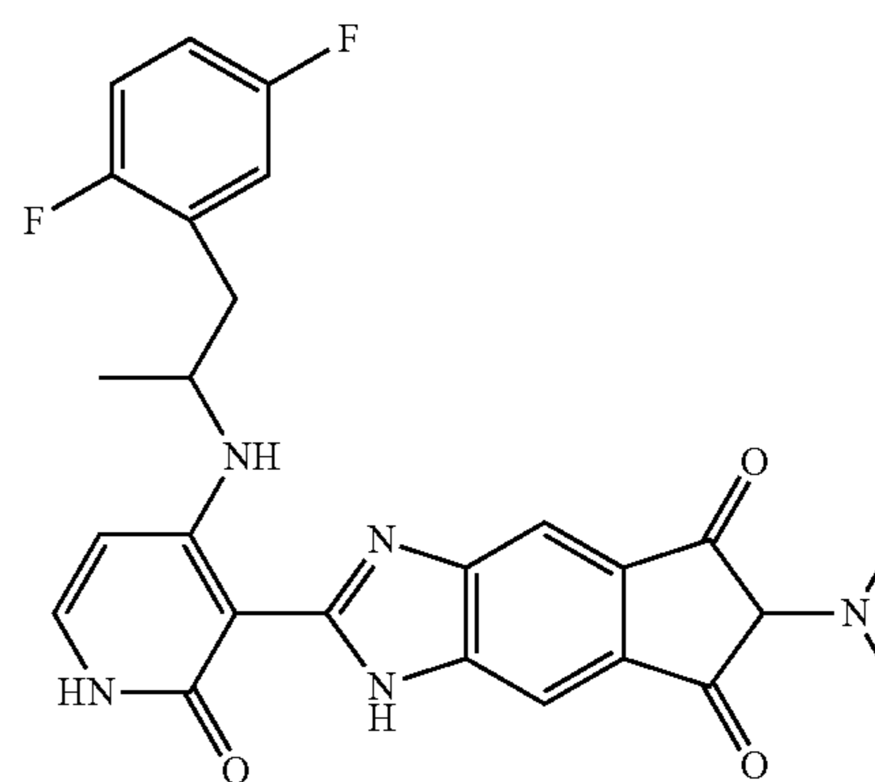
Compound 36
