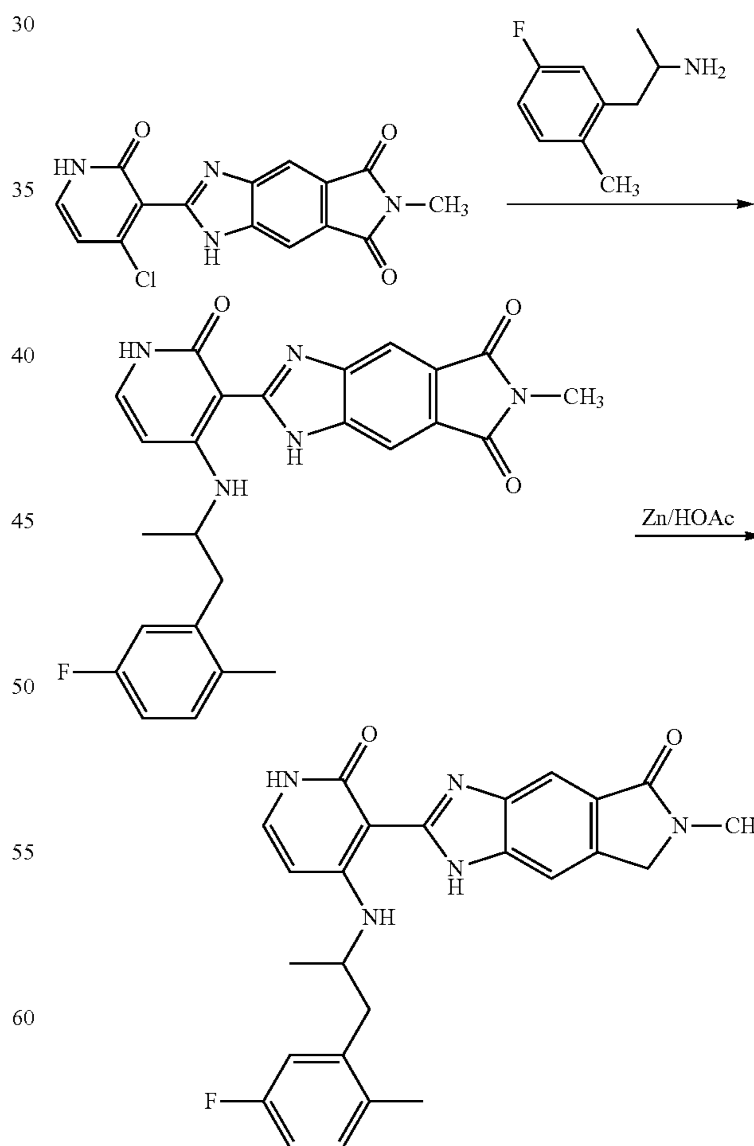
Compound 44
