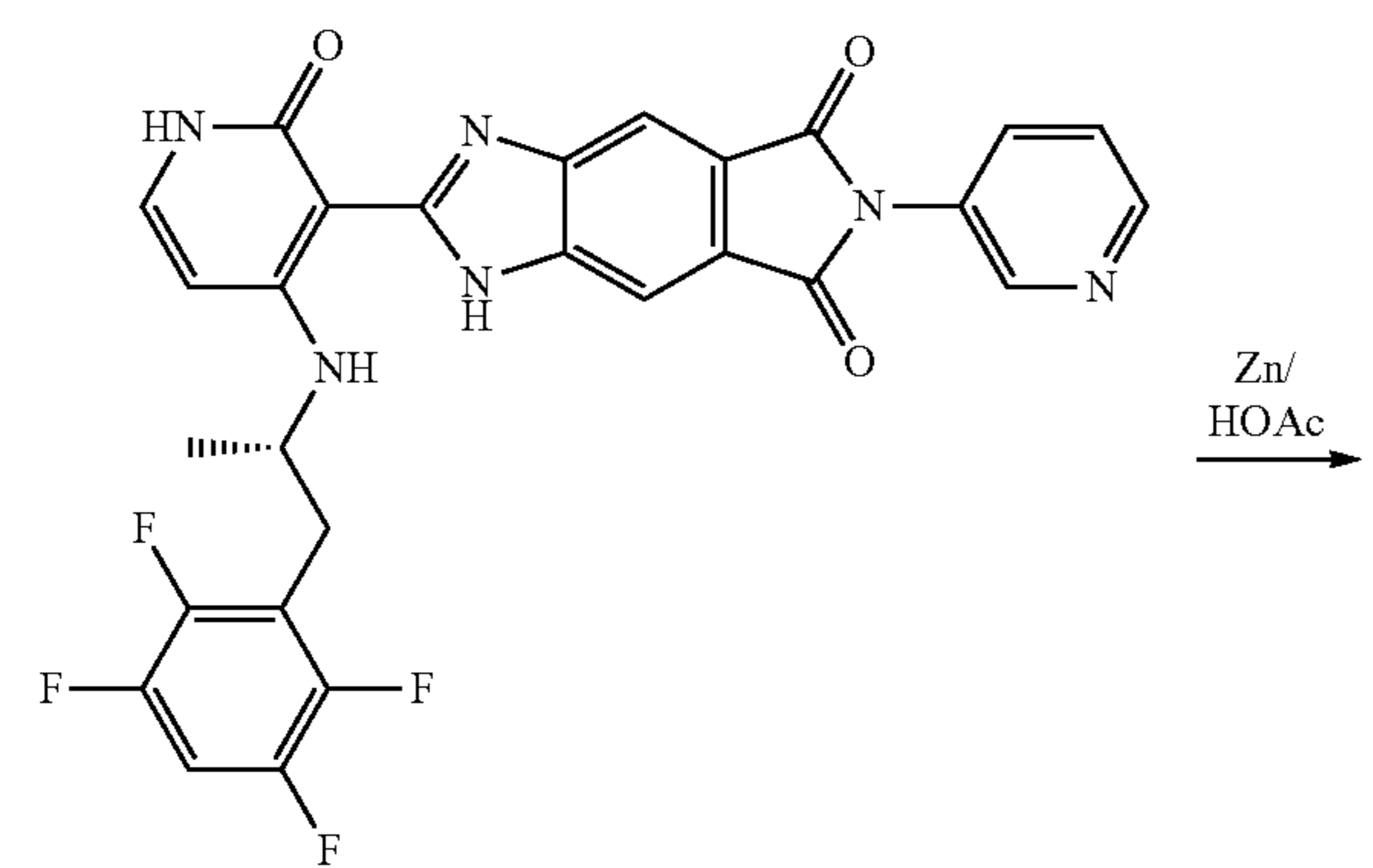
Compound 12
