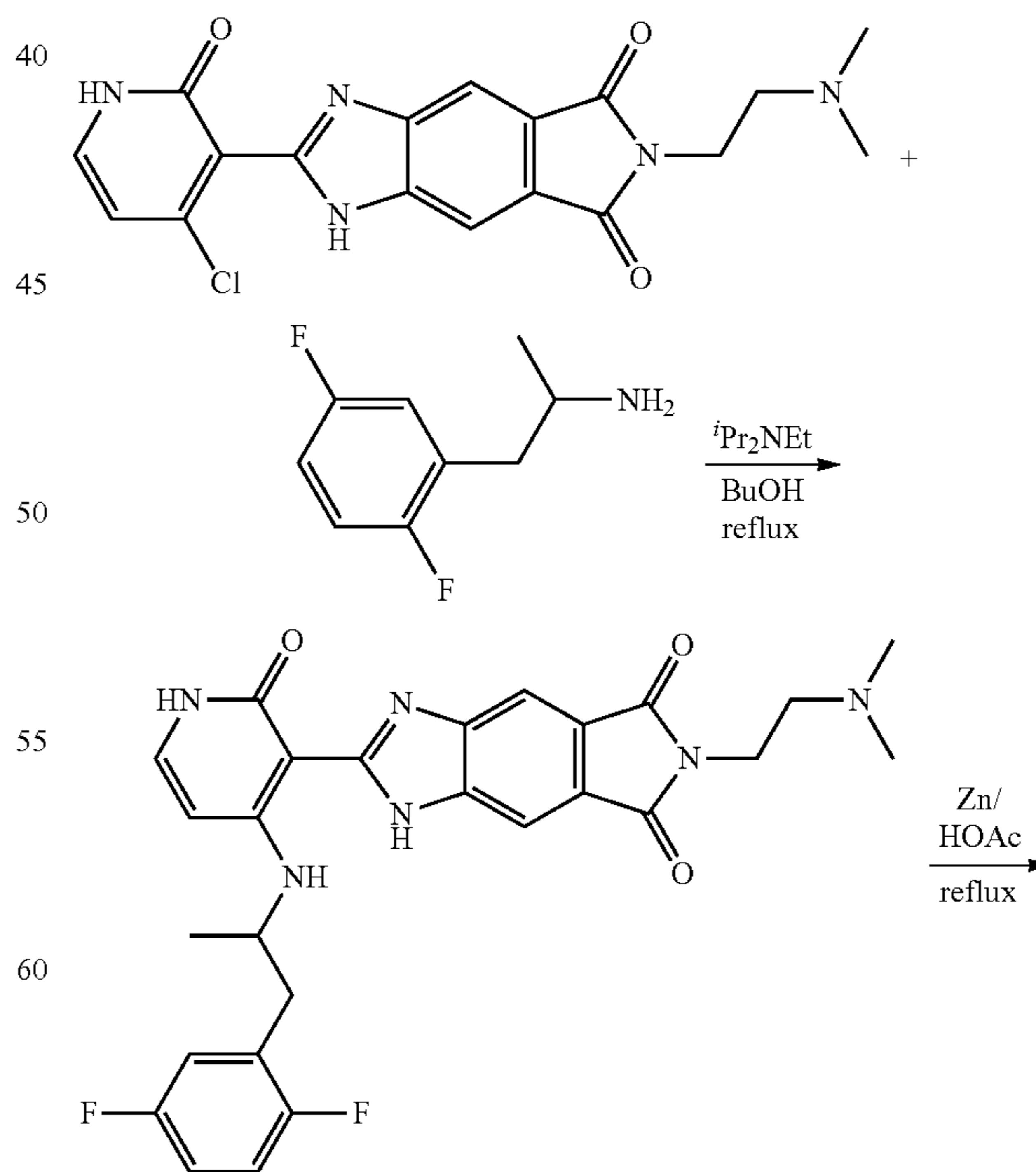
Compound 17
