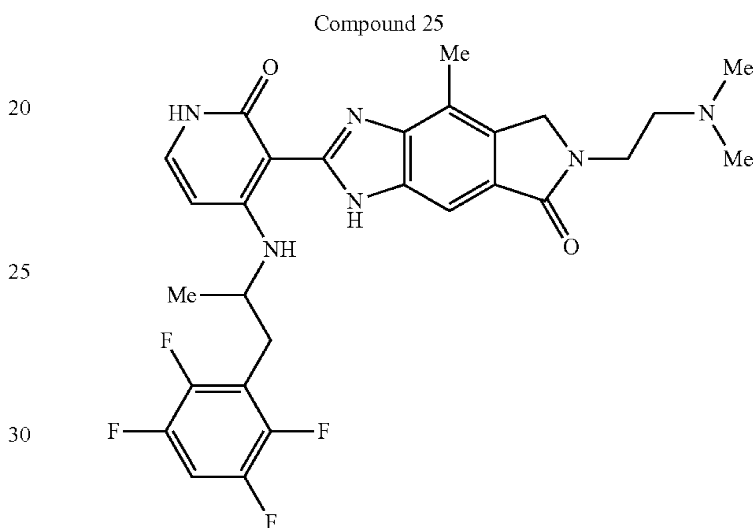
Compound 25A
