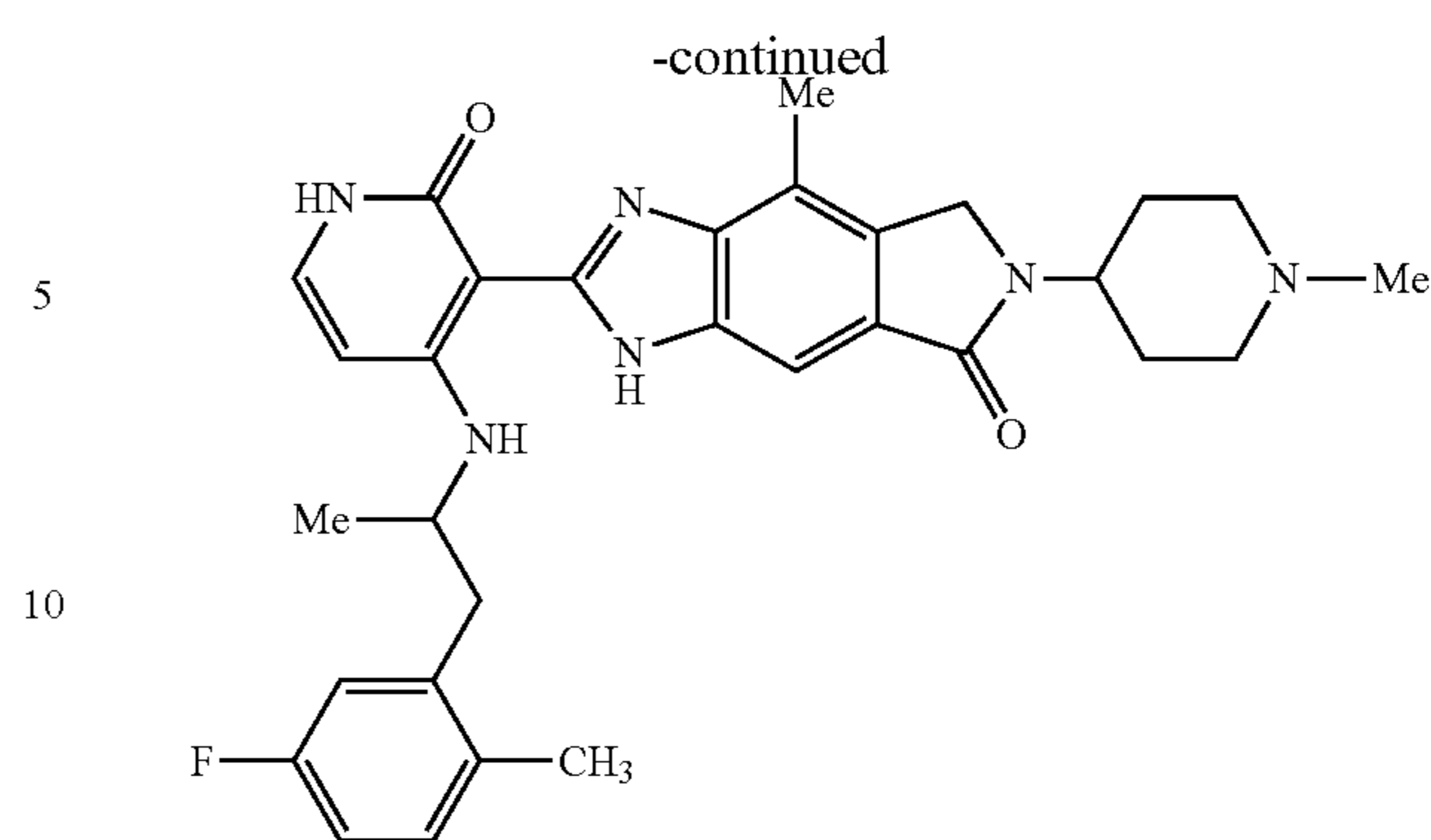
Compound 47B
