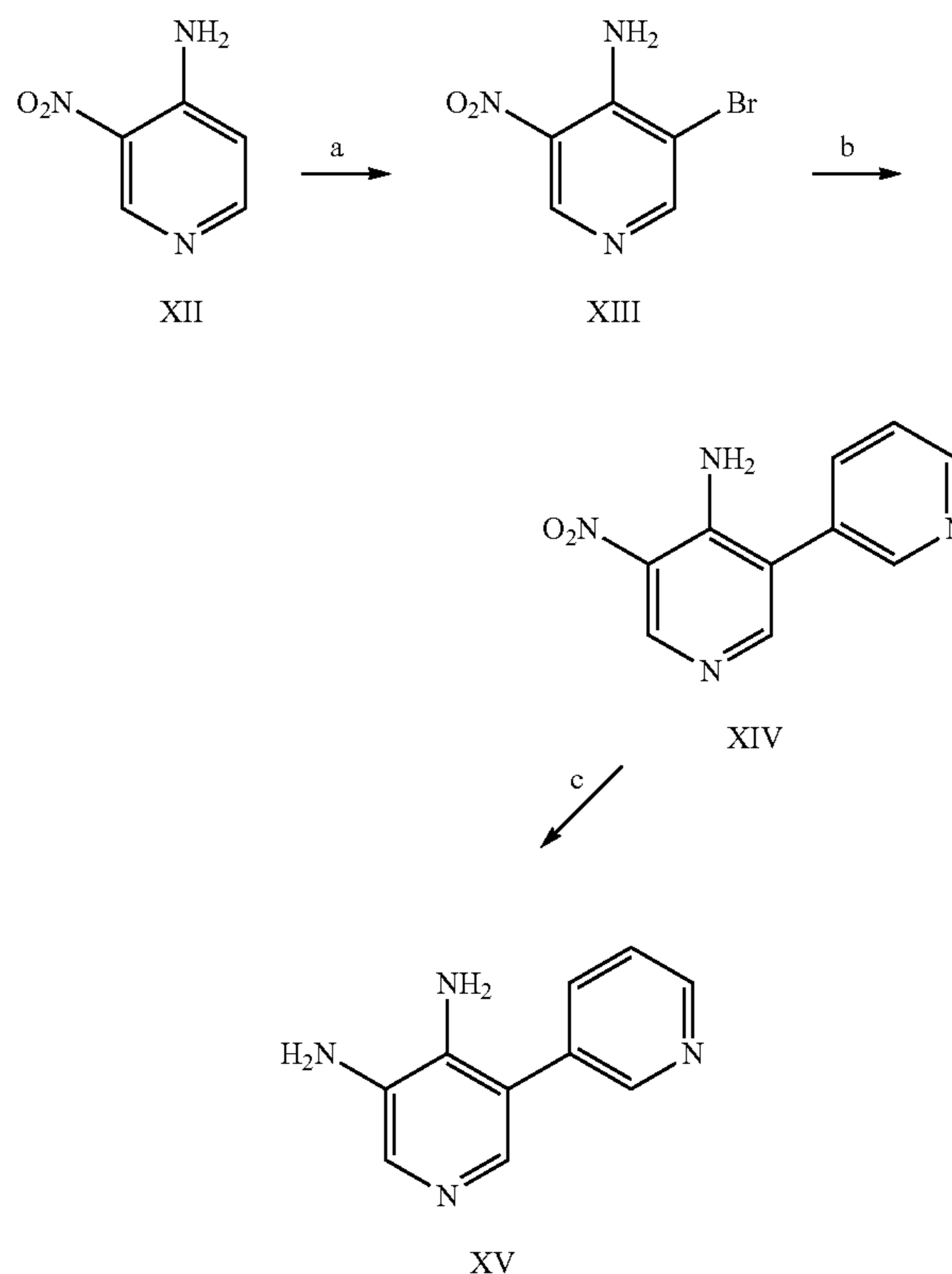
Scheme 3
