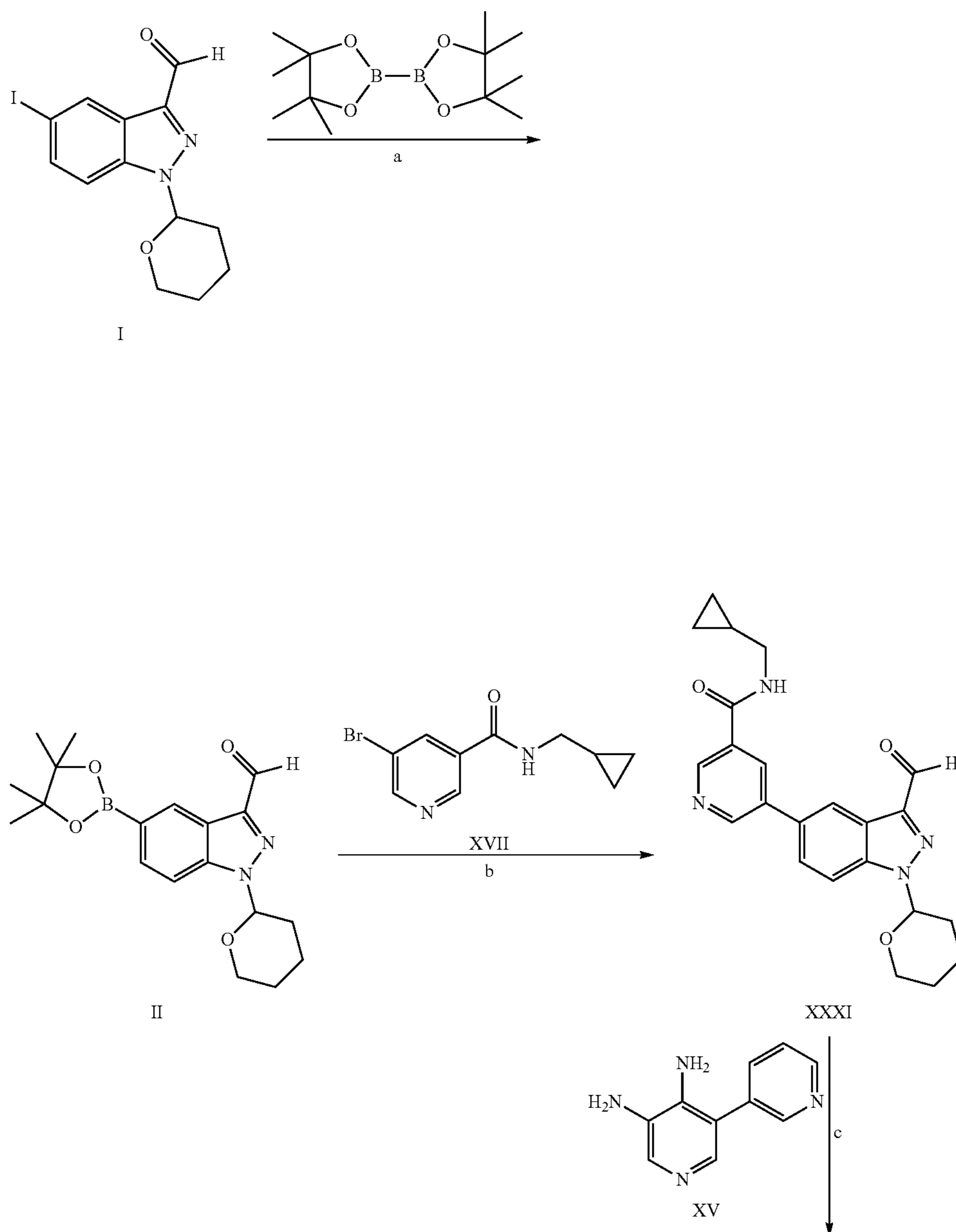
Scheme 6
