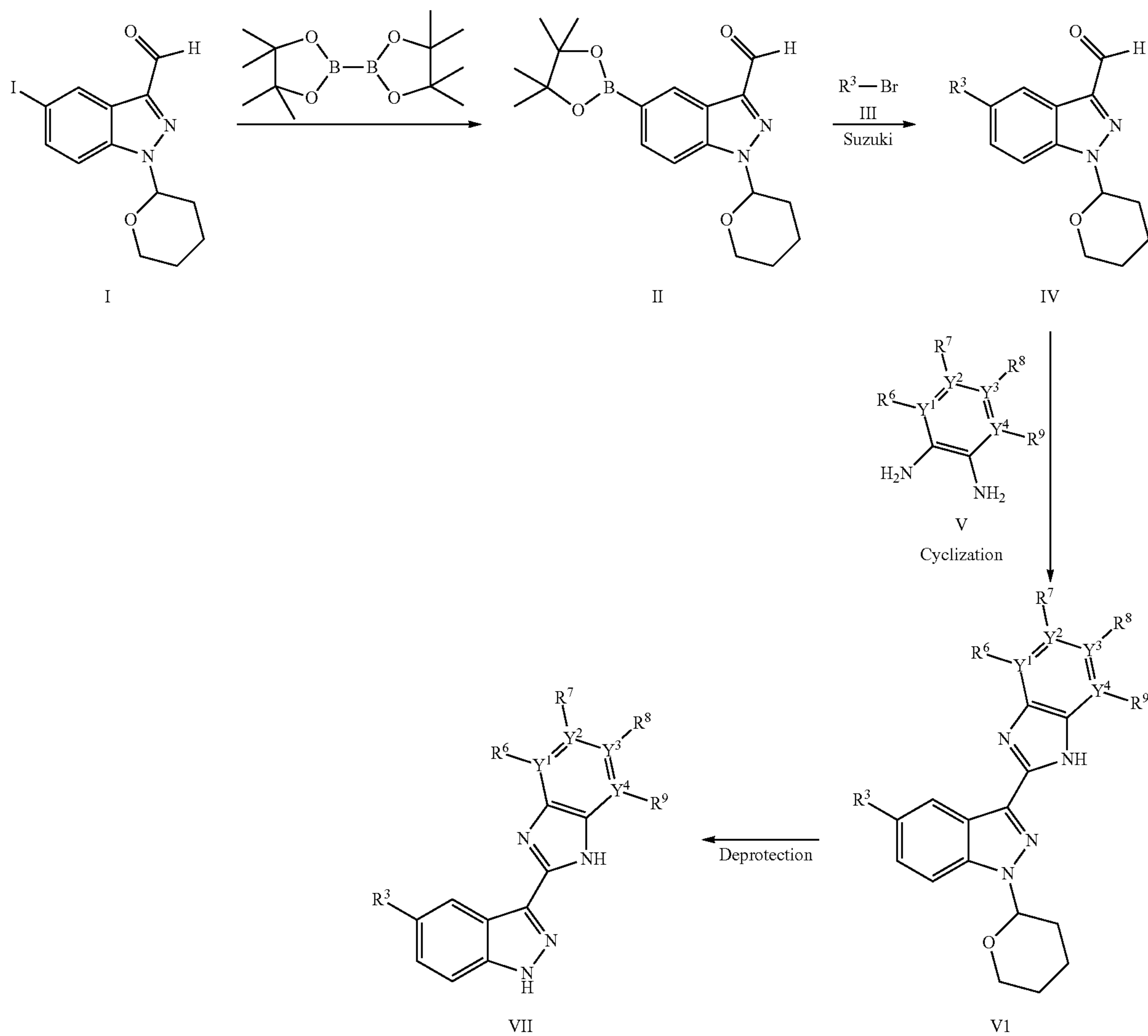
Scheme 1
