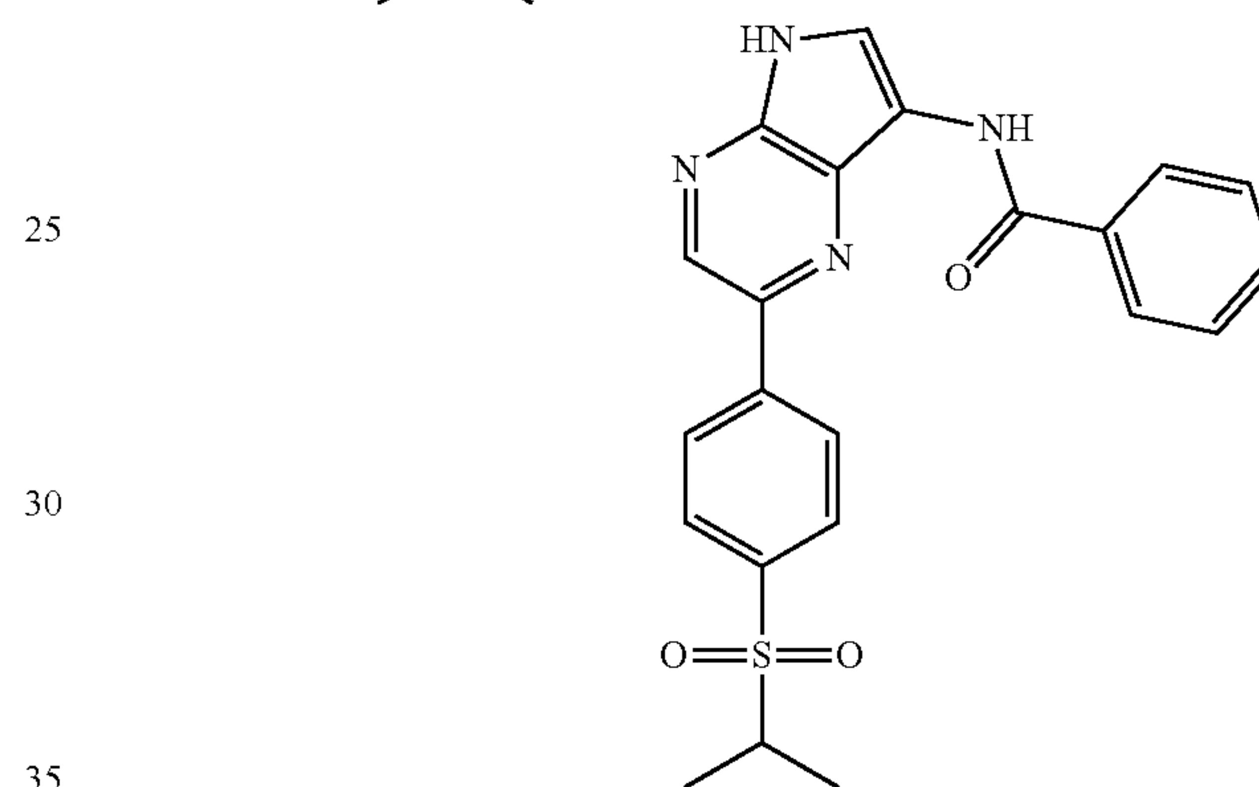
Compound I-1
