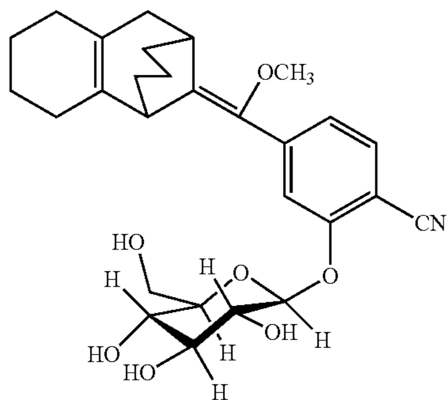
Synthesis of [(4-methoxy-4(3-β-D-glucoside-4-cyanophenyl)]spiro[1,2-dioxetane-3-1,3-tricyclo[7.3.1.0 2,7 ]tridec-2,7-ene
