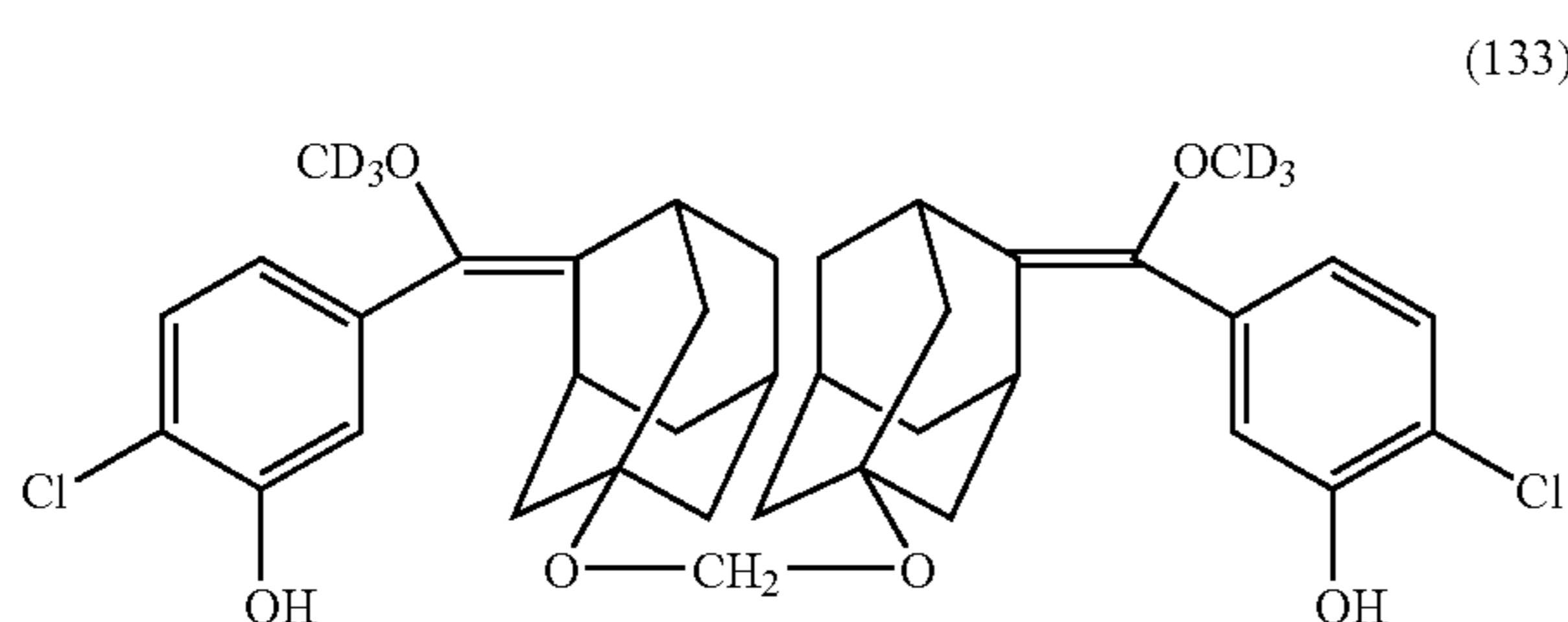
(c). Synthesis of bis-[(3-phosphoryloxy-4-chlorophenyl)methoxy(D3)methylene-5-oxy-adamantane, disodium salt]methane
