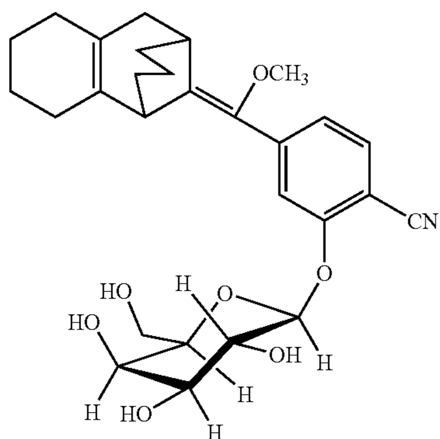
Synthesis of [(4-Methoxy-4(3-β-D-galactose-4-cyanophenyl)]spiro[1,2-dioxetane-3-1,3-tricyclo[7.3.1.0 2,7 ]tridec-2,7-ene (55)
