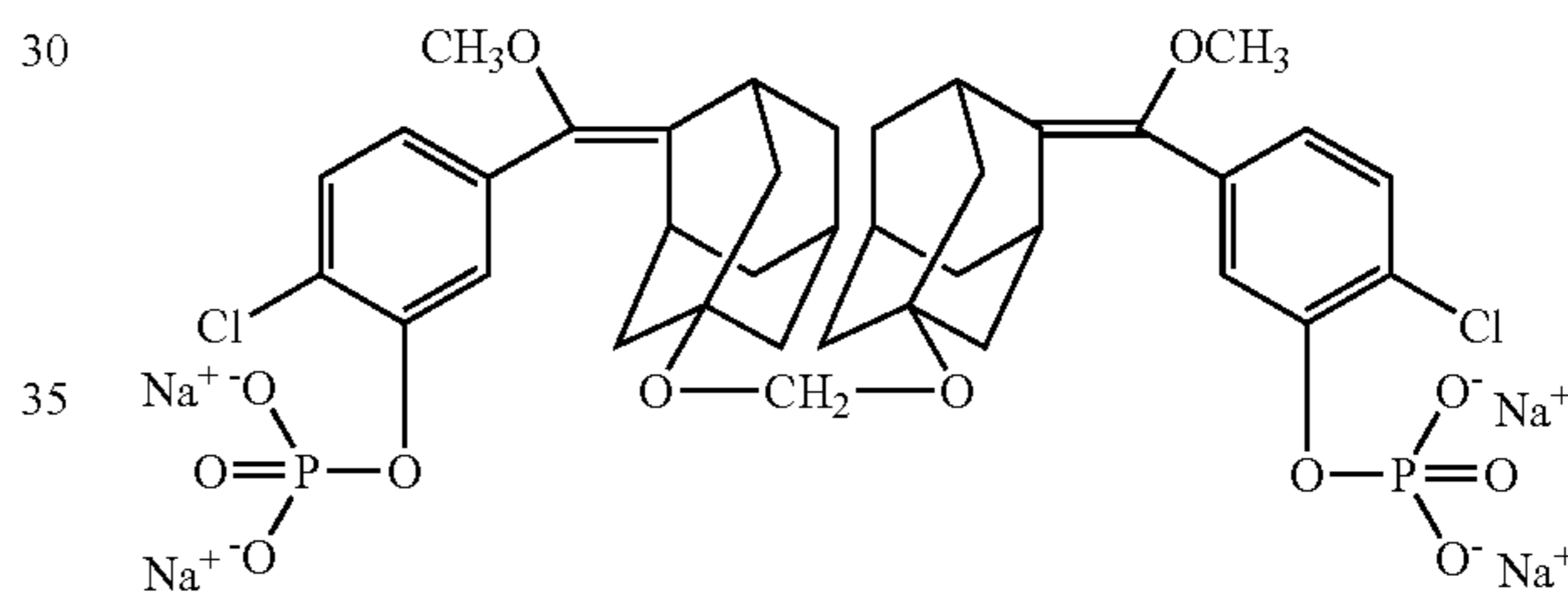
(c). Synthesis of bis-[(3-phosphoryloxy-4-chlorophenyl)methoxy(D3)methylene-5-oxy-adamantane, disodium salt]methane
