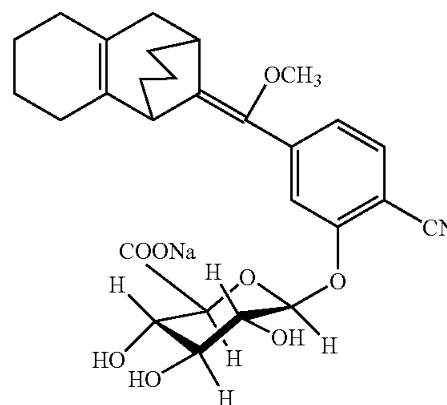
Synthesis of Sodium[(4-methoxy(D 3 )-4-(3-β-D-glucuronic acid-4-chlorophenyl)]spiro[1,2-dioxetane-3,2'-adamantane]
