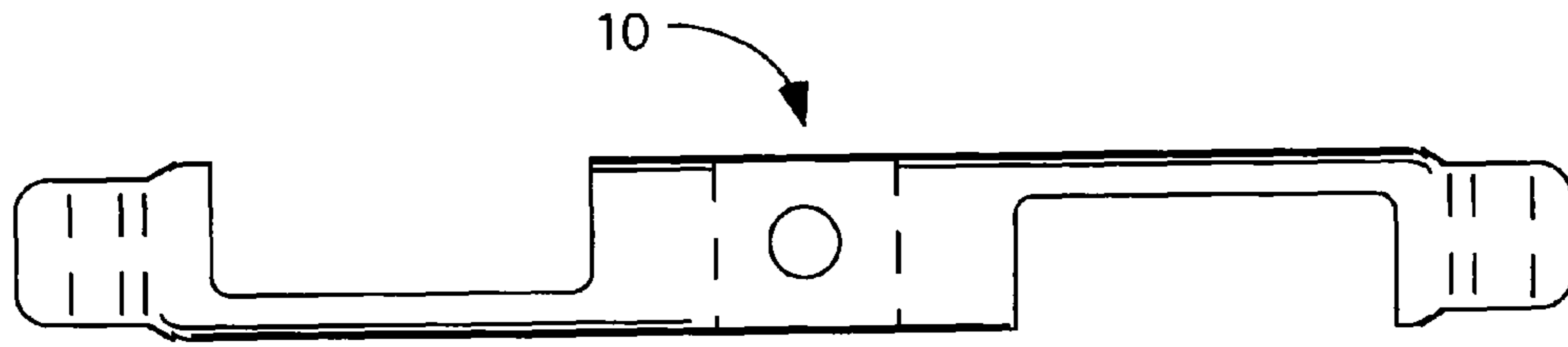
FIG. 1 PRIOR ART
