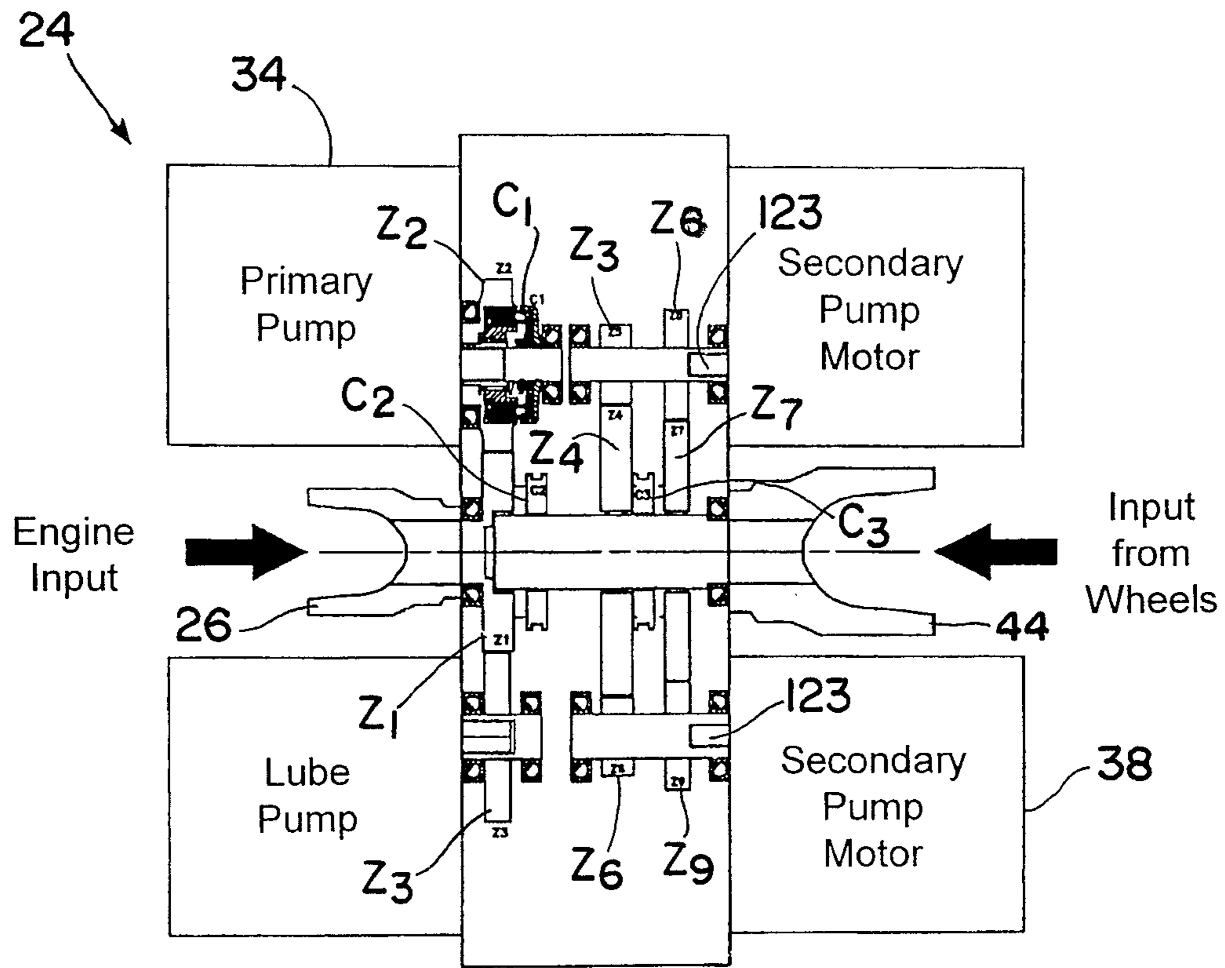
Braking/Charge Accum
