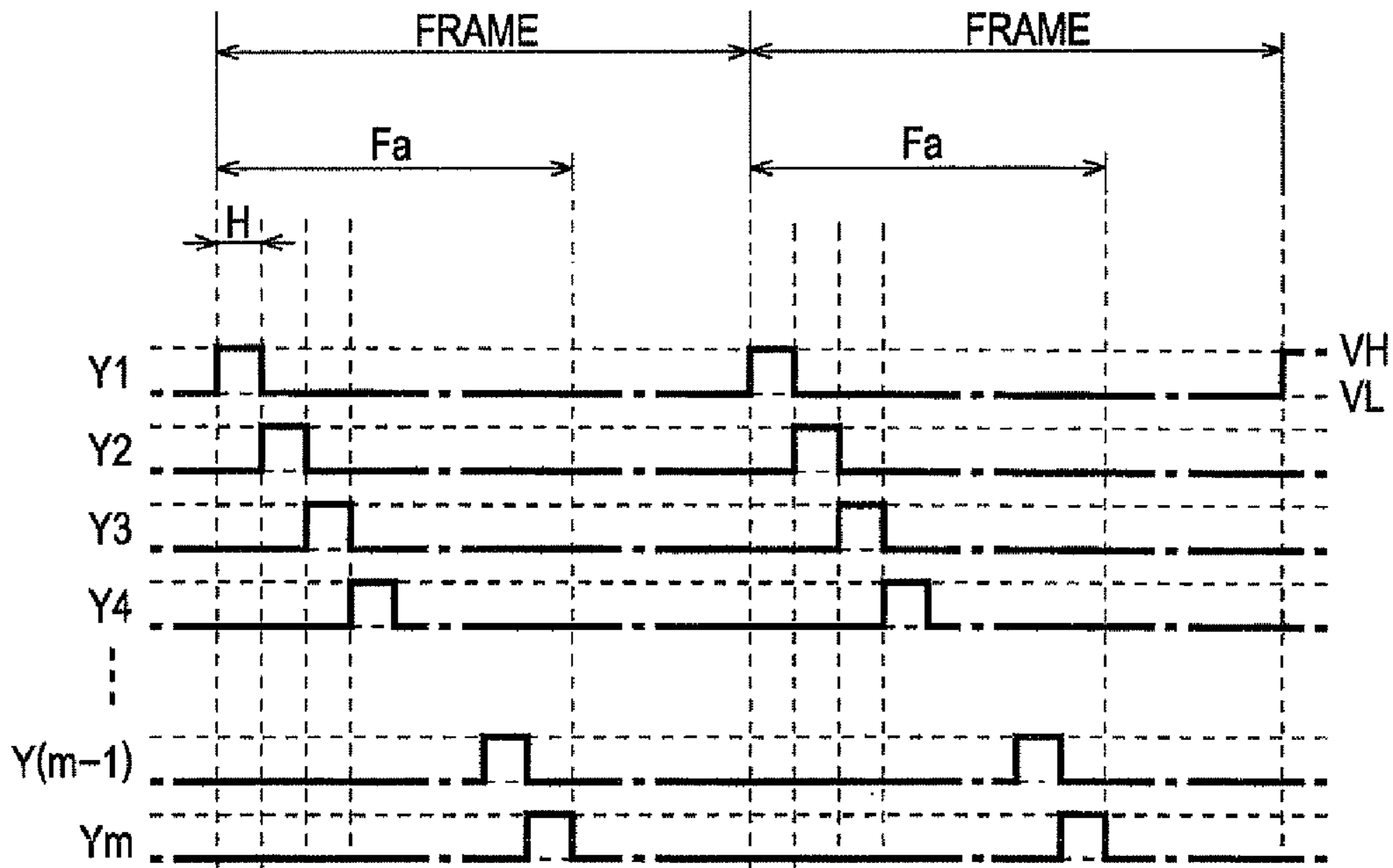
FIG. 5A SCANNING LINE DRIVING CIRCUIT
