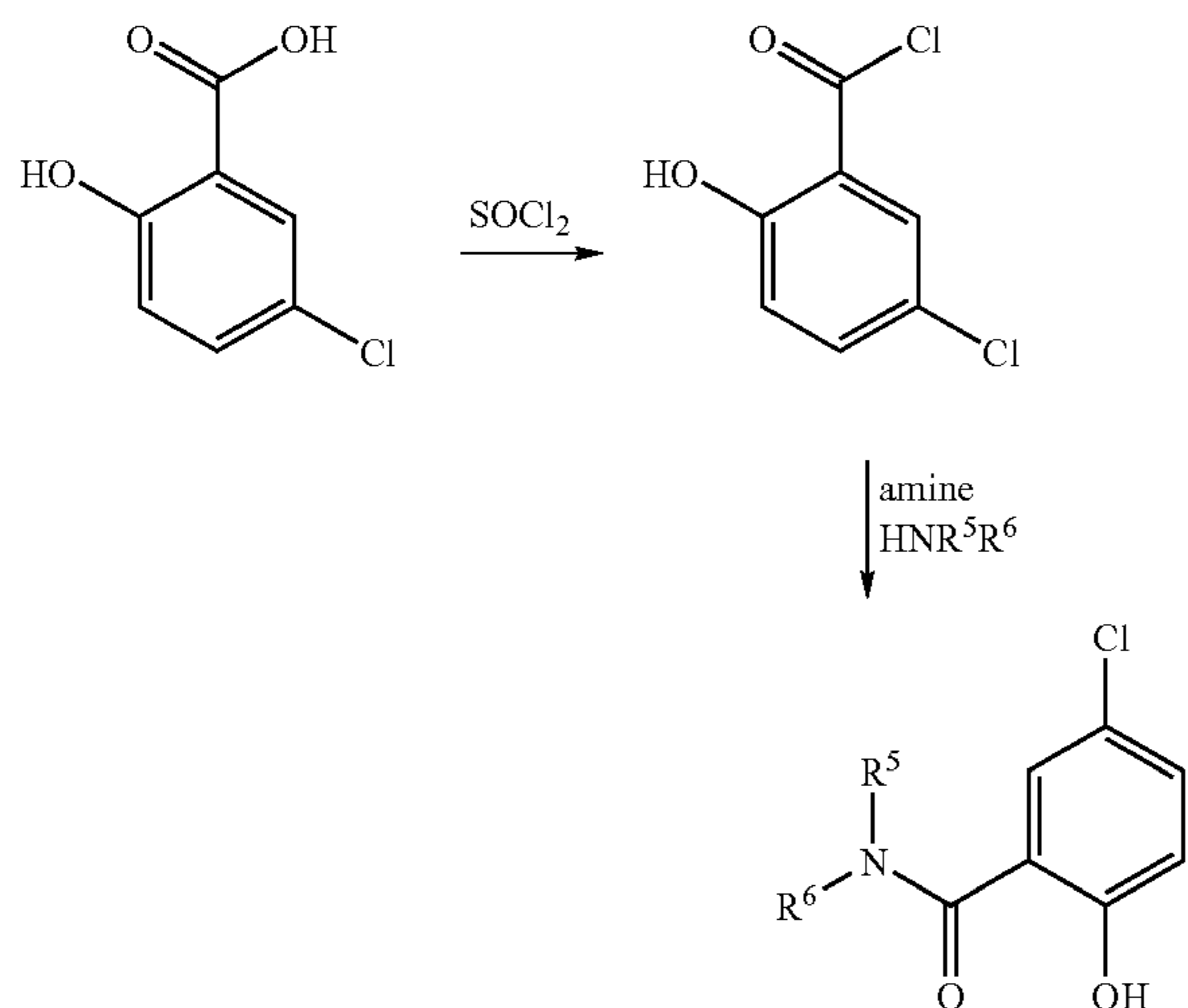
Scheme 1: 5-Chloro-2-hydroxybenzoic acid amides
