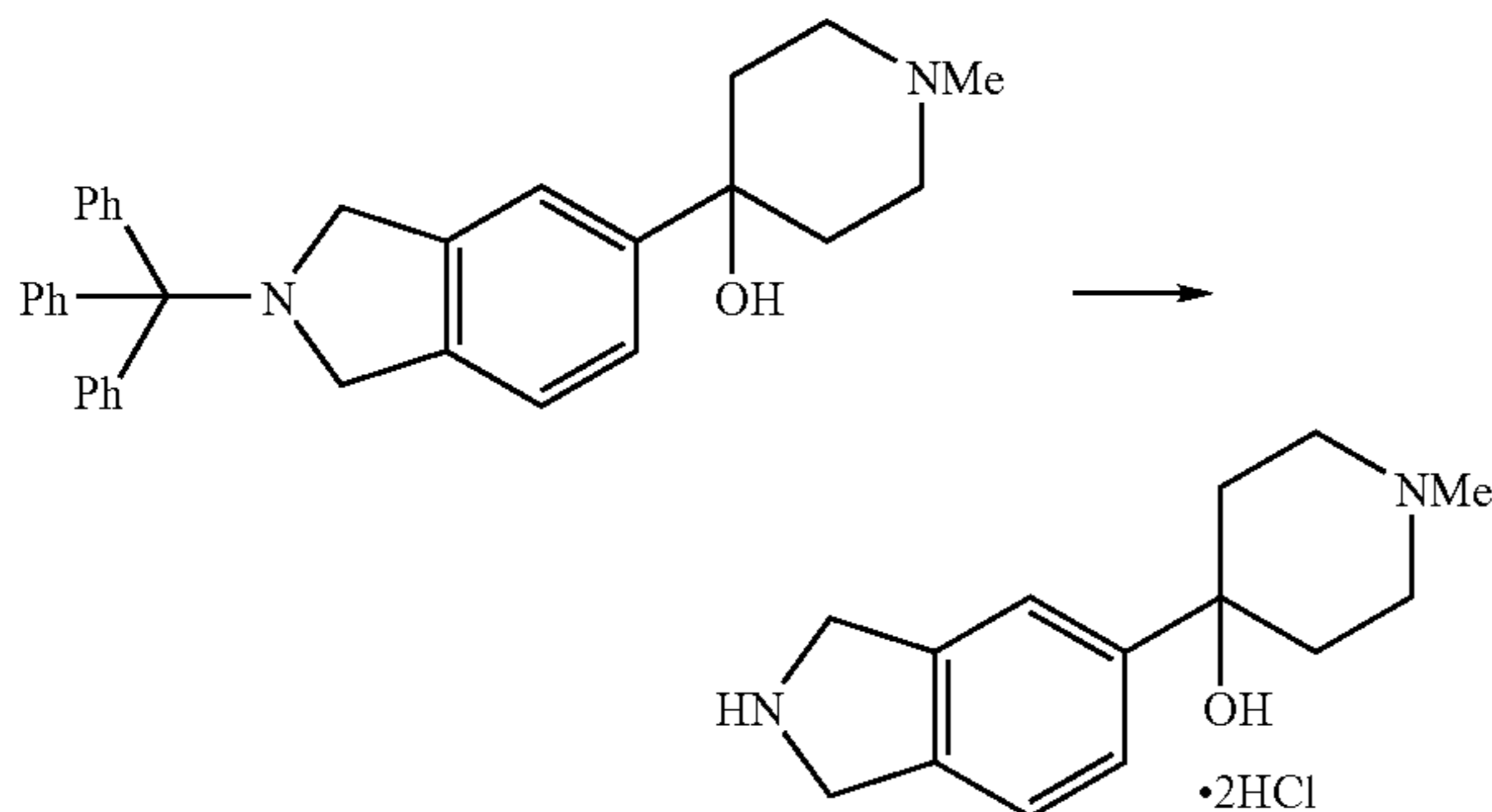
78C. 4-(2,3-Dihydro-1H-isoindol-5-yl)-1-methyl-piperidin-4-ol dihydrochloride
