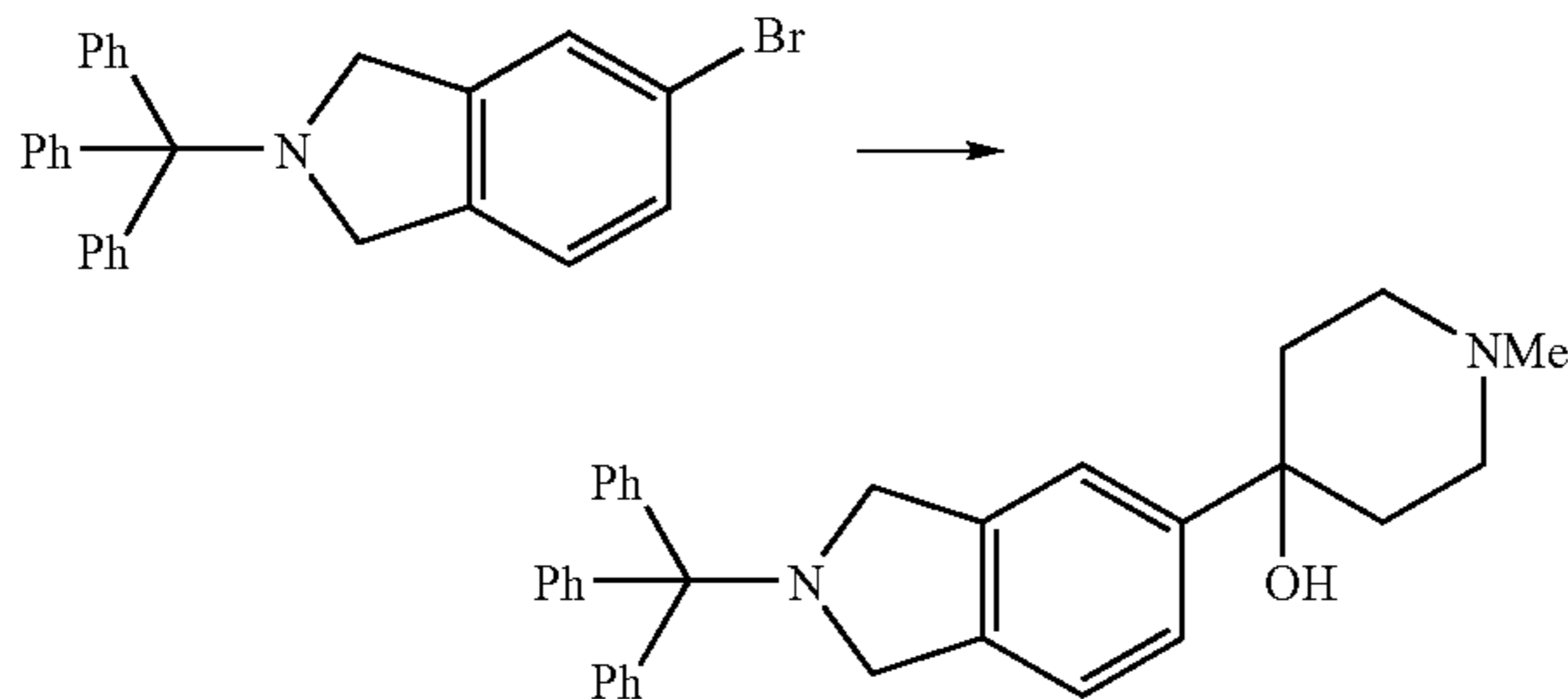
78B. 1-methyl-4-(2-trityl-2,3-dihydro-1H-isoindol-5-yl)-piperidin-4-ol
