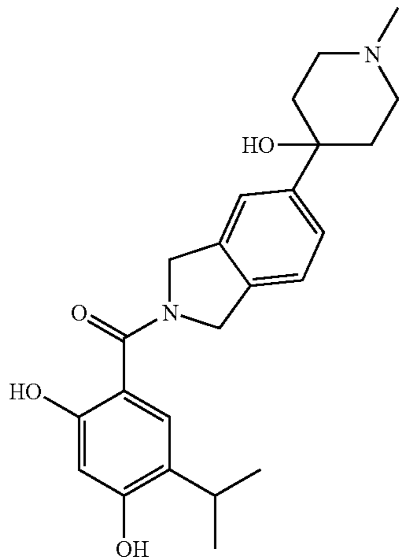
50A: Synthesis of 5-bromo-1,3-dihydro-isoindole-2-carboxylic acid tert-butyl ester
