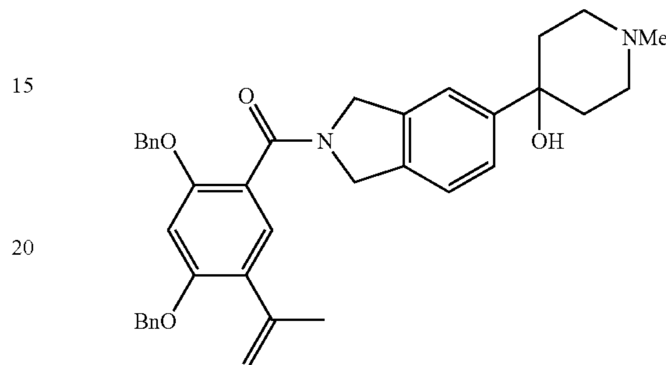
78D. (2,4-Bis-benzyloxy-5-isopropenyl-phenyl)-[5-(4-hydroxy-1-methyl-piperidin-4-yl)-1,3-dihydro-isoindol-2-yl]-methanone
