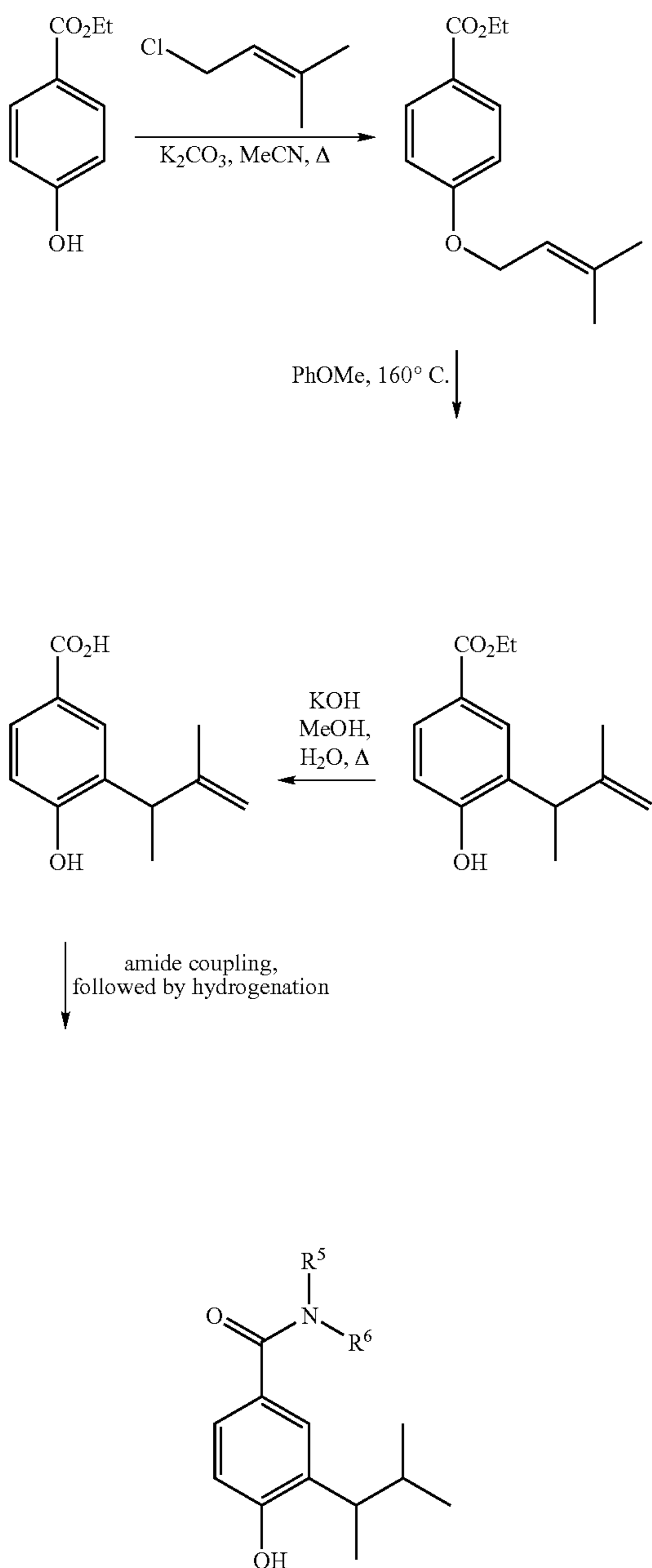
Scheme 5: 4-Hydroxy-3-(1', 2'-dimethyl-propyl)-benzoic acid amides
