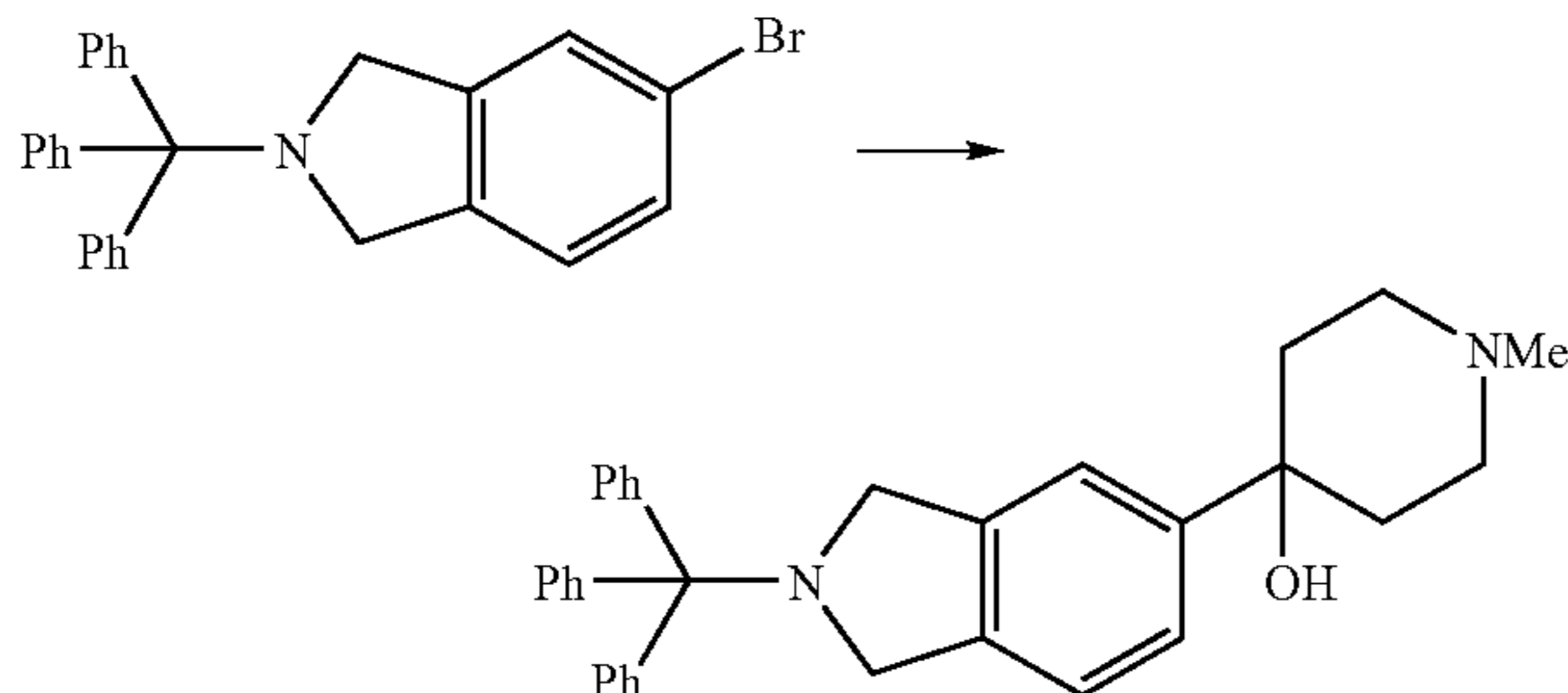
78B. 1-methyl-4-(2-trityl-2,3-dihydro-1H-isoindol-5-yl)-piperidin-4-ol
