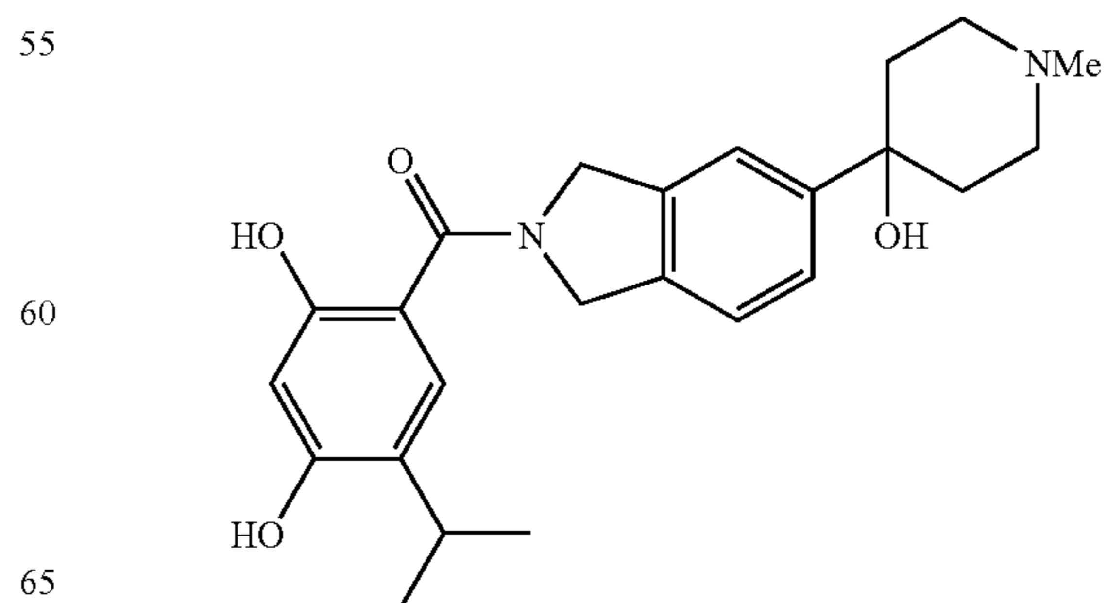
78E. (2,4-Dihydroxy-5-isopropyl-phenyl)-[5-(4-hydroxy-methyl-piperidin-4-yl)-1,3-dihydro-isoindol-2-yl]-methanone
