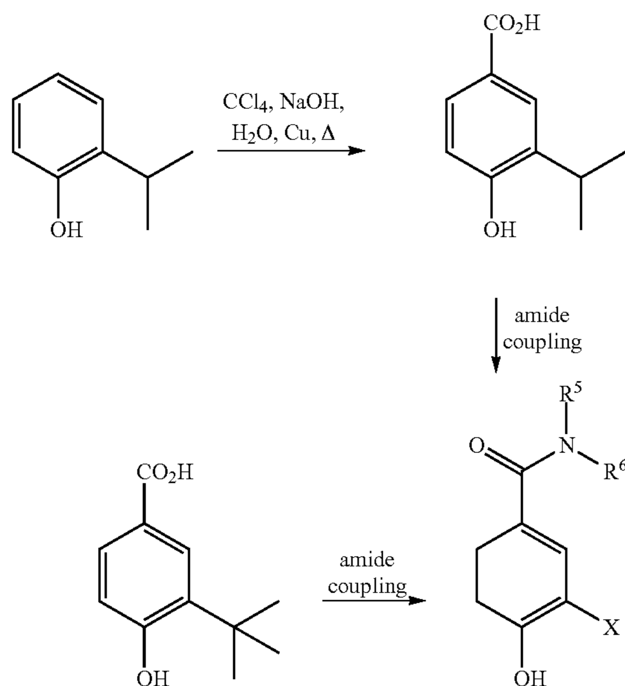
Scheme 3: 3-Alkyl-4-hydroxybenzoic acid amides
