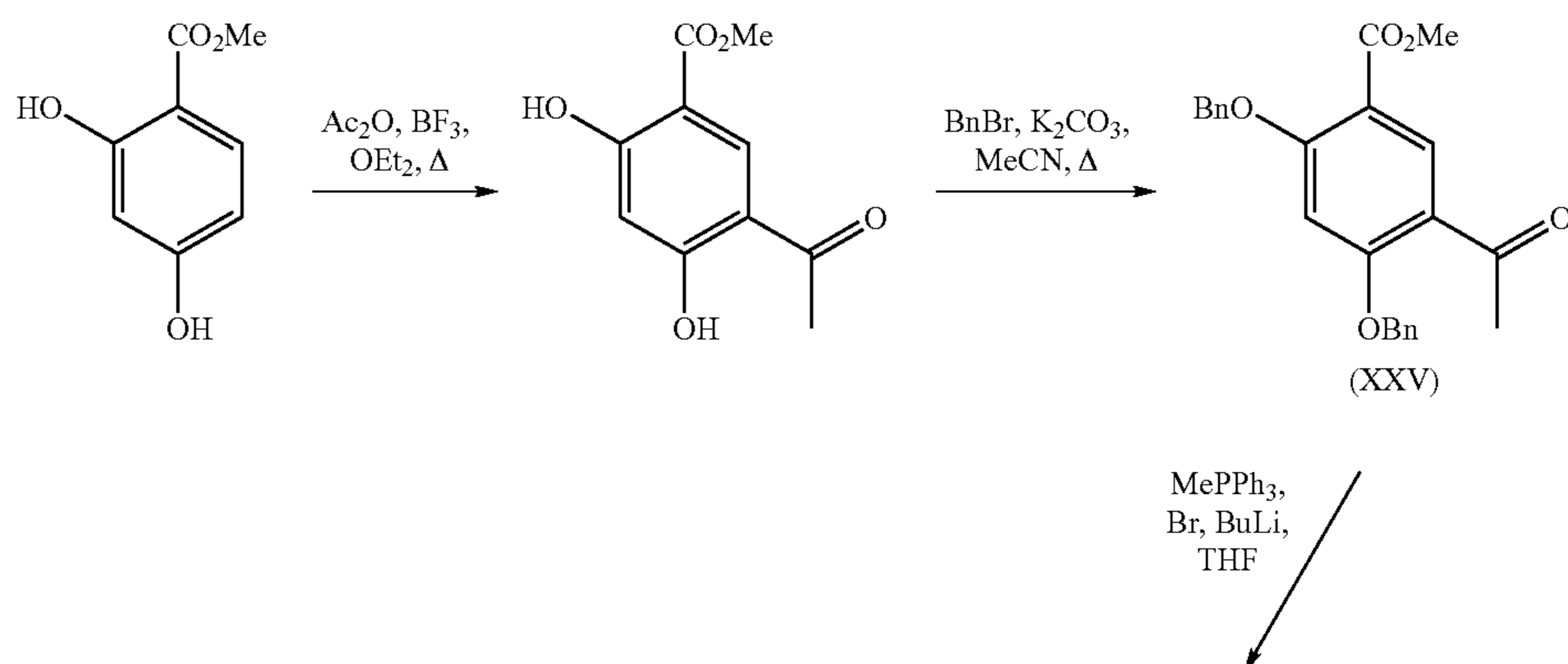
Scheme 4: 2,4-Dihydroxy-5-isopropyl-benzoic acid amides
