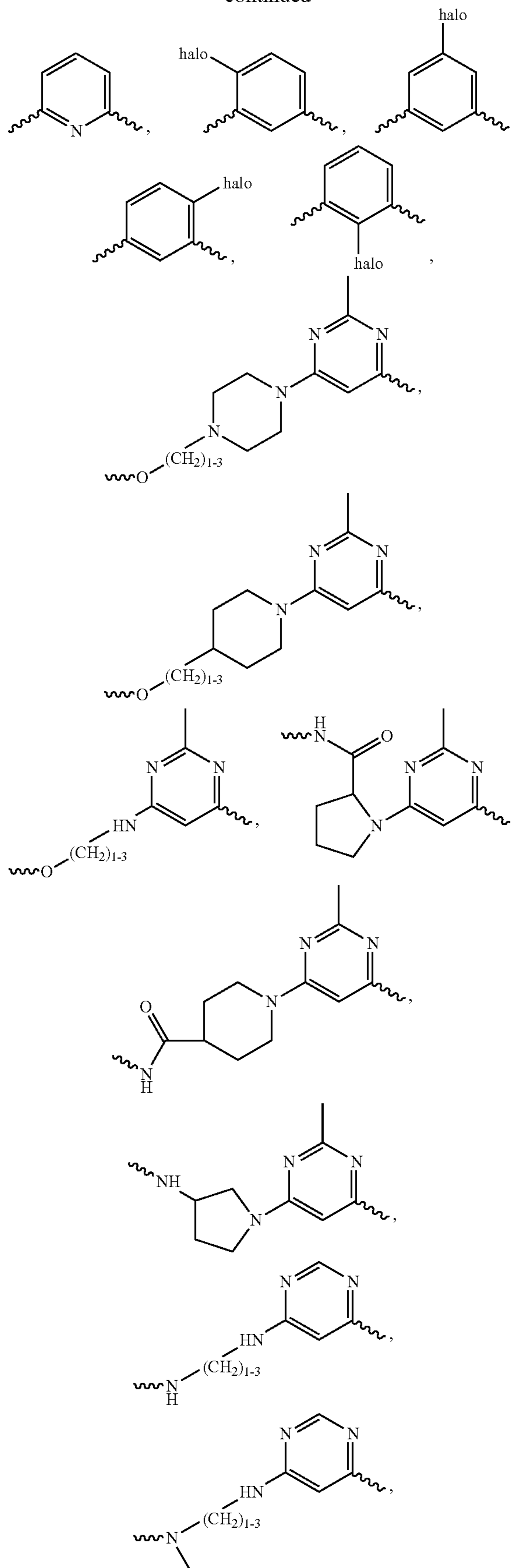
Formula Ib-C
