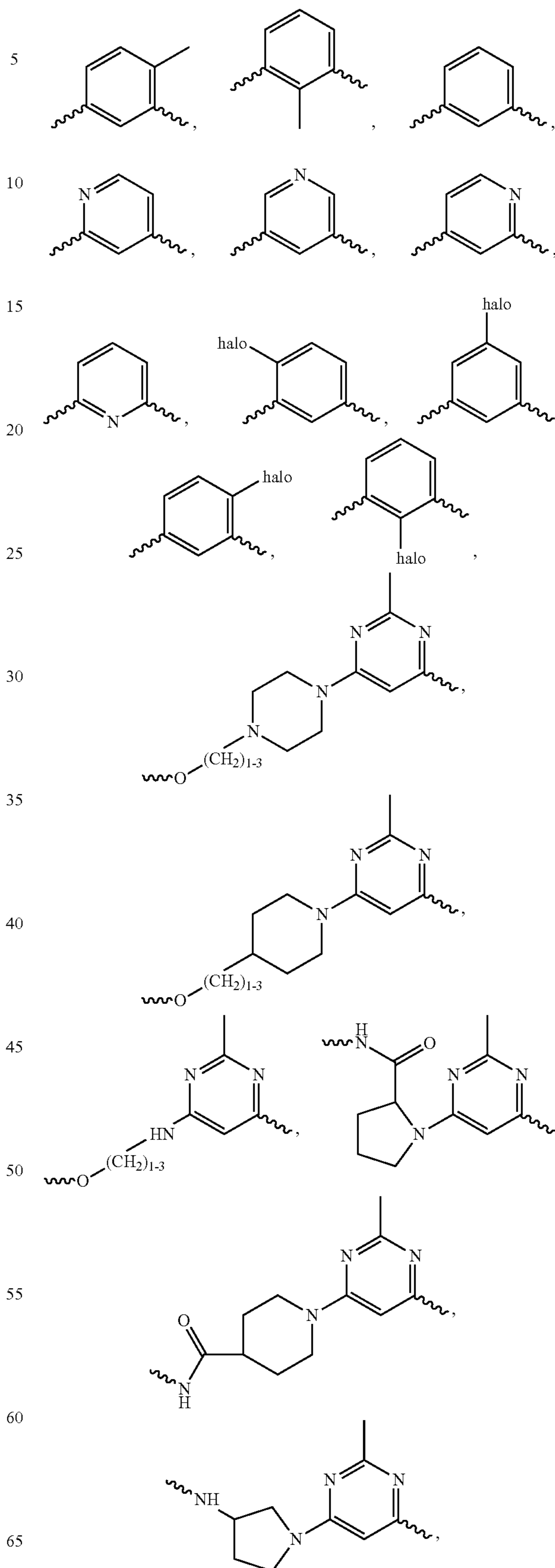
Formula Ia-C
