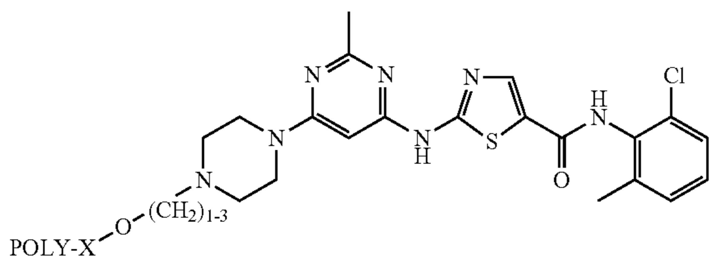
Formula Ic-C
