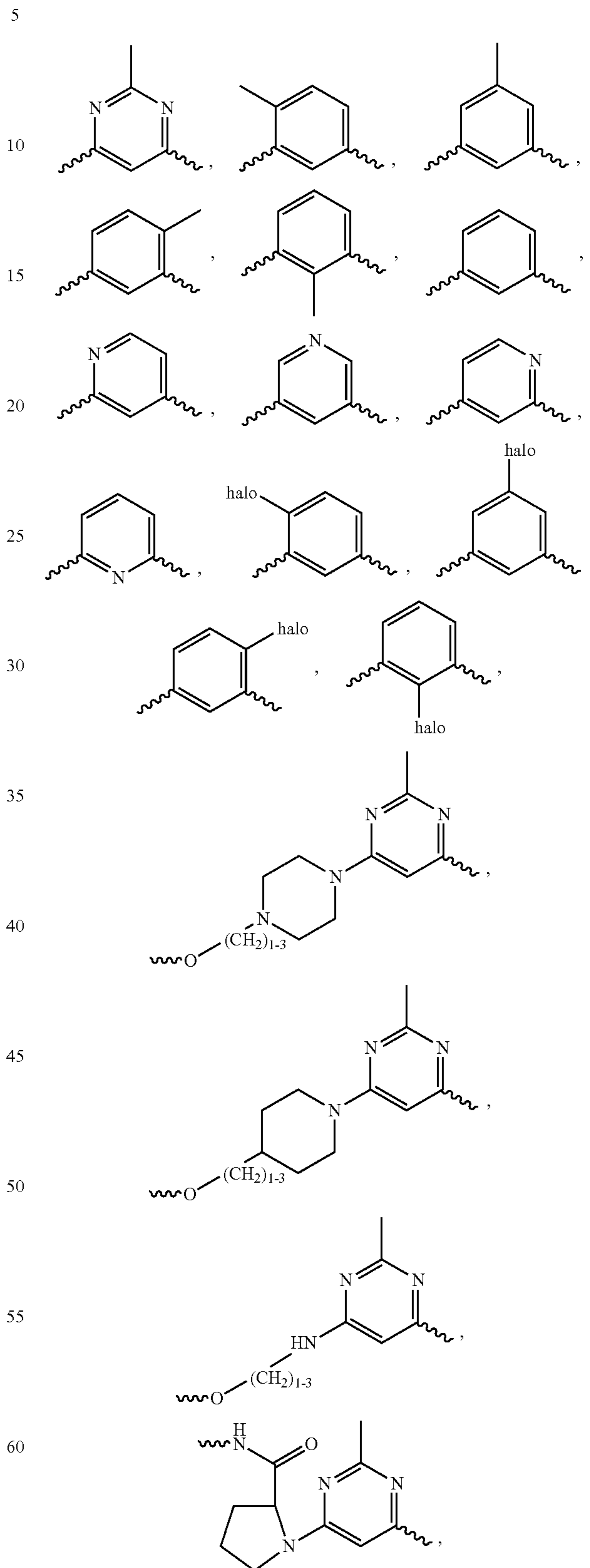
Formula Ia-C
