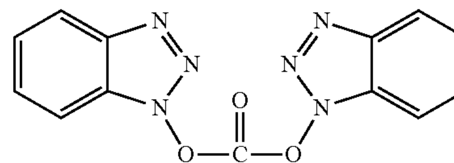
di(1-benzotriazolyl)carbonate (diBTC)
