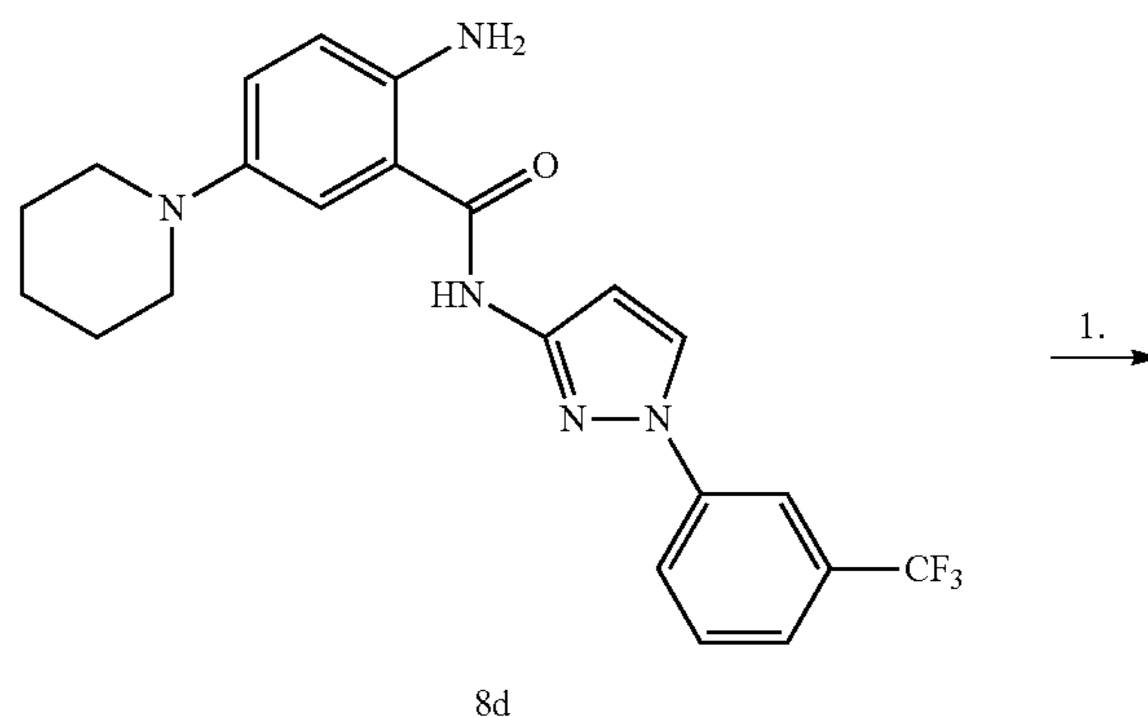
Scheme 11:
