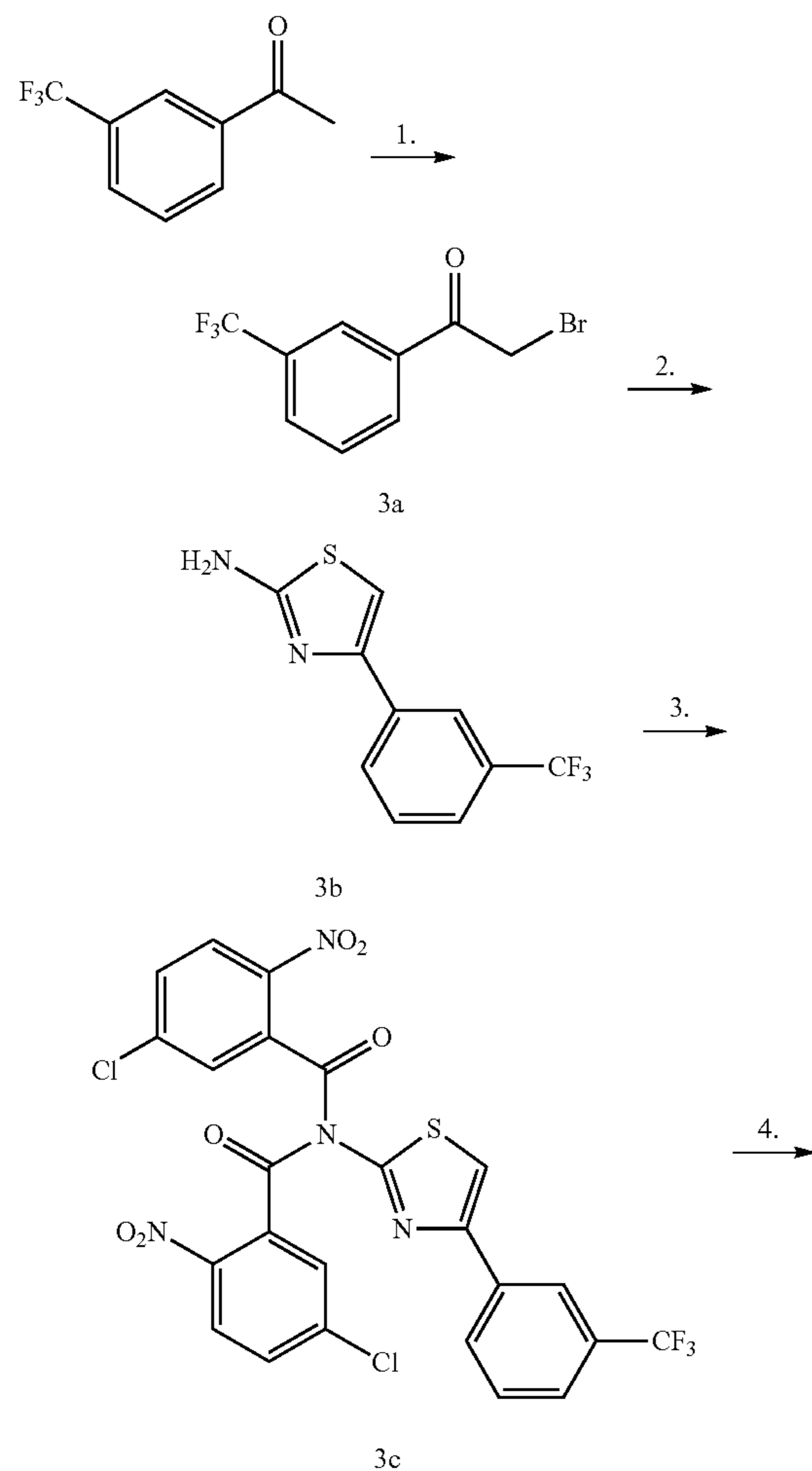
Scheme 3.
