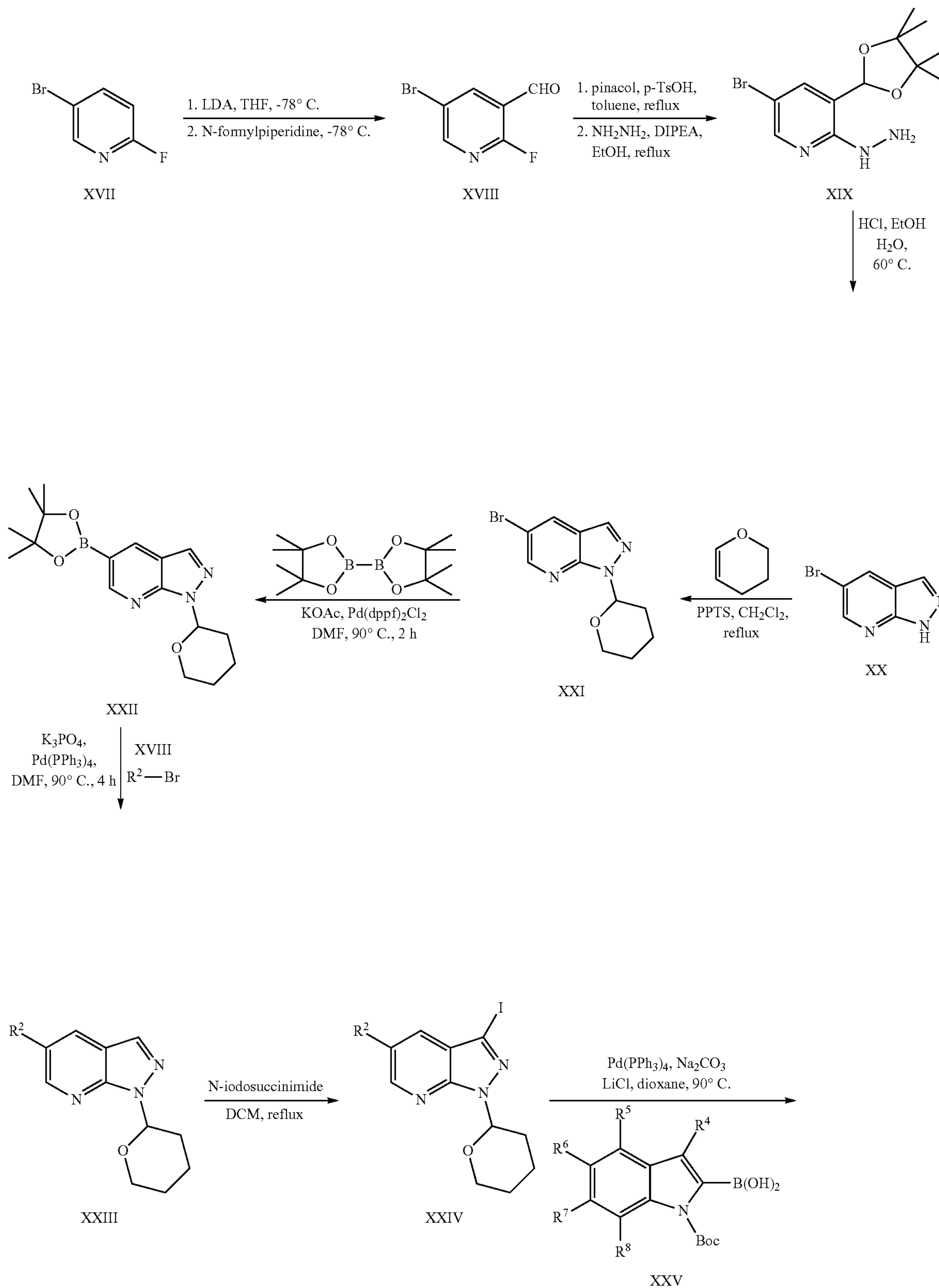
Scheme 3
