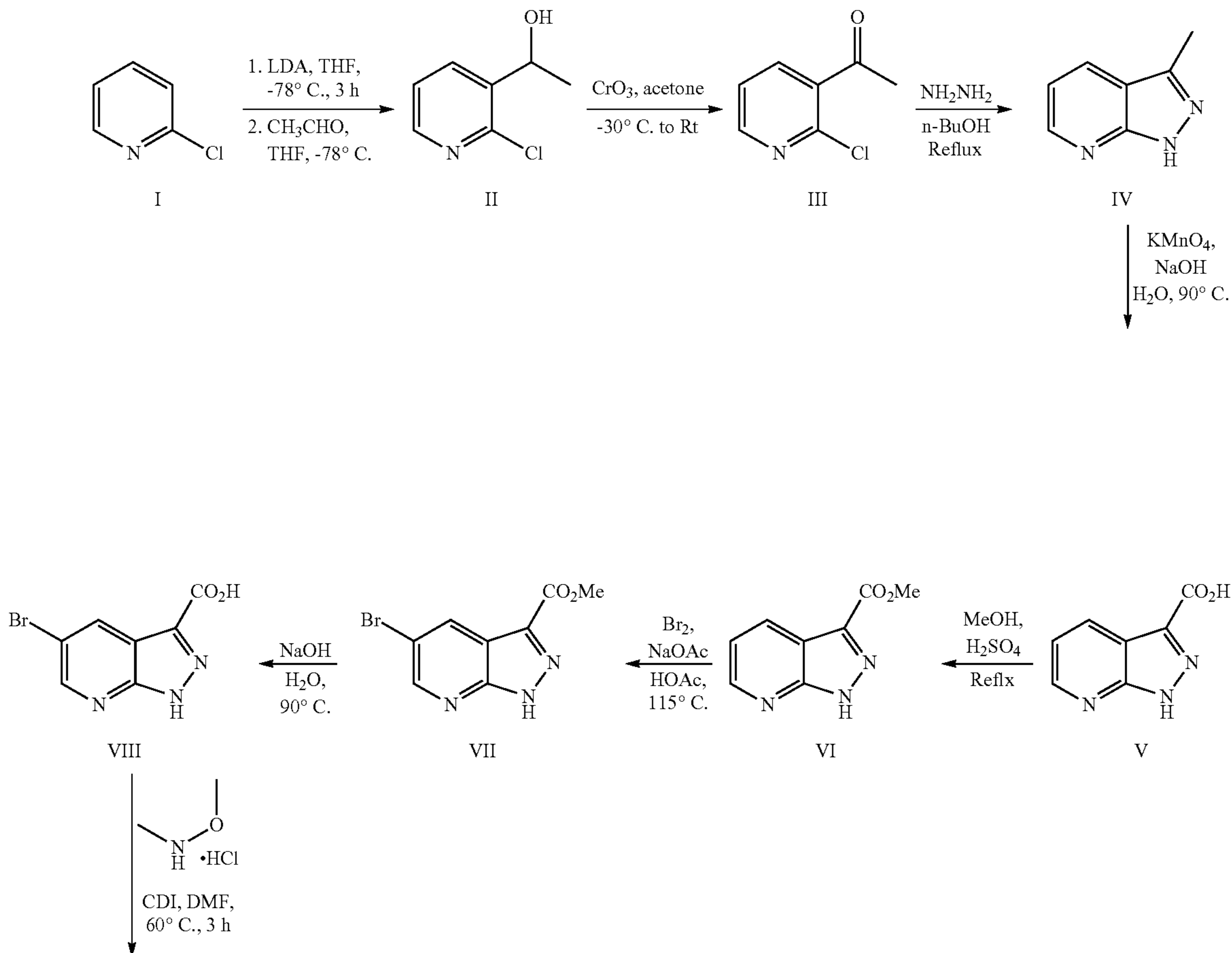
Scheme 1
