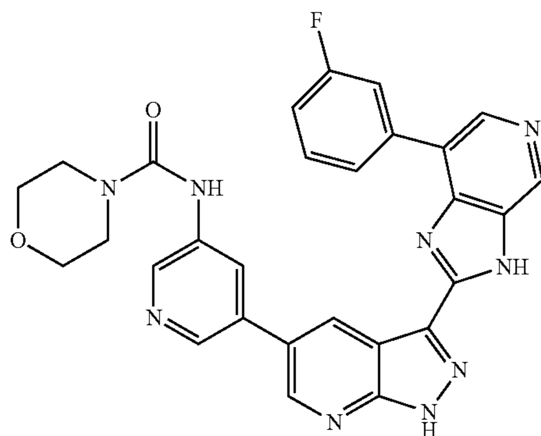
N-(5-(3-(7-(3-fluorophenyl)-3H-imidazo[4,5-c]pyridin-2-yl)-1H-pyrazolo[3,4-b]pyridin-5-yl)pyridin-3-yl)morpholine-4-carboxamide 62
