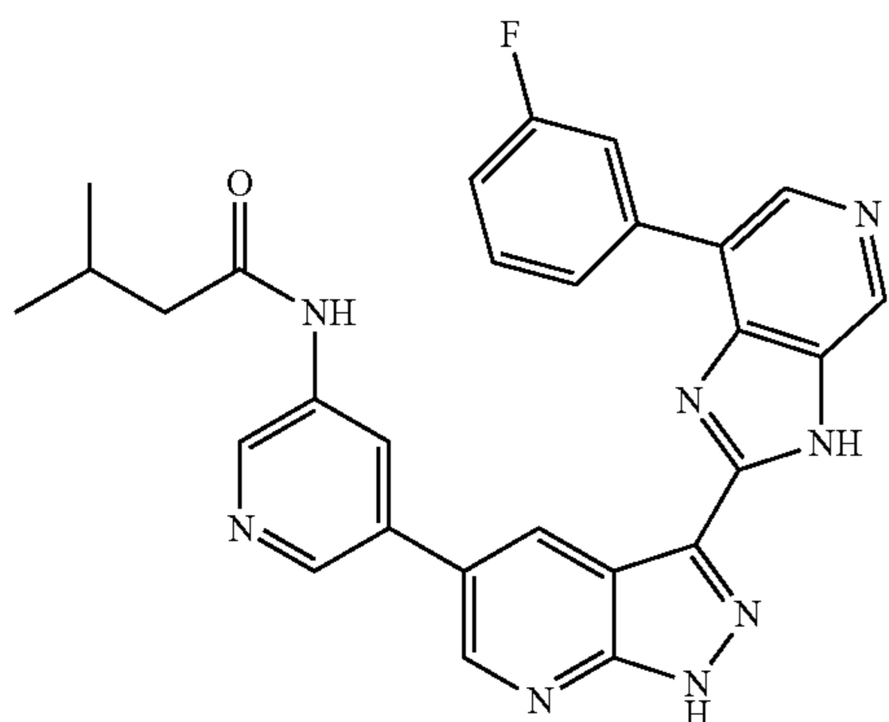
N-(5-(3-(7-(3-fluorophenyl)-3H-imidazo[4,5-c]pyridin-2-yl)-1H-pyrazolo[3,4-b]pyridin-5-yl)pyridin-3-yl)-3-methylbutanamide 61
