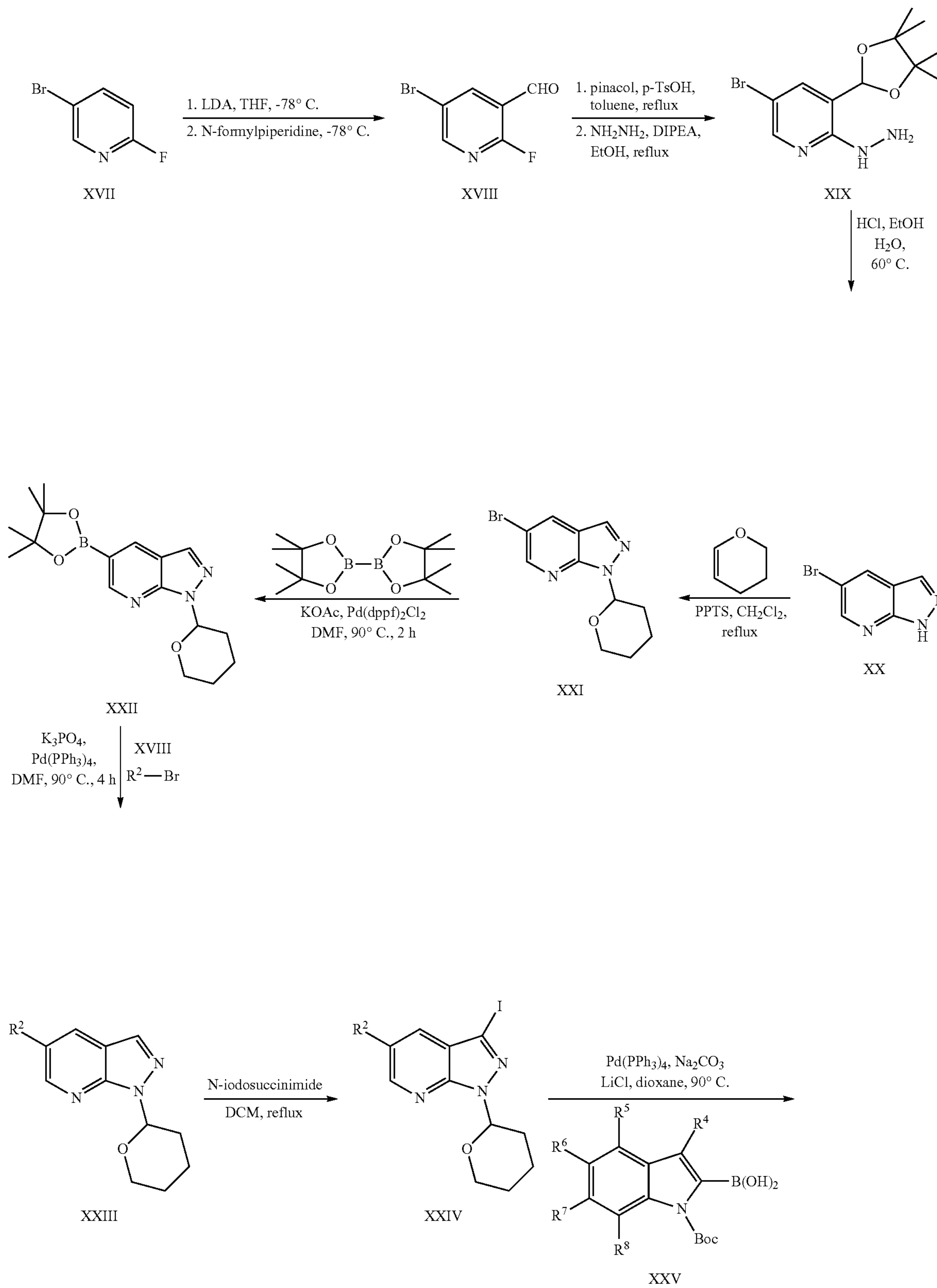
Scheme 3
