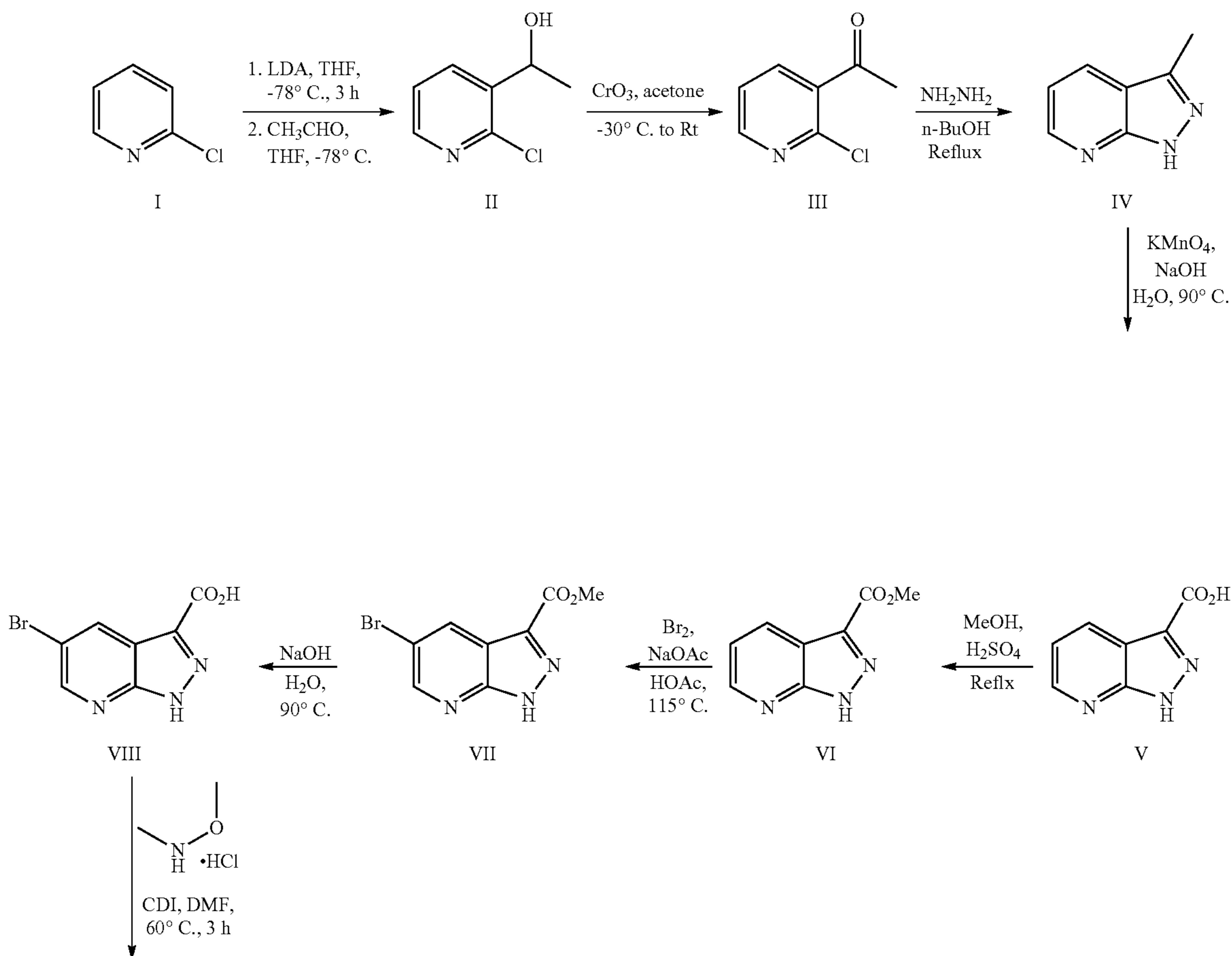
Scheme 1
