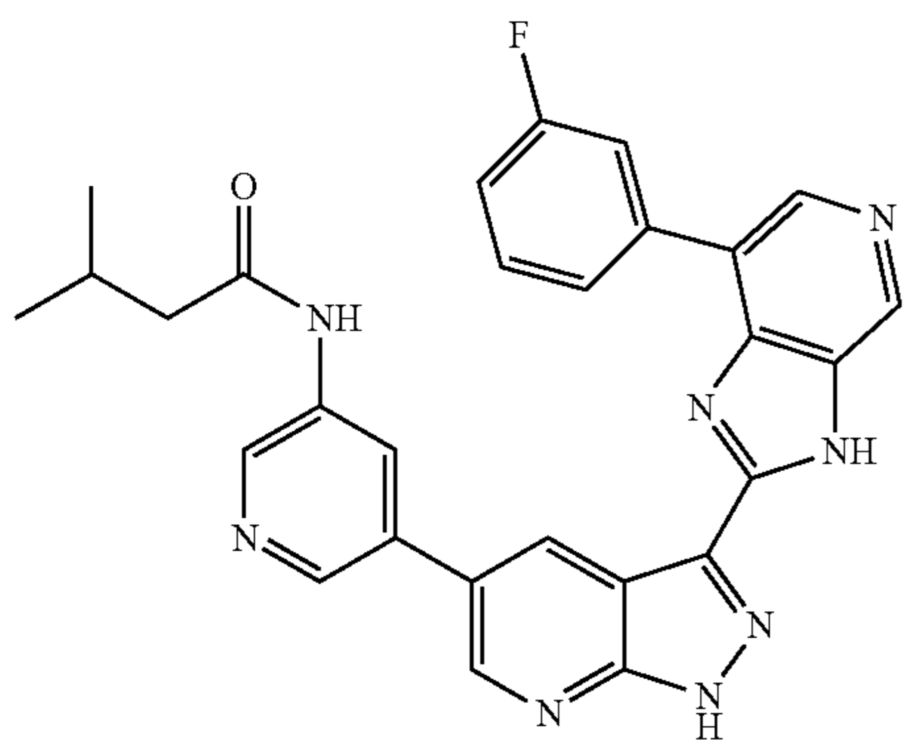
N-(5-(3-(7-(3-fluorophenyl)-3H-imidazo[4,5-c]pyridin-2-yl)-1H-pyrazolo[3,4-b]pyridin-5-yl)pyridin-3-yl)-3-methylbutanamide 61
