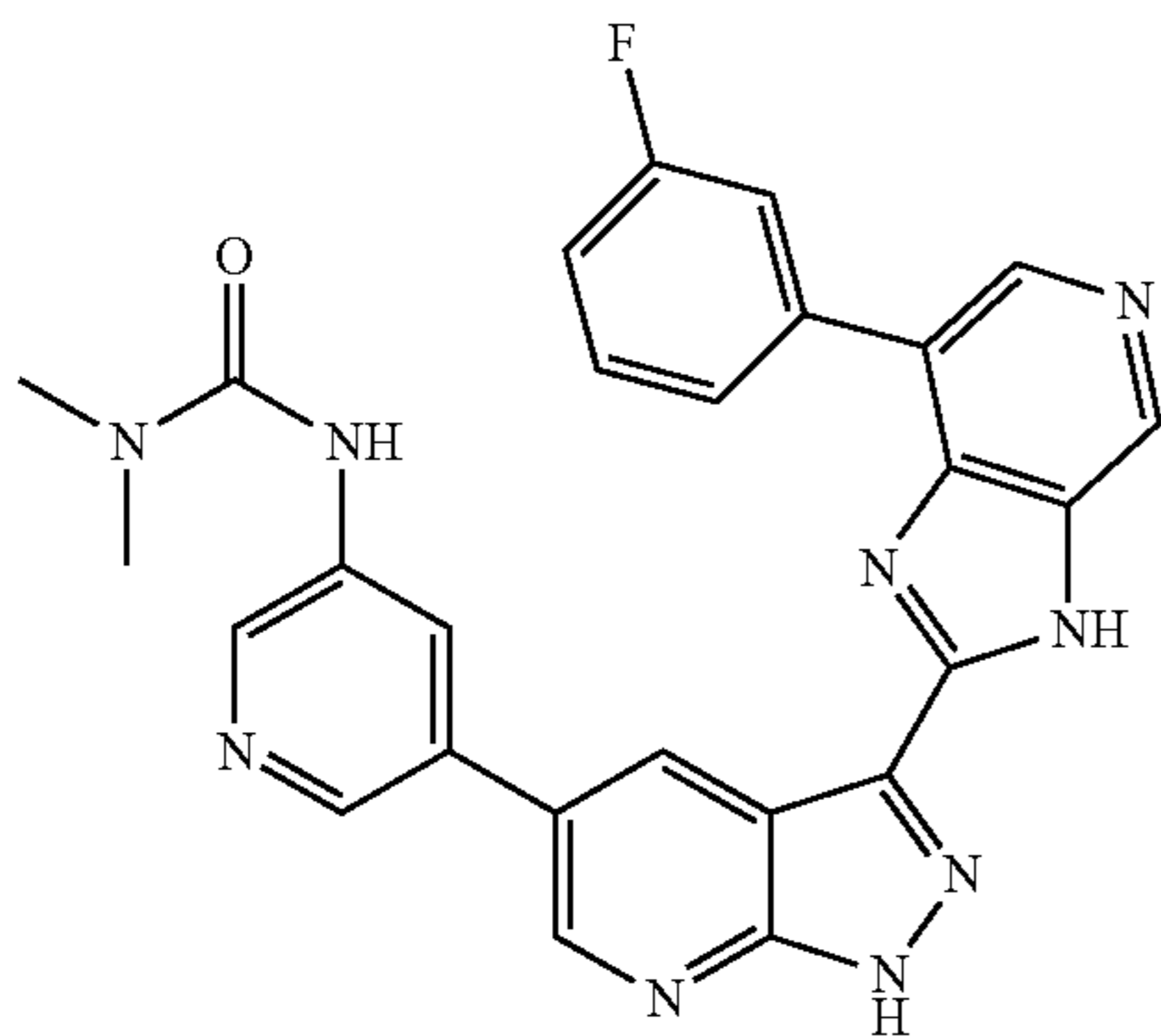
3-(5-(3-(7-(3-fluorophenyl)-3H-imidazo[4,5-c]pyridin-2-yl)-1H-pyrazolo[3,4-b]pyridin-5-yl)pyridin-3-yl)-1,1-dimethylurea 66
