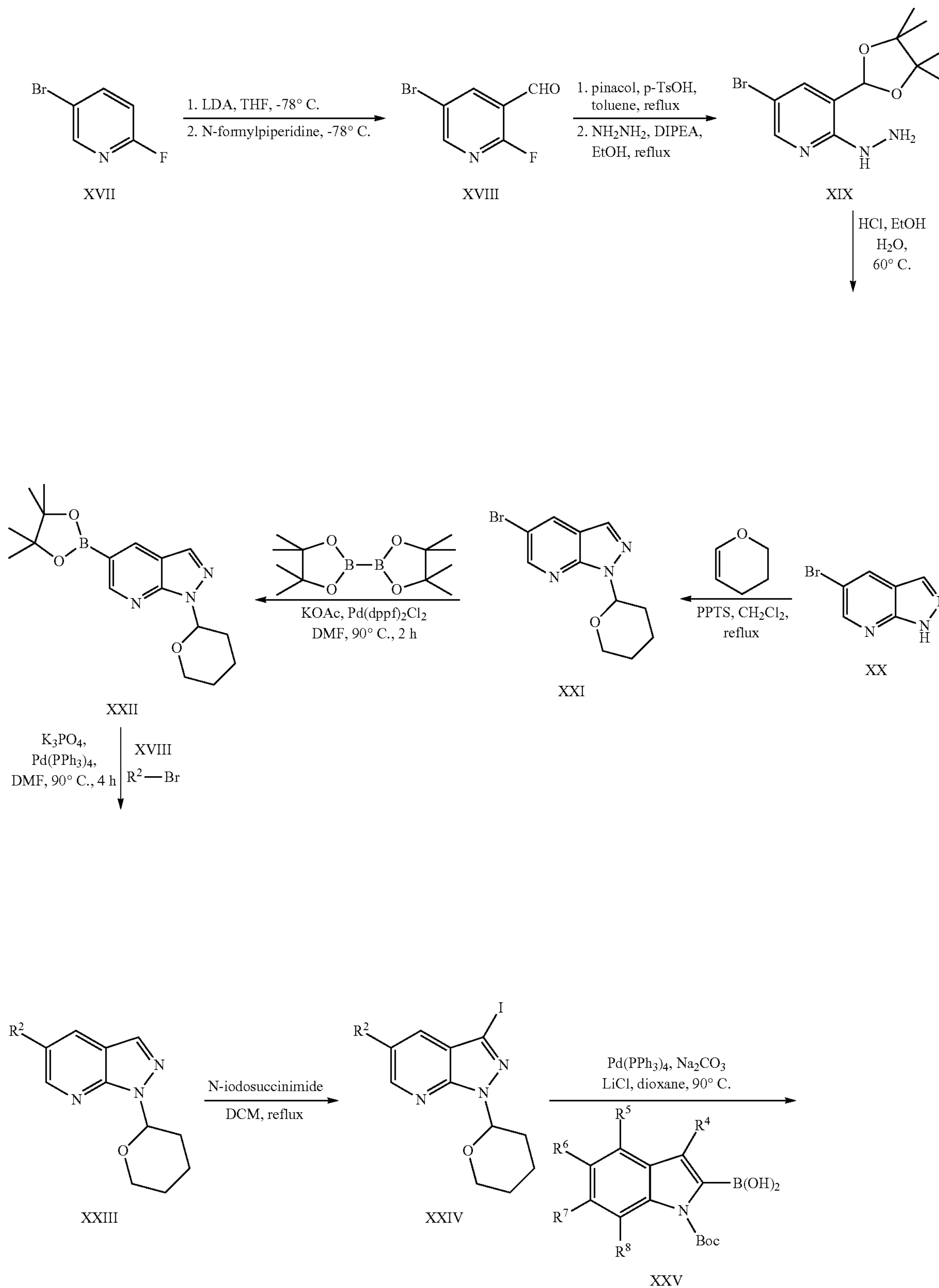
Scheme 3
