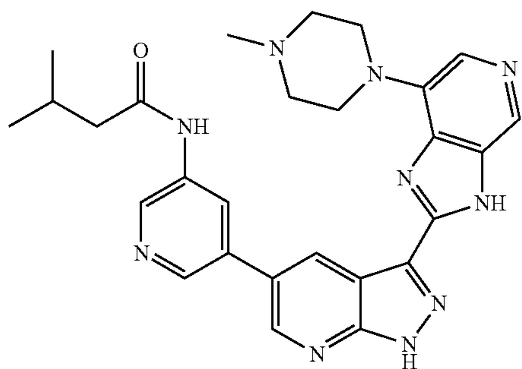
3-methyl-N-(5-(3-(7-(4-methylpiperazin-1-yl)-3H-imidazo[4,5-c]pyridin-2-yl)-1H-pyrazolo[3,4-b]pyridin-5-yl)pyridin-3-yl)butanamide 57
