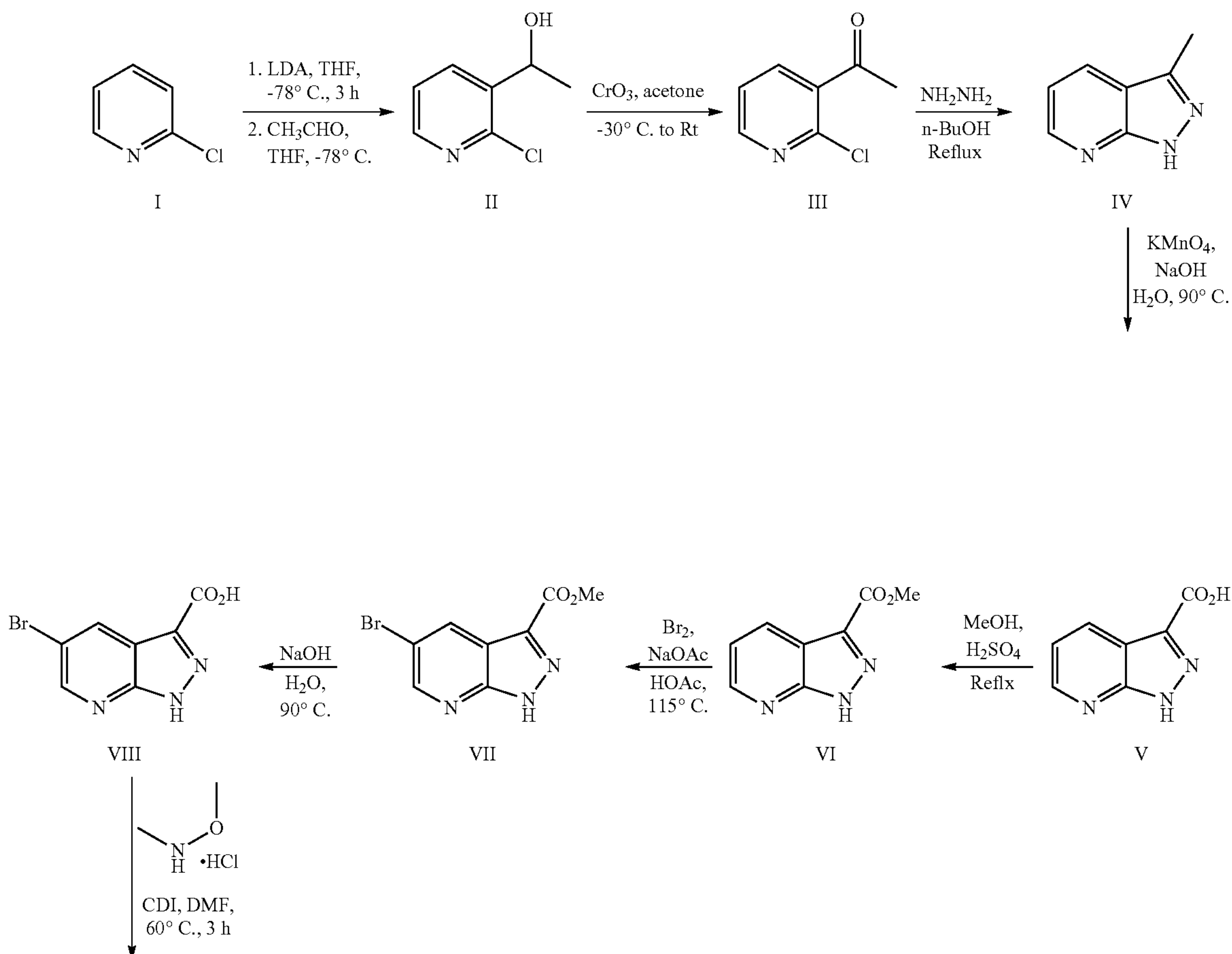
Scheme 1
