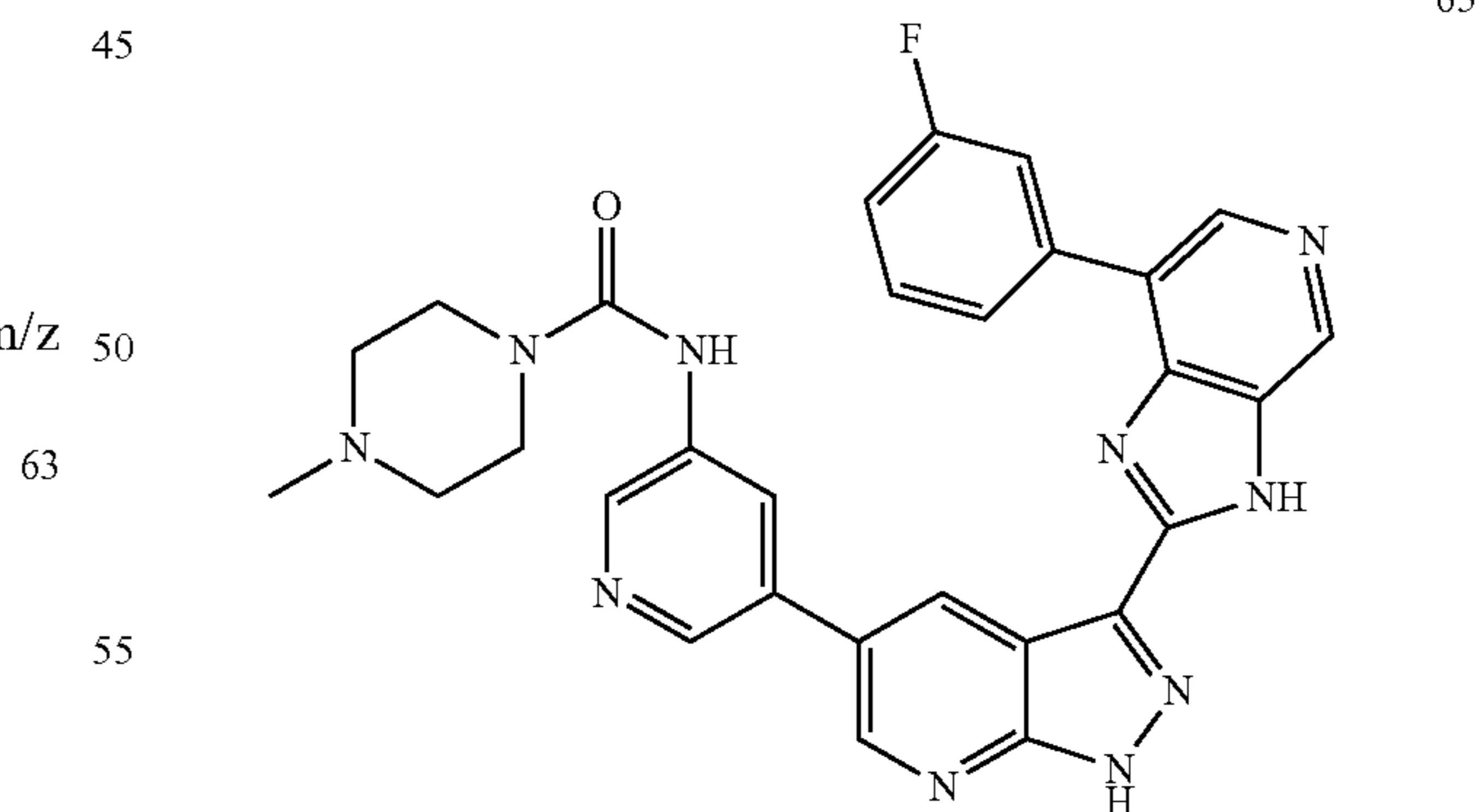
N-(5-(3-(7-(3-fluorophenyl)-3H-imidazo[4,5-c]pyridin-2-yl)-1H-pyrazolo[3,4-b]pyridin-5-yl)pyridin-3-yl)morpholine-4-carboxamide 62
