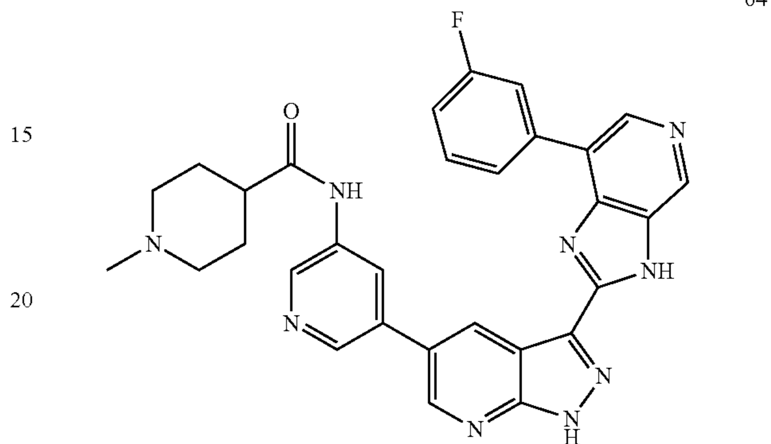
N-(5-(3-(7-(3-fluorophenyl)-3H-imidazo[4,5-c]pyridin-2-yl)-1H-pyrazolo[3,4-b]pyridin-5-yl)pyridin-3-yl)-3-methylbutanamide 61
