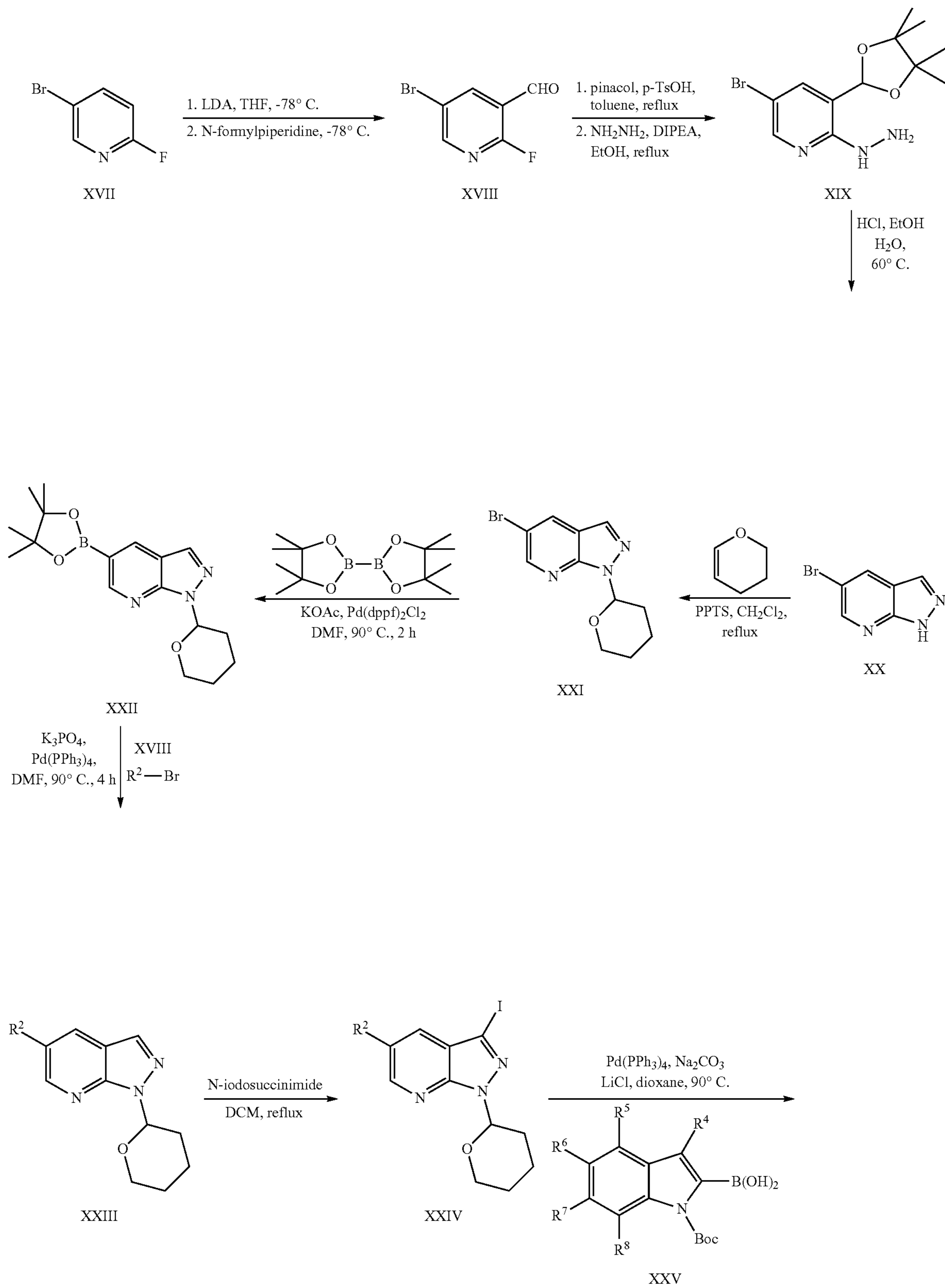
Scheme 3
