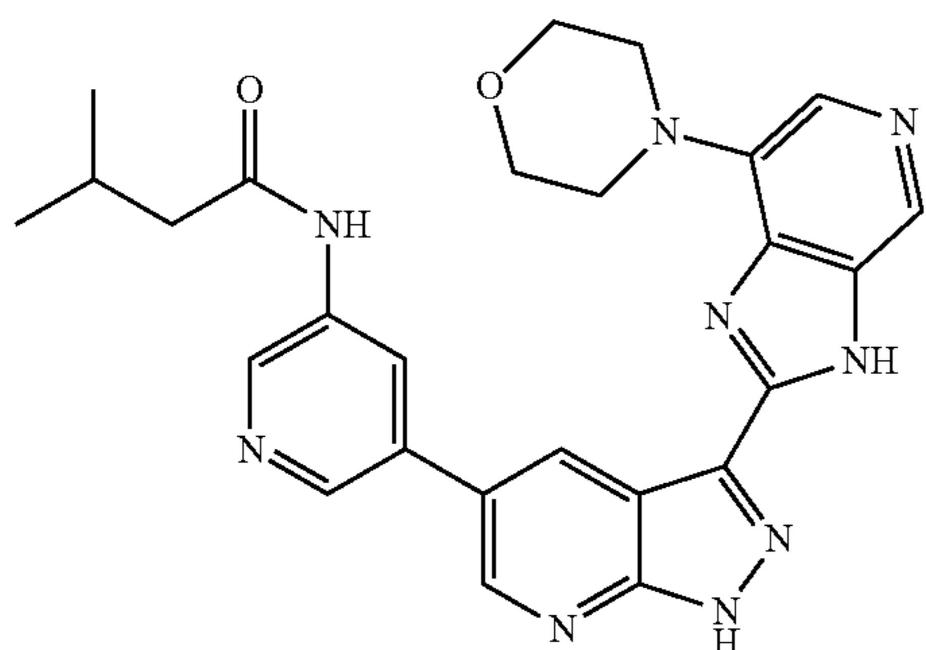
3-methyl-N-(5-(3-(7-morpholino-3H-imidazo[4,5-c]pyridin-2-yl)-1H-pyrazolo[3,4-b]pyridin-5-yl)pyridin-3-yl)butanamide 56
