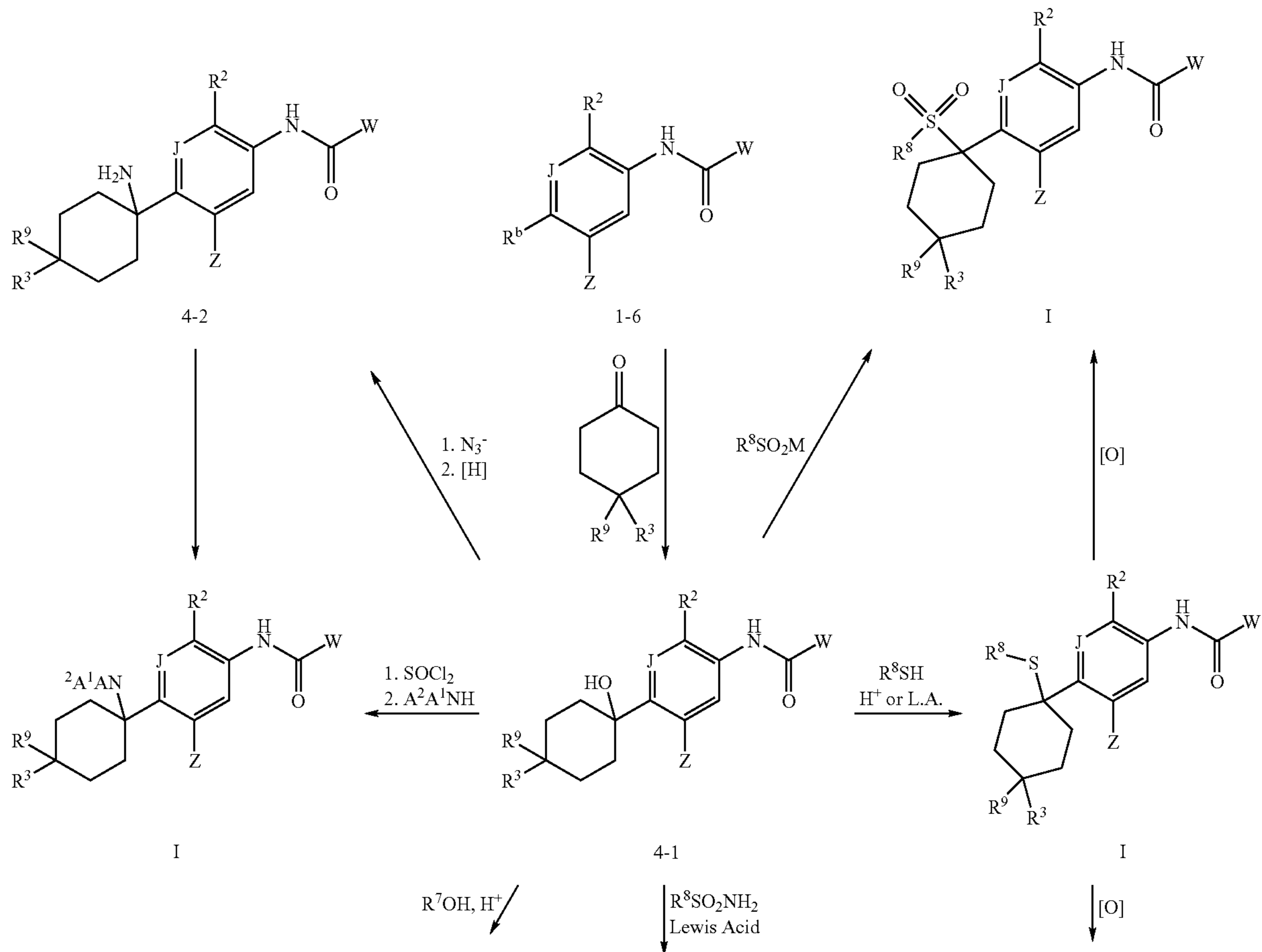
Scheme 4
