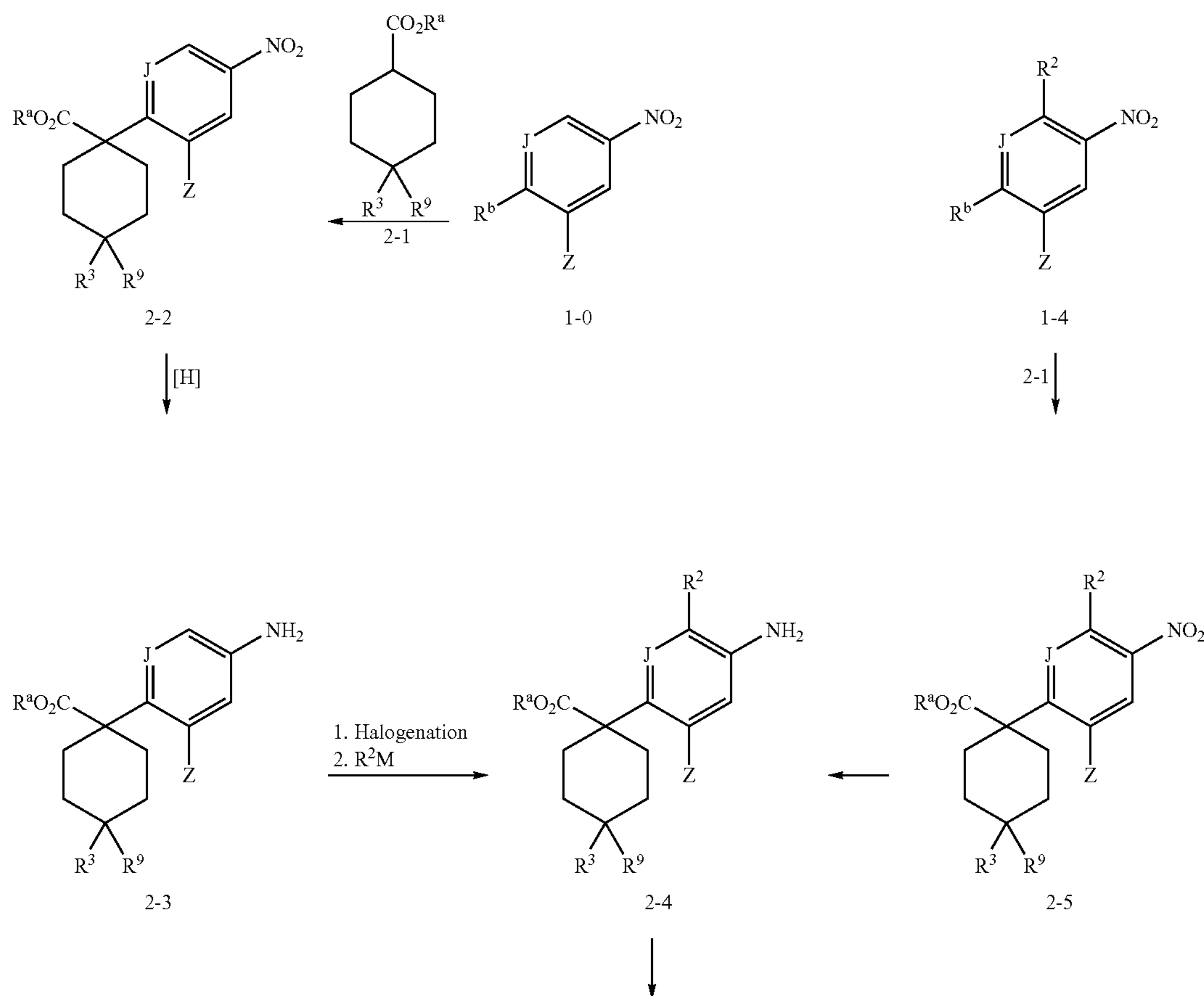
Scheme 2
