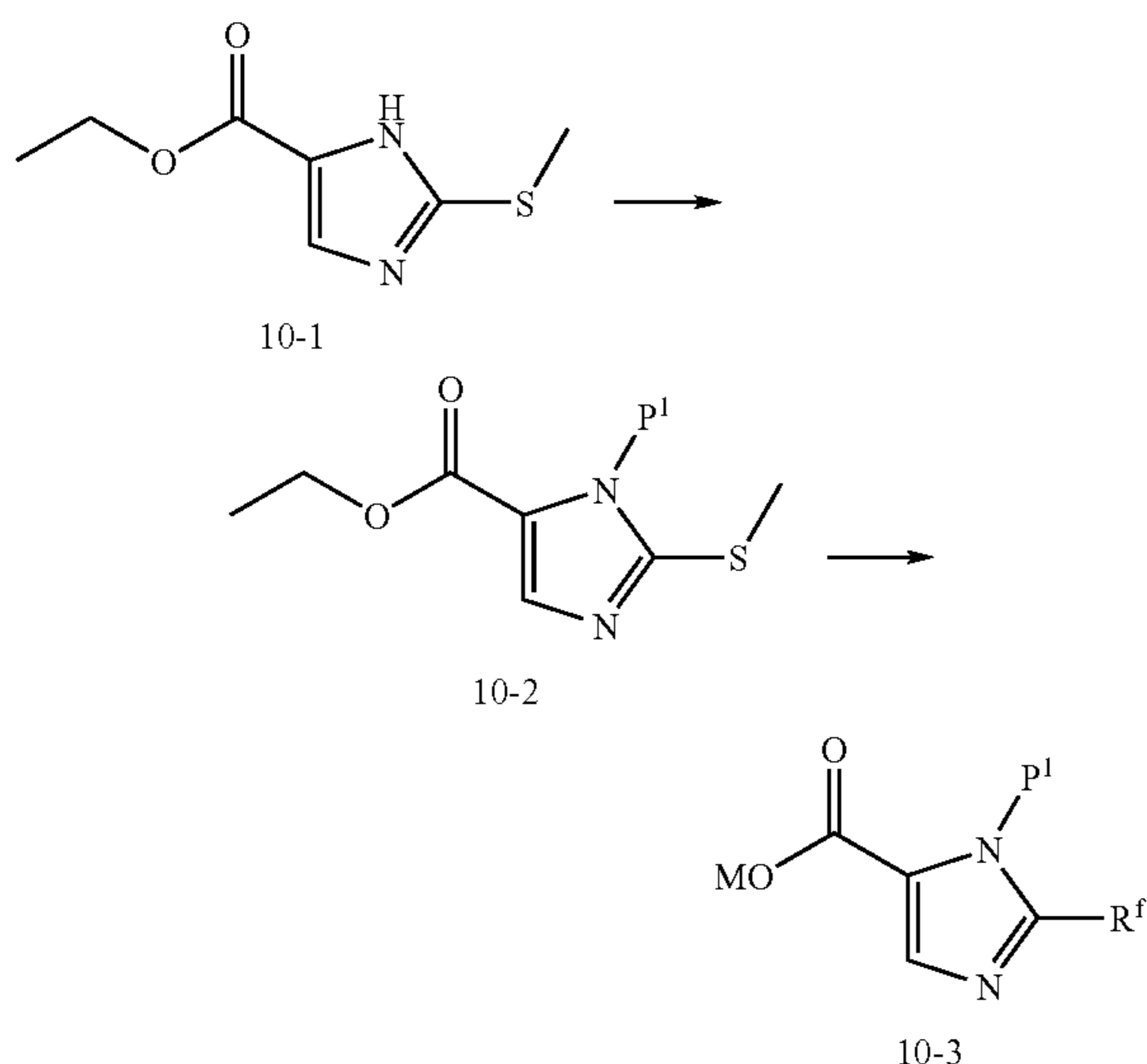
Scheme 10
