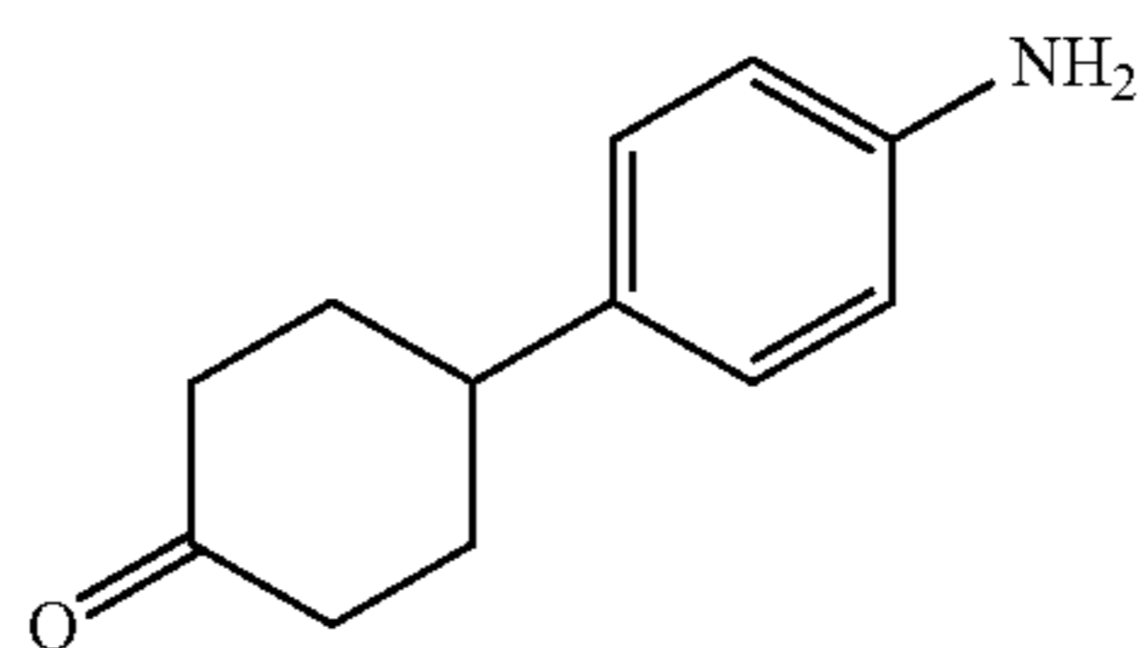
b) 4-(4-Amino-phenyl)-cyclohexanone
