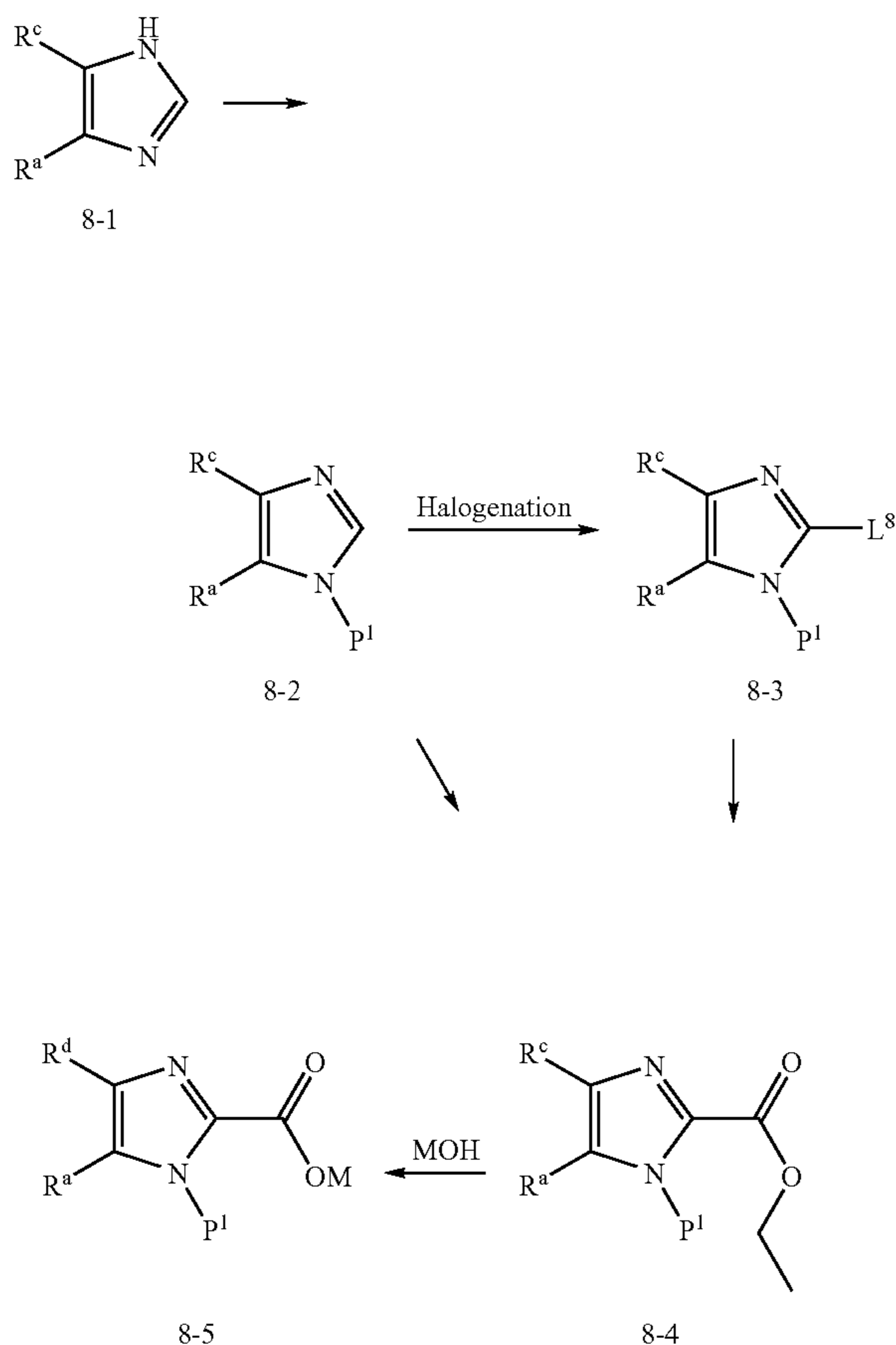
Scheme 8
