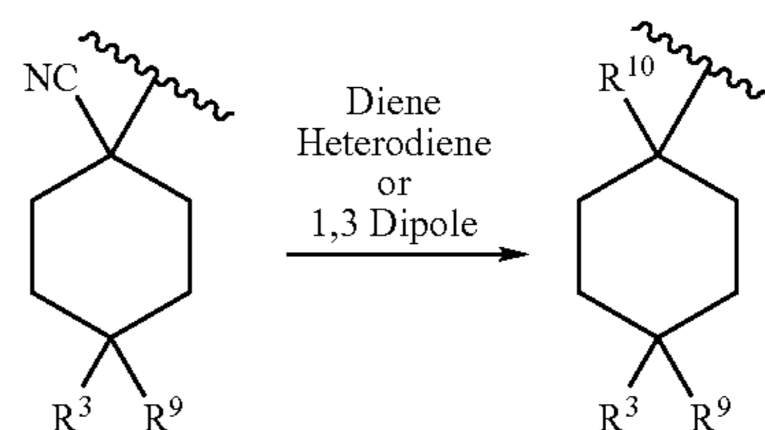
Scheme 3a
