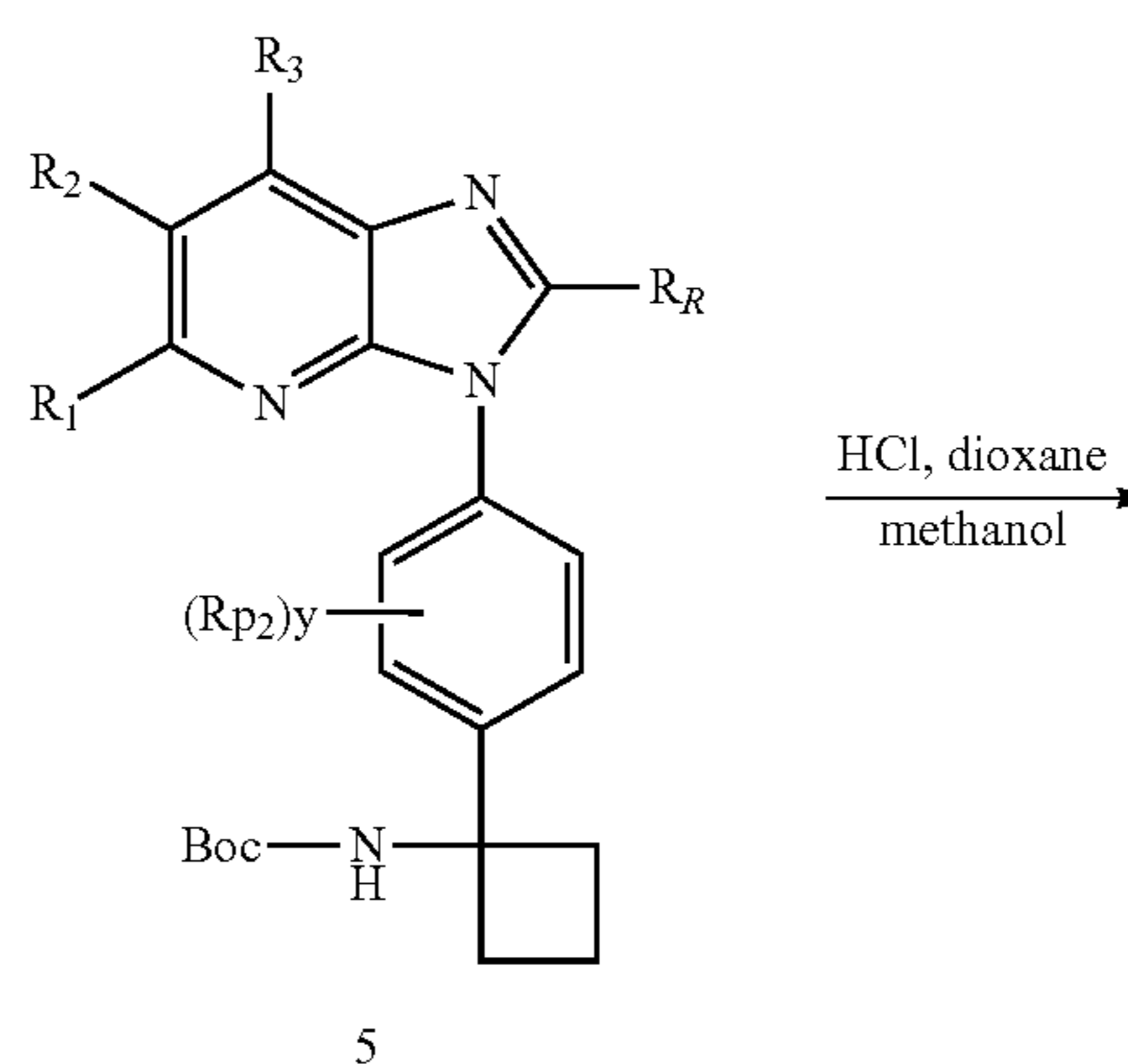
Scheme 2.: Deprotection of BOC-group
