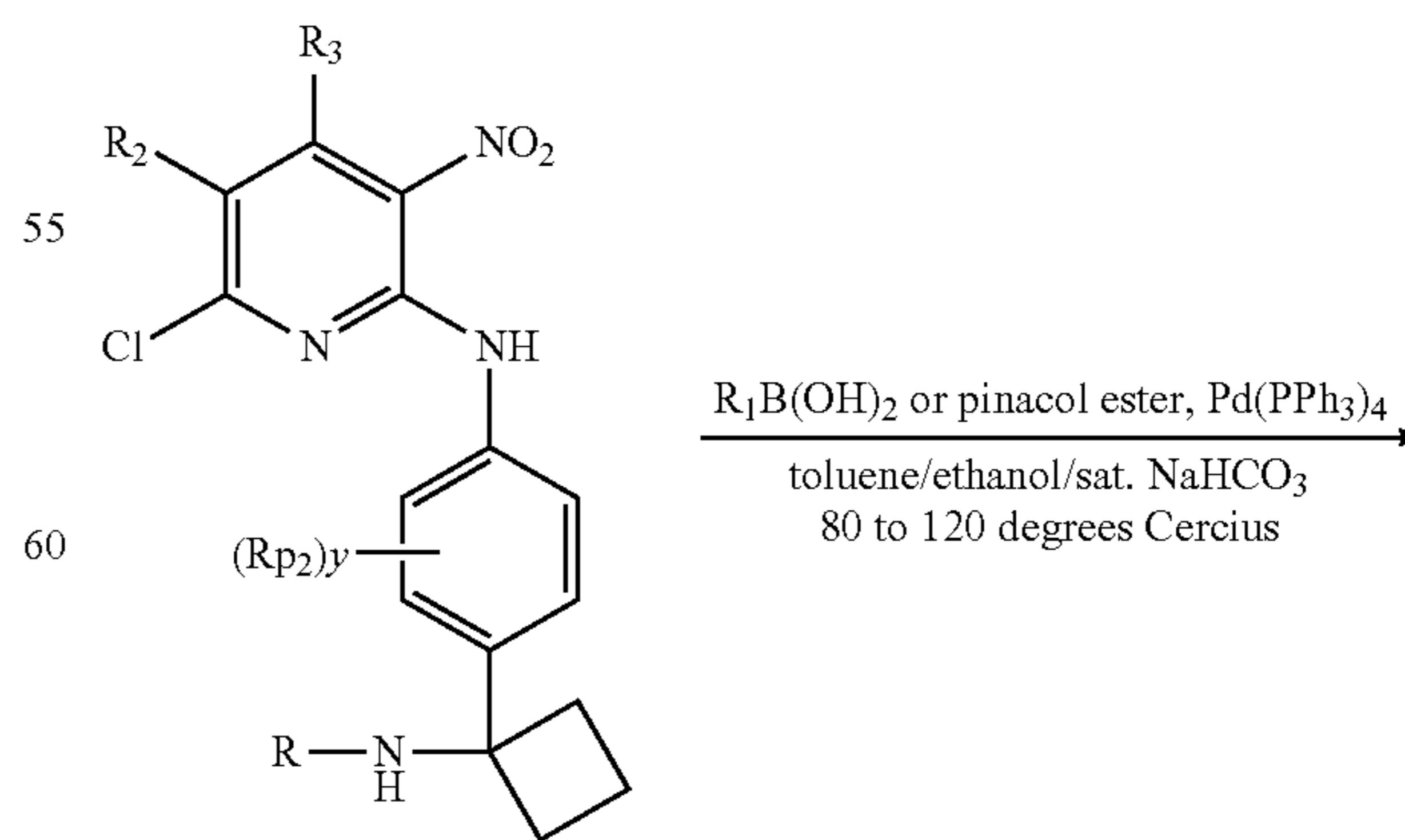
Scheme 5: Suzuki coupling 1
