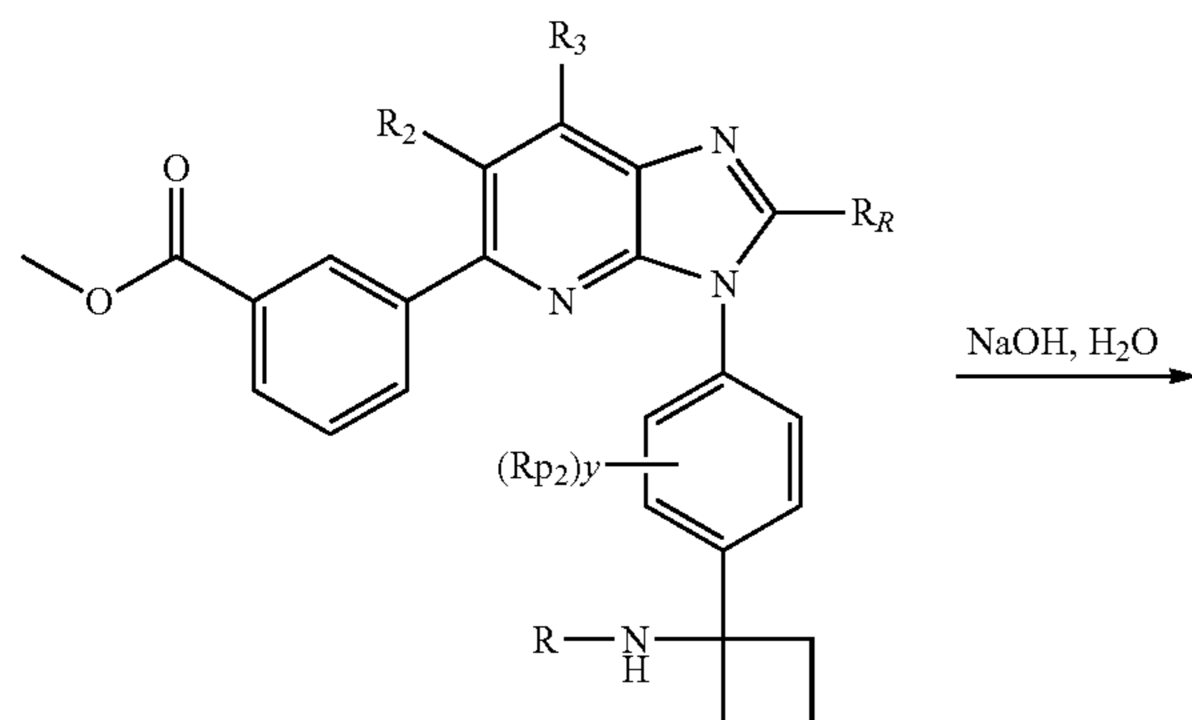
Scheme 4: Saponification
