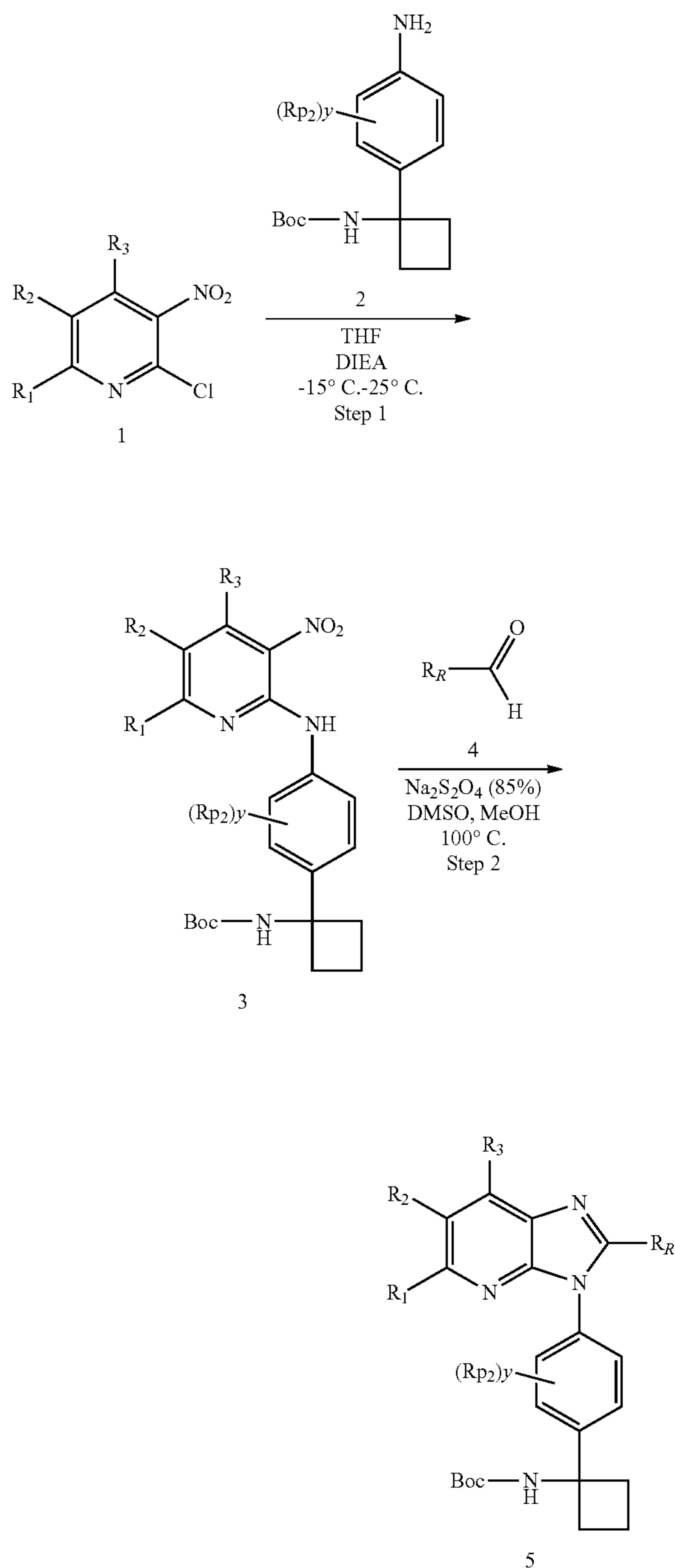
Scheme 1: Imidazopyridine formation and substitution on pyridine
