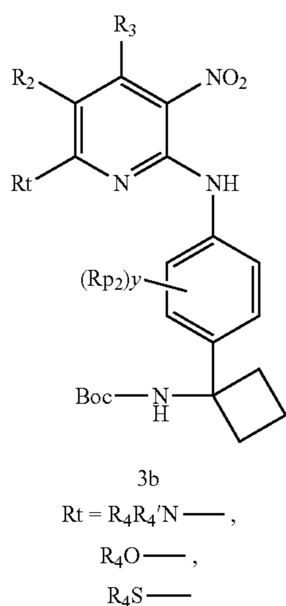
Scheme 2.: Deprotection of BOC-group
