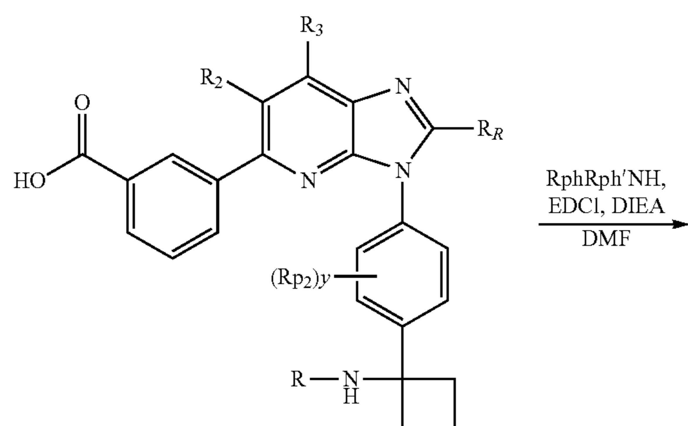
Scheme 3: Amido formation
