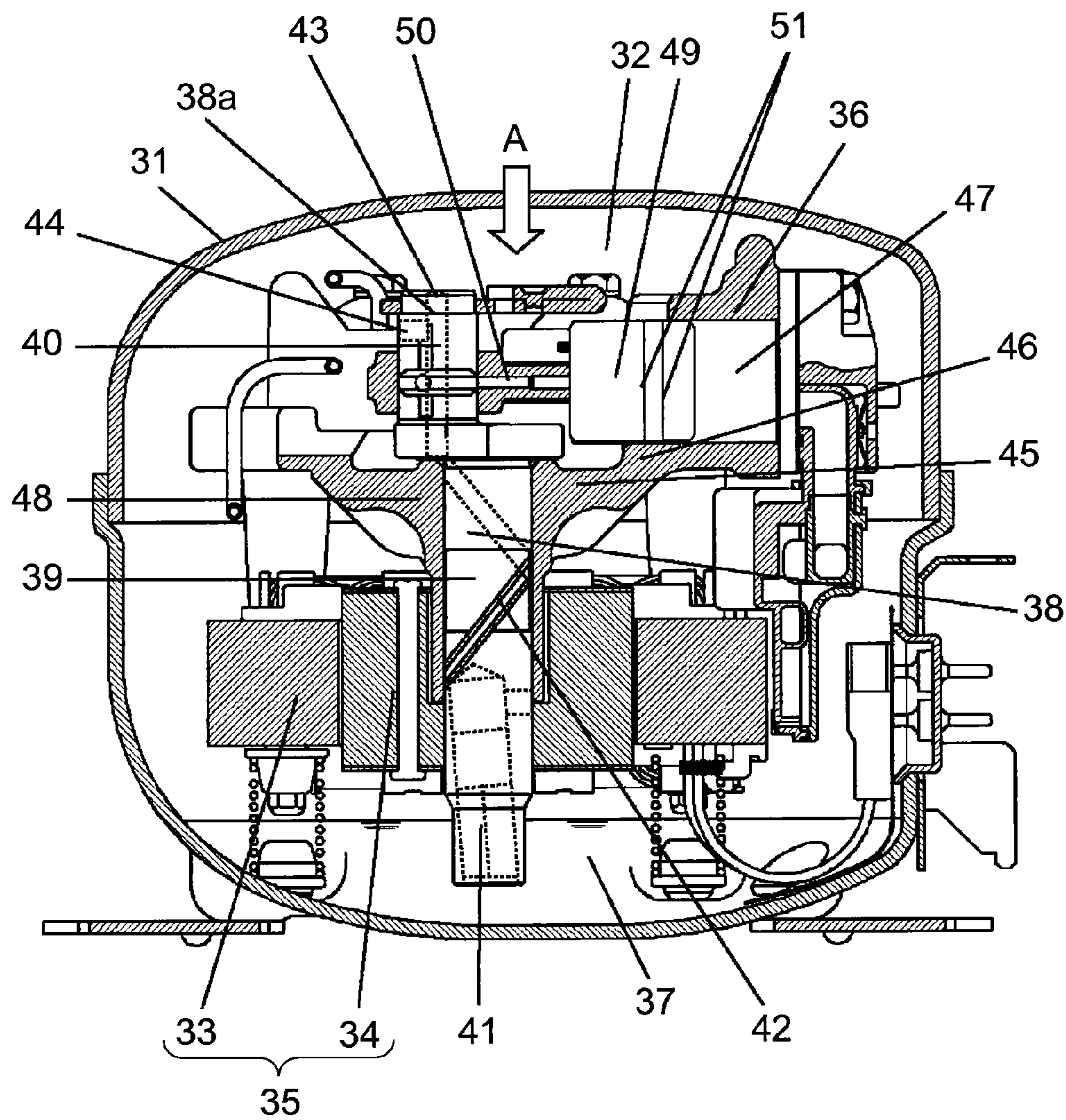
FIG. 19 PRIOR ART
