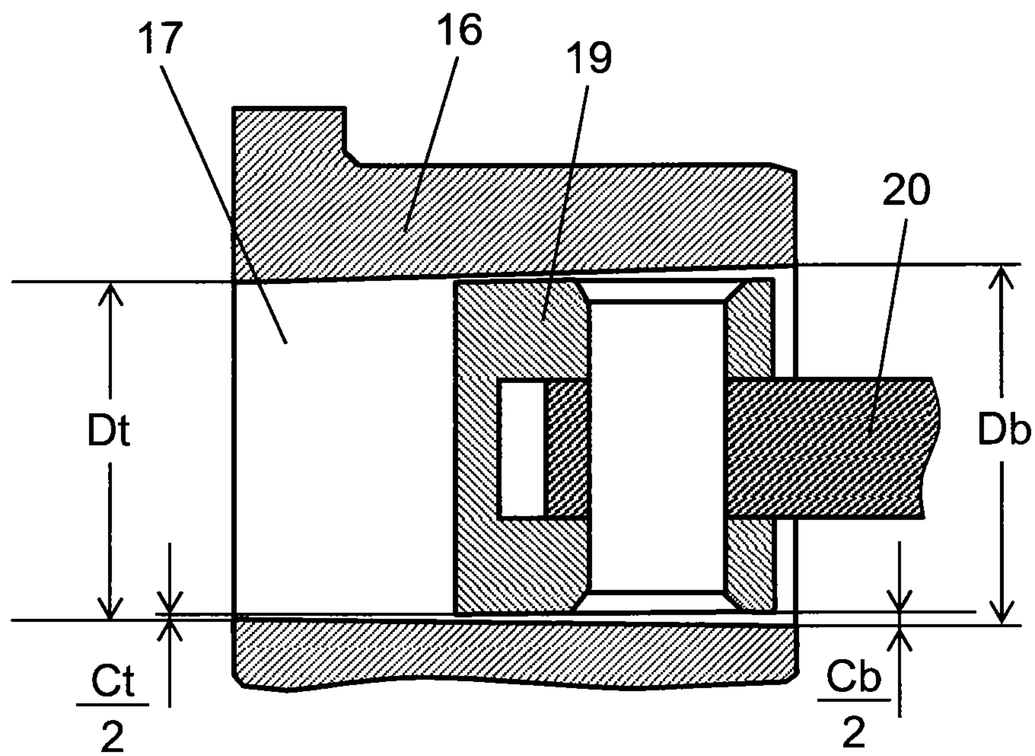
FIG. 18 PRIOR ART
