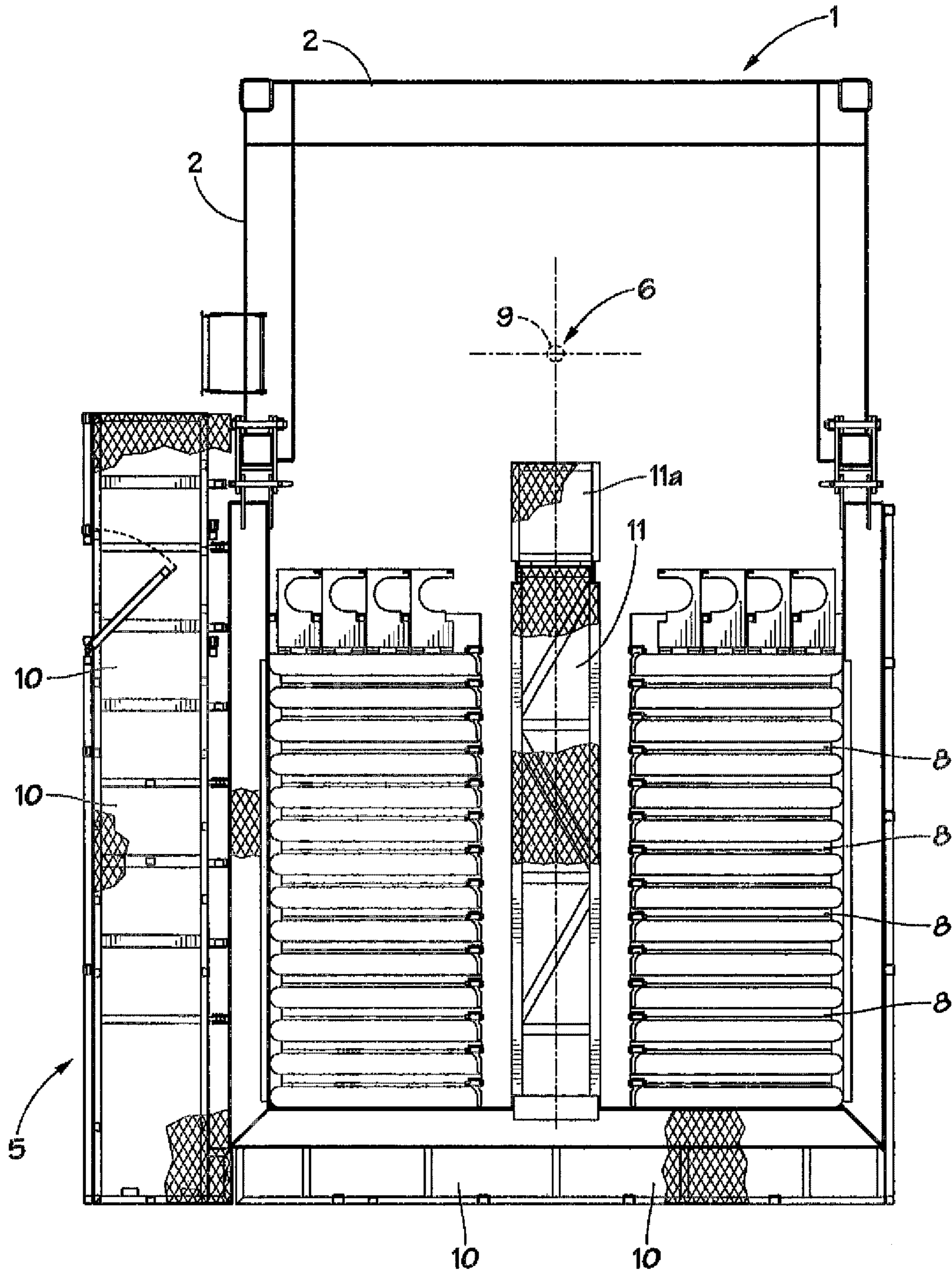
FIG. 1c (PRIOR ART)
