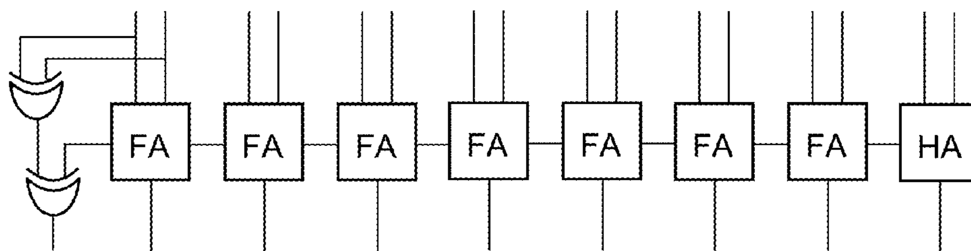
Sign-Extended 8-bit Adder
