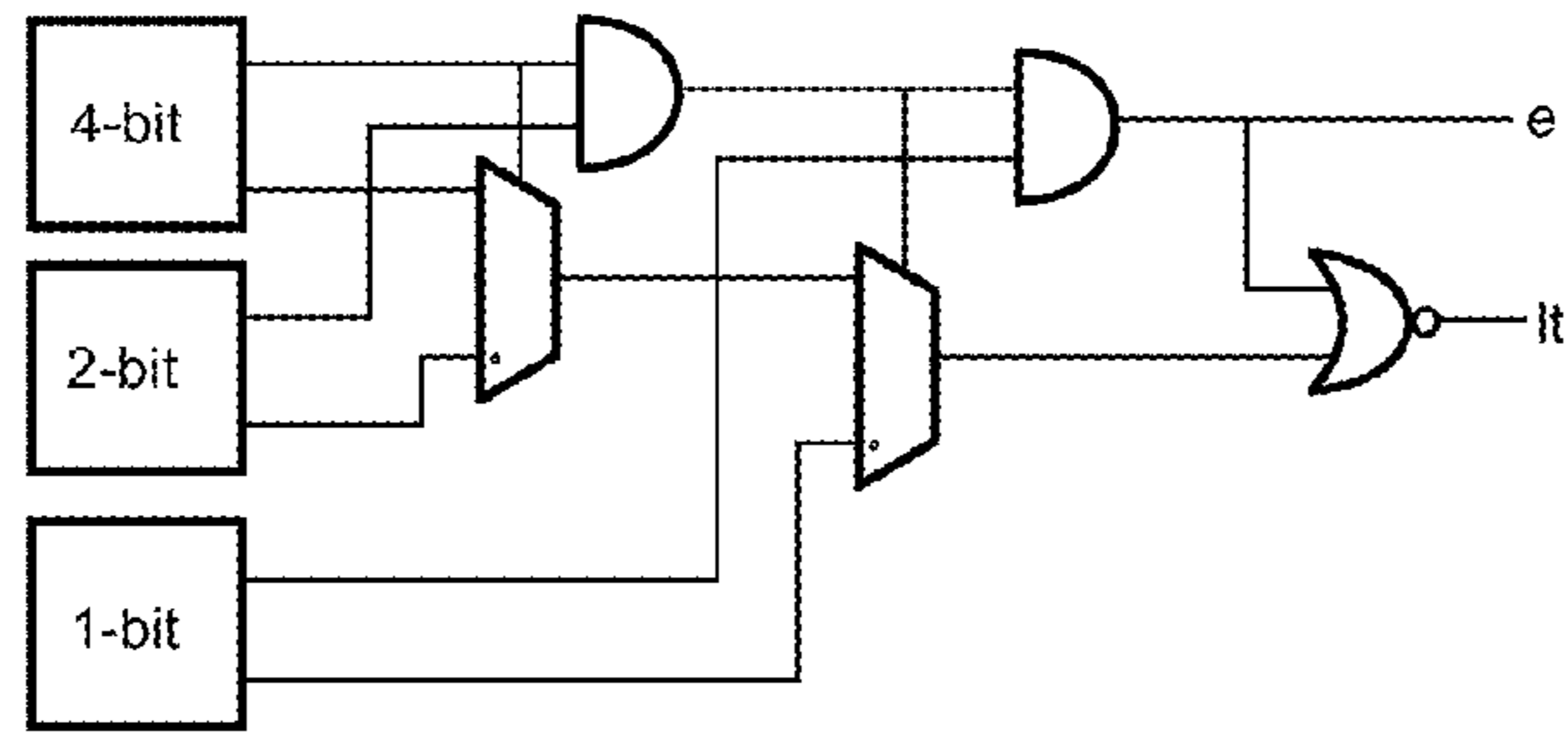
11-Bit Less Than
