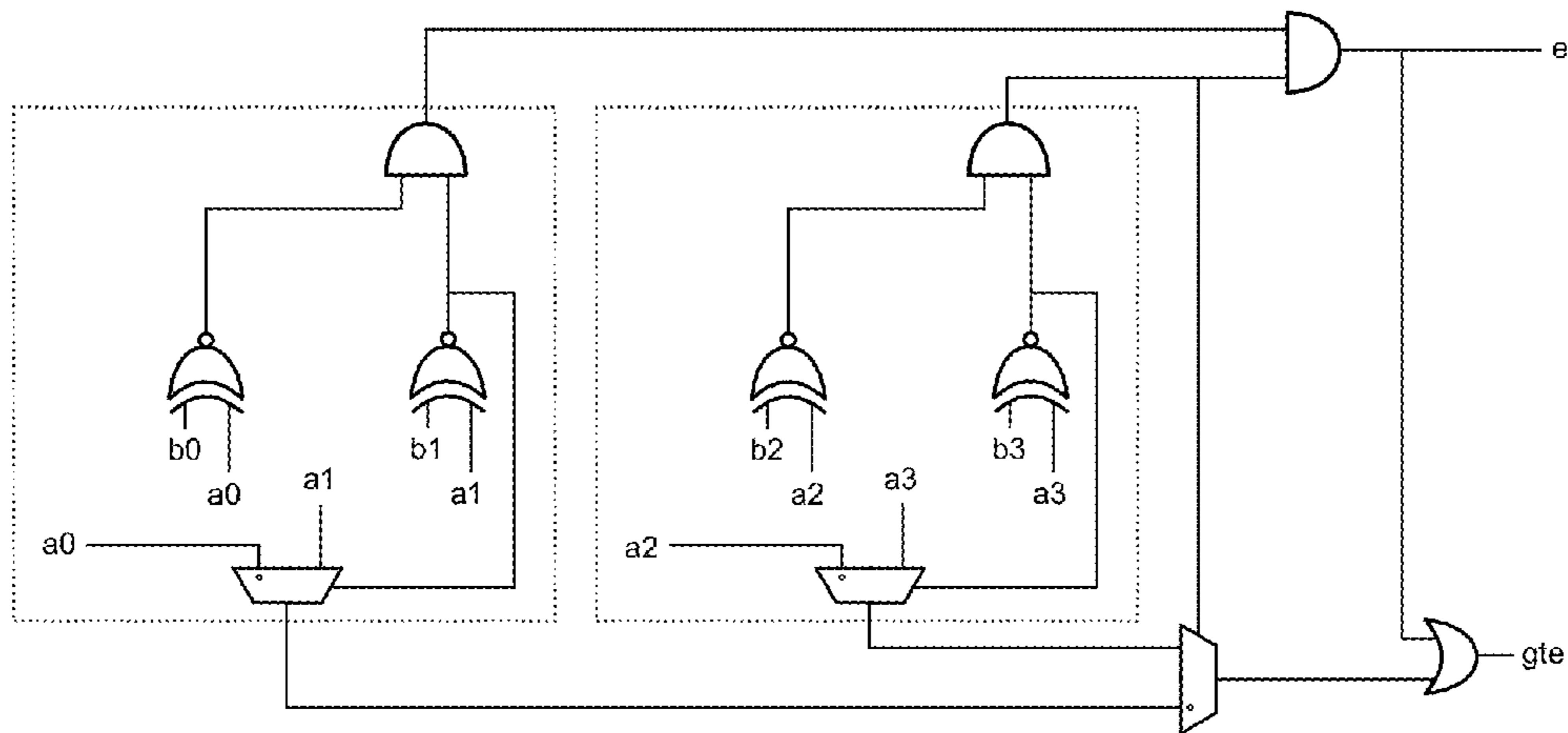
4-Bit Greater Than Or Equal
