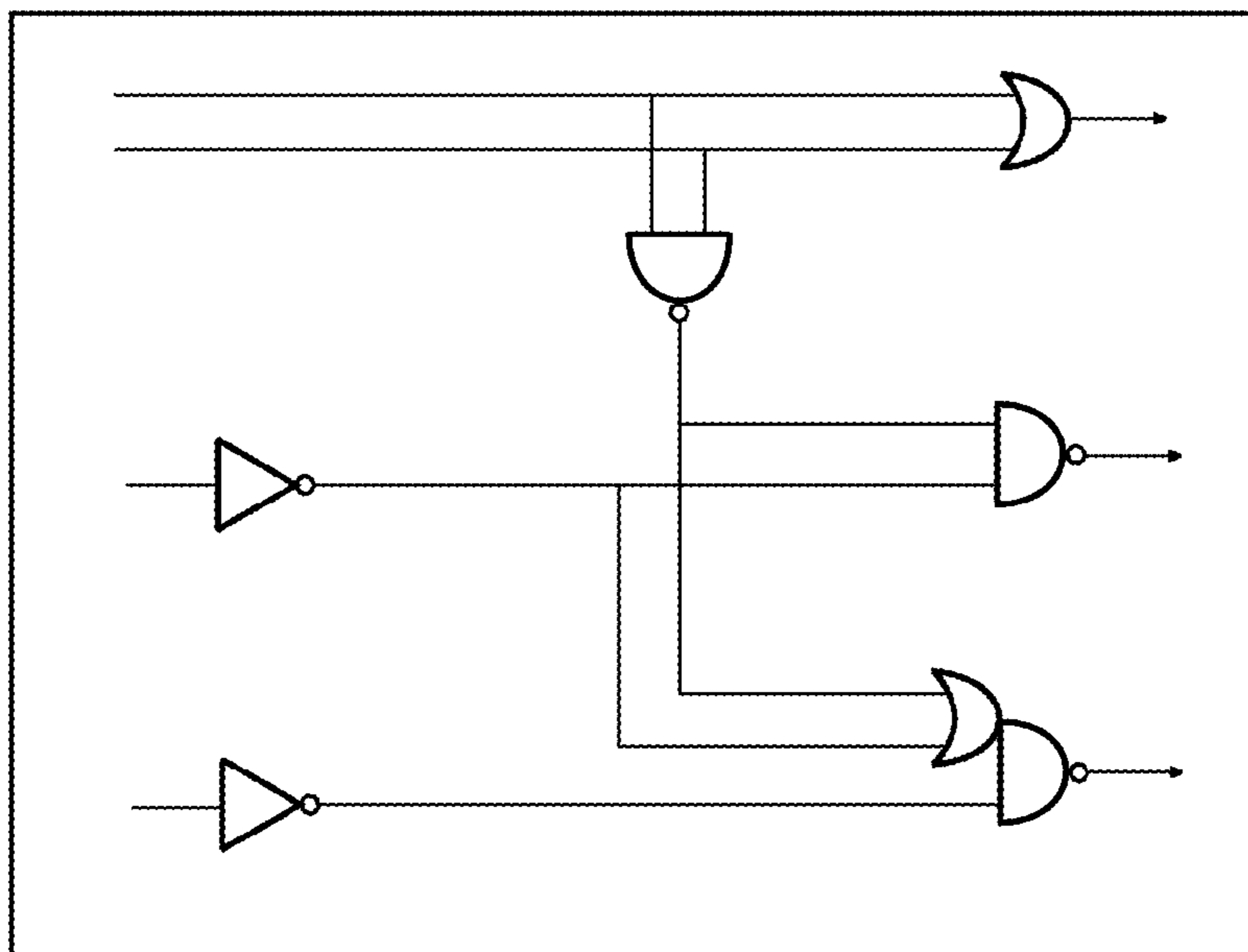
Carry Compression
