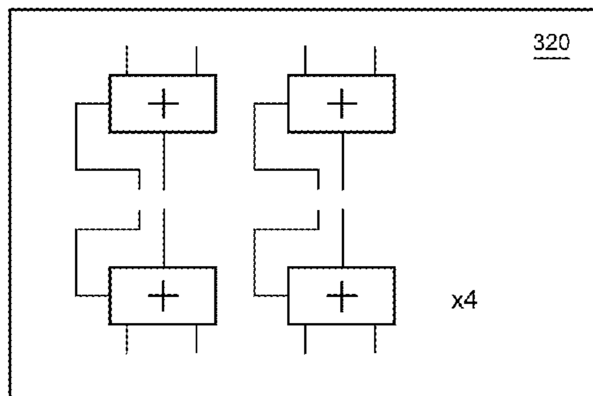
r-Edge Sliding
