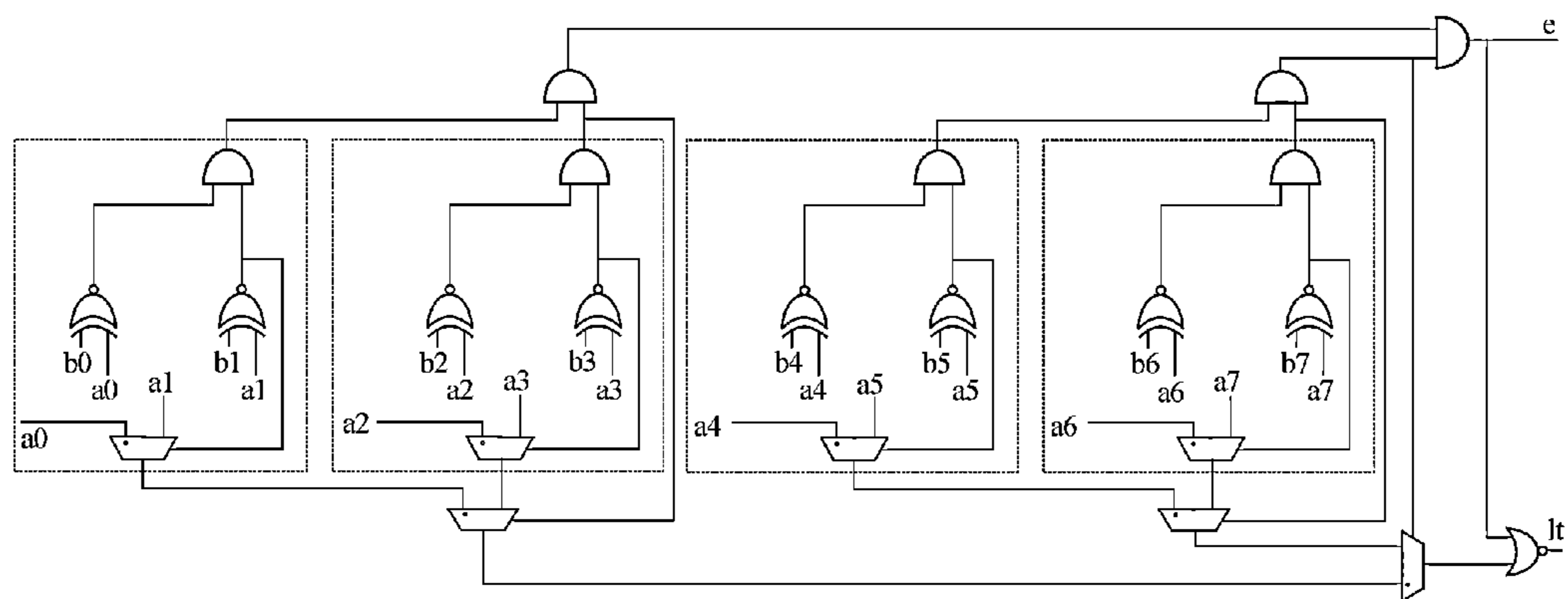
8-Bit Less Than
