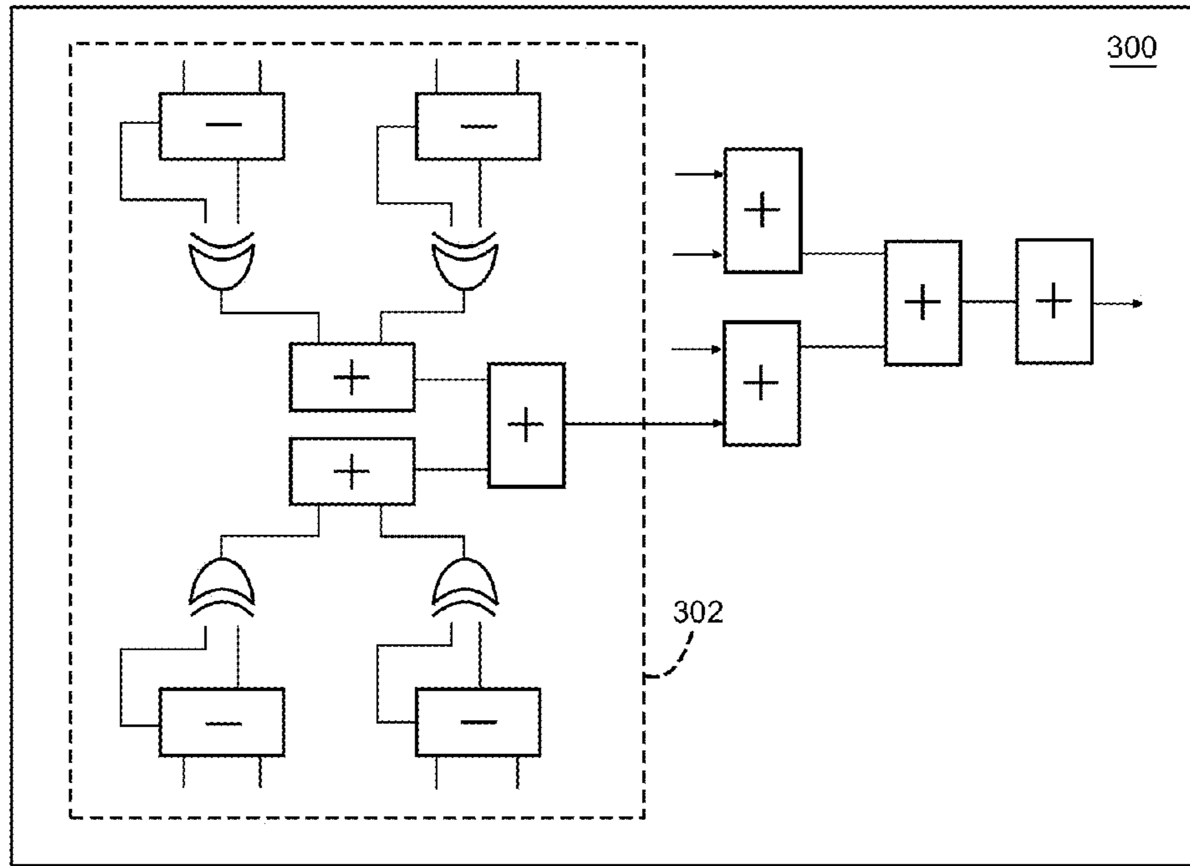
i-SAD Exact
