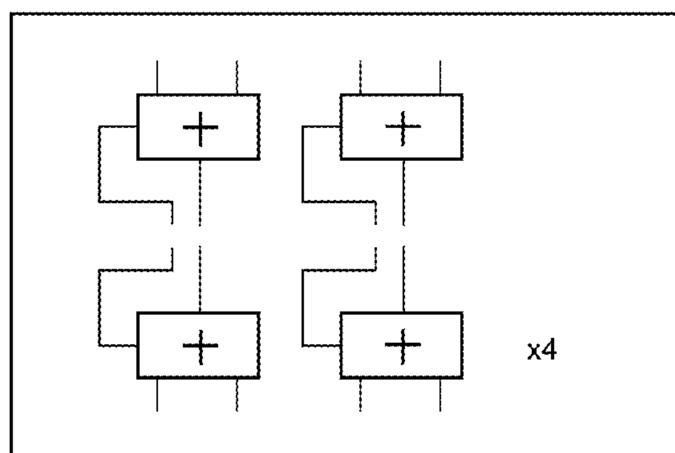
r-Edge Exact
