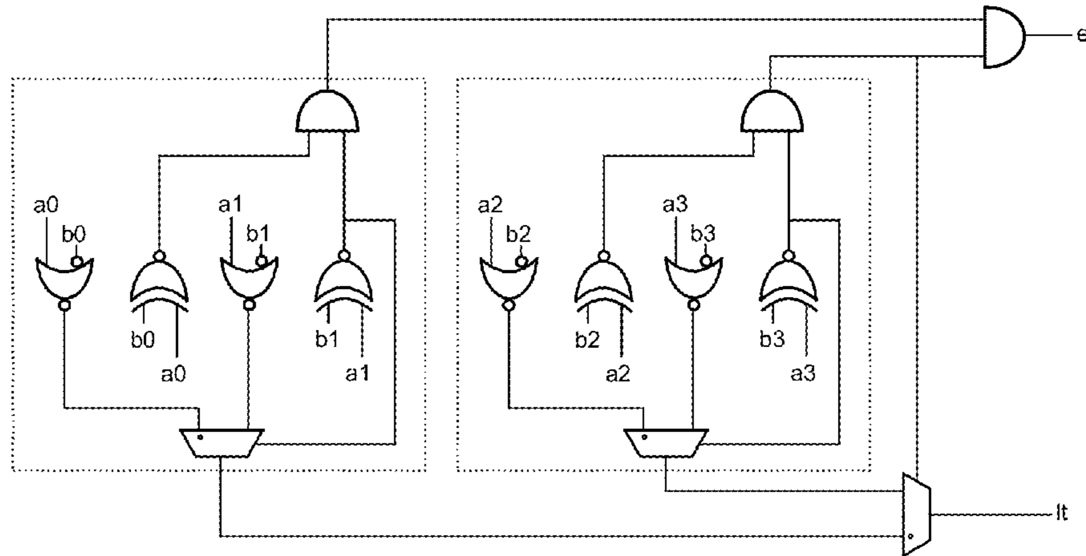
4-Bit Less Than
