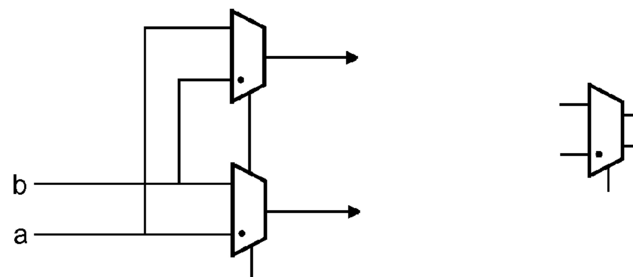
Two-Way Selector
