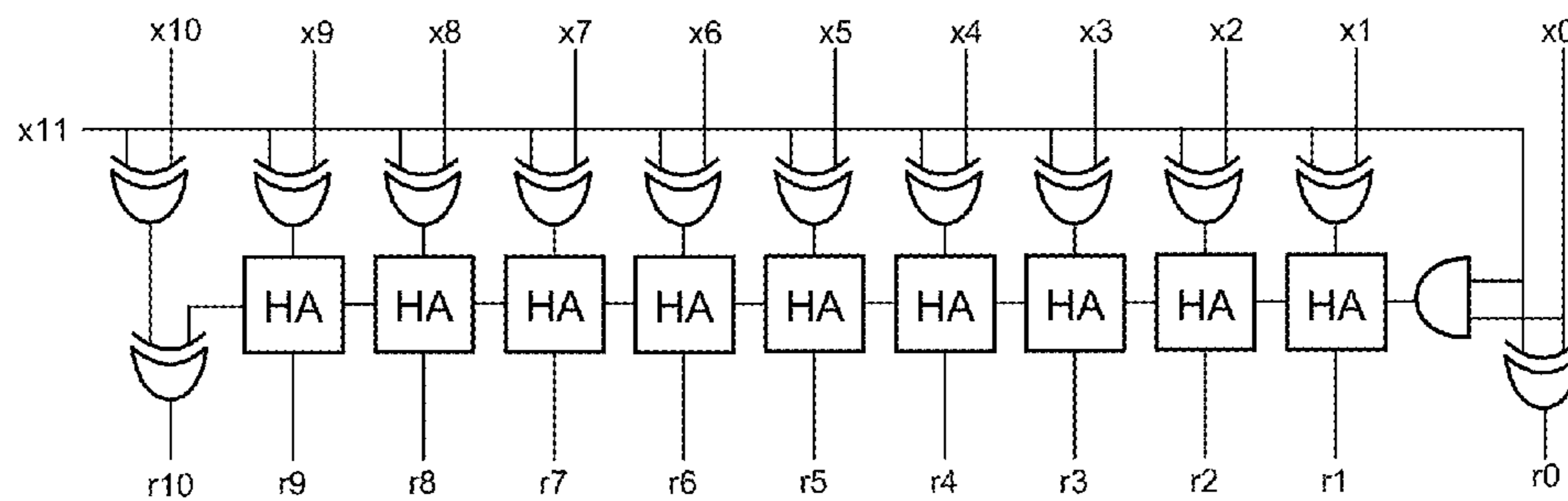
12-Bit Modulus
