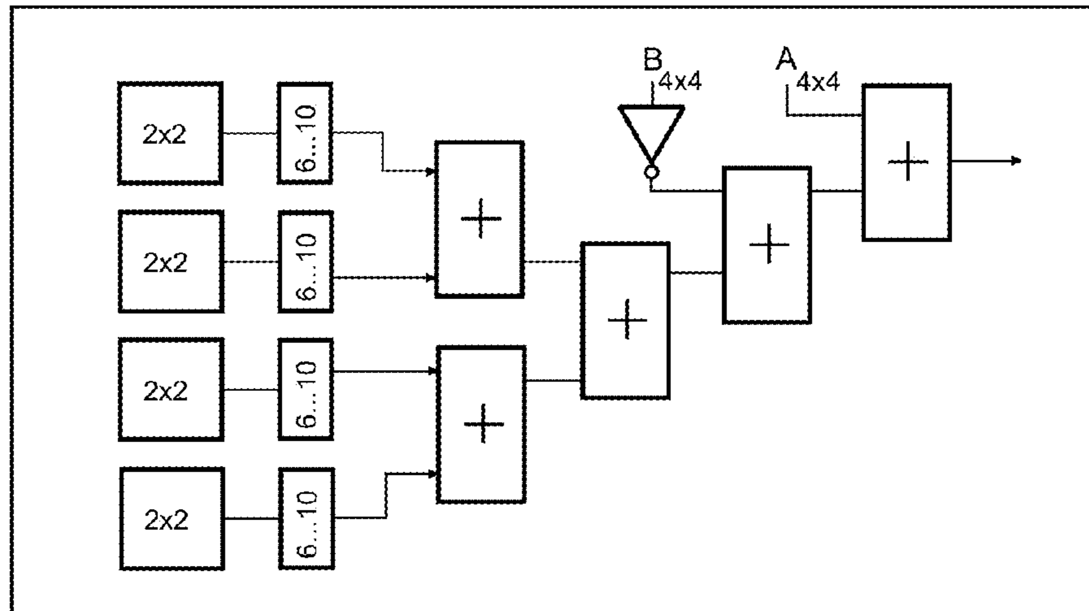
4x4 SAD Using Sliding Arithmetic
