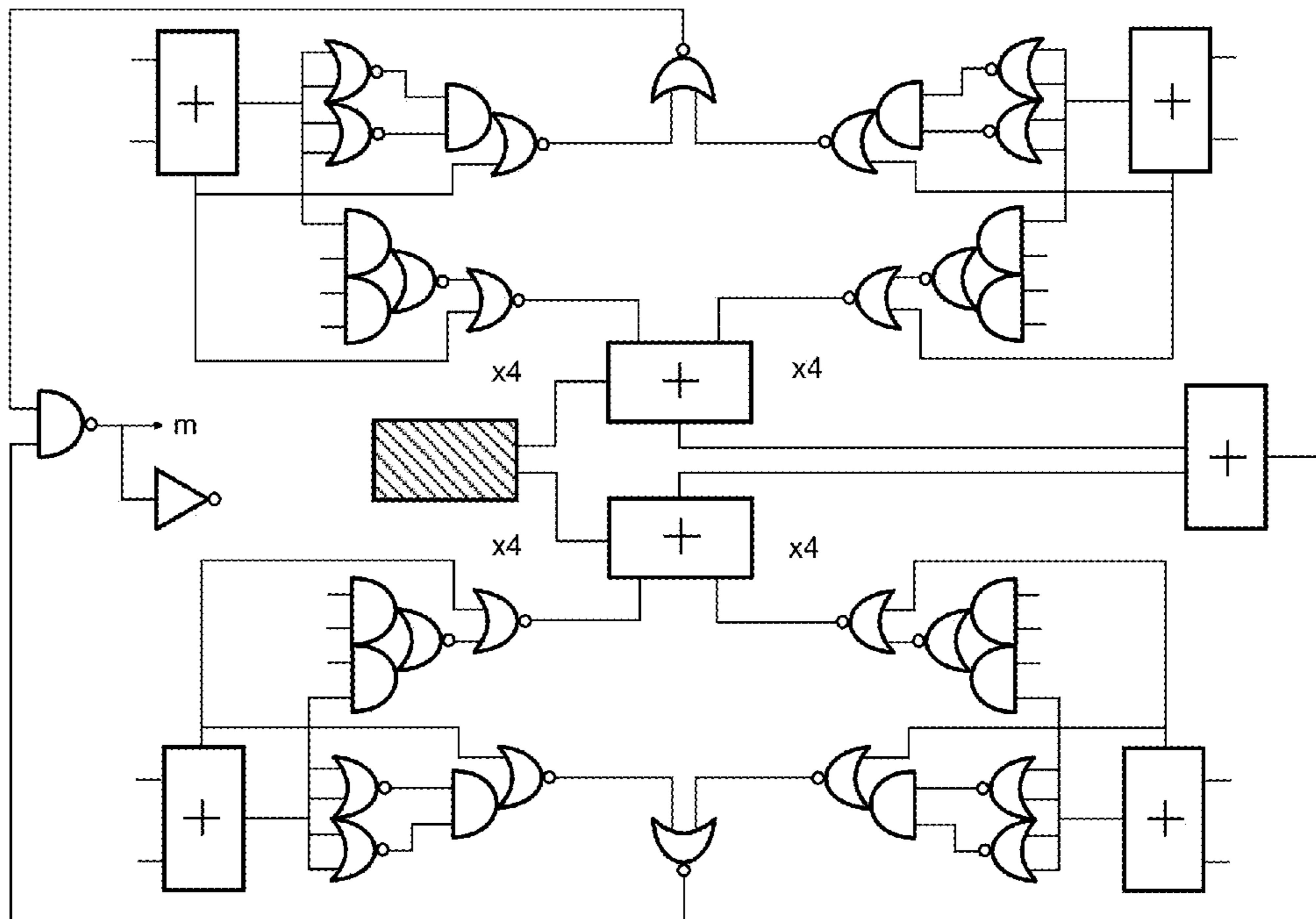
Integer 2x2 SAD Using Sliding Arithmetic
