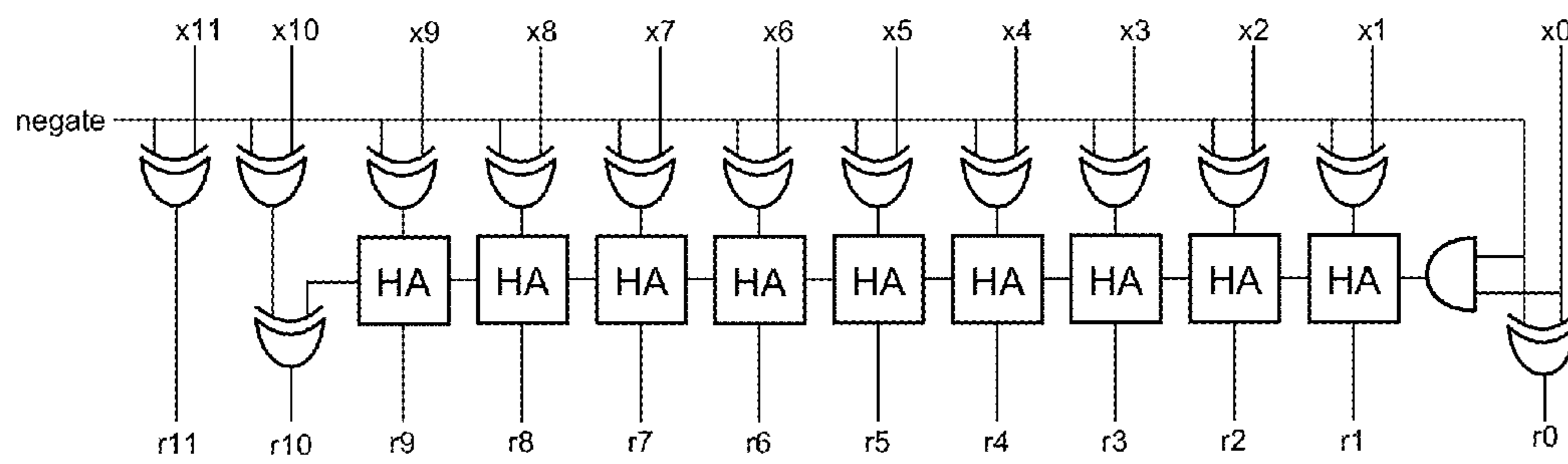
12-Bit Multiply By 1 or -1
