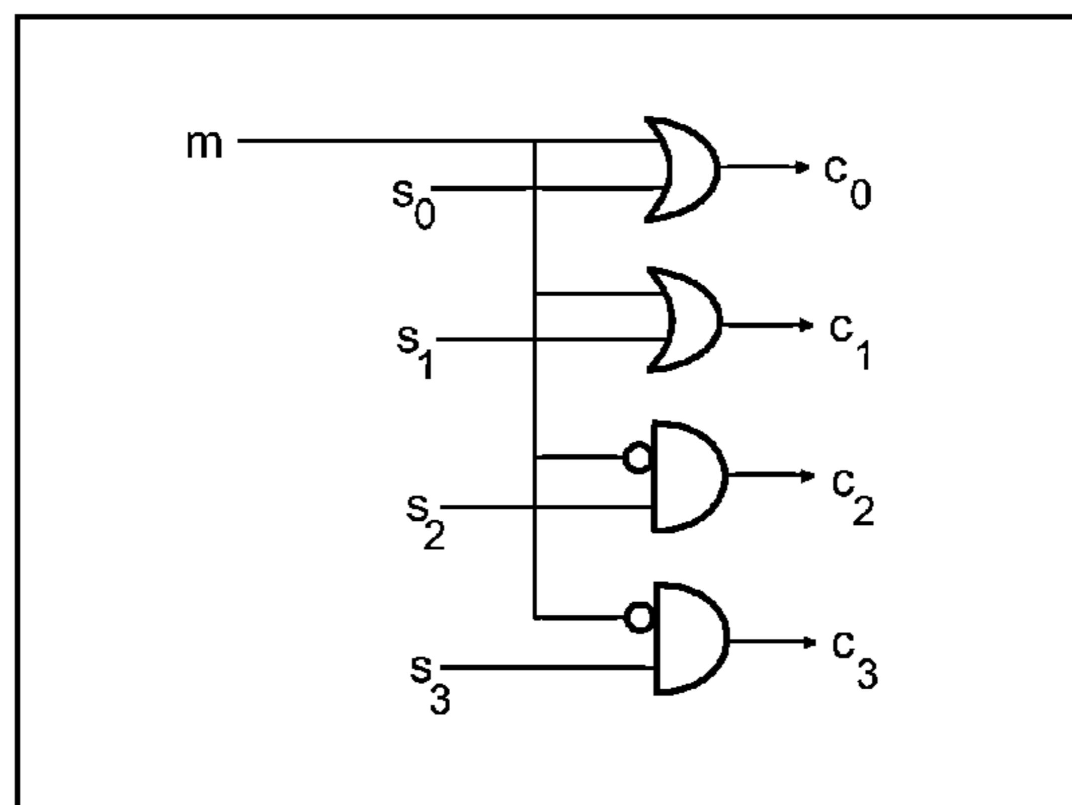
Adapting Carry-In
