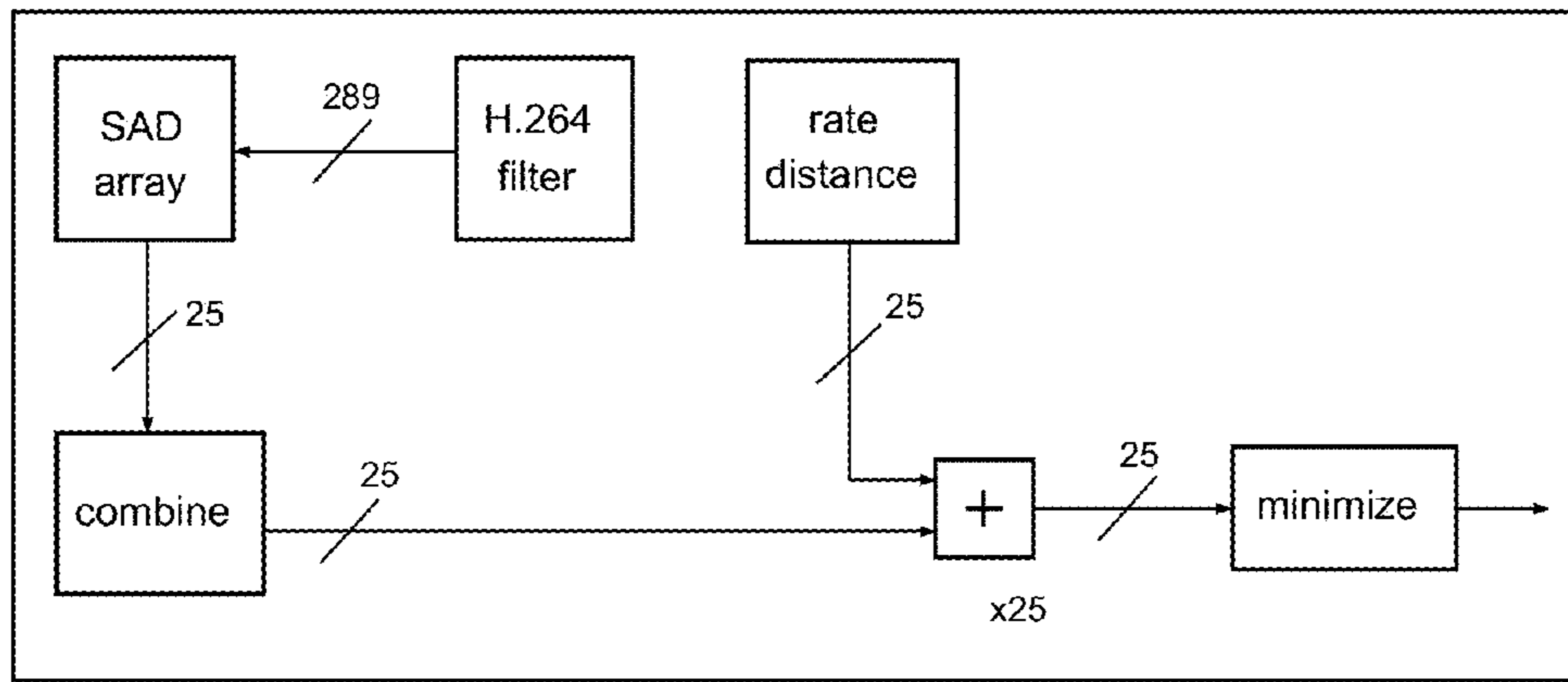
Basic Architecture for H.264 Final Search
