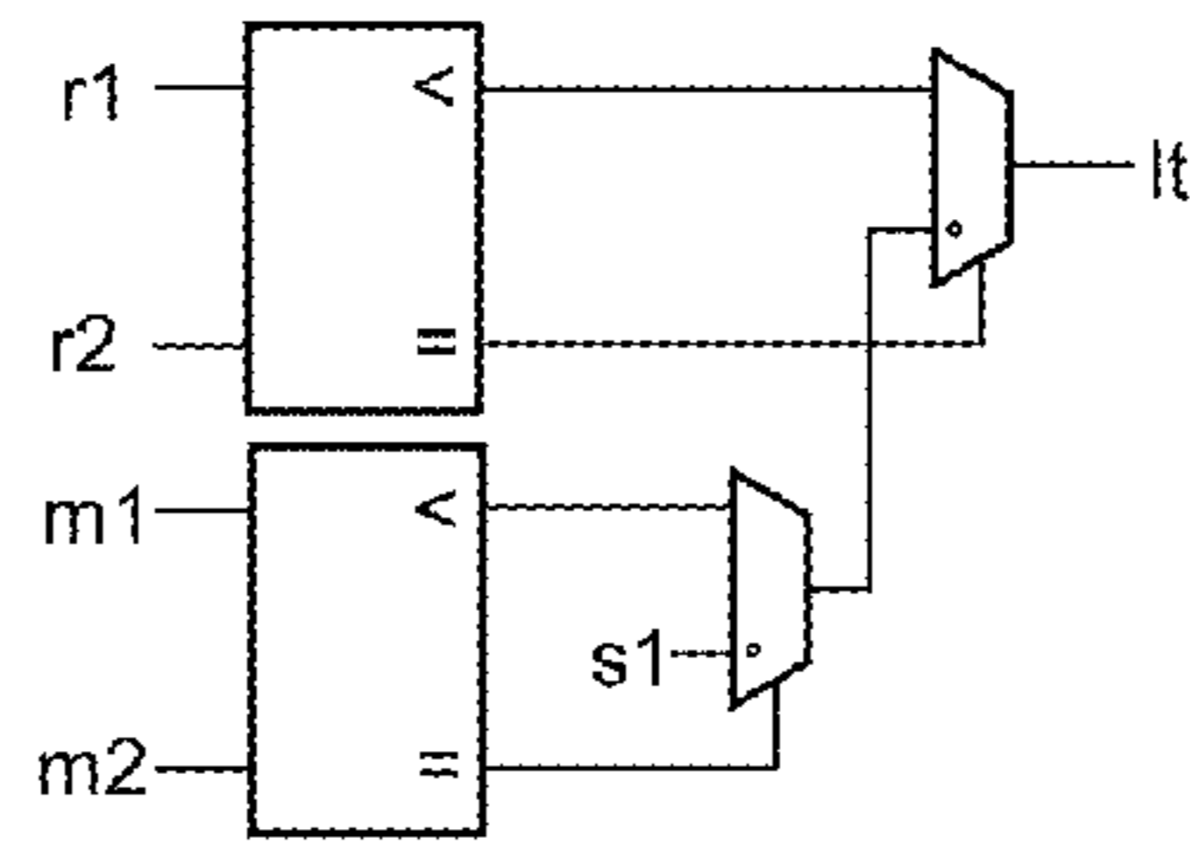
Local Minima Comparison Logic
