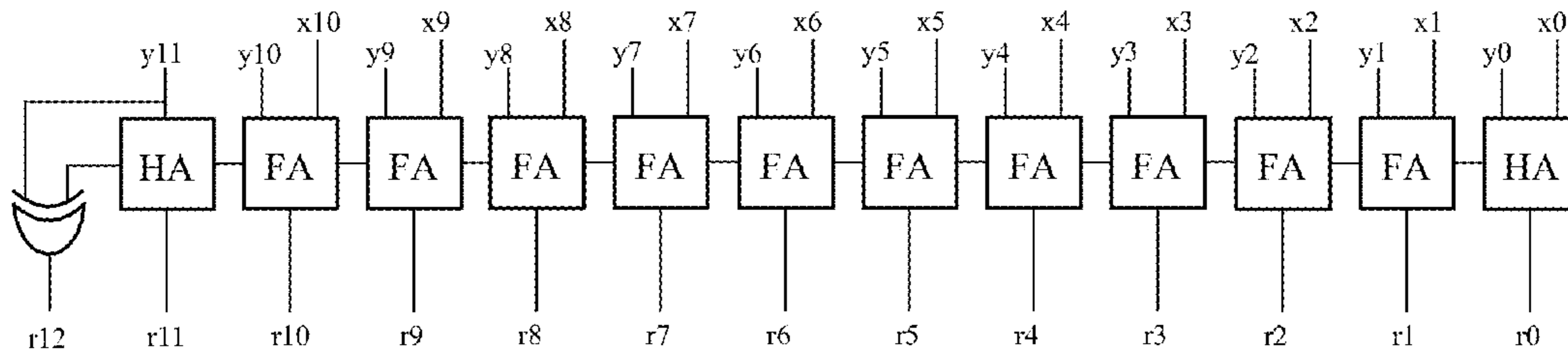
Unsigned/Signed Add
