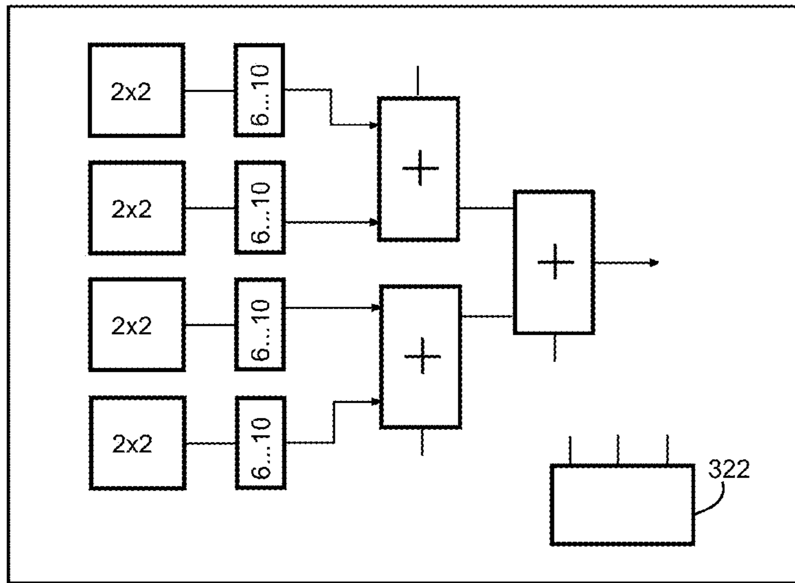
4x4 r-SAD Using Sliding Arithmetic
