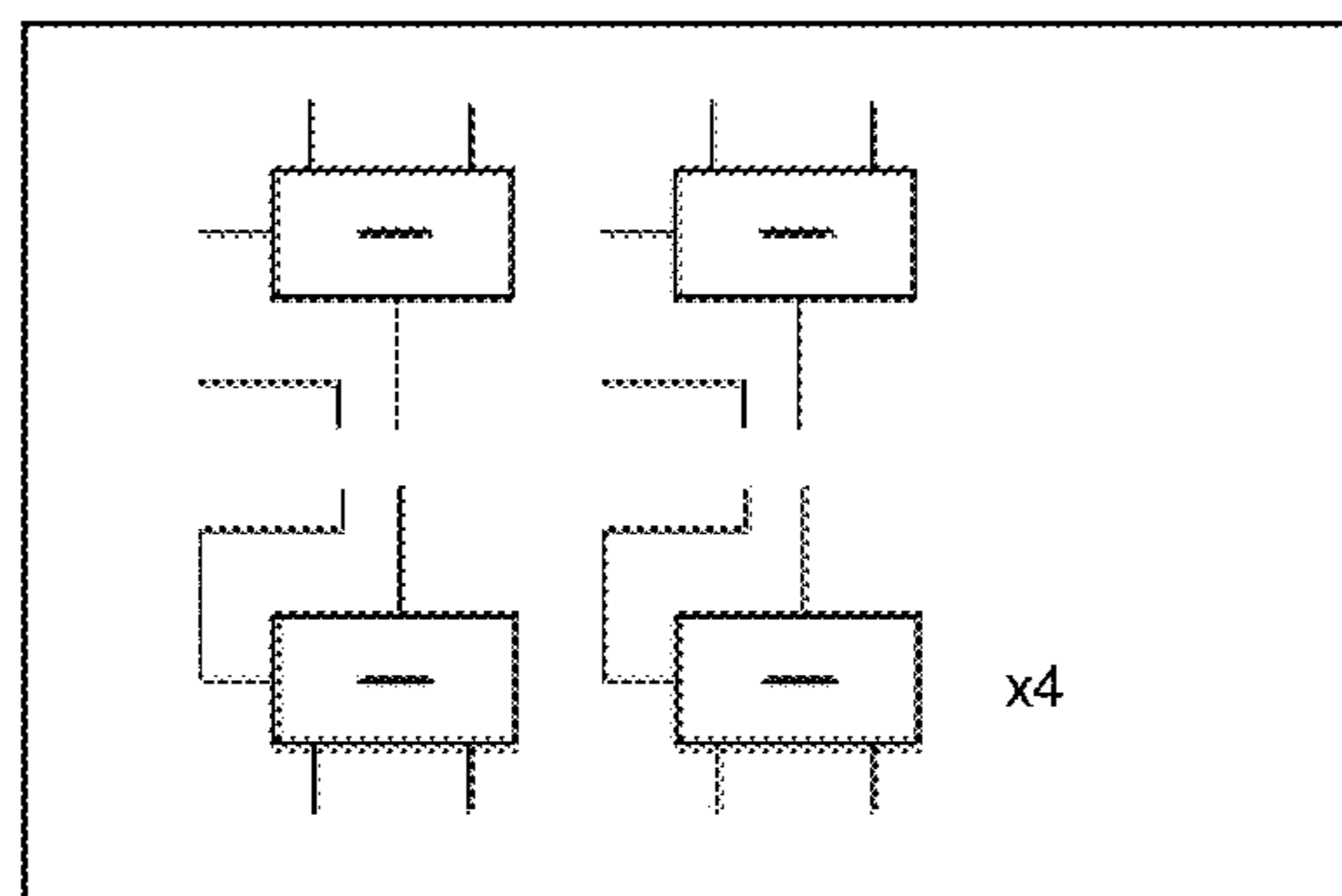
i-Edge Sliding
