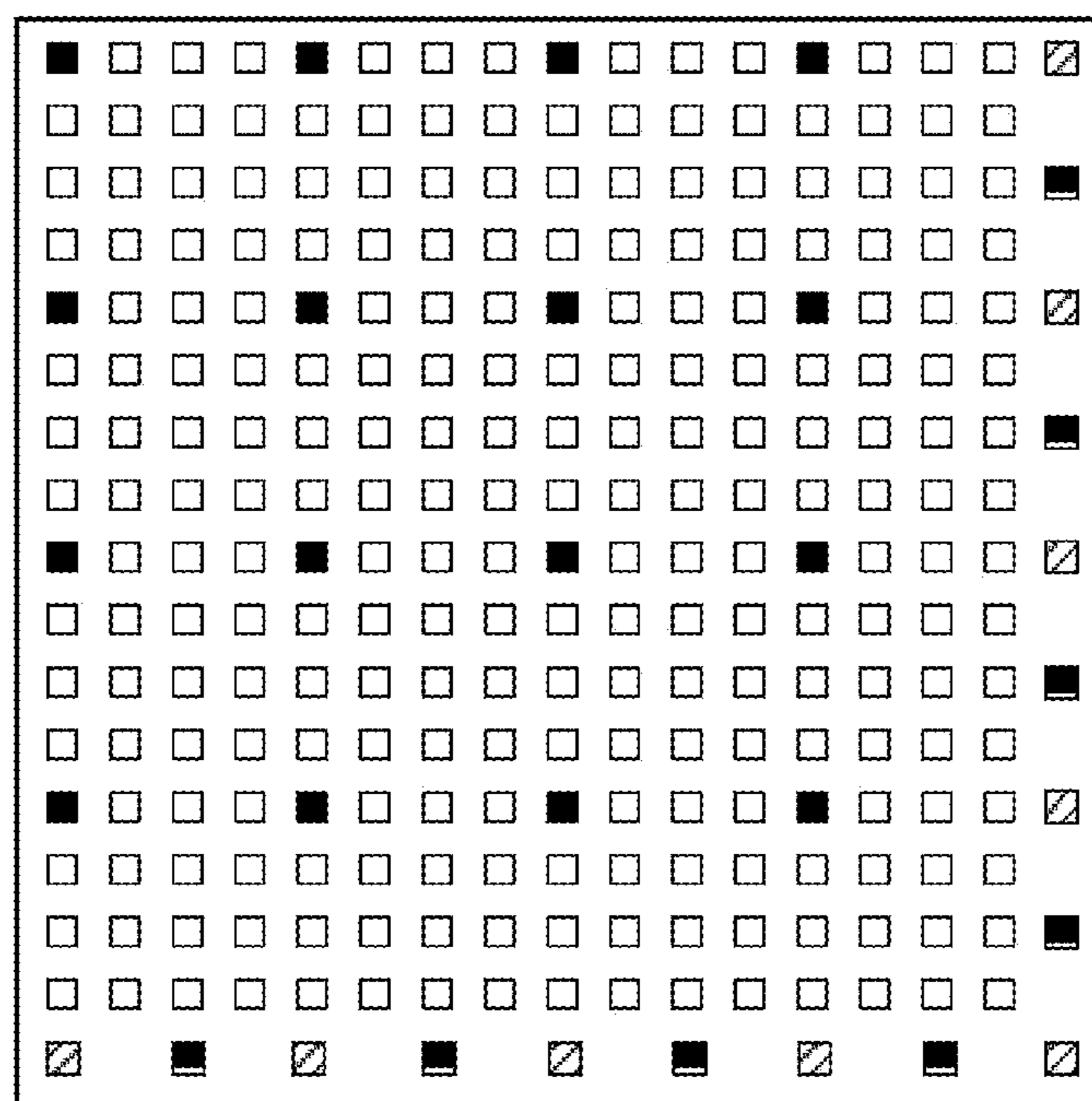
Fractional Array
