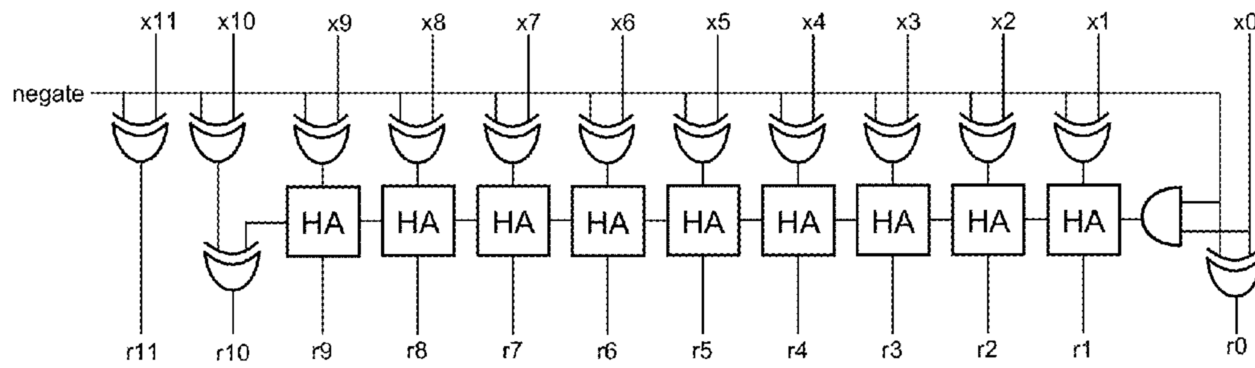
12-Bit Multiply By 1 or -1
