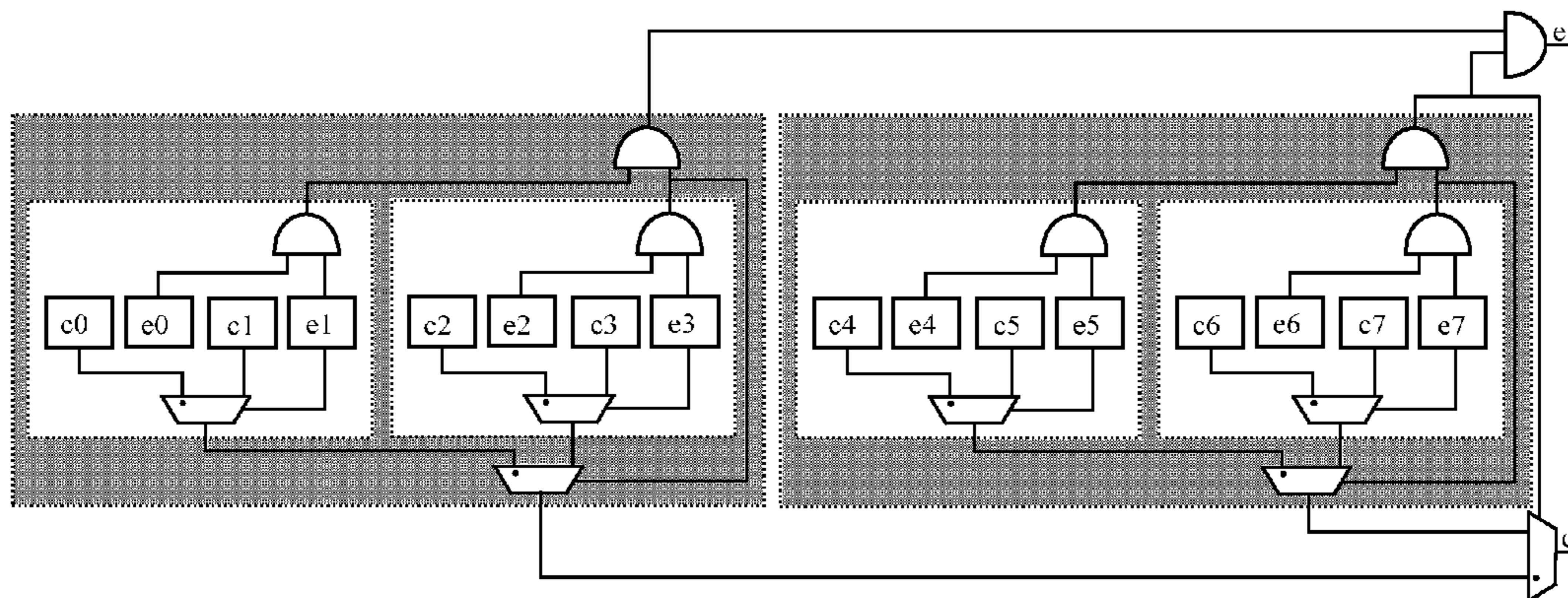
8-Bit Hierarchical Comparison
