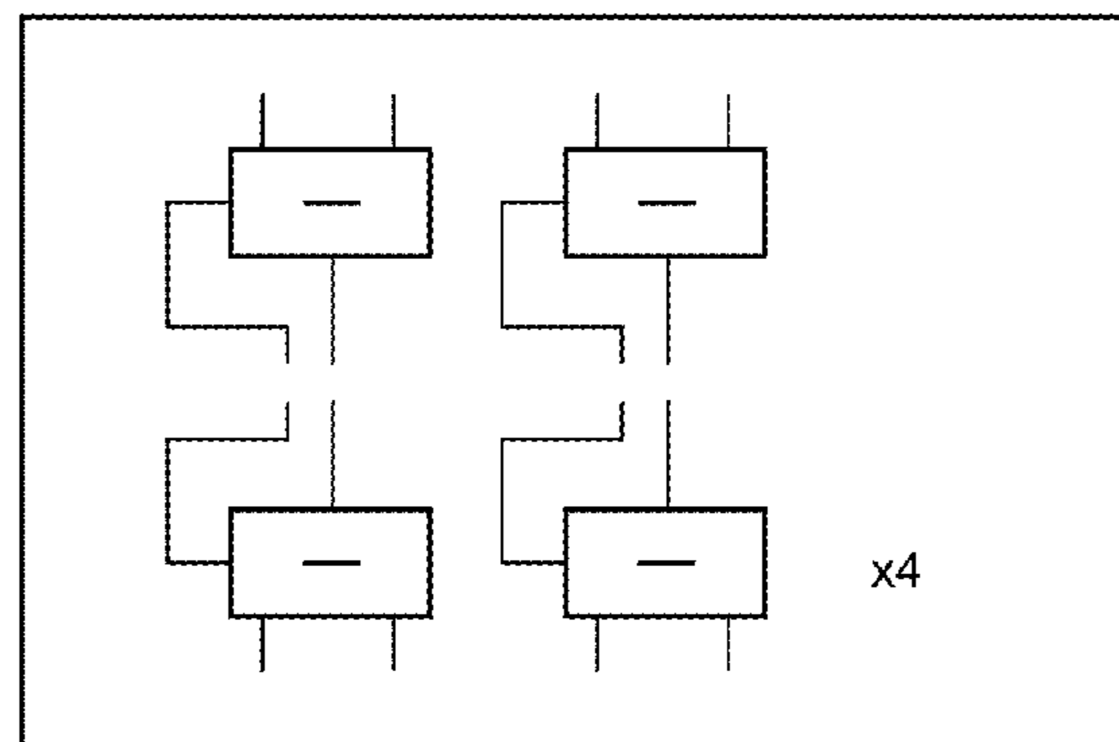
i-Edge Exact
