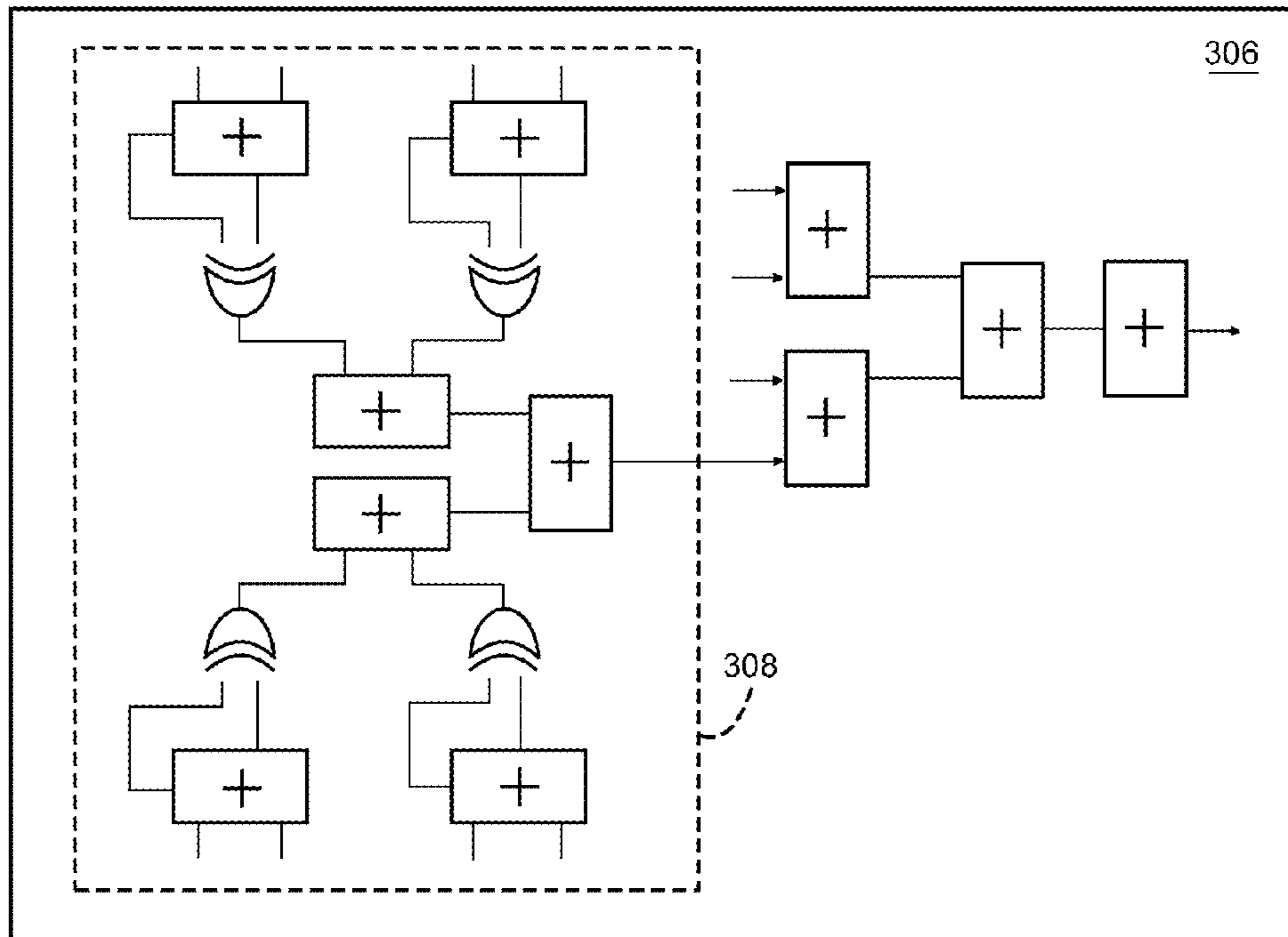
r-SAD Exact
