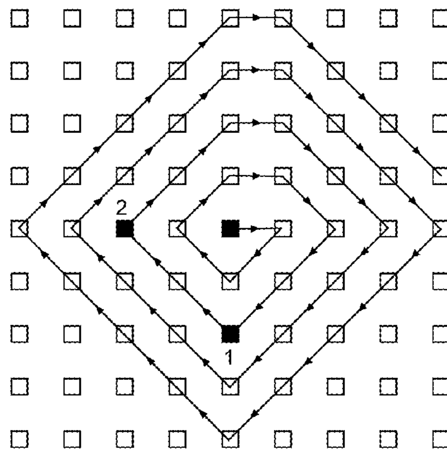
Clockwise Spiral-Search
