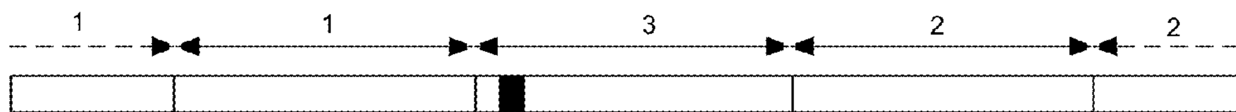
Scan-Line Strides
