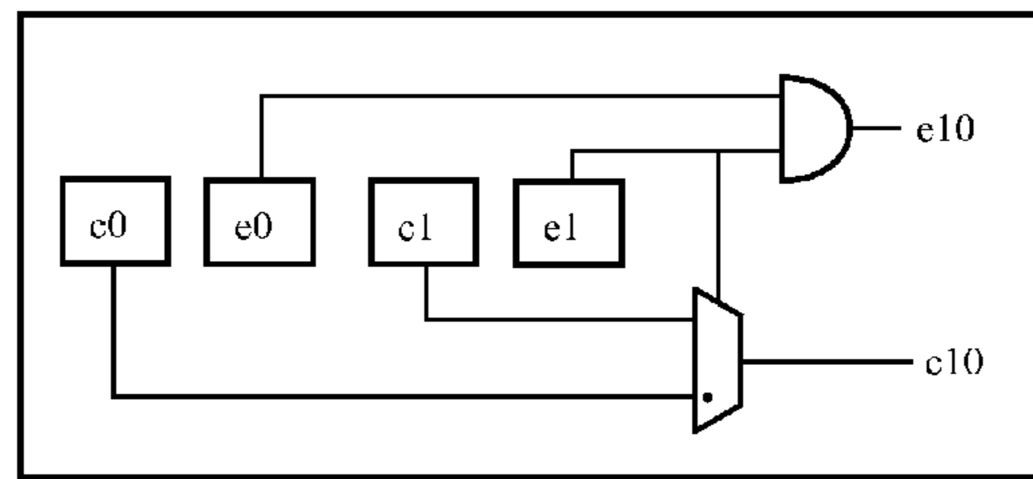
Basic Comparison Cell
