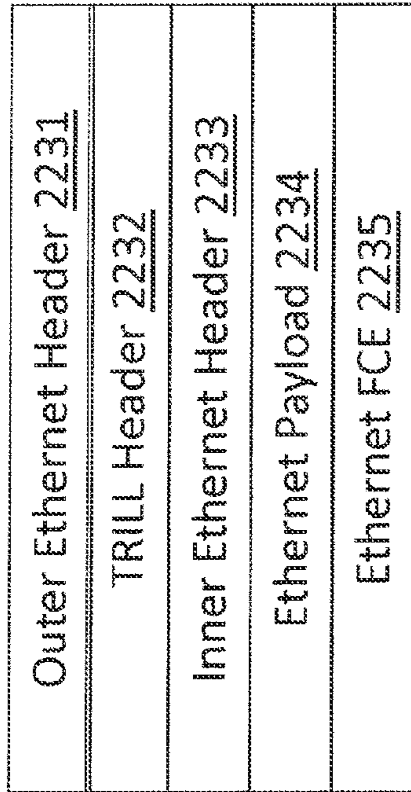
An Ethernet Encapsulated TRILL Frame 2230
