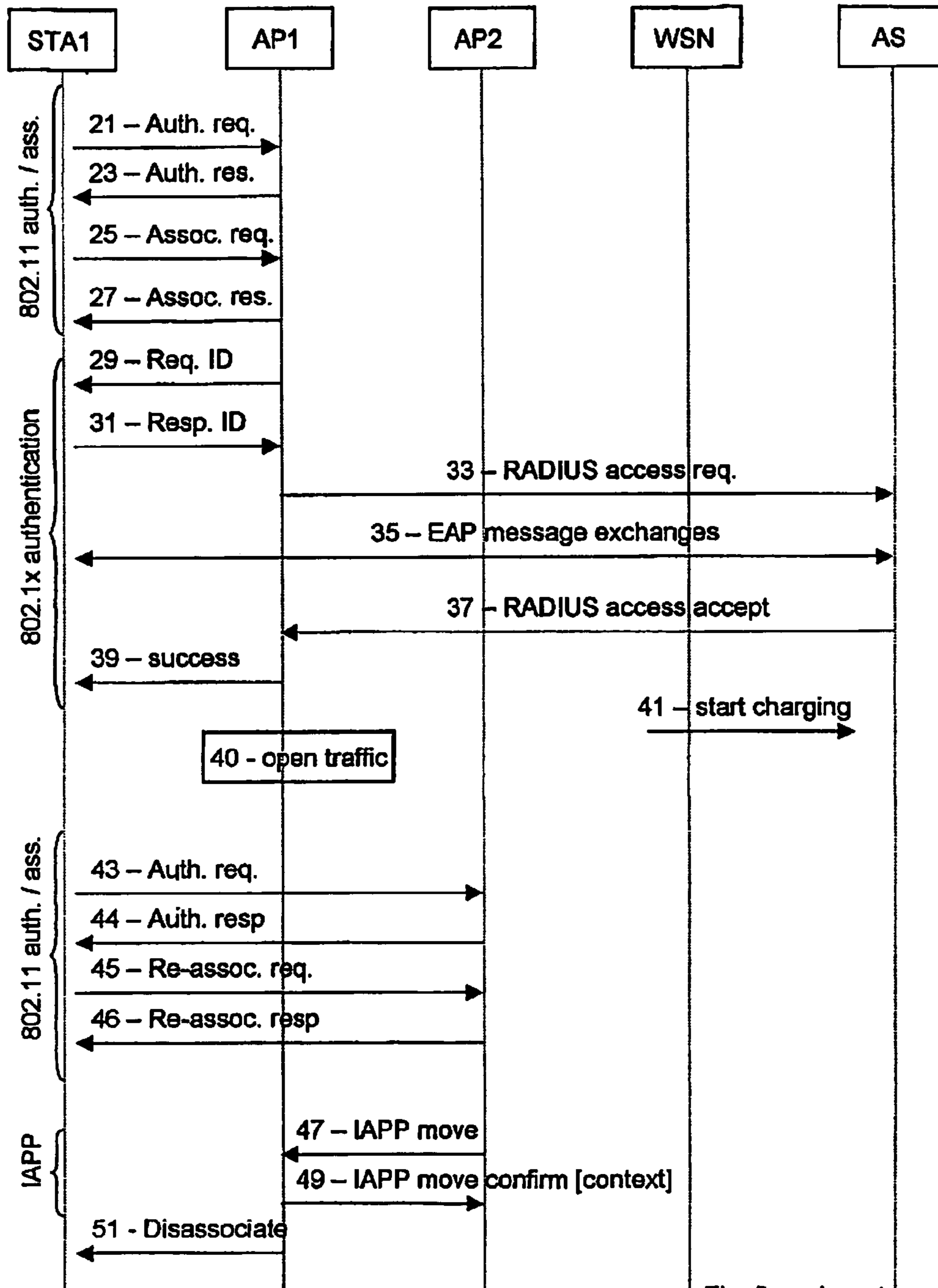
Fig. 5 - prior art
