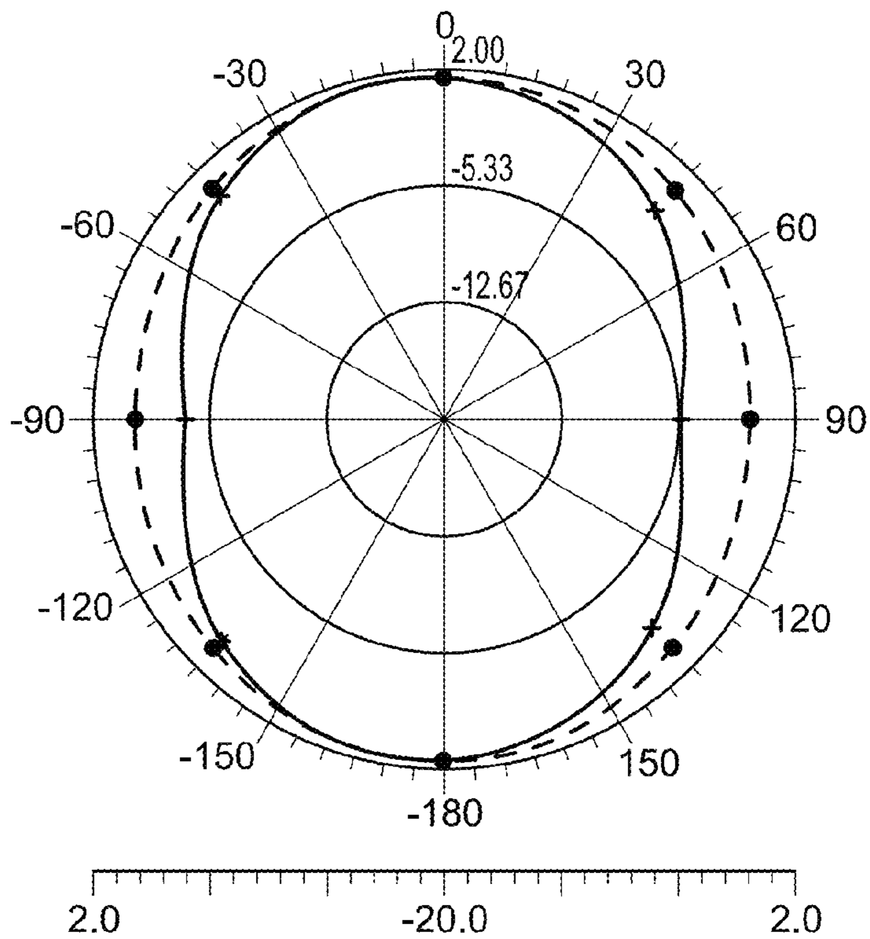
Antenna Patterns @ 2.45 GHz Max Gain = 2 dBi
