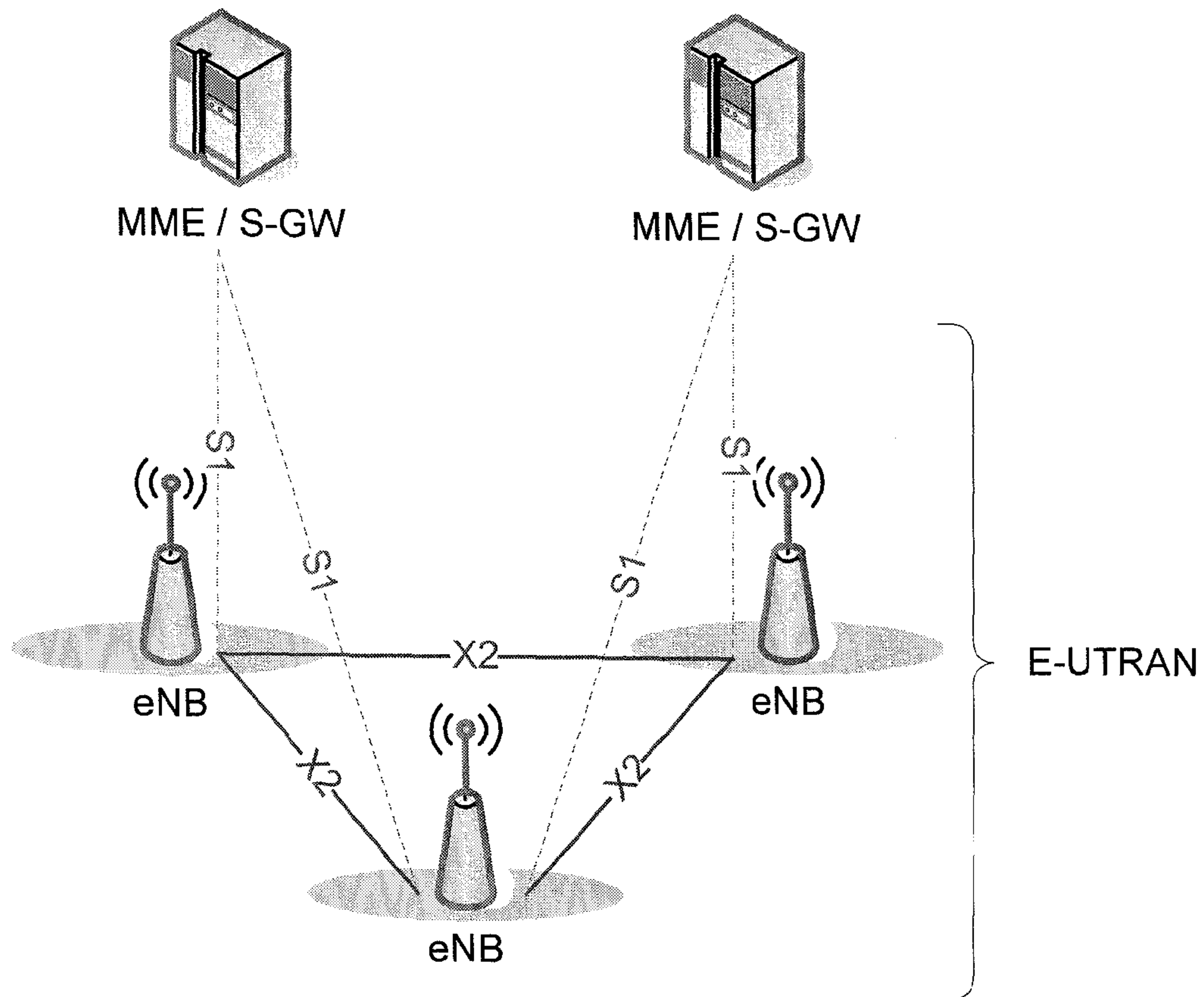
Figure 1 (Prior Art)
