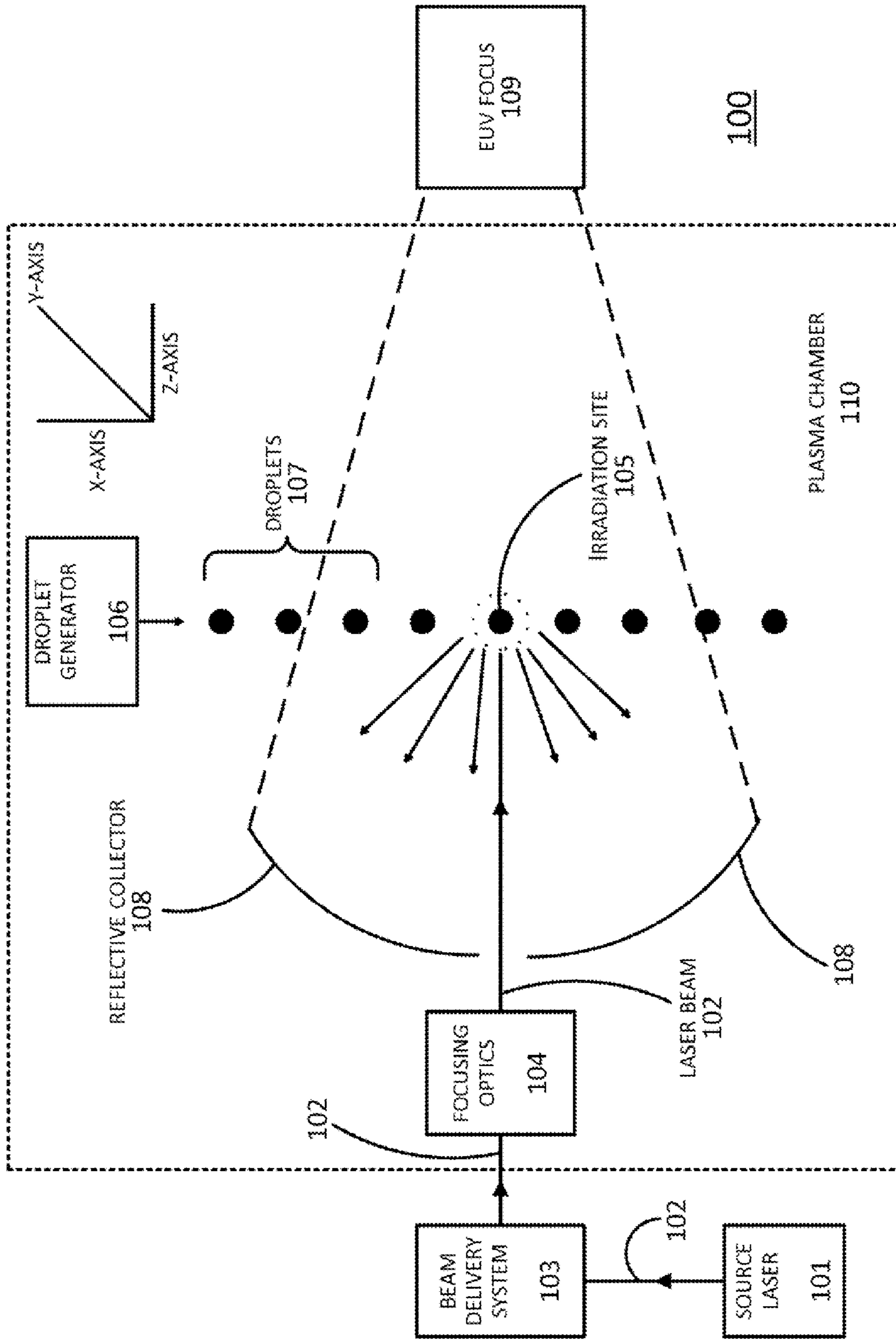
FIGURE 1 (Prior art)
