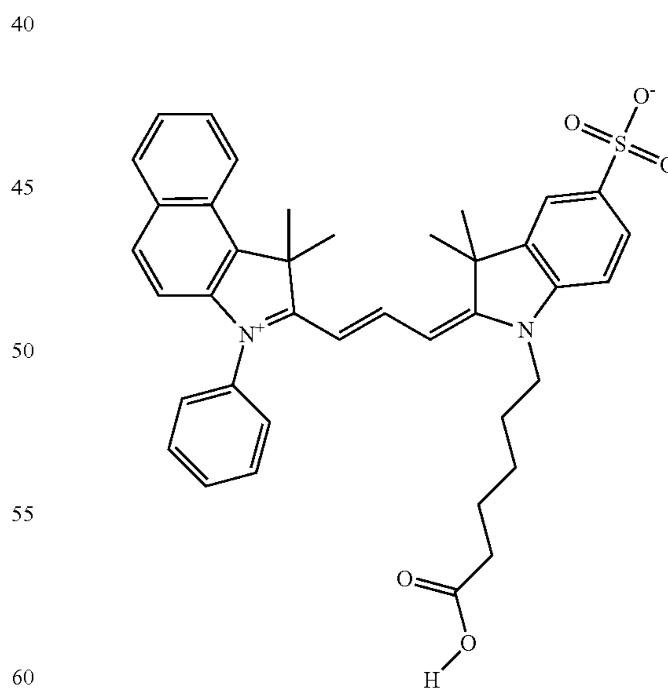
Indocarbocyanine I-5 (8)
