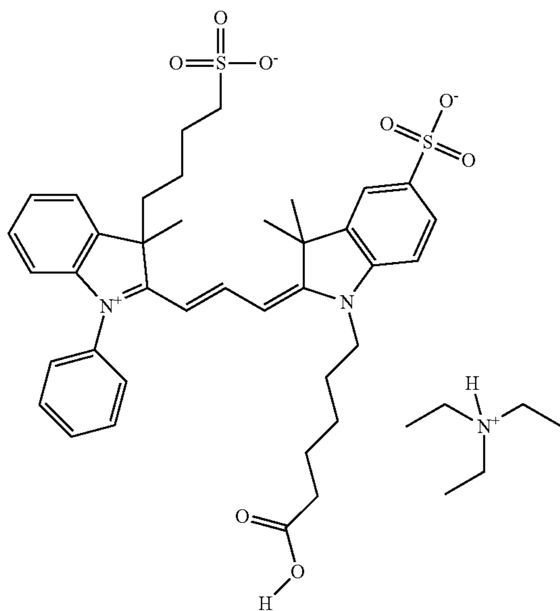
Indocarbocyanine I-4 (7)
