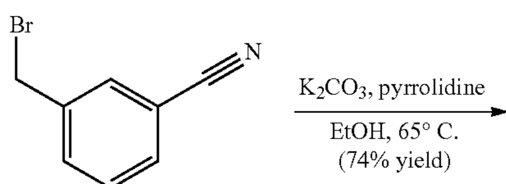
Scheme 3
