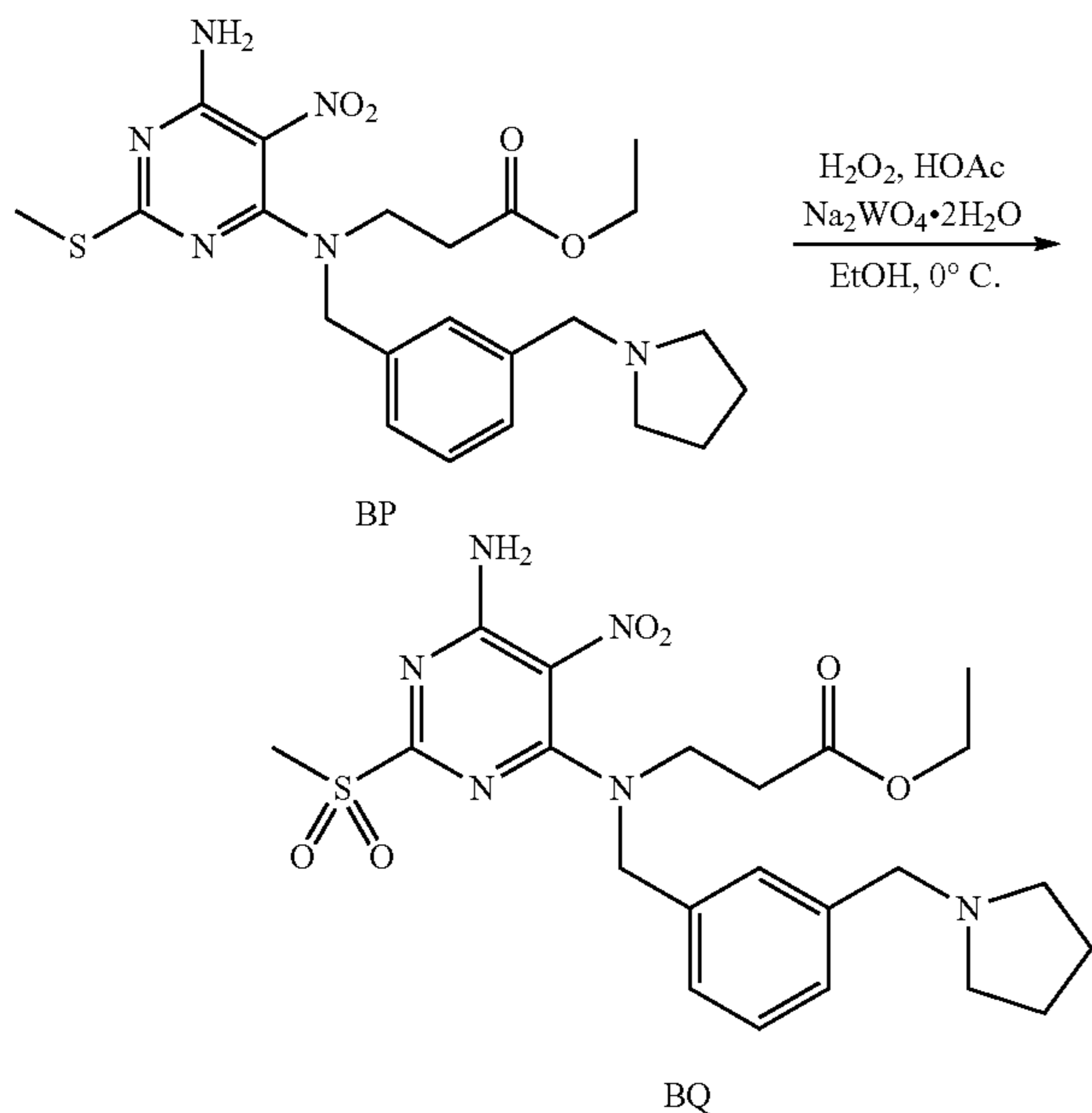
Scheme 36
