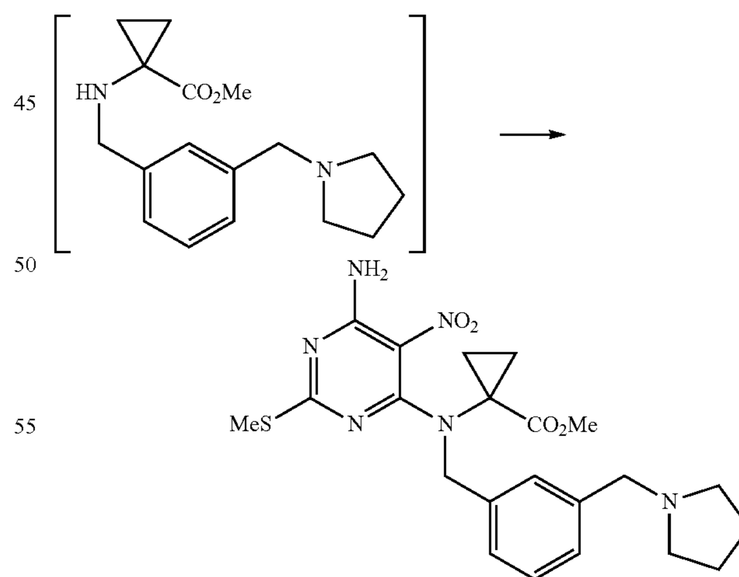
Scheme 19
