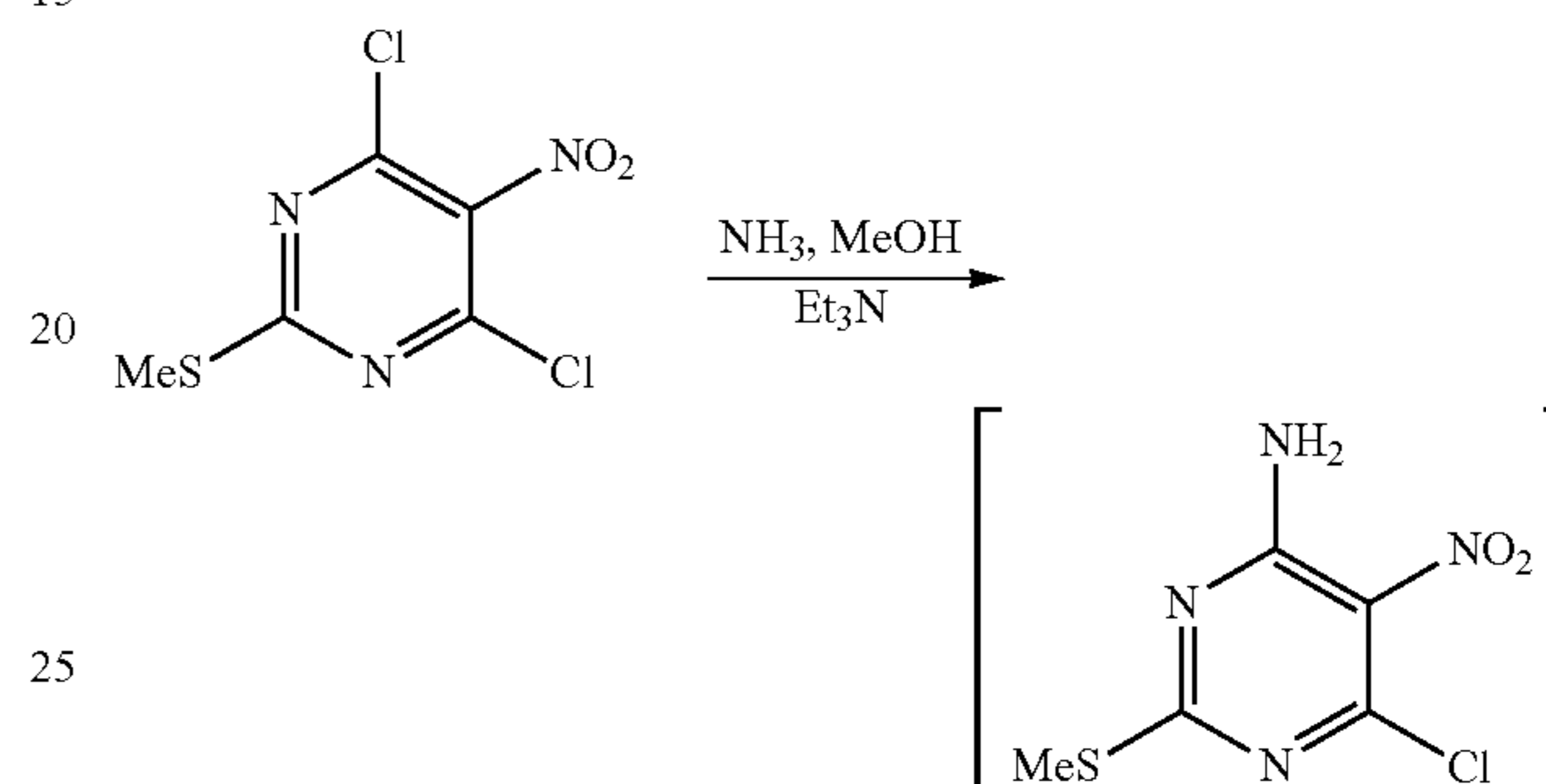
Scheme 18
