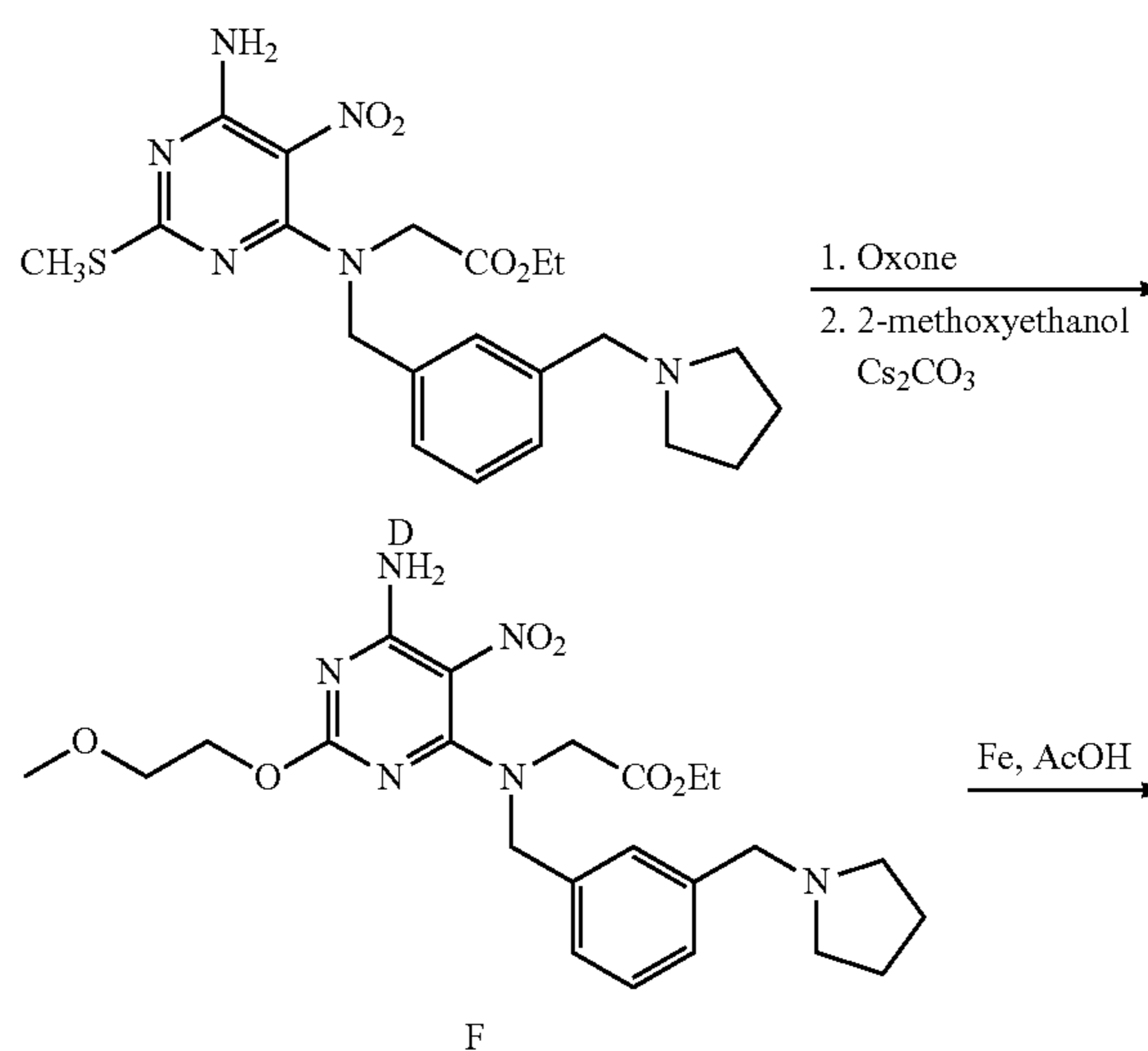
Scheme 2
