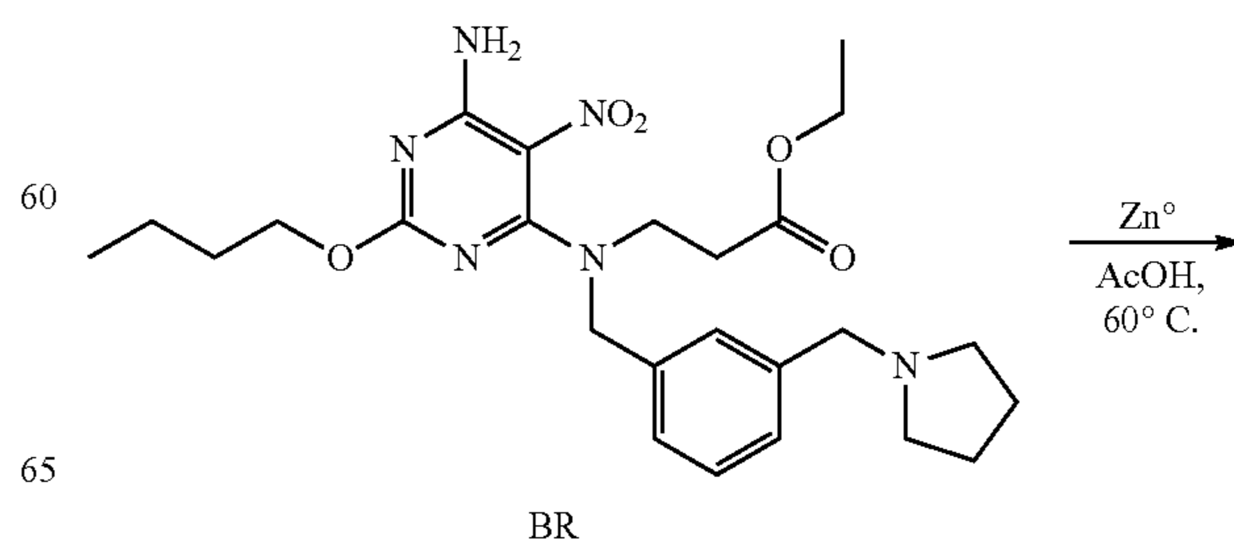
Scheme 38:
