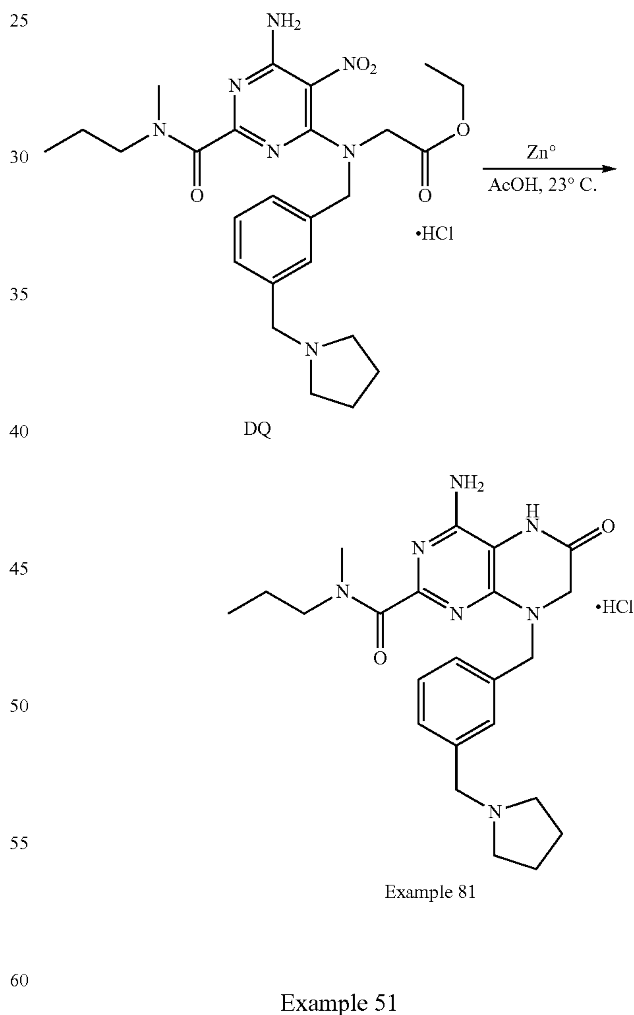
Scheme 84:
