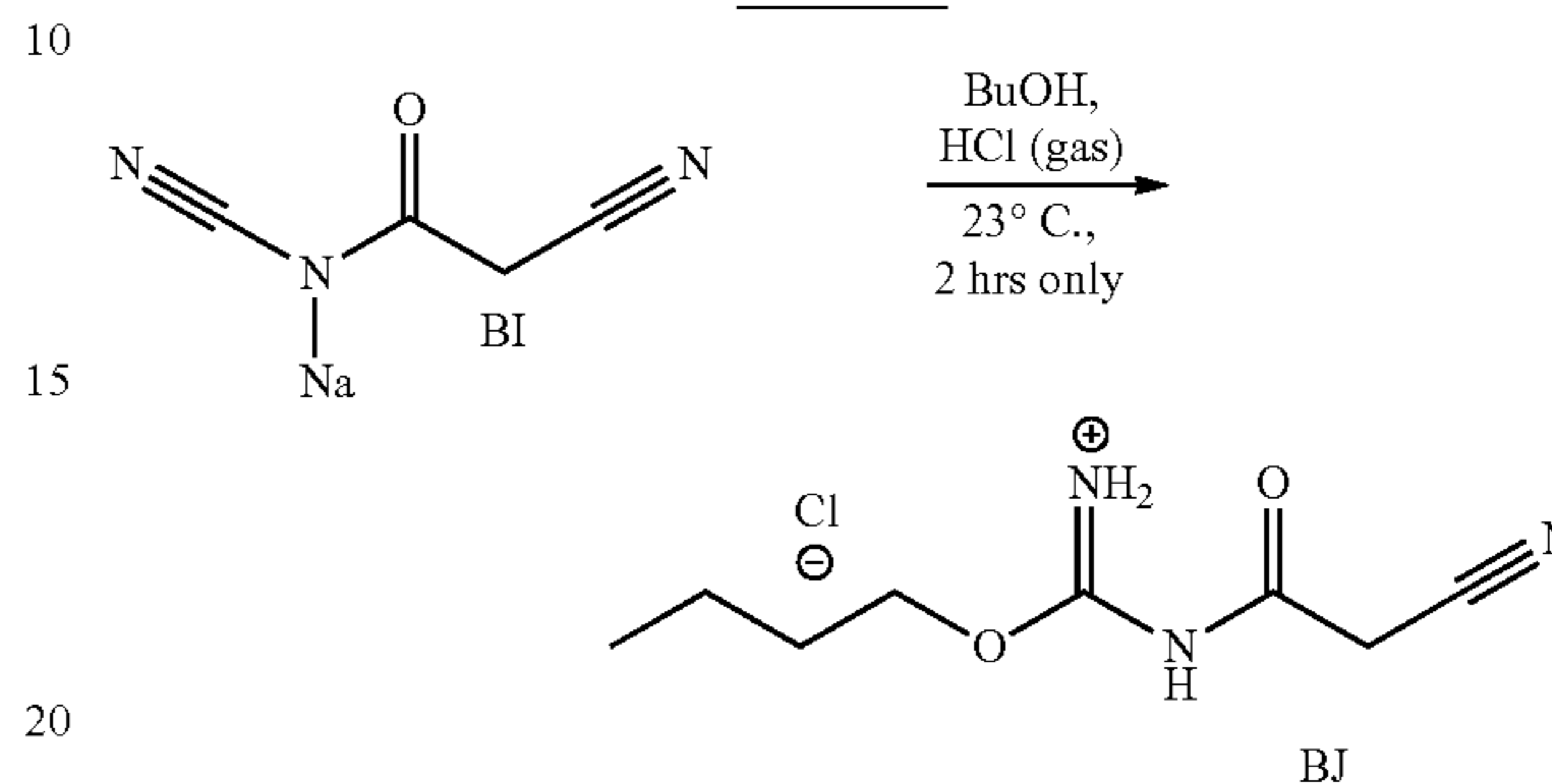
Scheme 28
