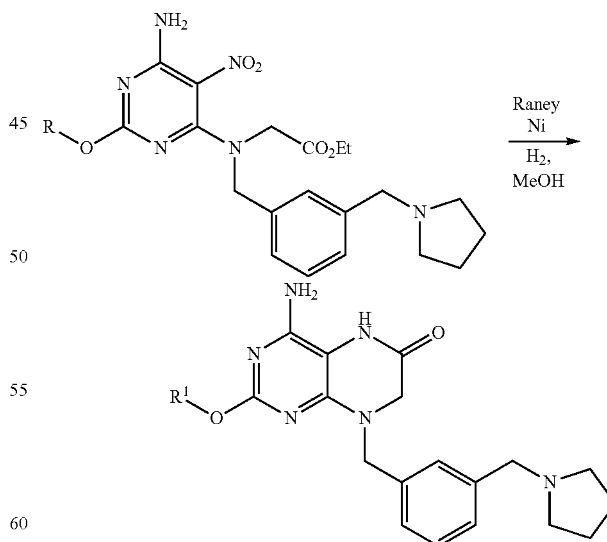
Scheme 15
