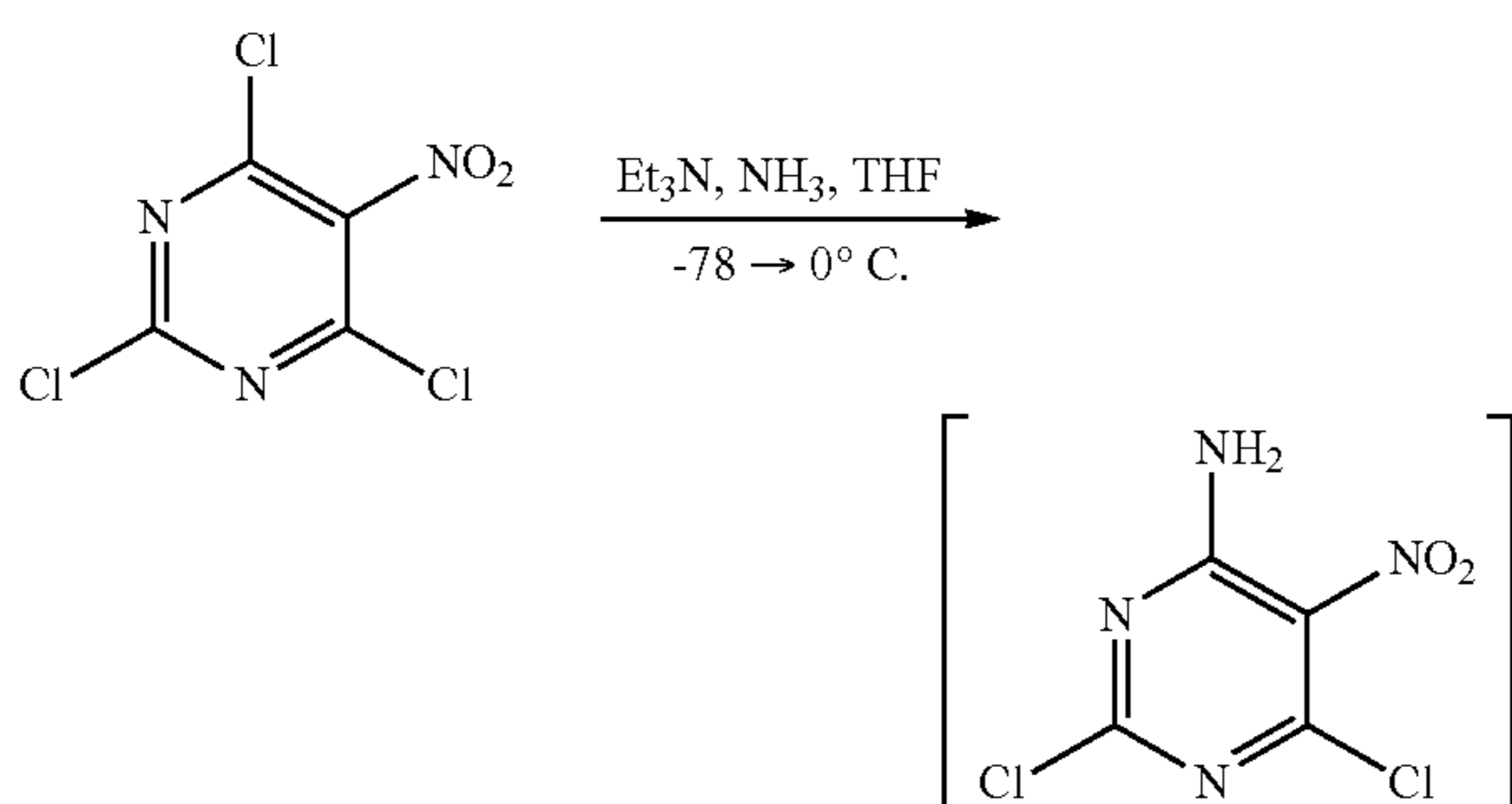
Scheme 39
