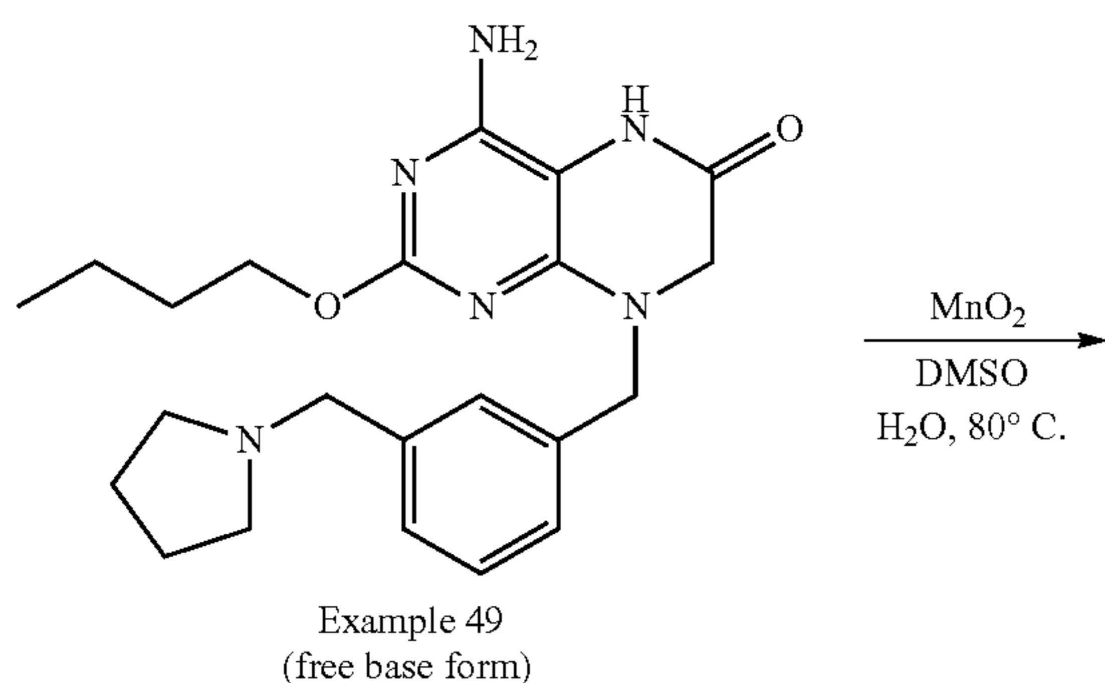
Scheme 87
