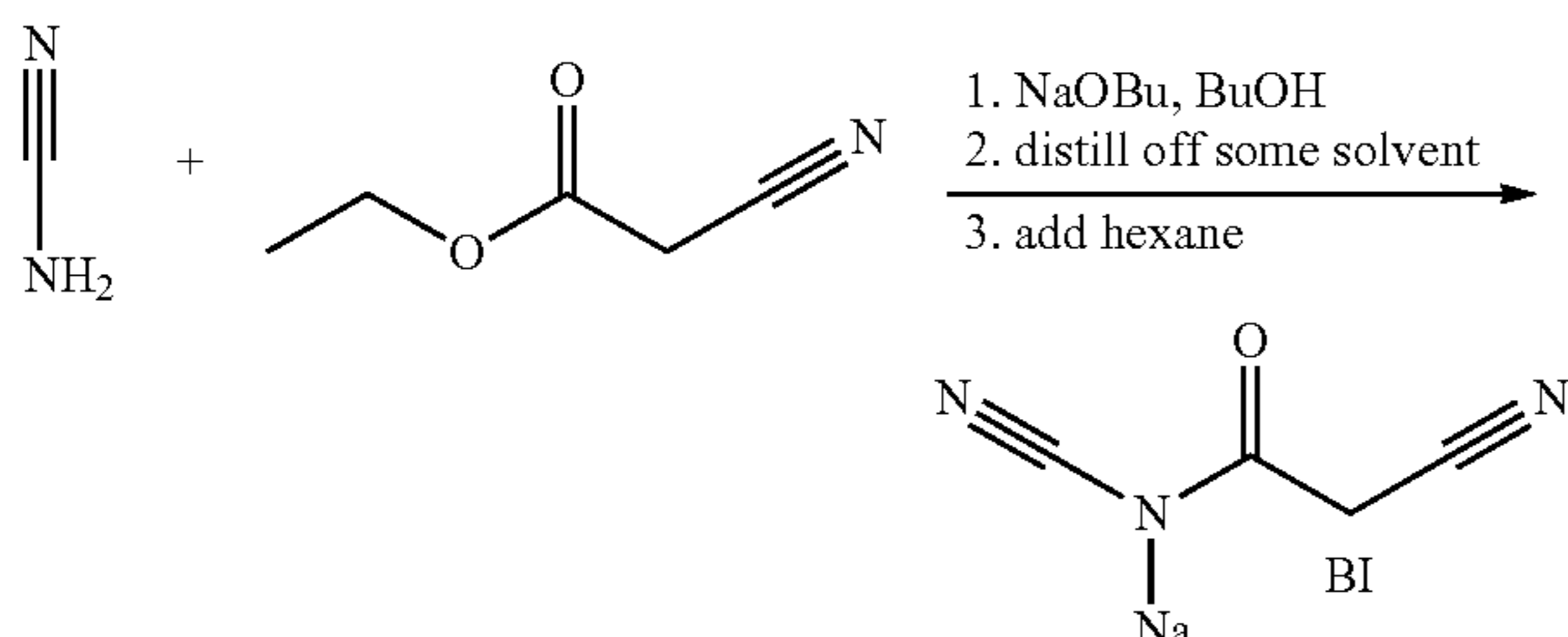
Scheme 27
