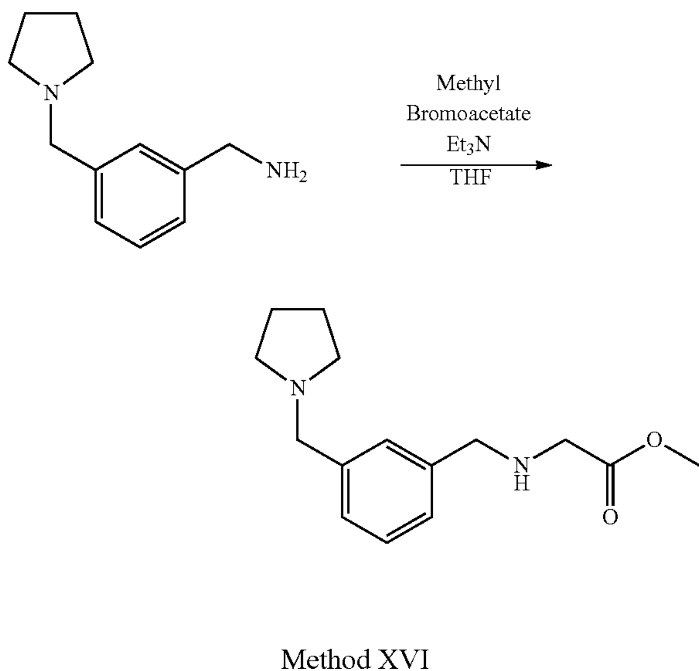
Scheme 20
