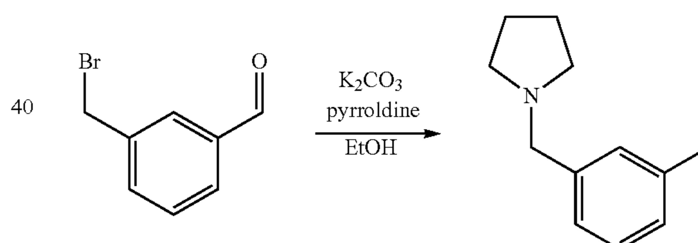
Scheme 4
