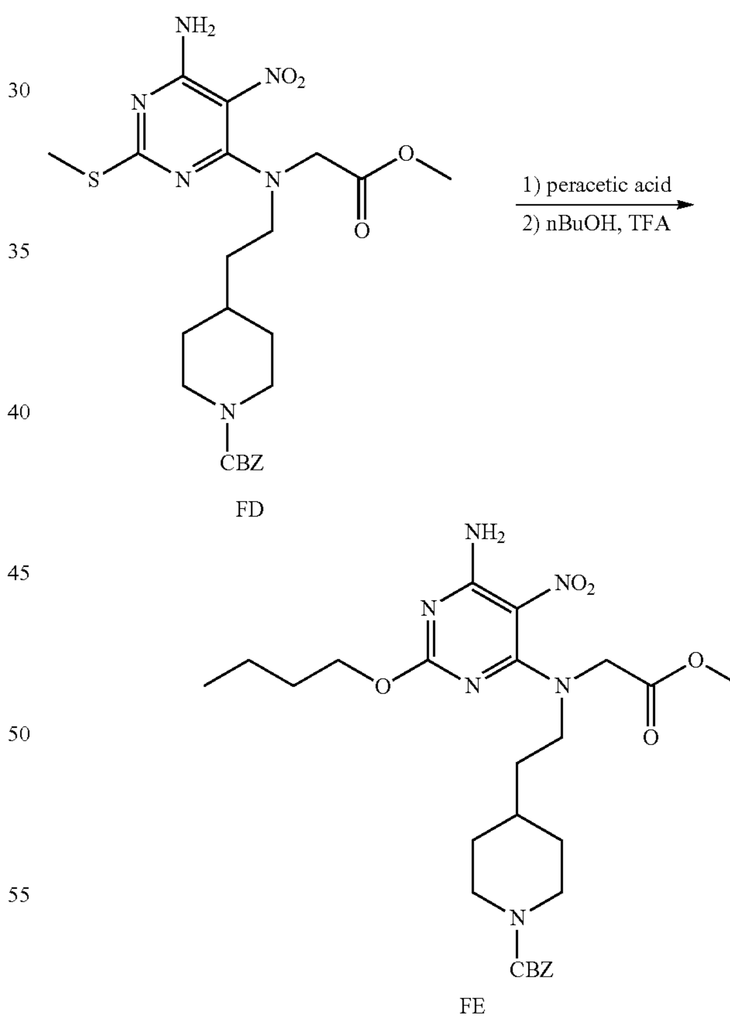
Scheme 93
