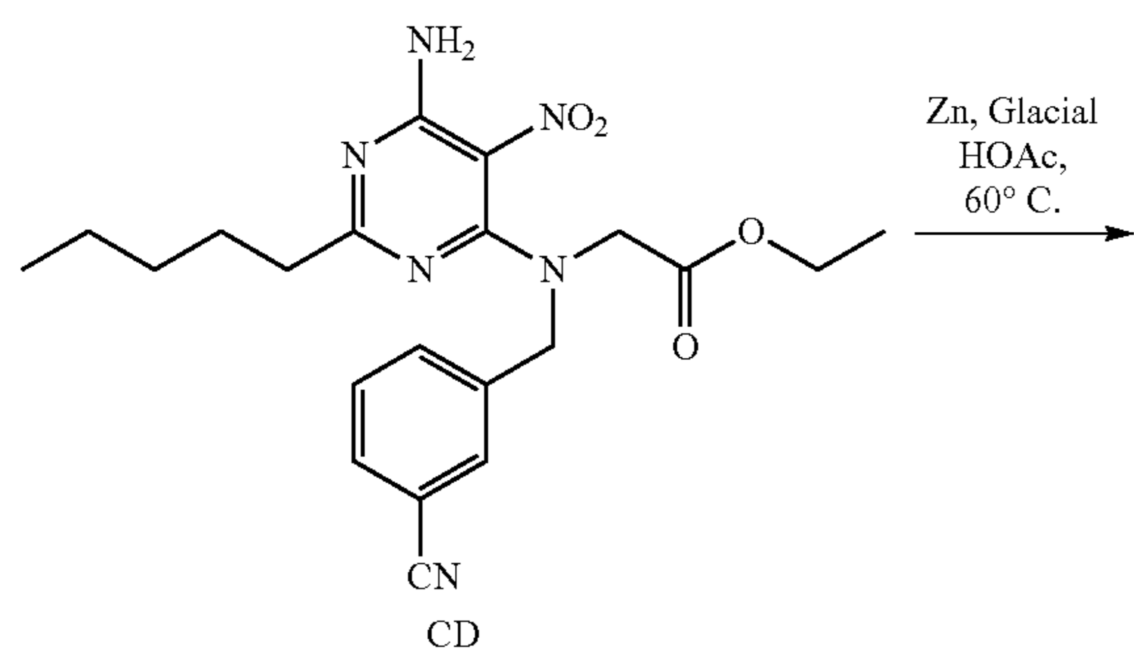
Scheme 52
