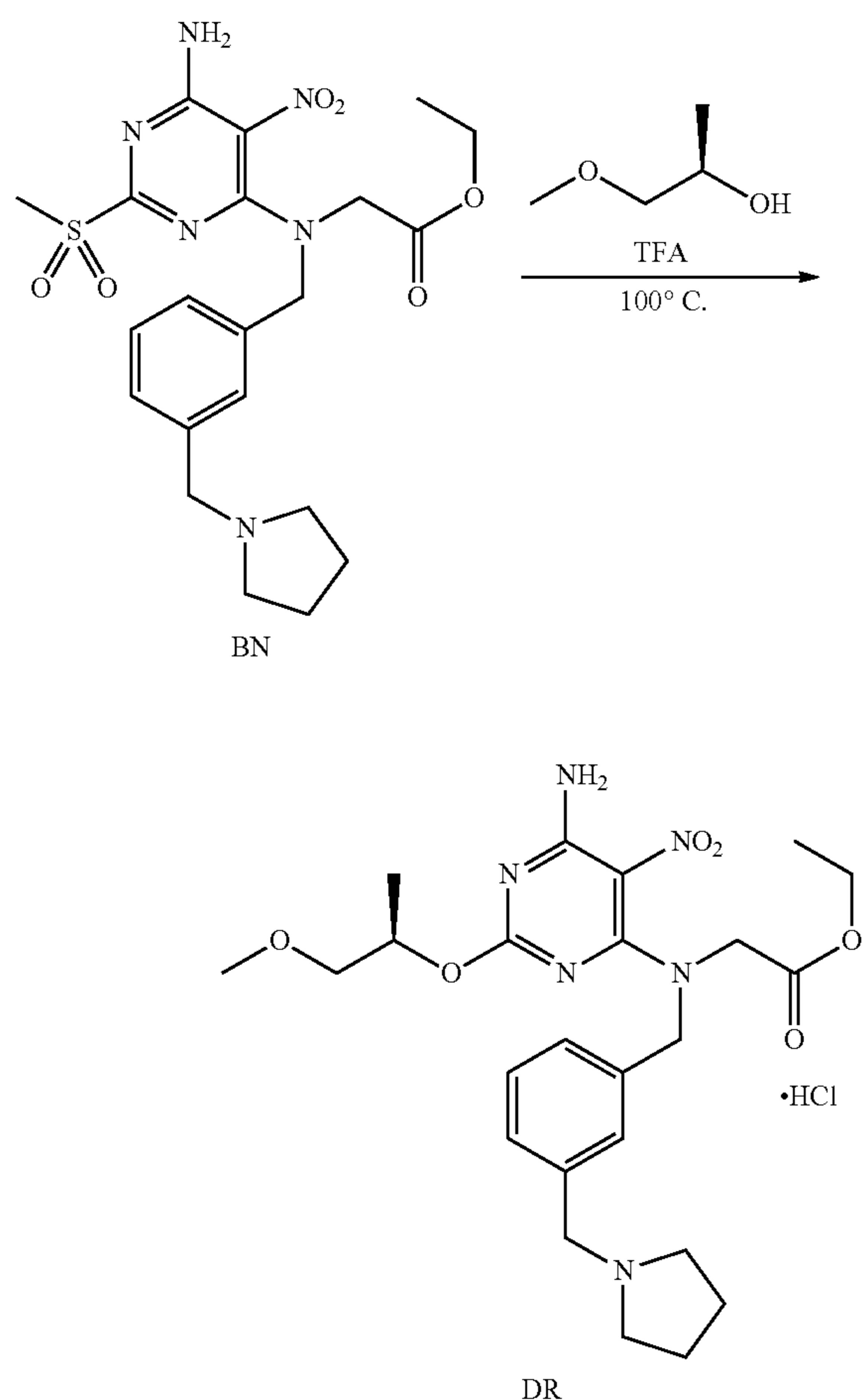
Scheme 85
