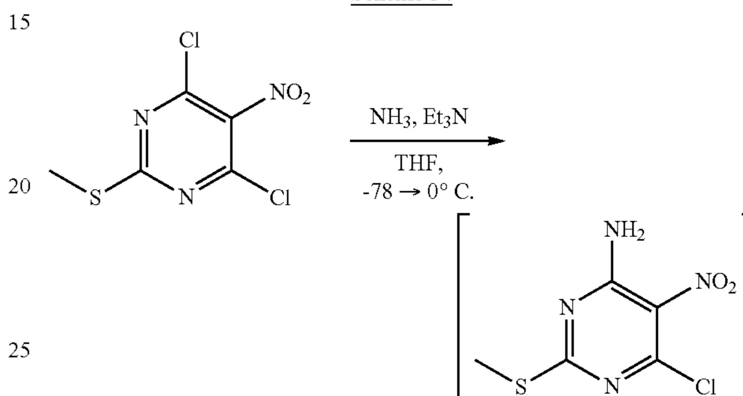
Scheme 34
