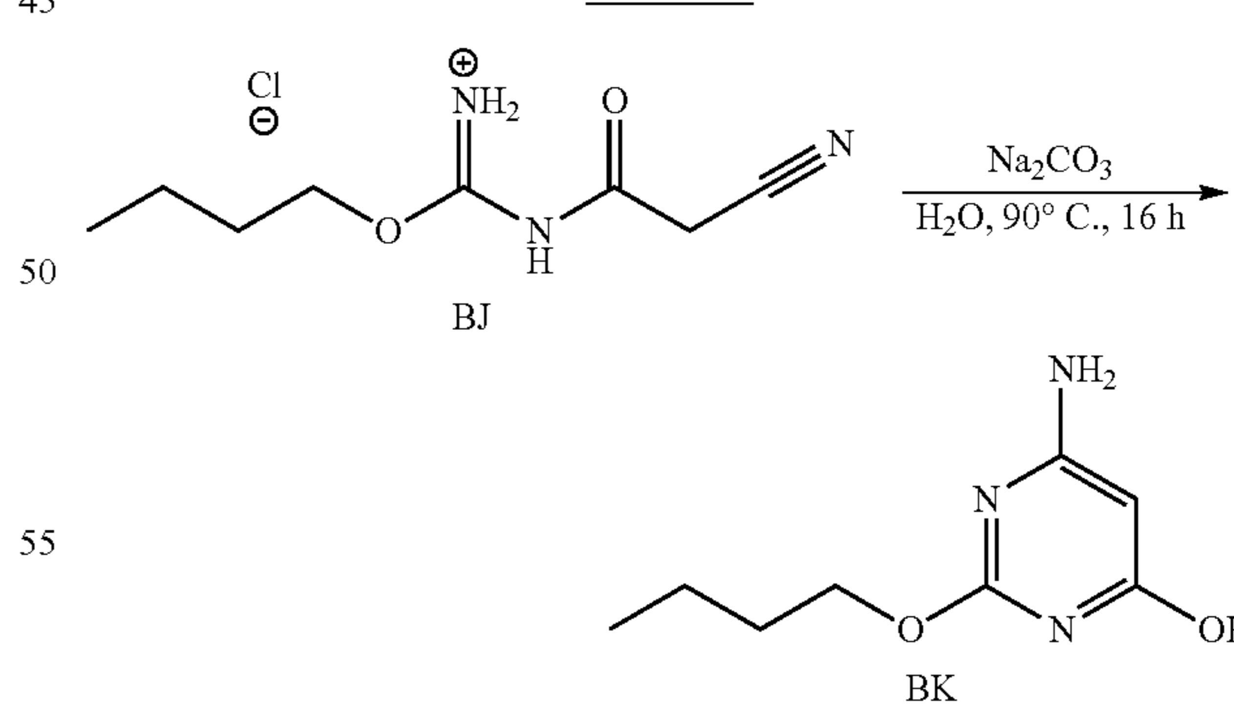
Scheme 29
