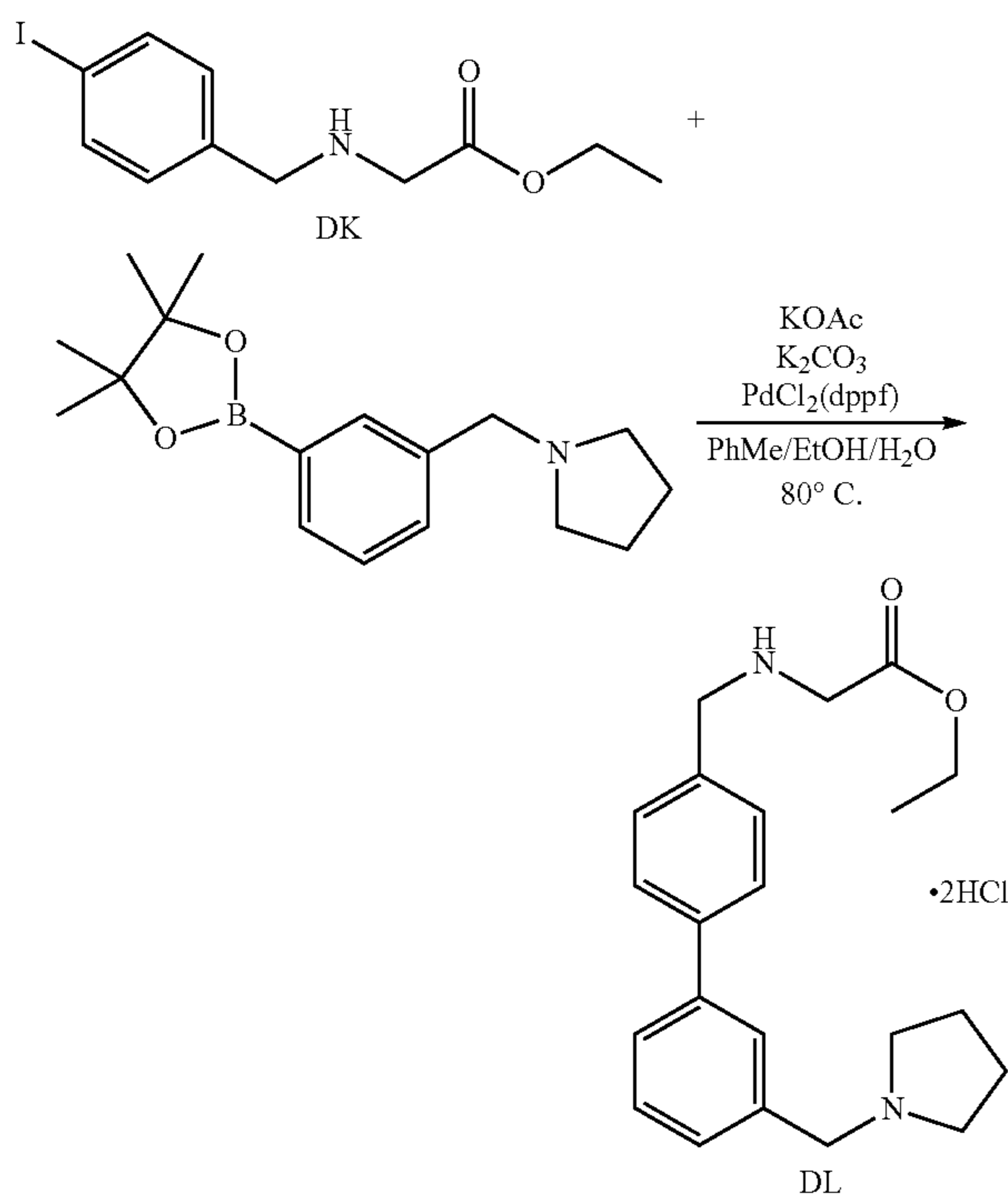
Scheme 78
