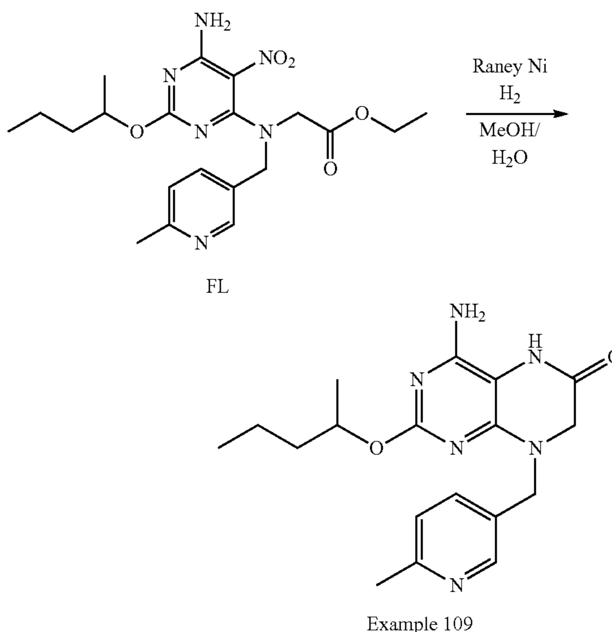
Scheme 101:
