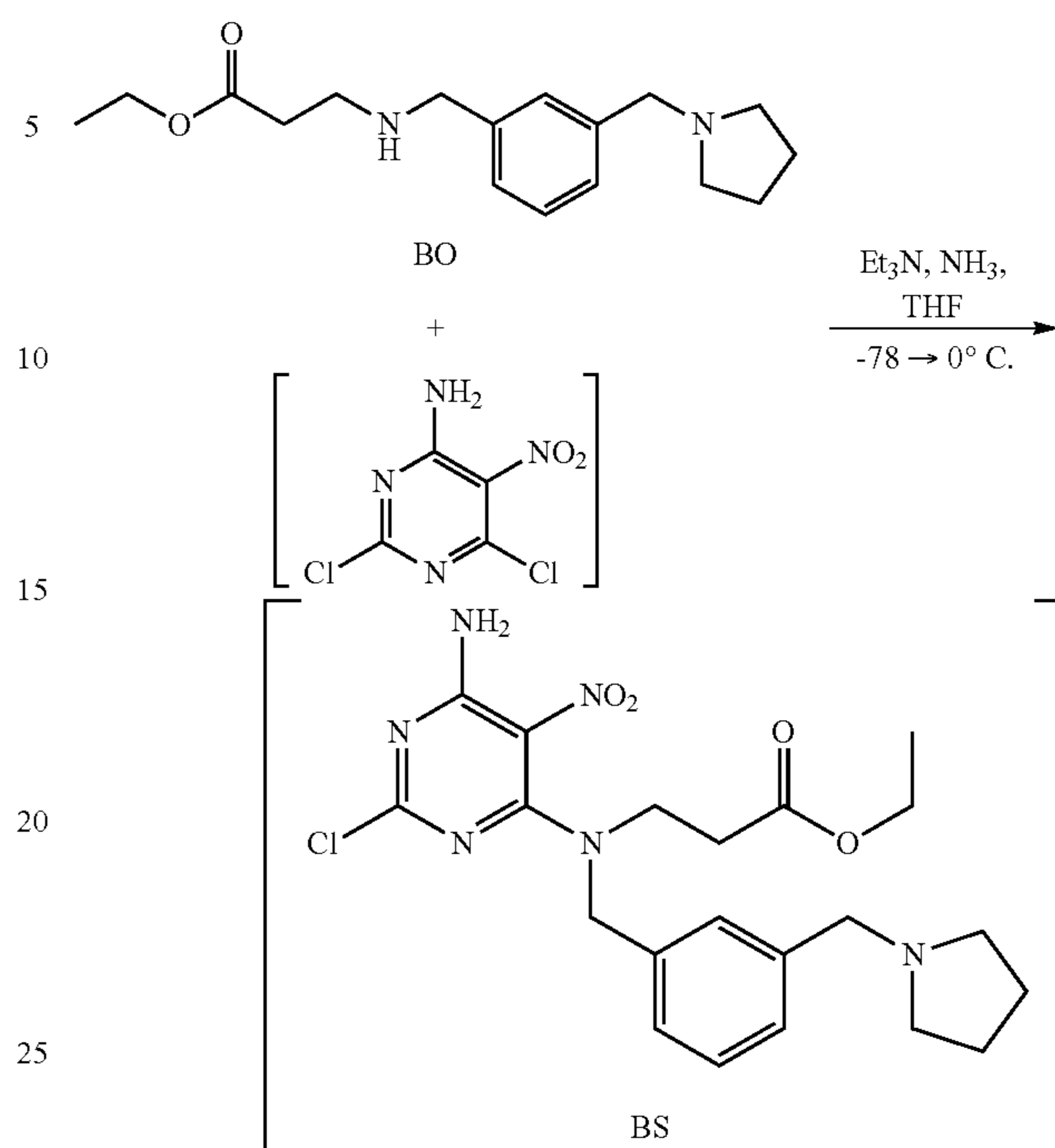
Scheme 40
