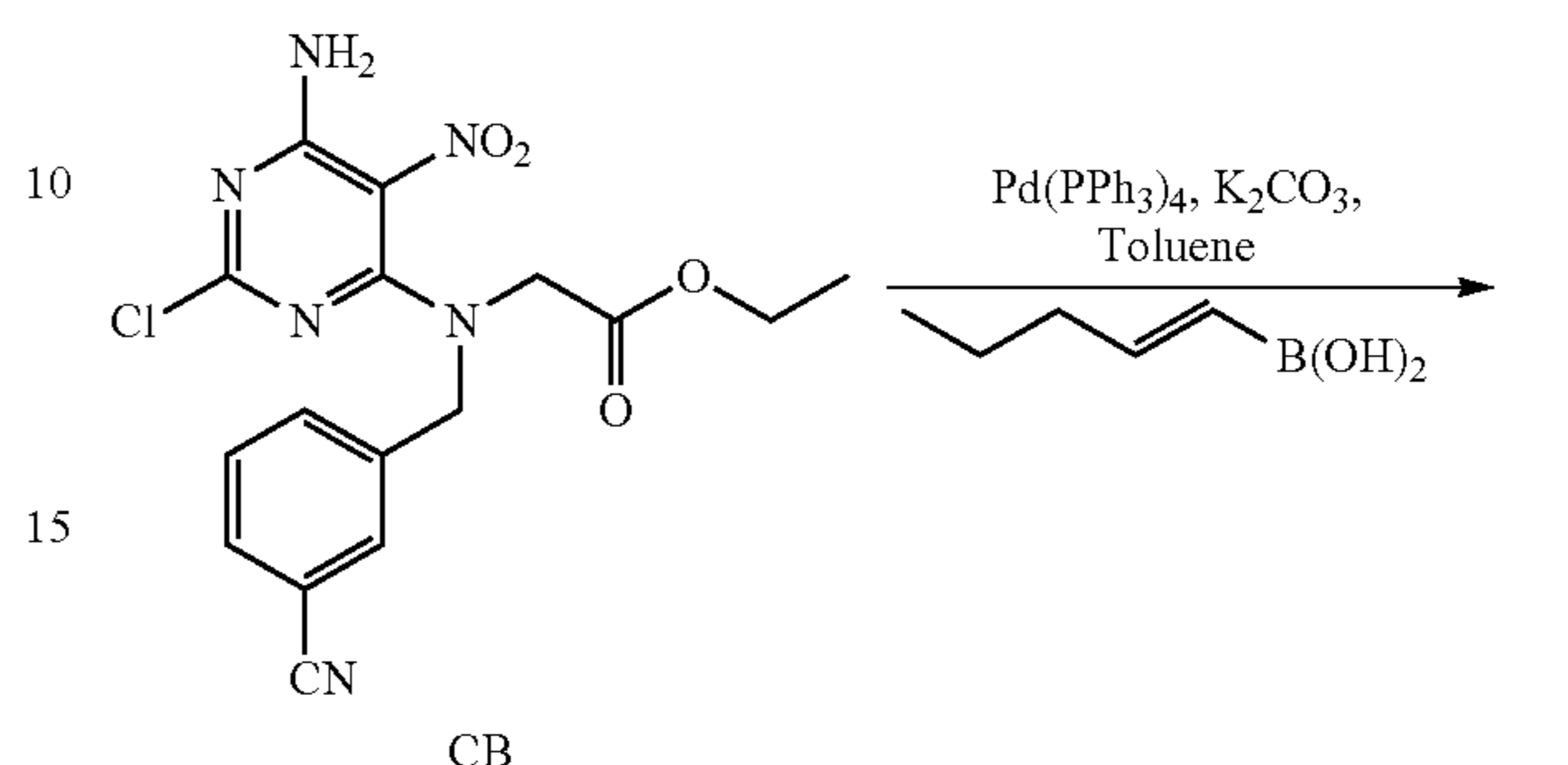
Scheme 50
