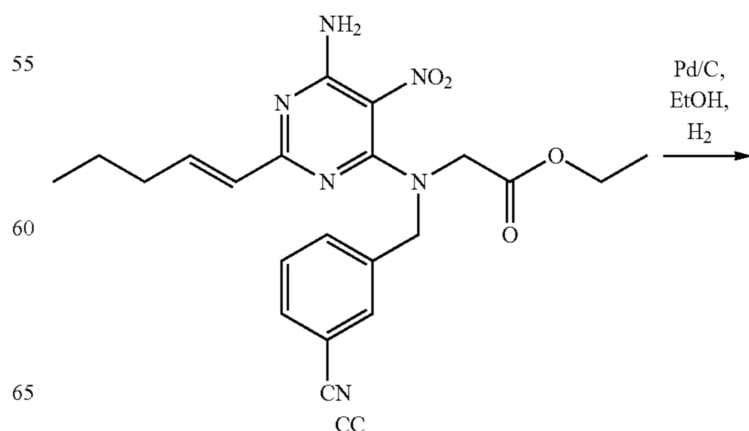
Scheme 51
