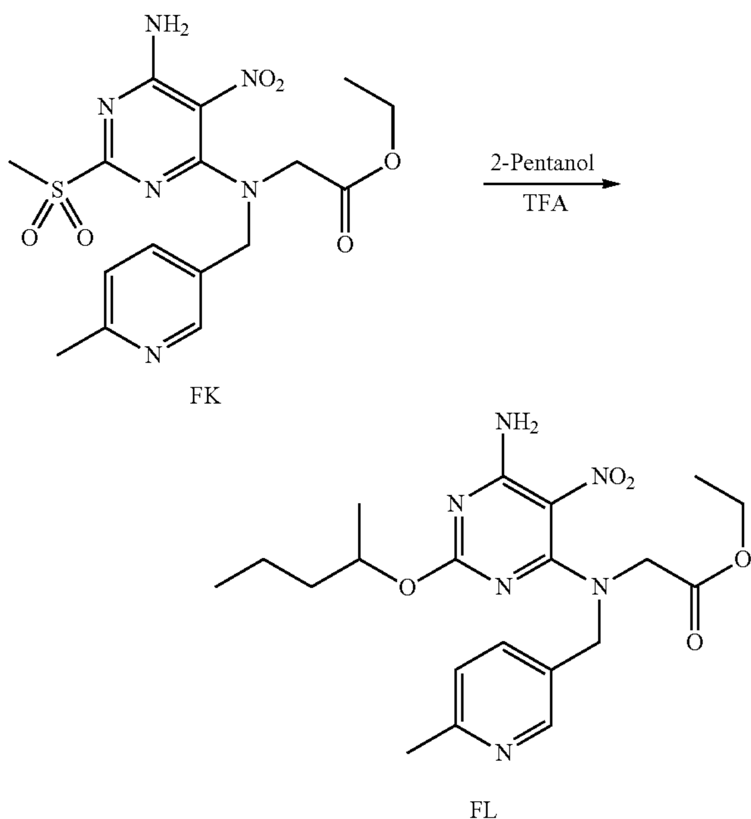
Scheme 100:
