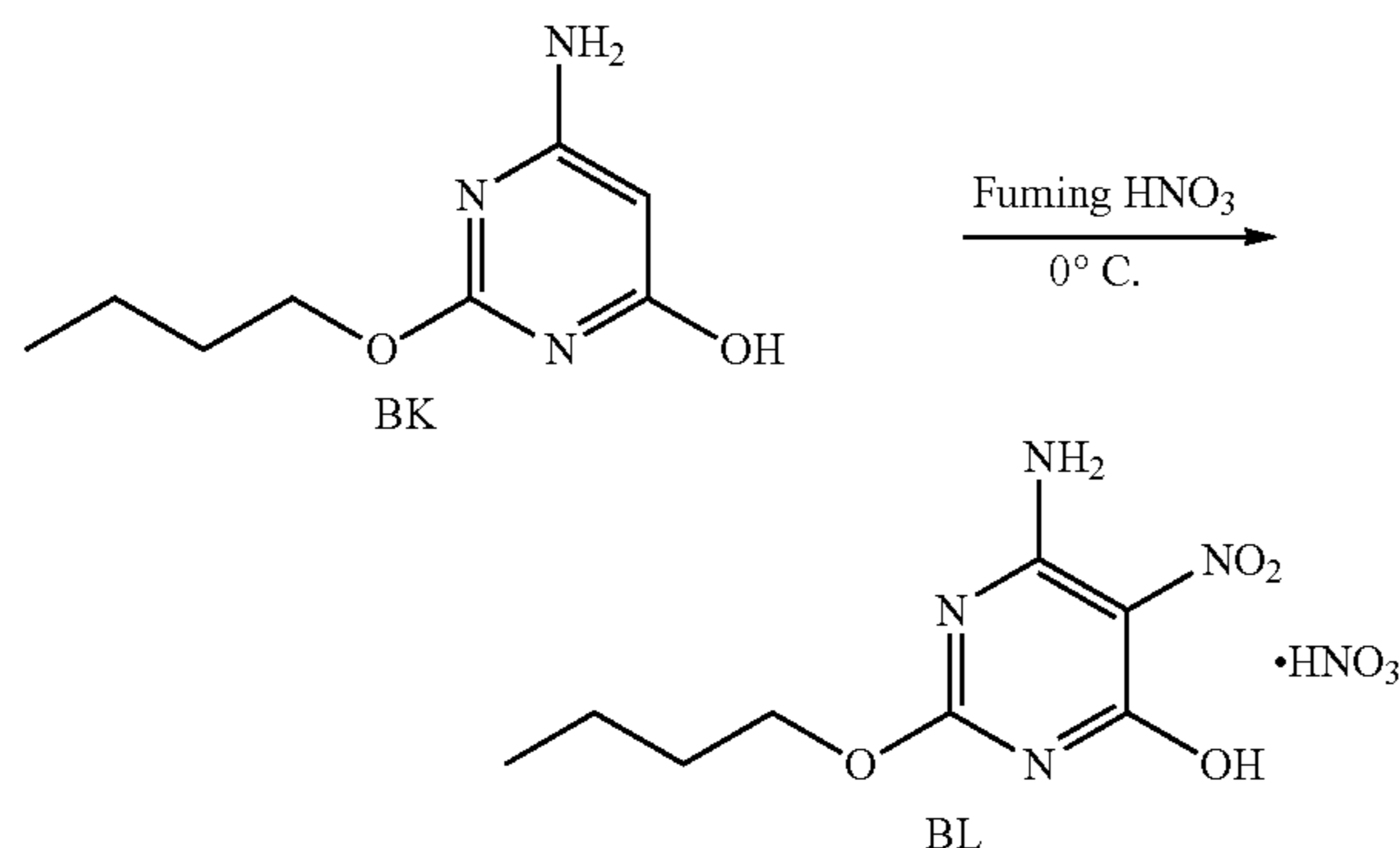
Scheme 30
