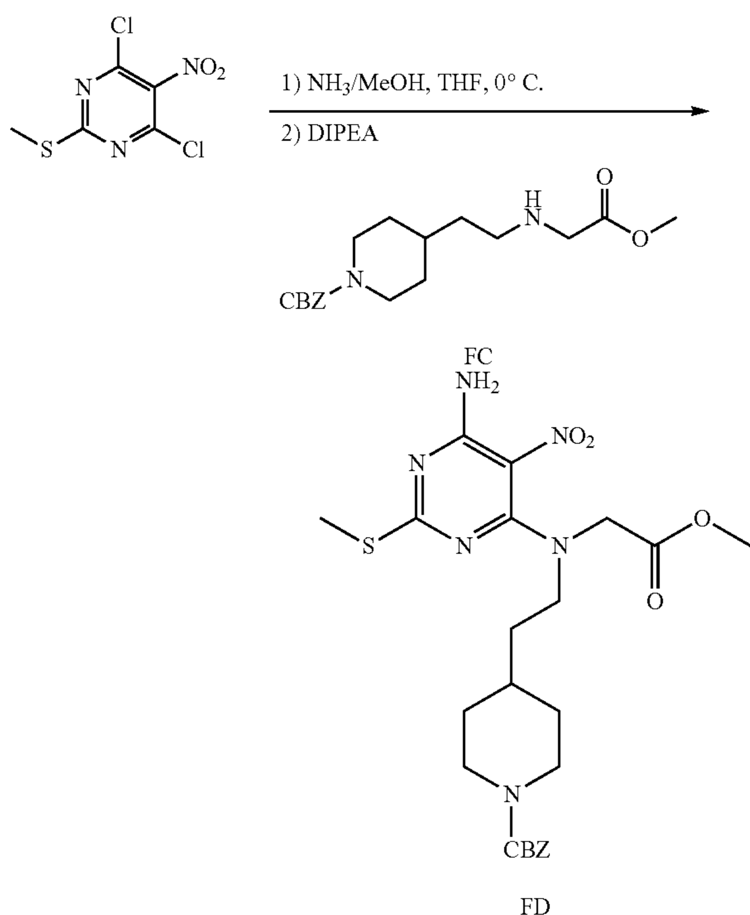
Scheme 92
