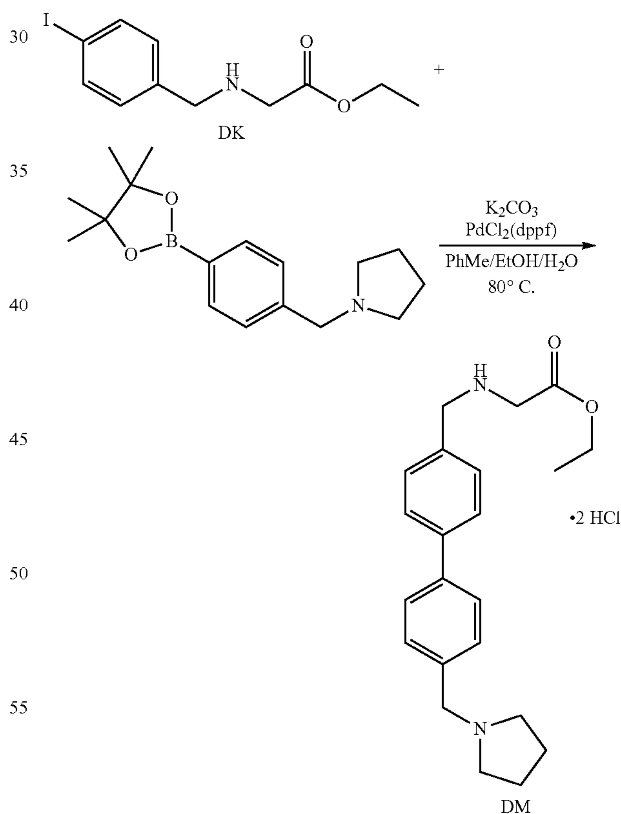
Scheme 79
