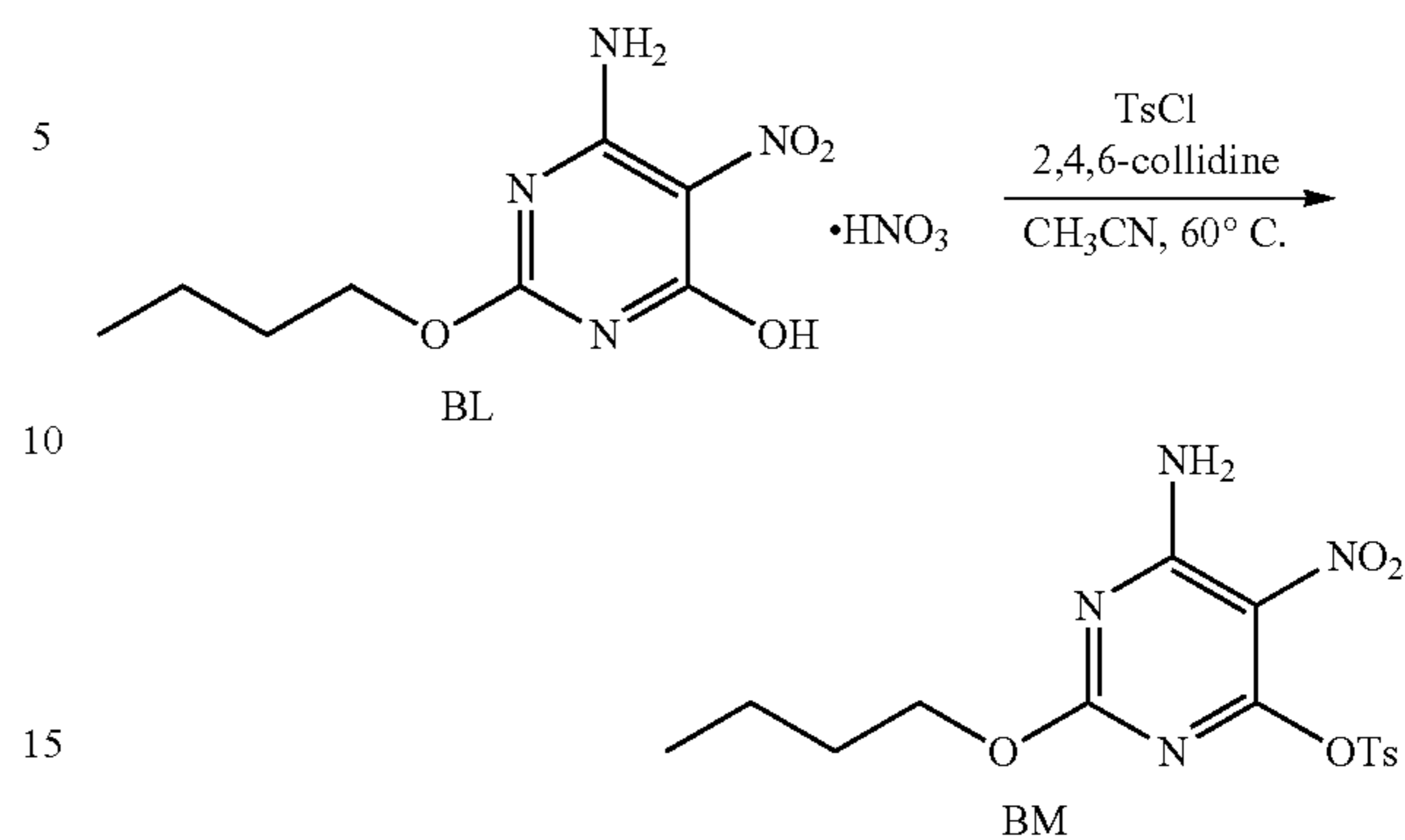
Scheme 31
