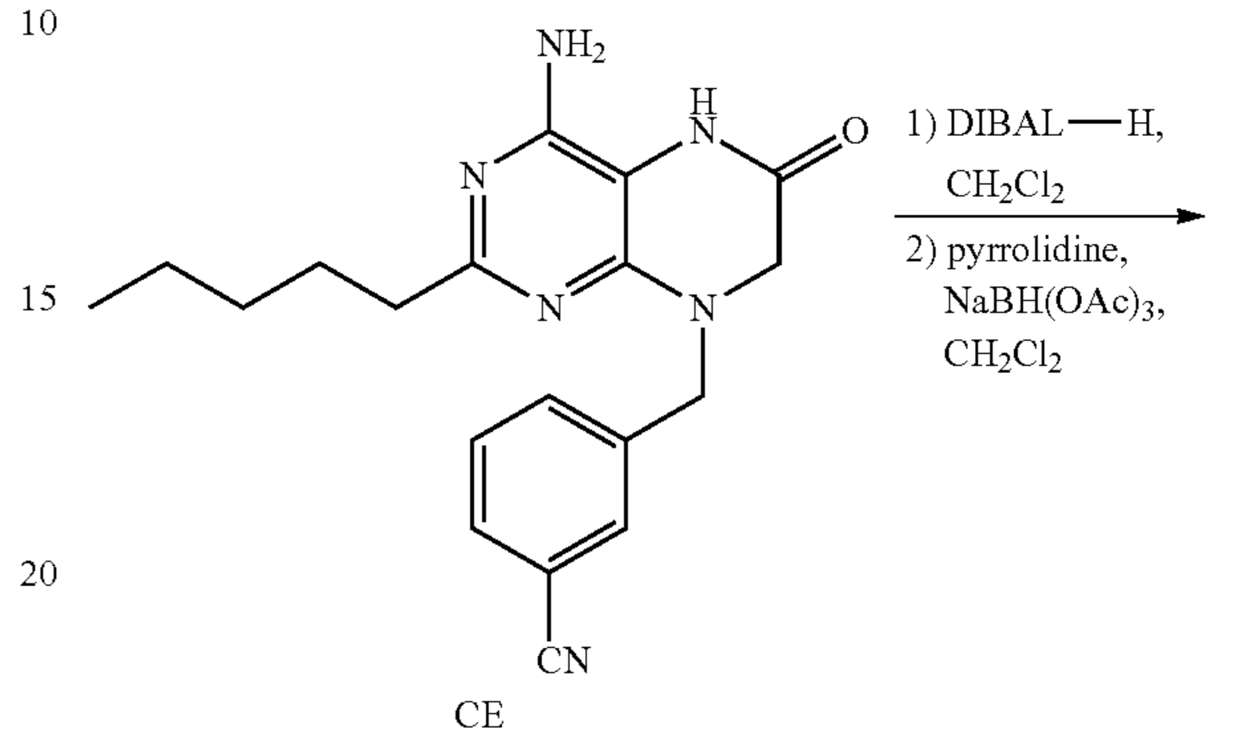
Scheme 53:
