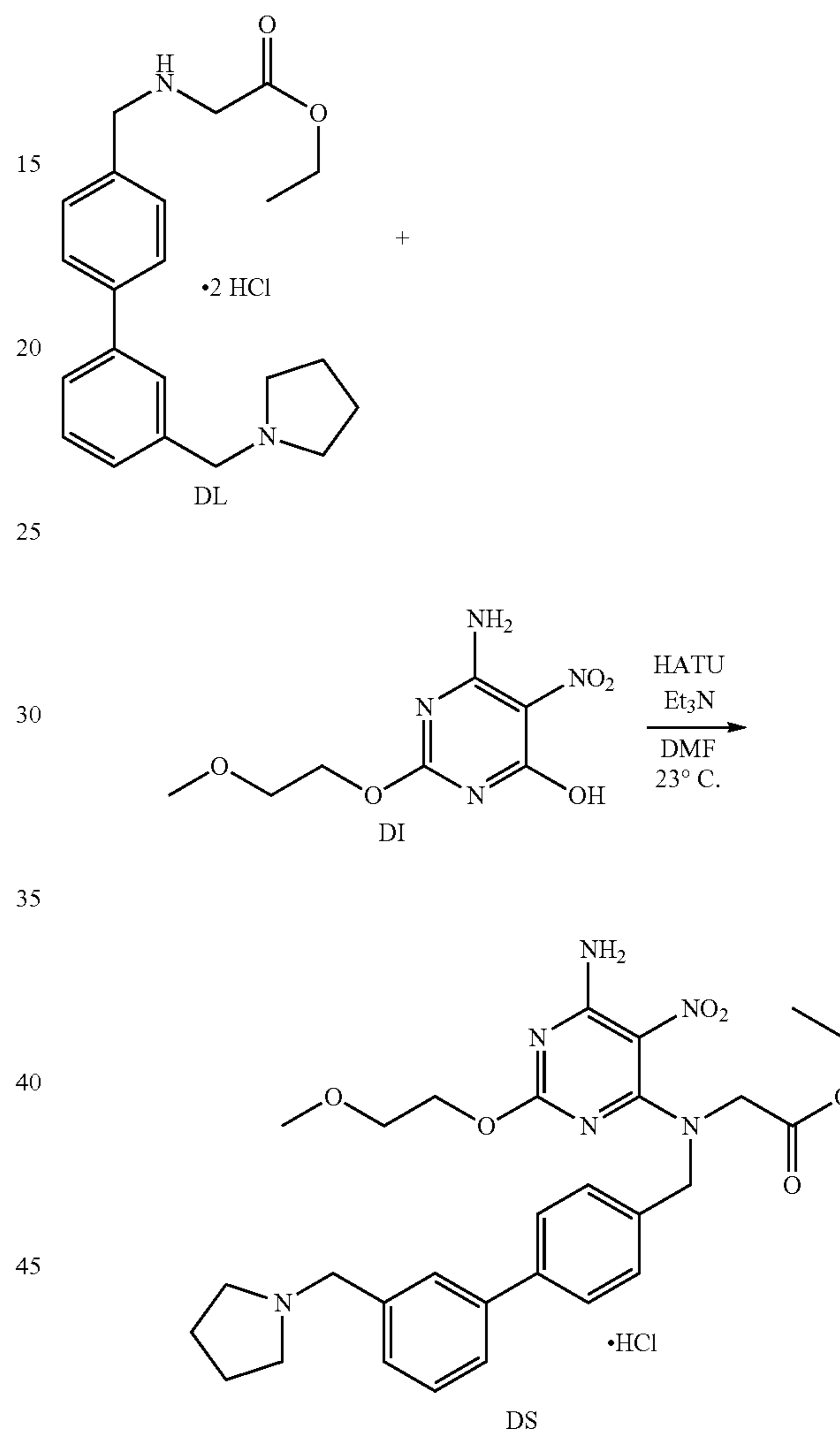
Scheme 86
