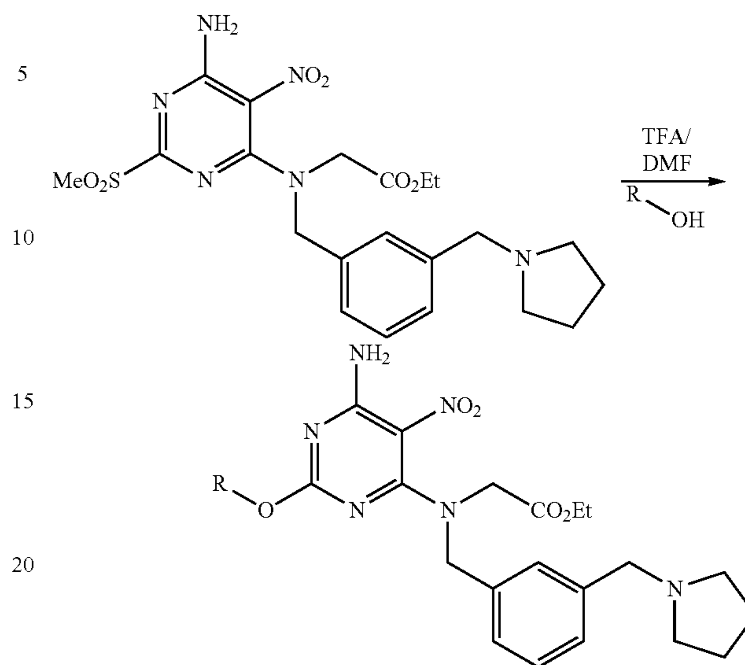
Scheme 14
