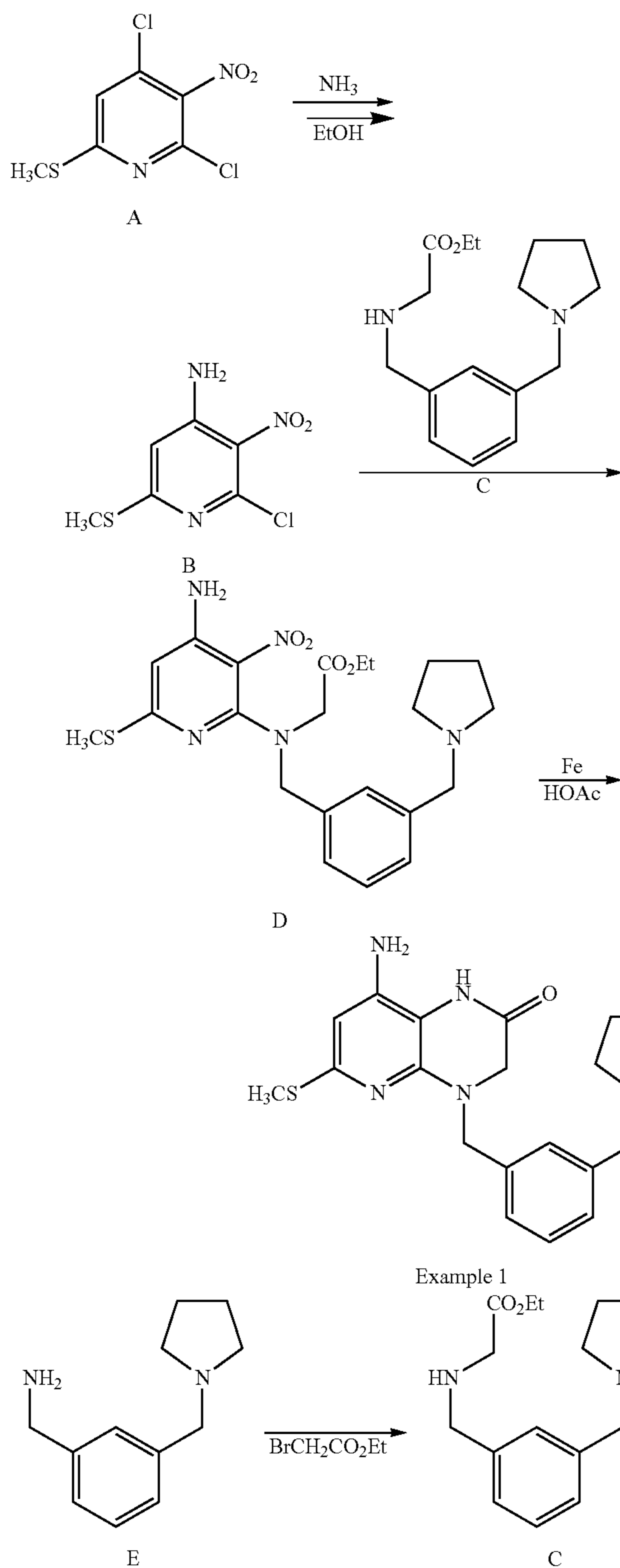
Scheme 1
