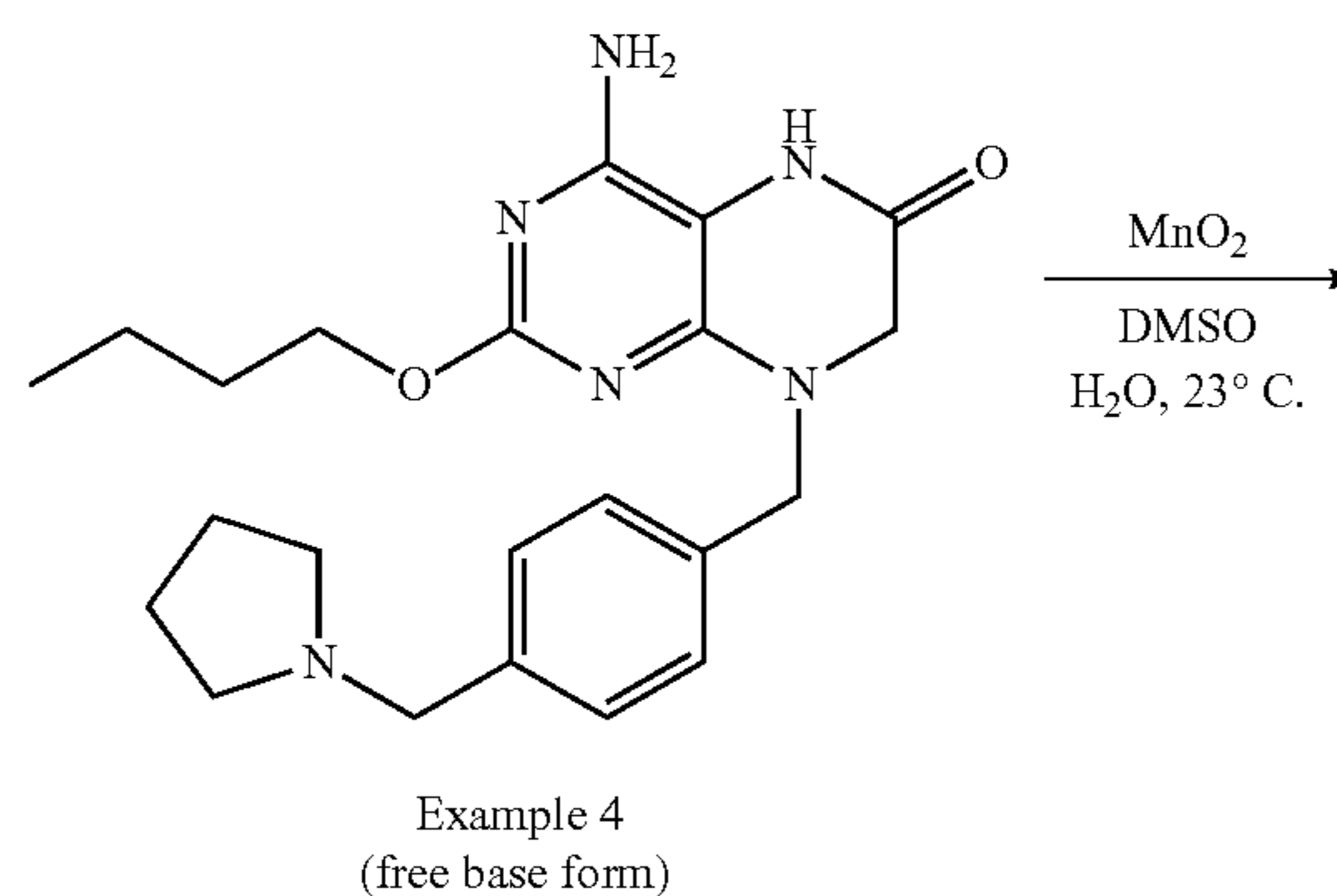
Scheme 88:
