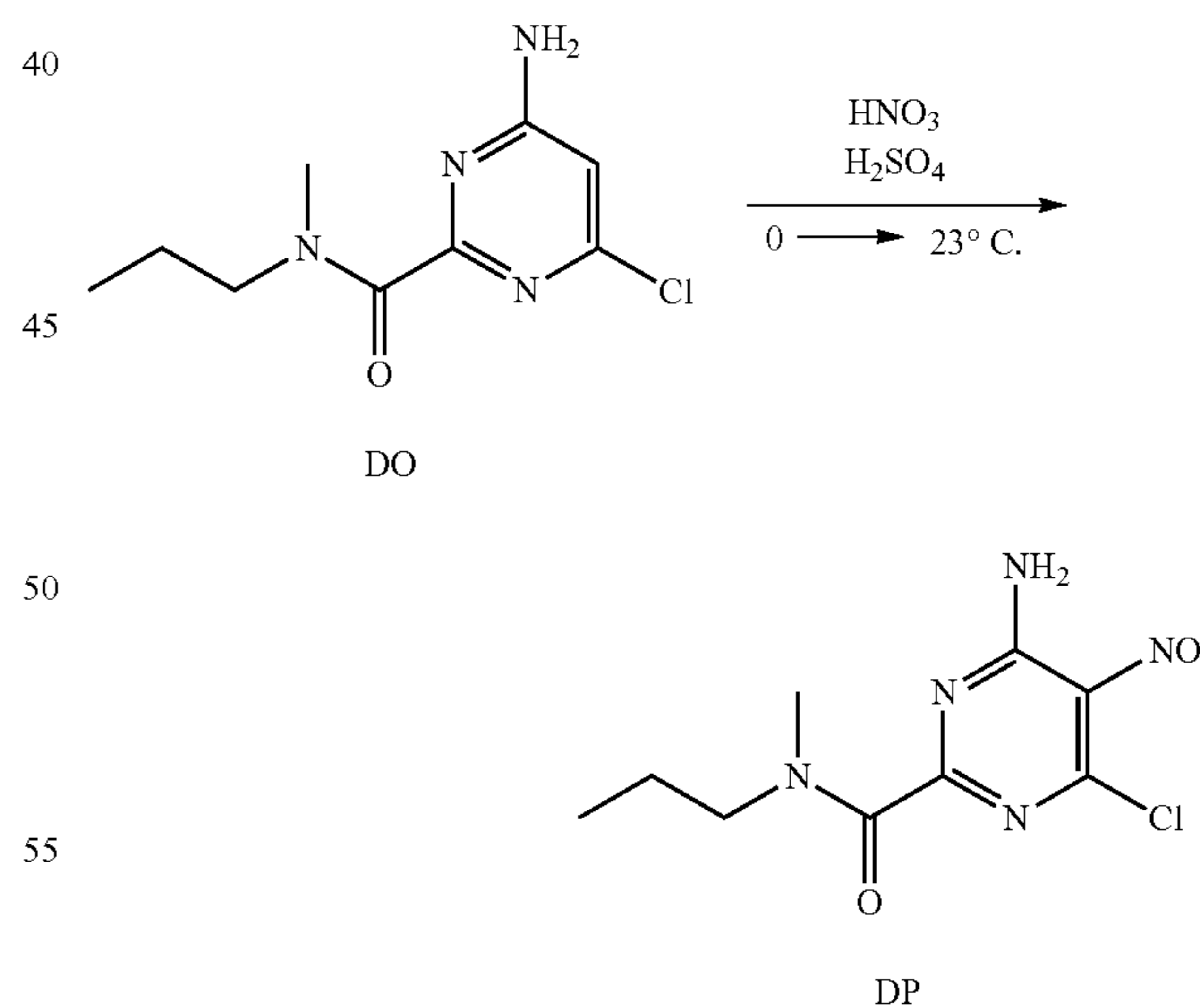
Scheme 82
