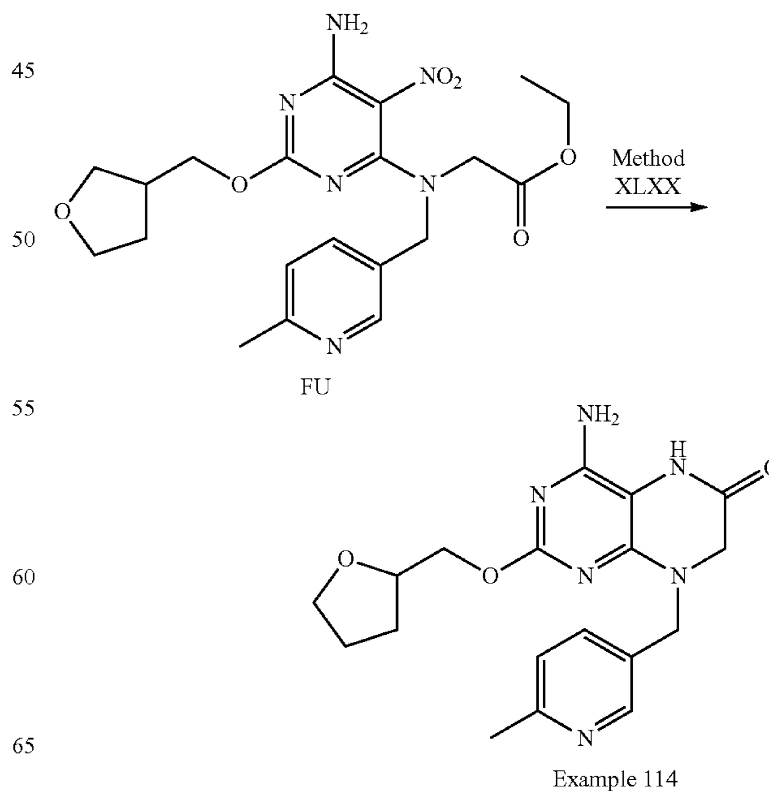
Scheme 113:
