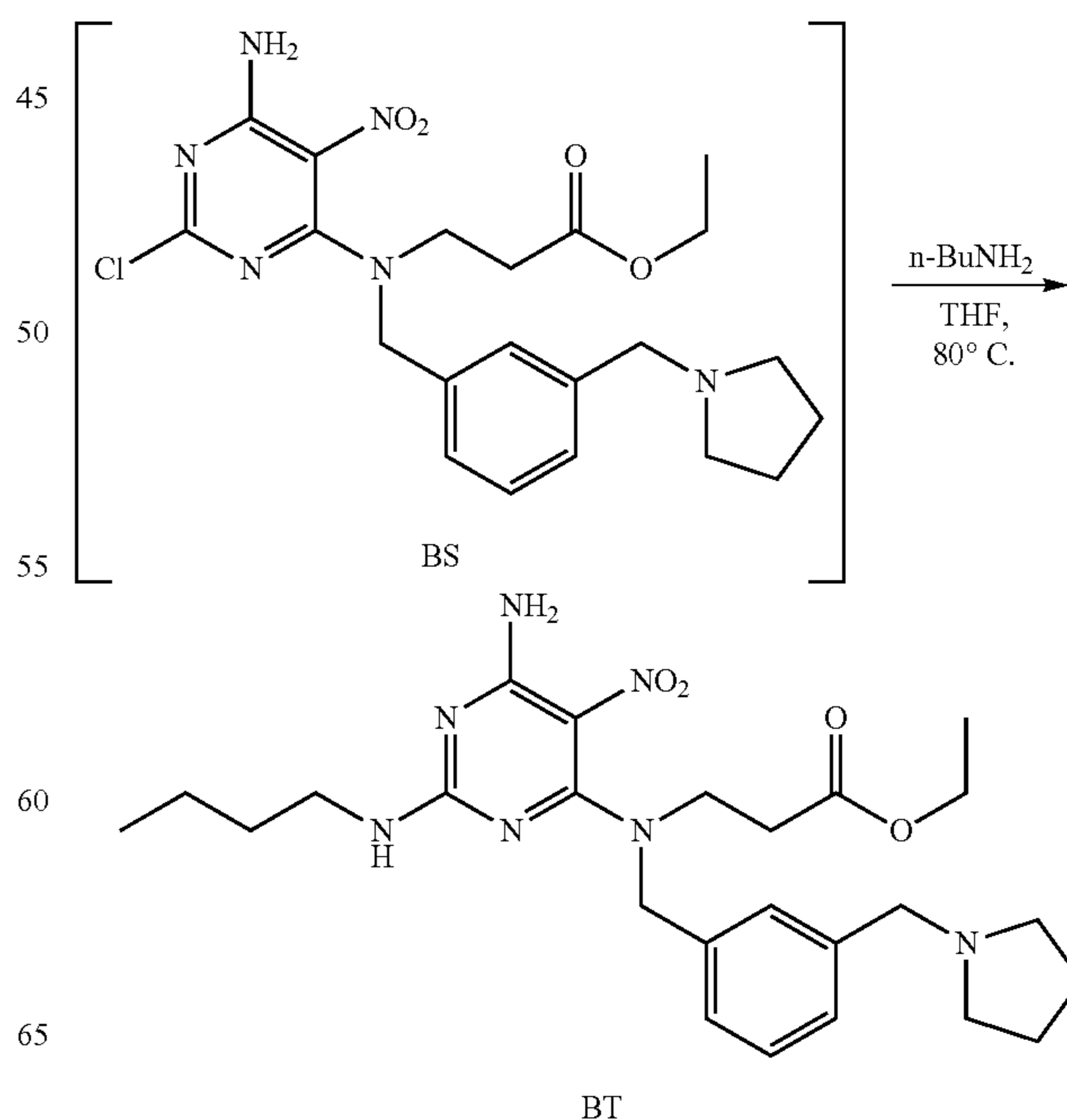
Scheme 41
