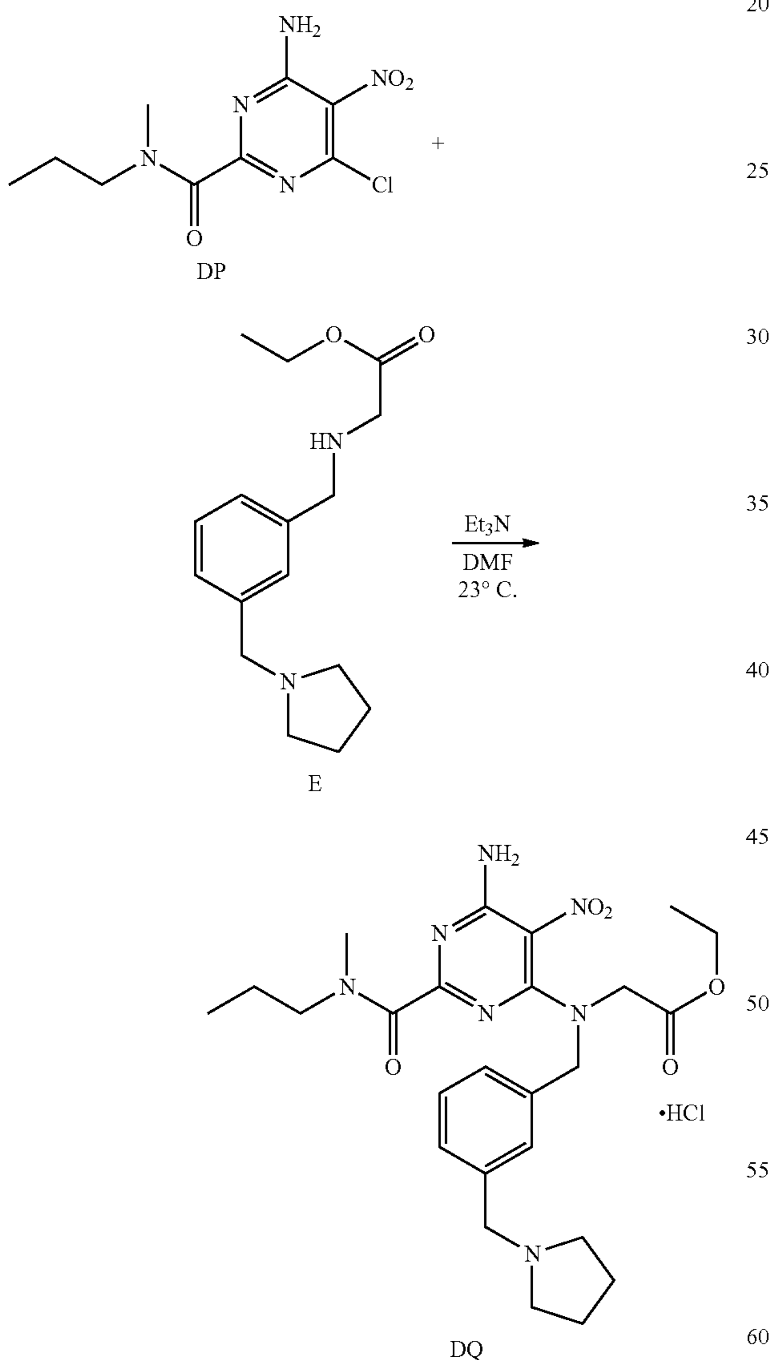
Scheme 83:
