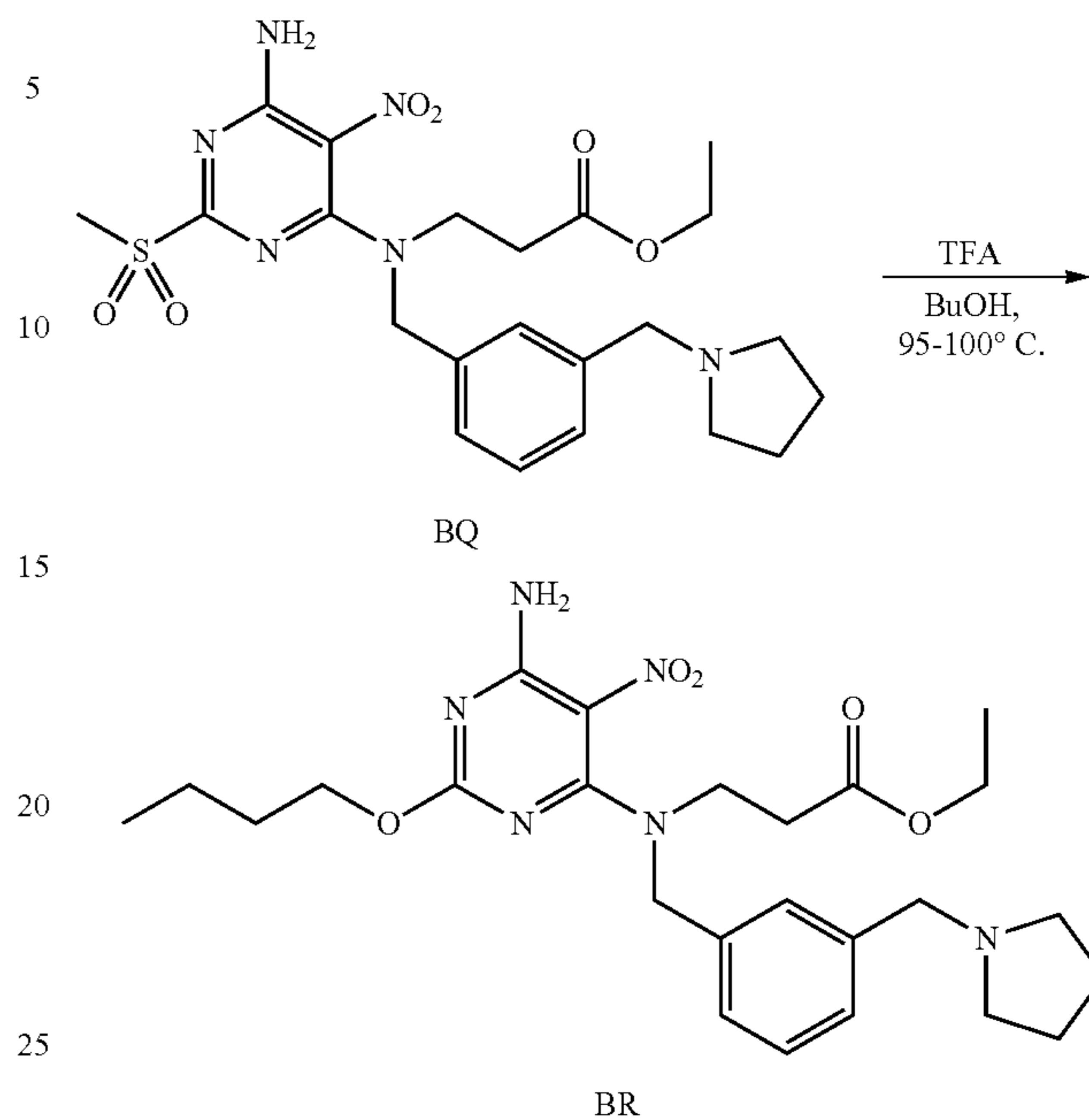
Scheme 37
