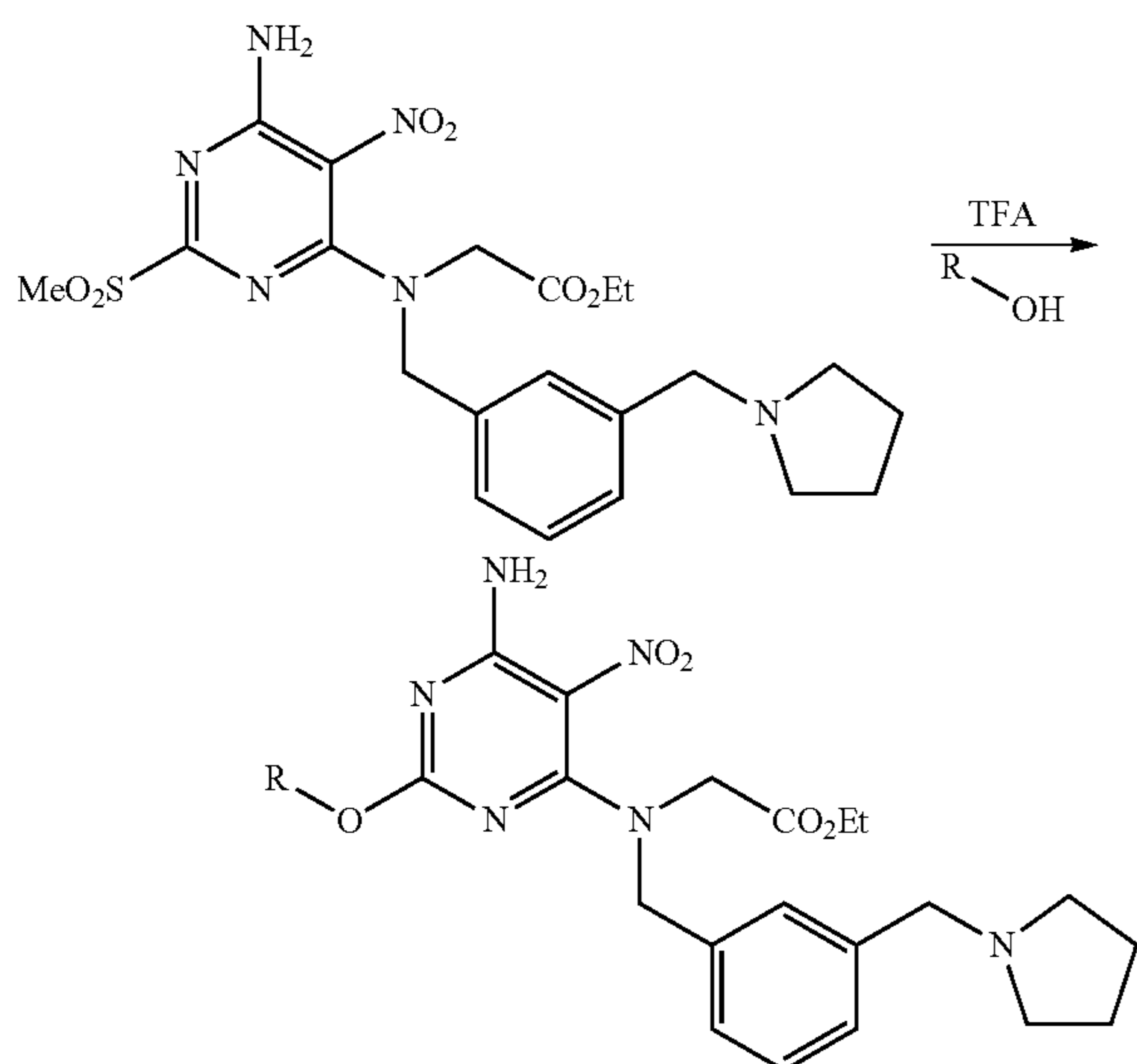
Scheme 13
