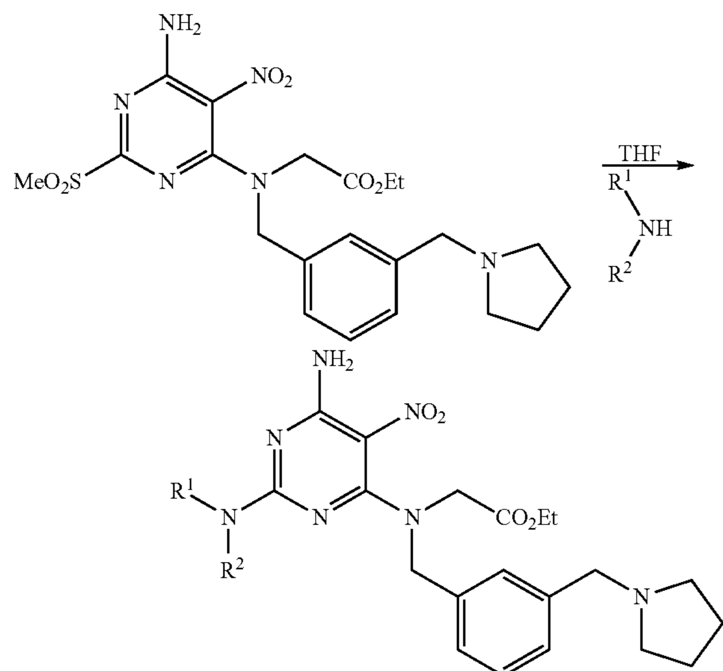
Scheme 16
