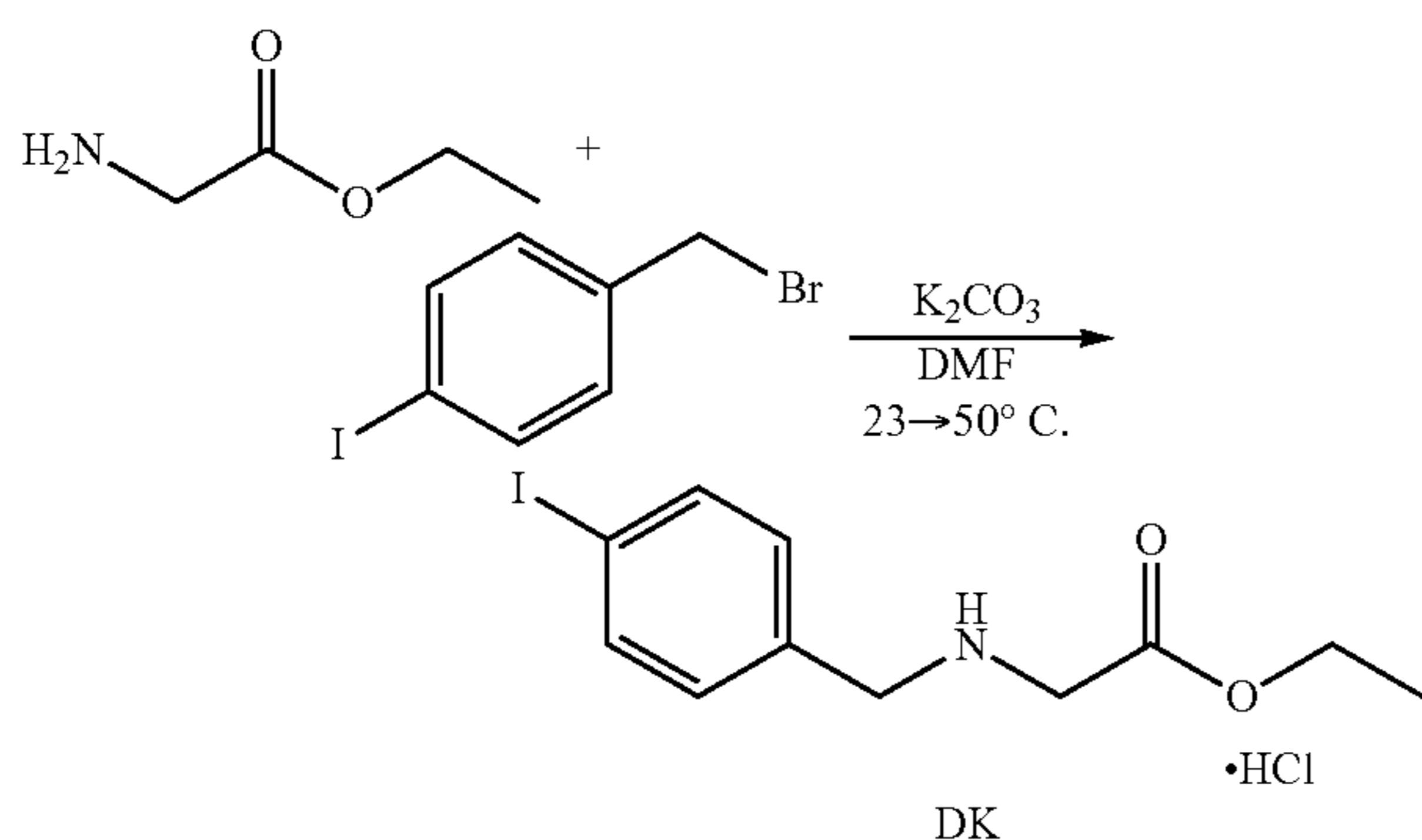
Scheme 77
