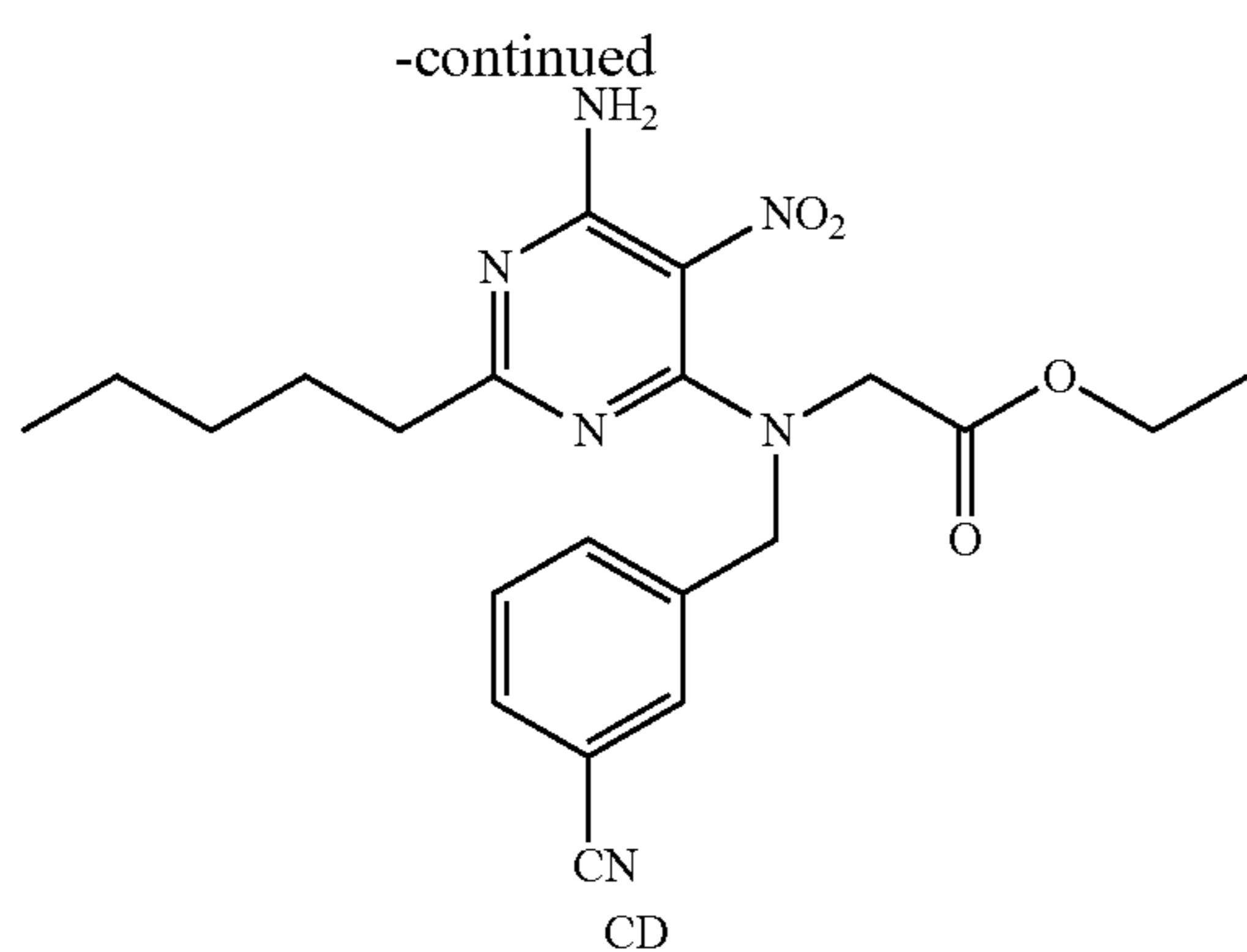
Scheme 53:
