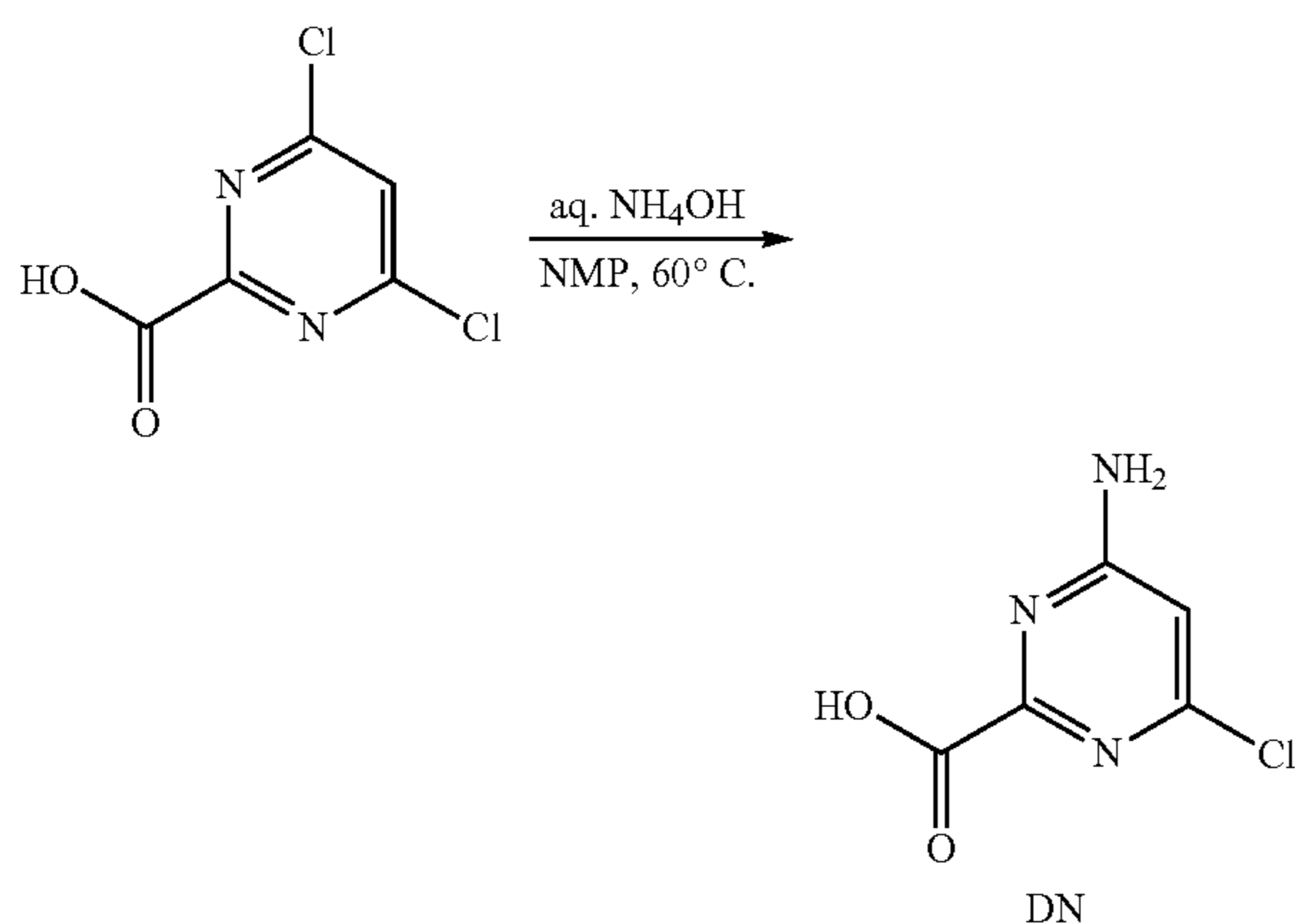
Scheme 80
