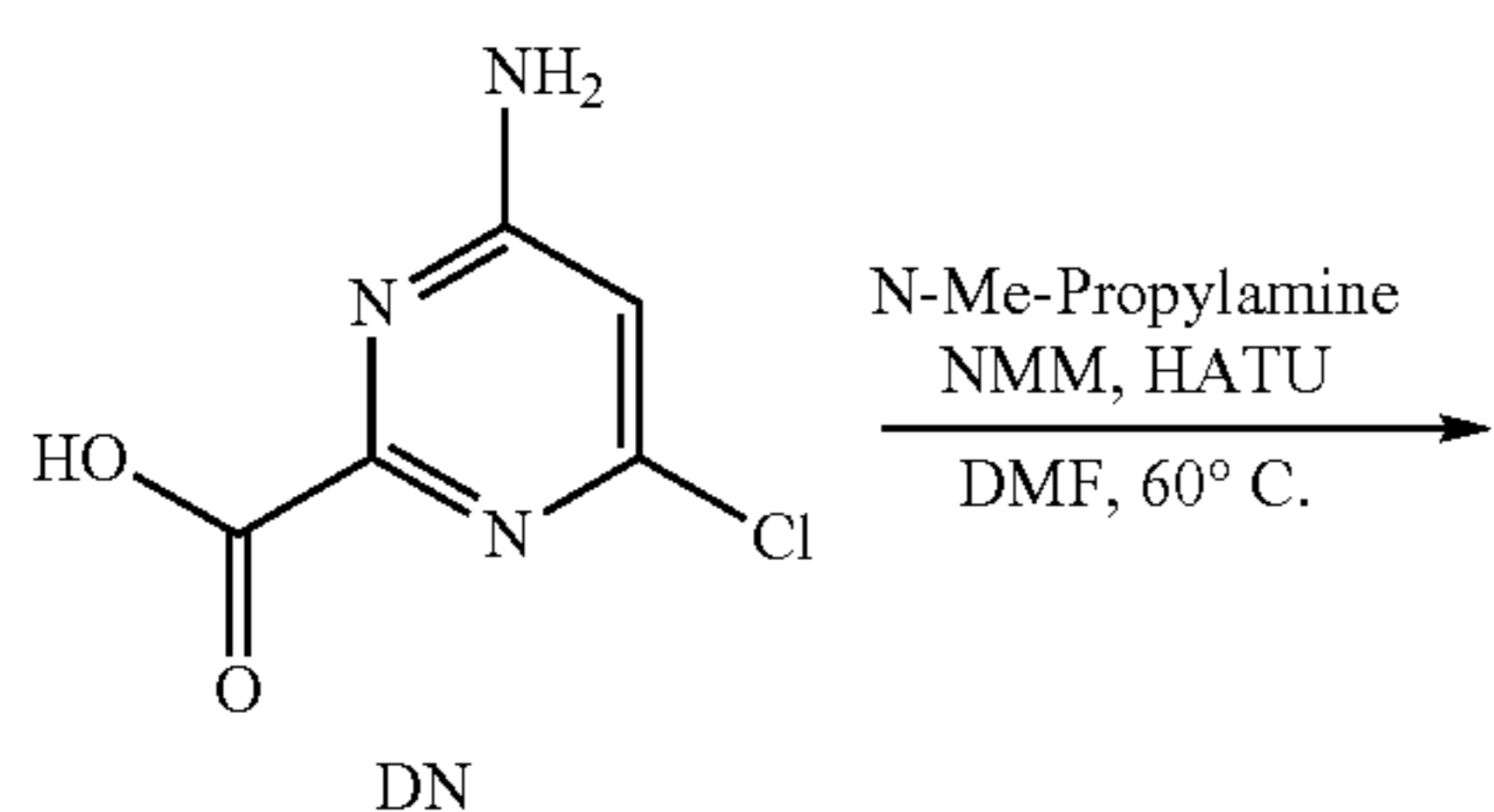
Scheme 81:
