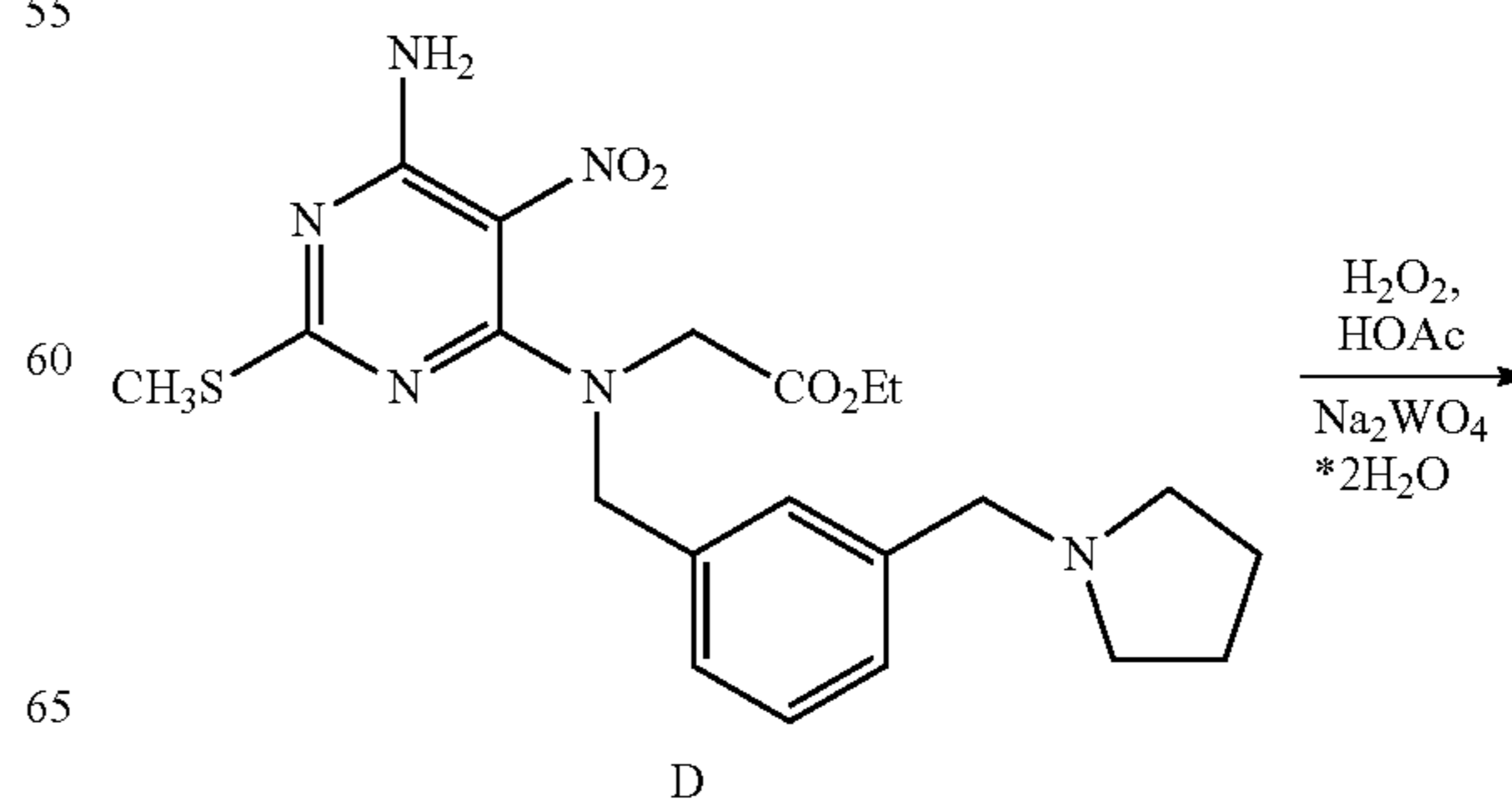
Scheme 32
