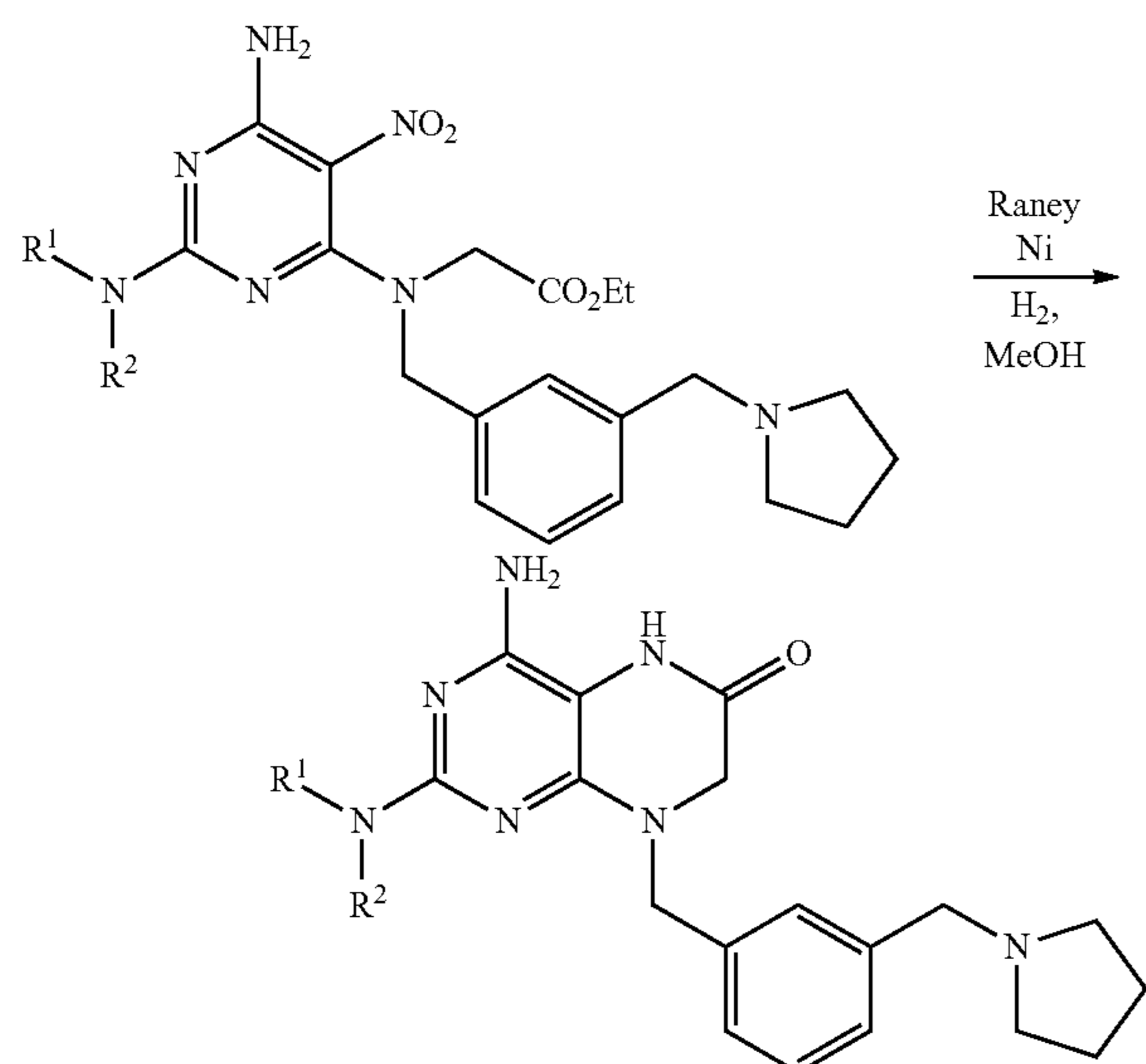
Scheme 17
