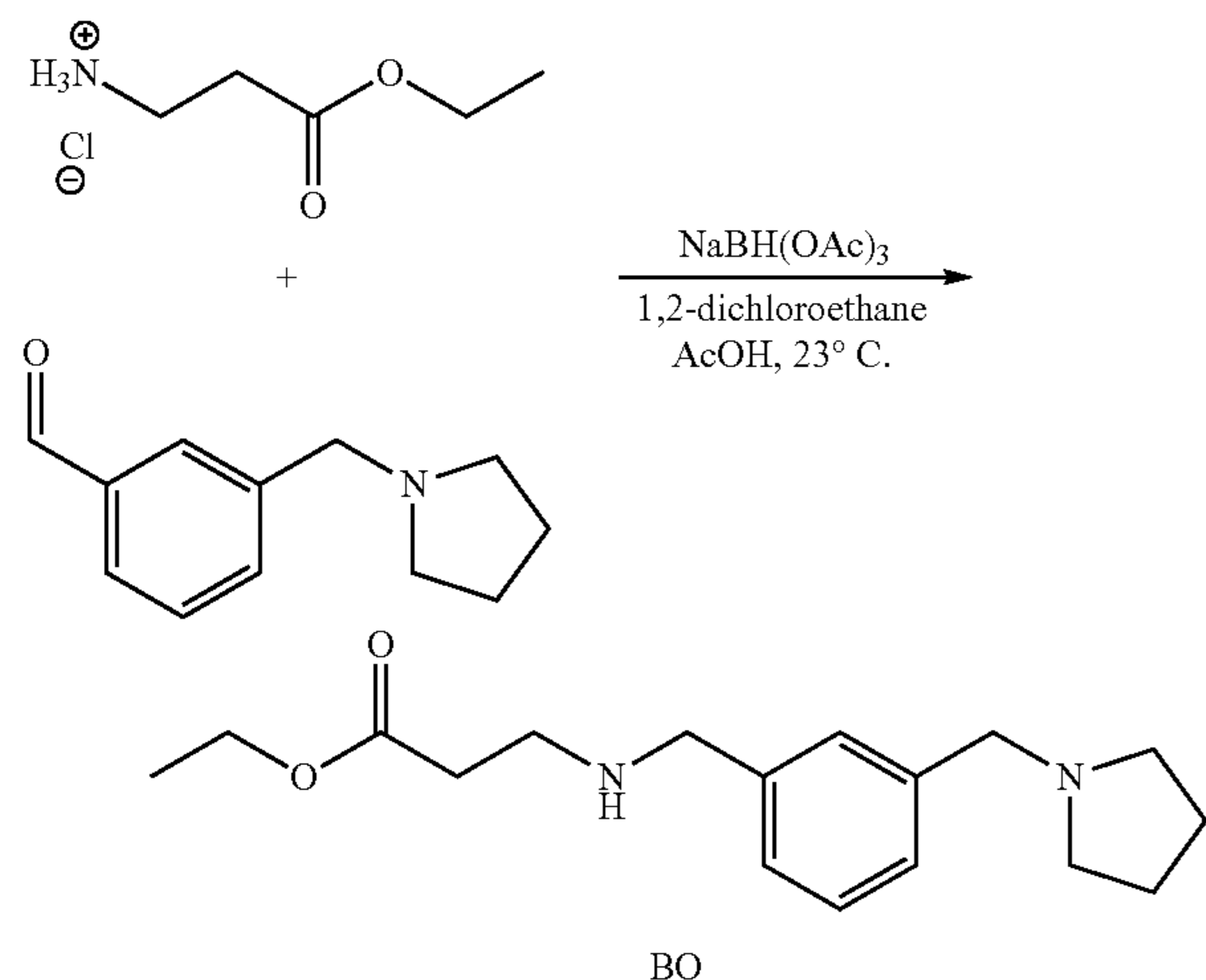
Scheme 33
