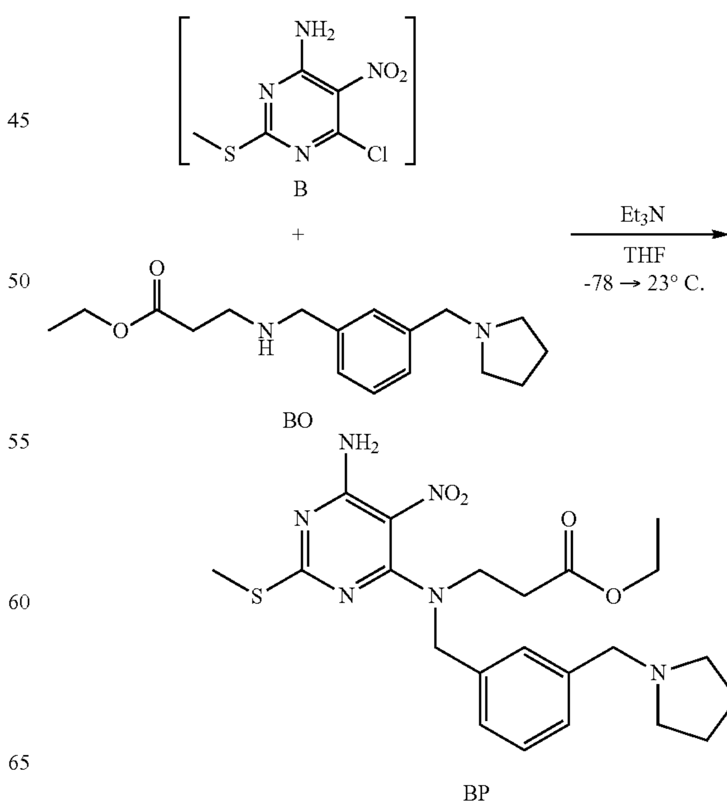
Scheme 35
