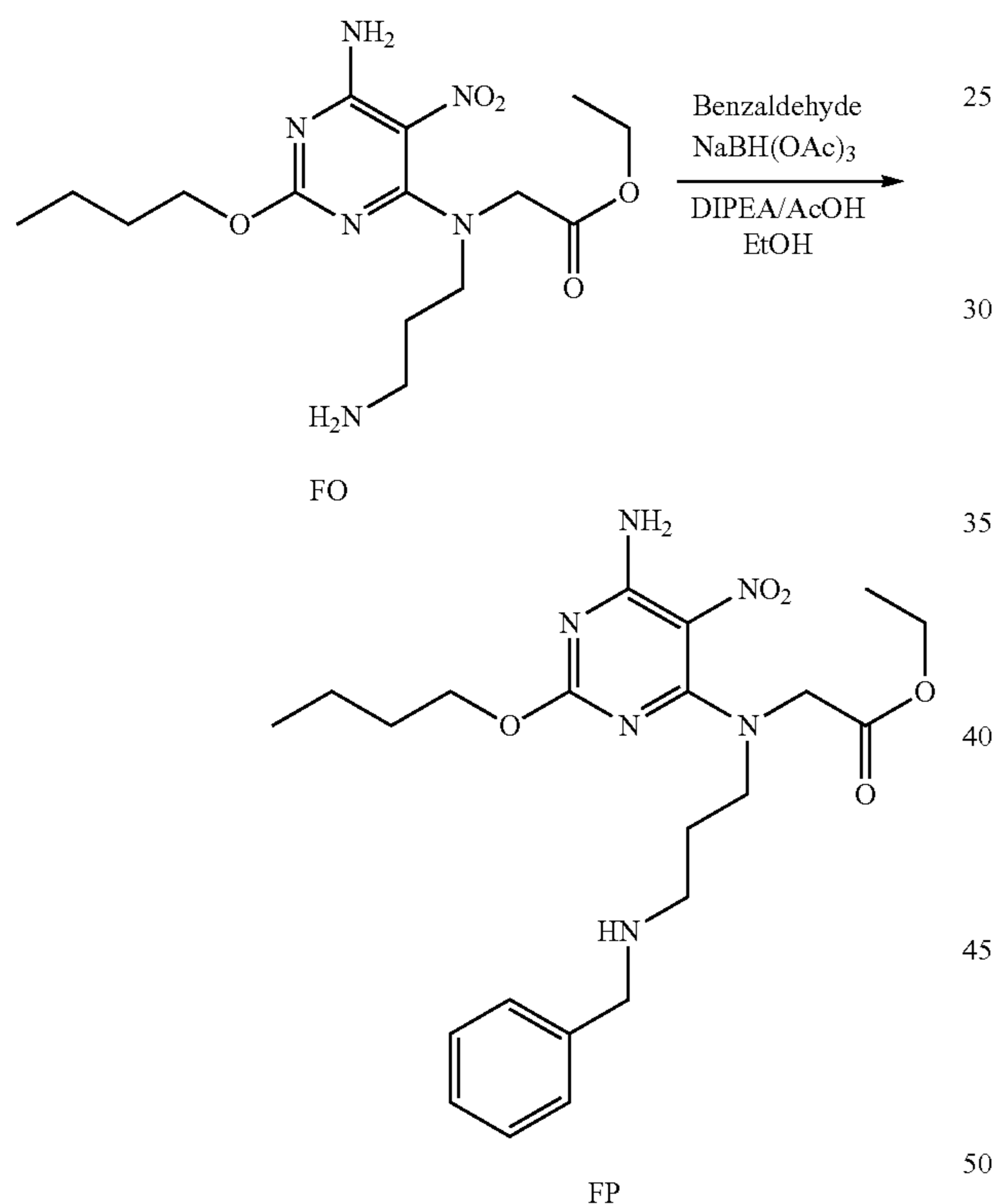
Scheme 106:
