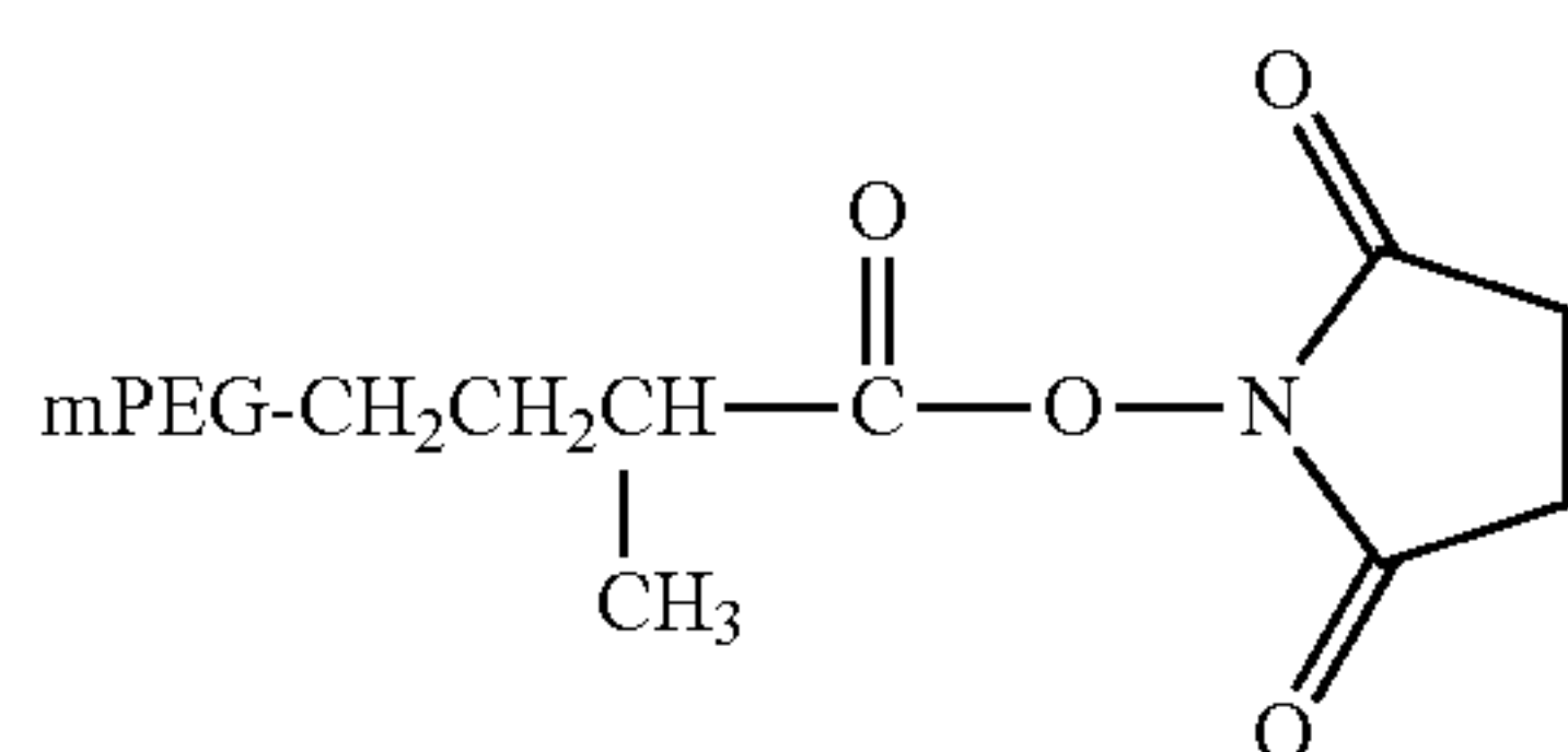
mPEG-Succinimidyl α-methylbutanoate (mPEG-SMB)
