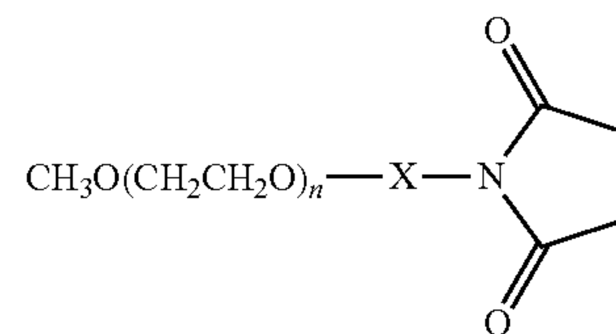
X = carboxymethyl
