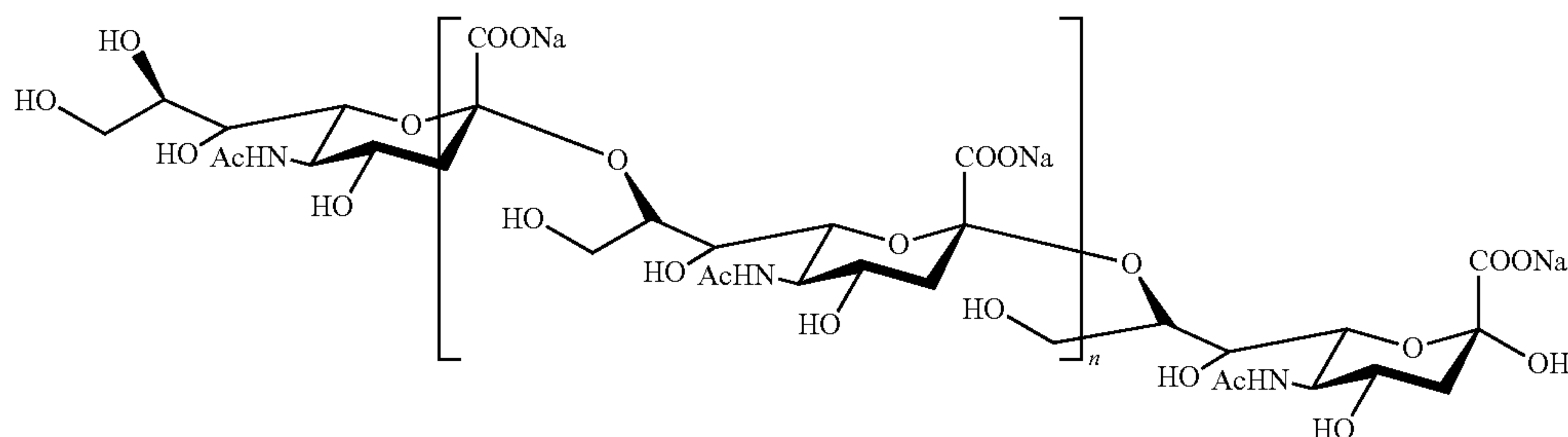
Structure of Colominic Acid (Homopolymer of N-Acetylneuraminic Acid)
