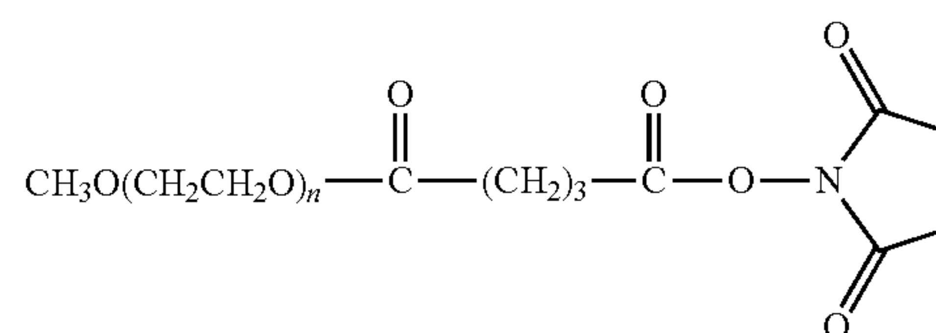
mPEG Succinimidyl glutarate
