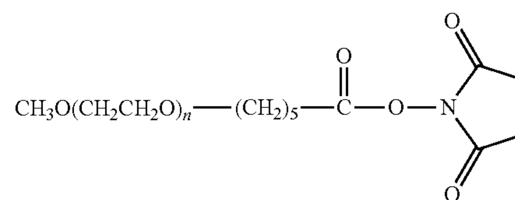
x = succinate
