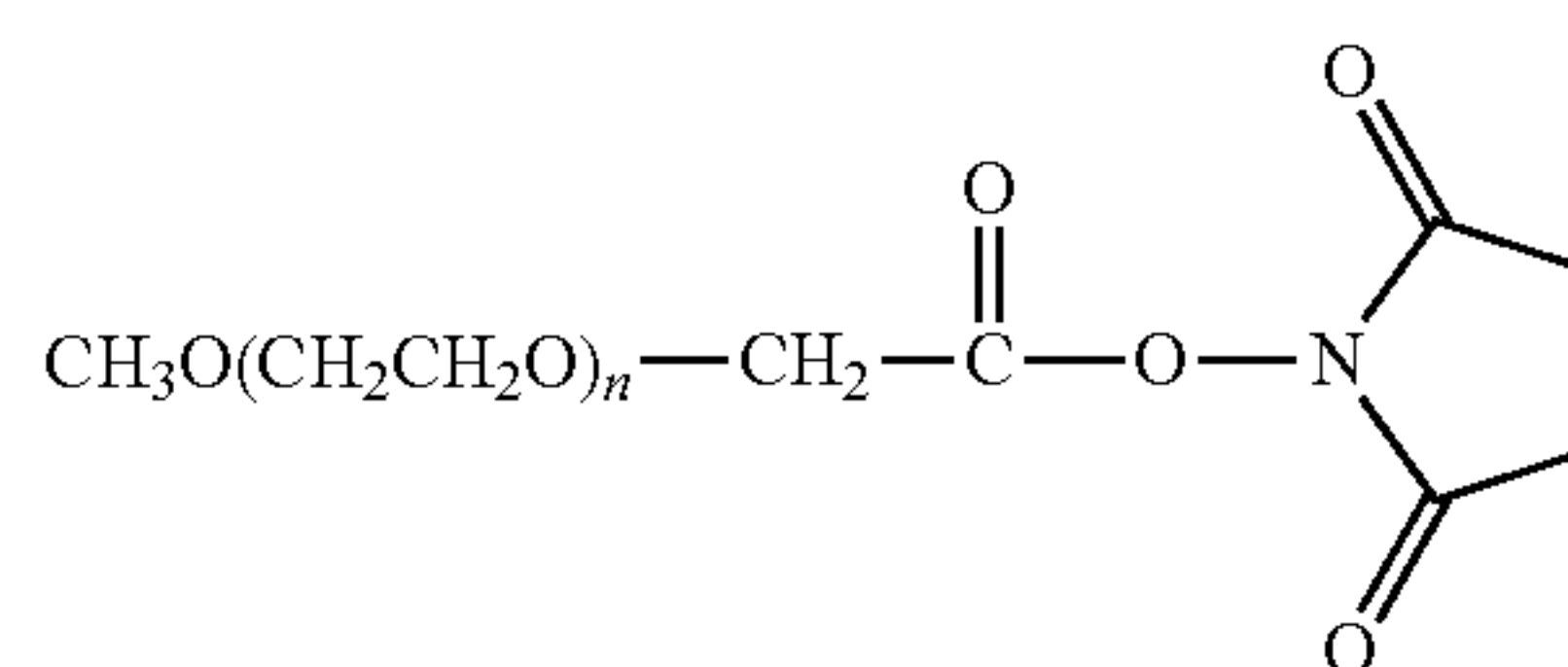
X = carboxypentyl
