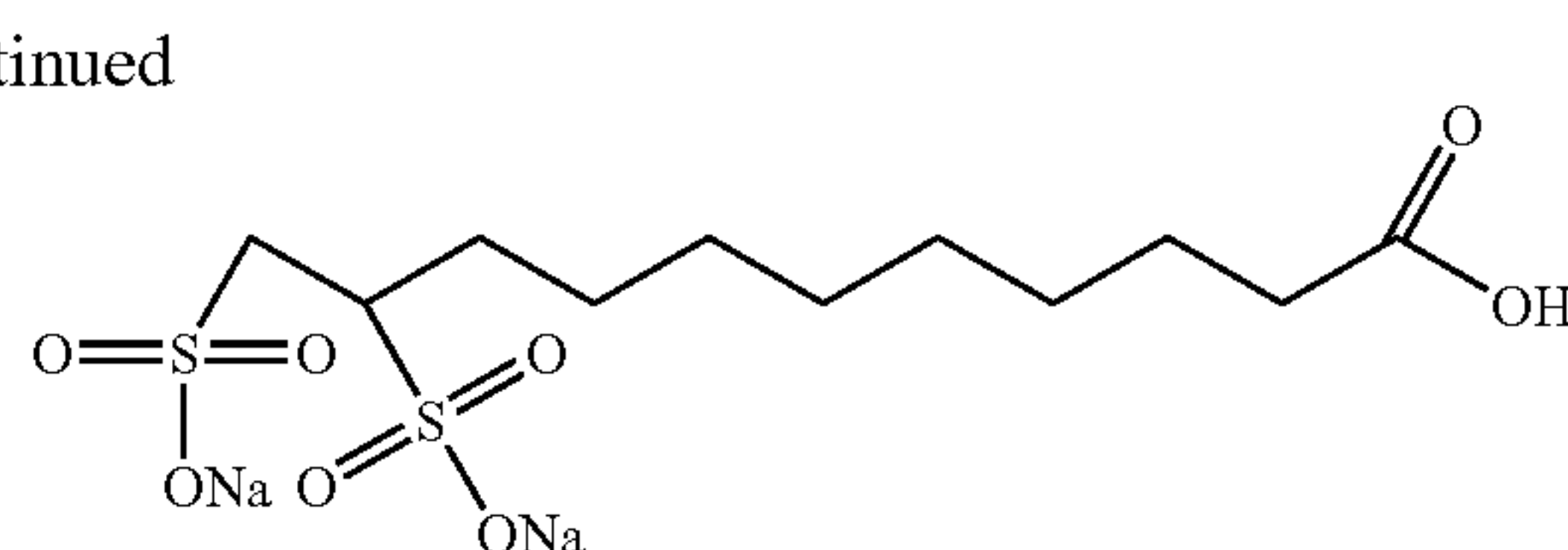
10, 11-Disulfofoundecanoic acid
