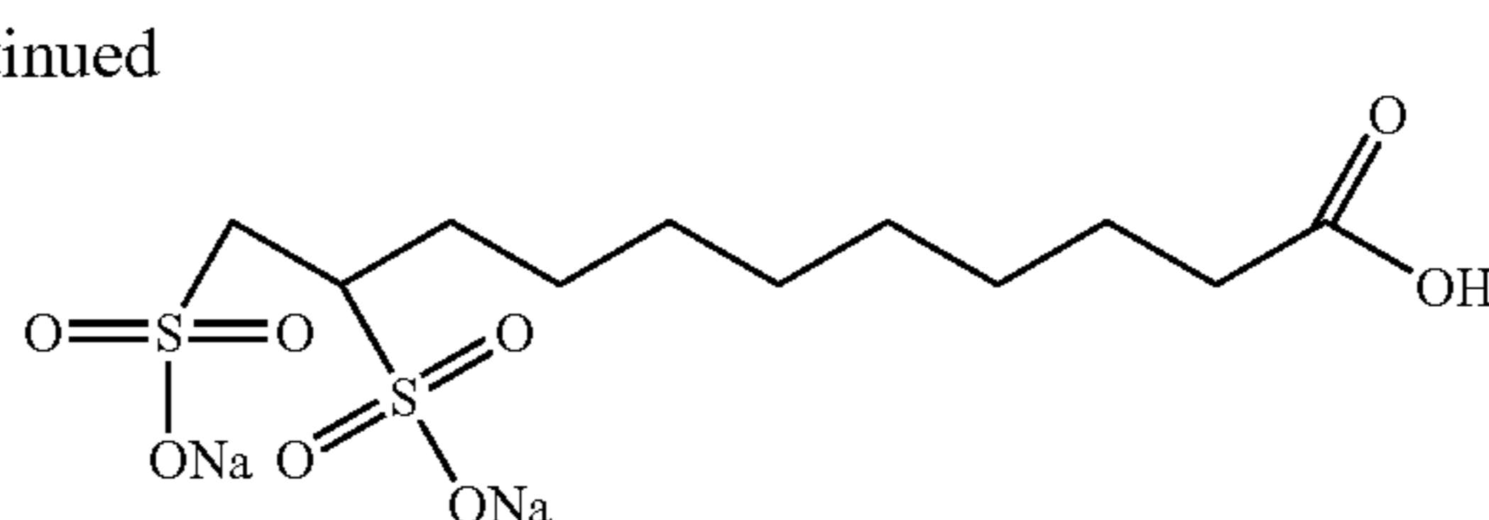
10, 11-Disulfoundecanoic acid
