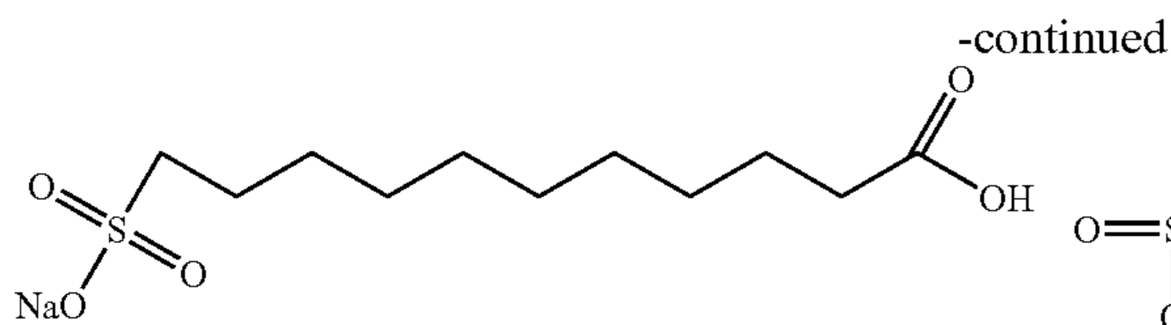
11-Sulfoundecanoic acid
