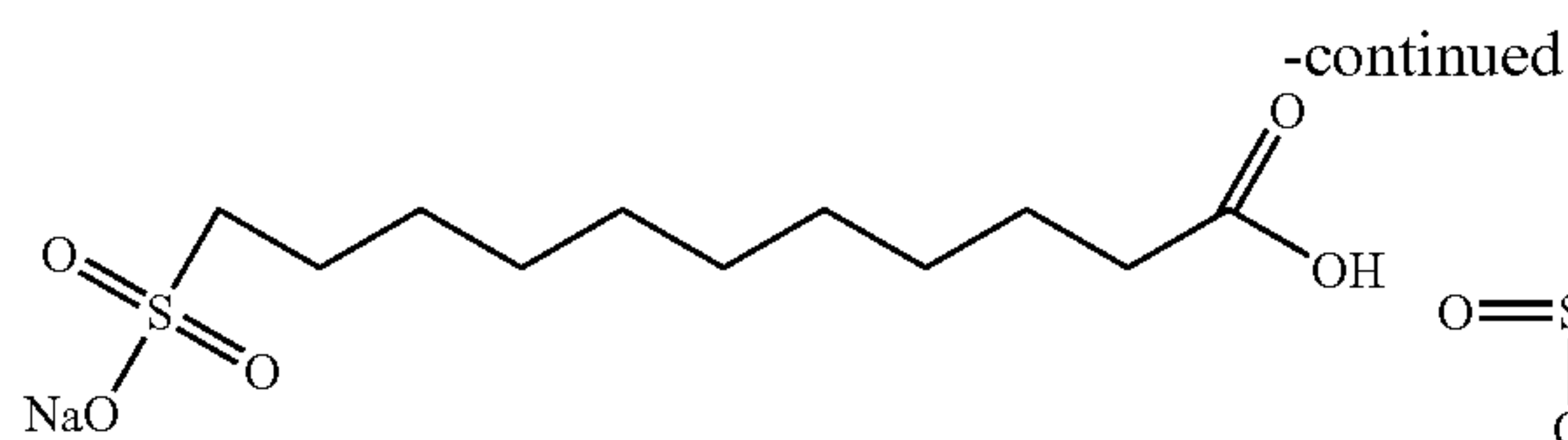
11-Sulfofoundecanoic acid
