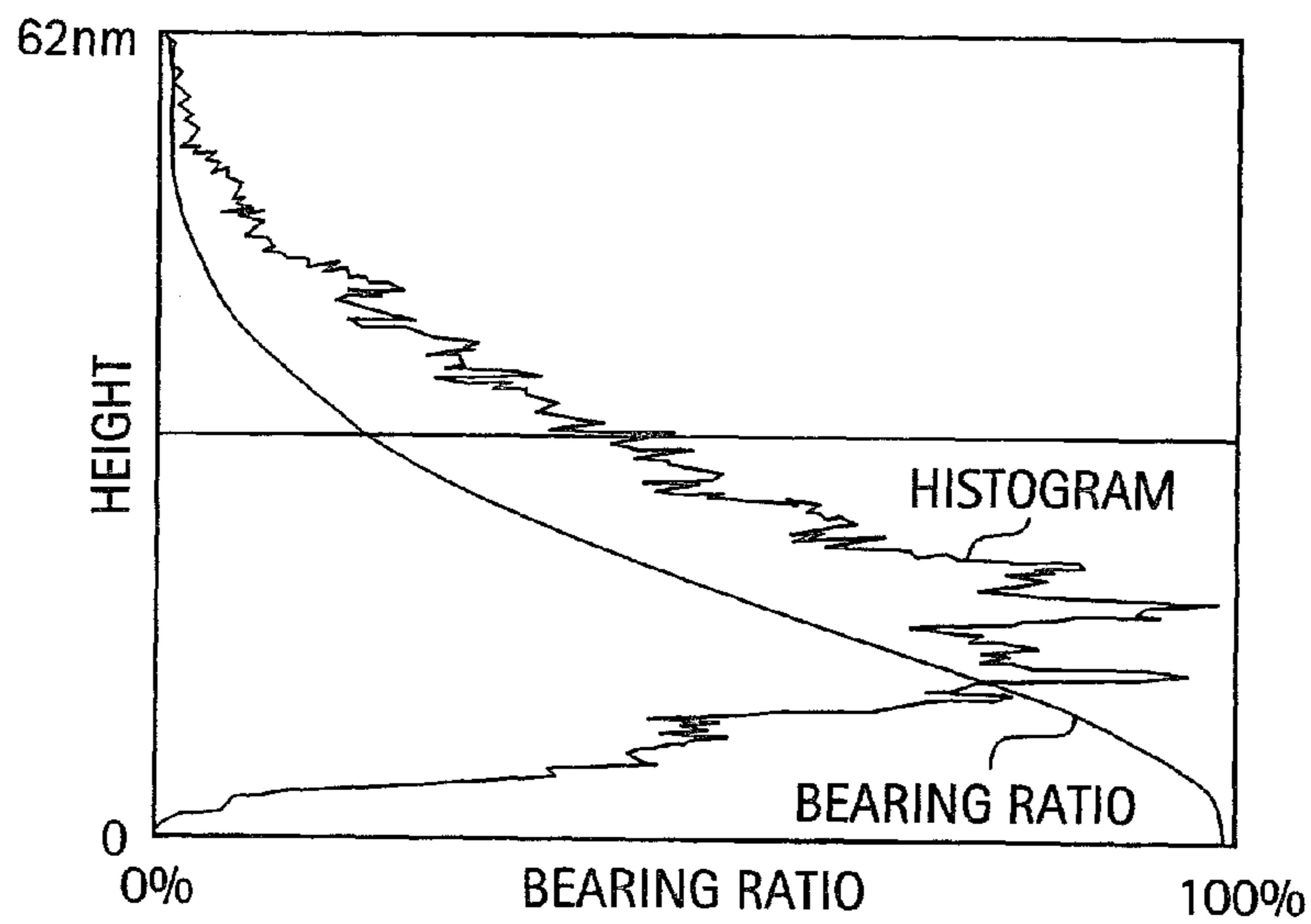
BEFORE HIGH TEMPERATURE ANNEALING
