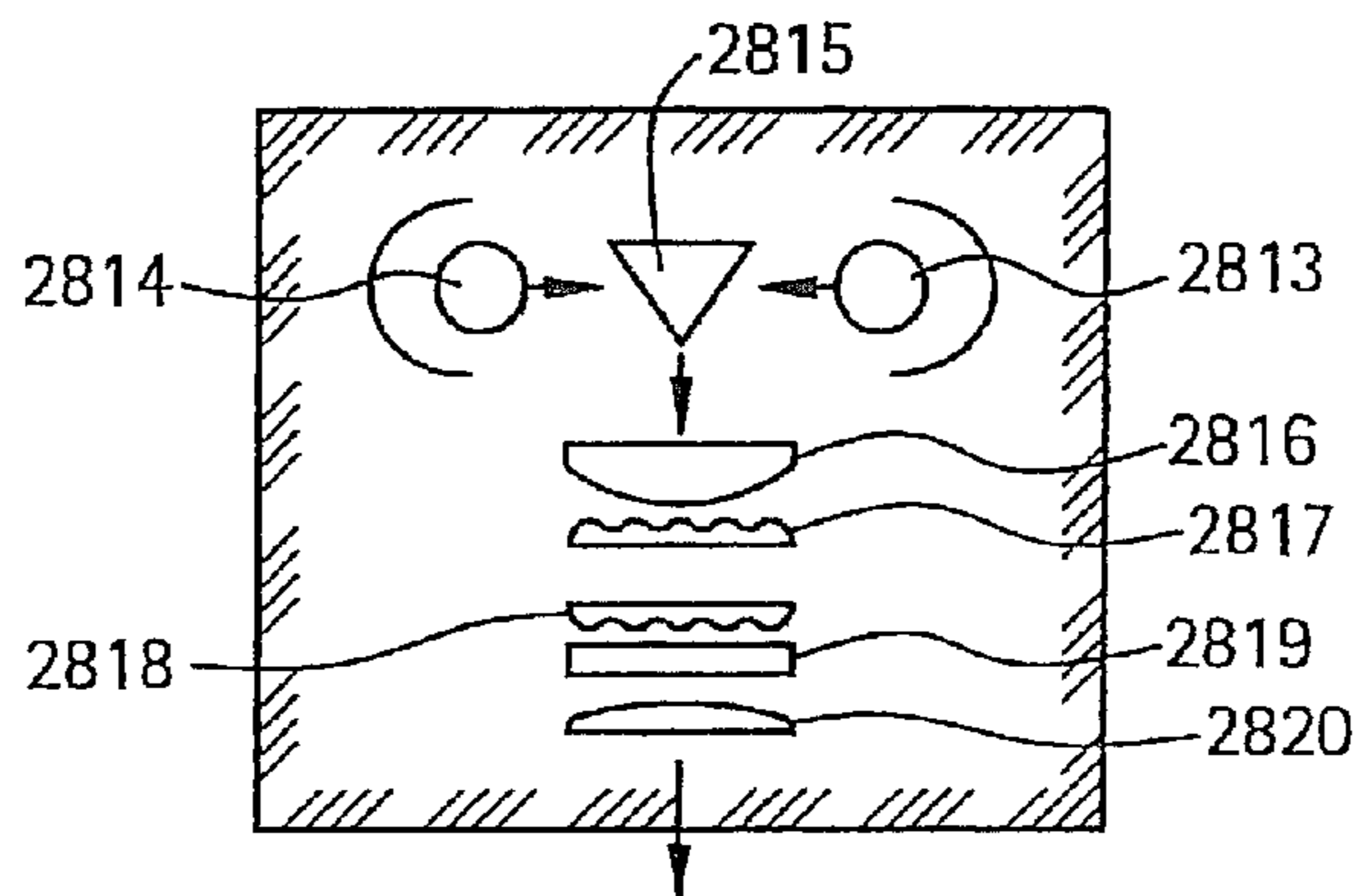
LIGHT SOURCE OPTICAL SYSTEM
