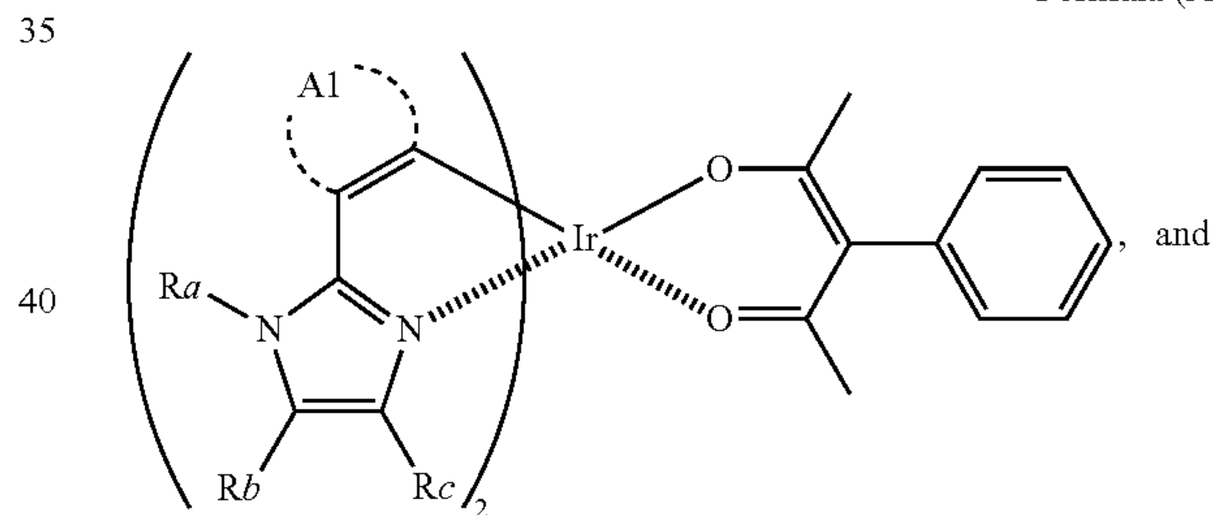
Formula (A-9)
