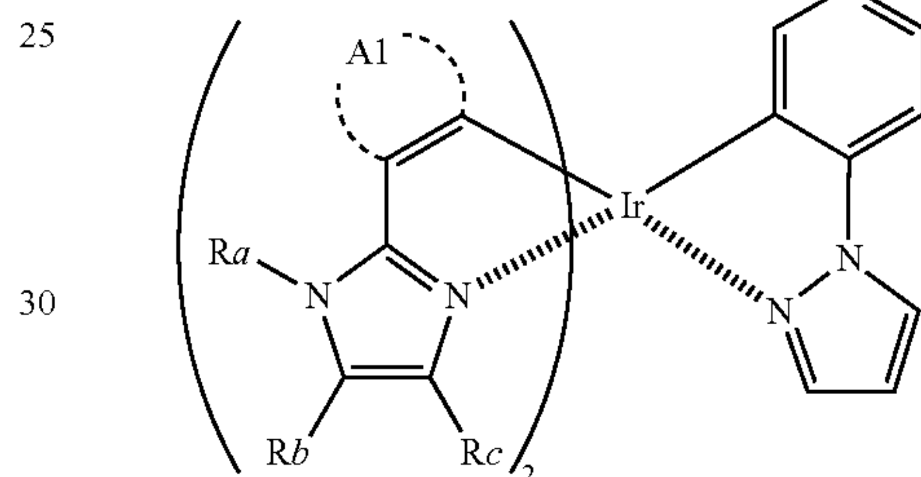
Formula (A-1)
