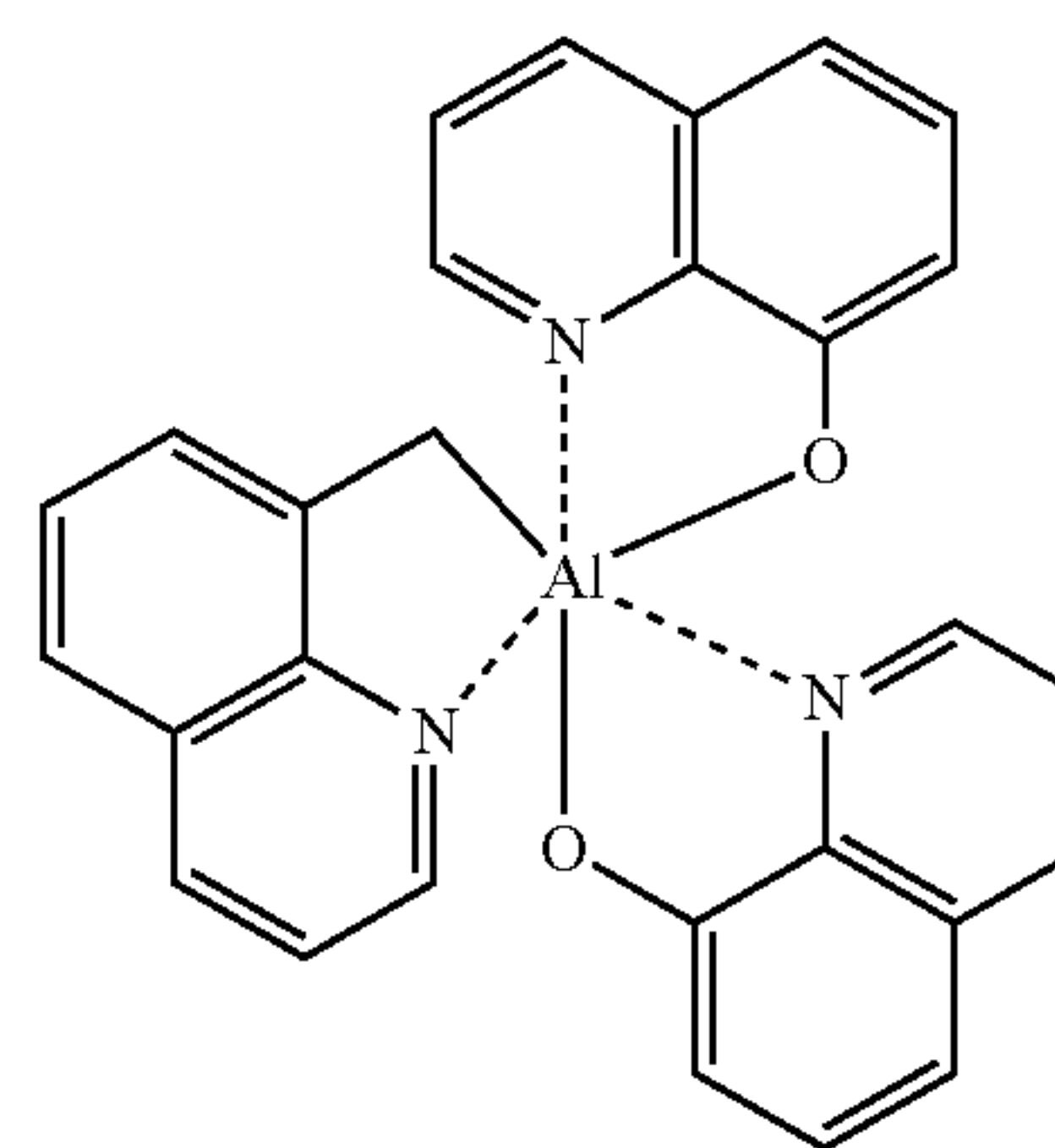
\text{Alq}_3
