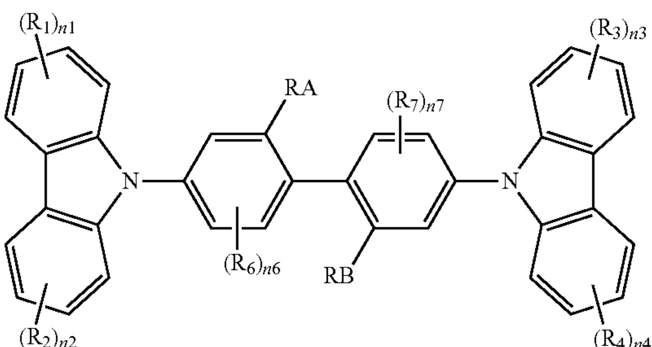
Formula (3)
