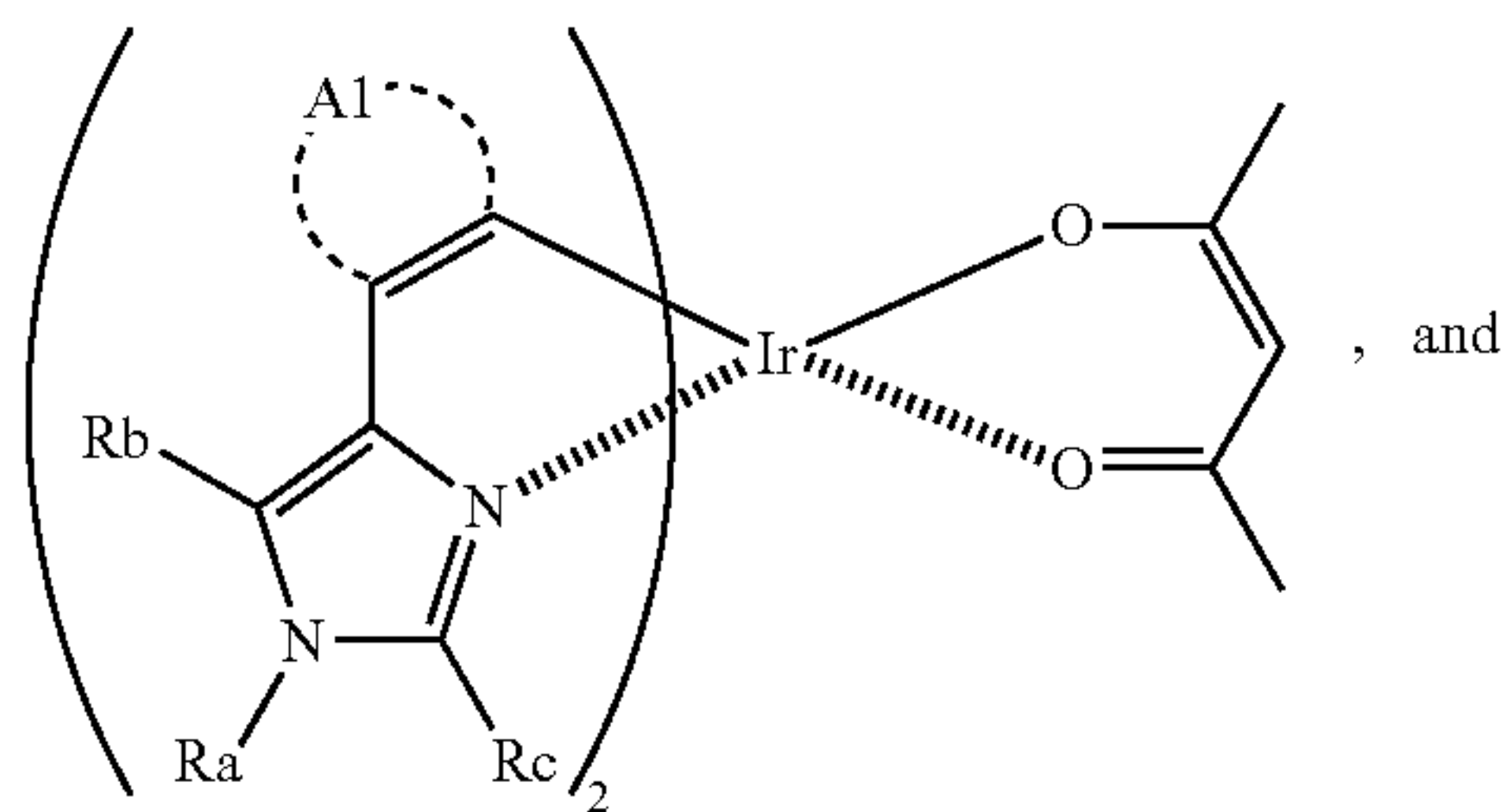
Formula (C-3)
