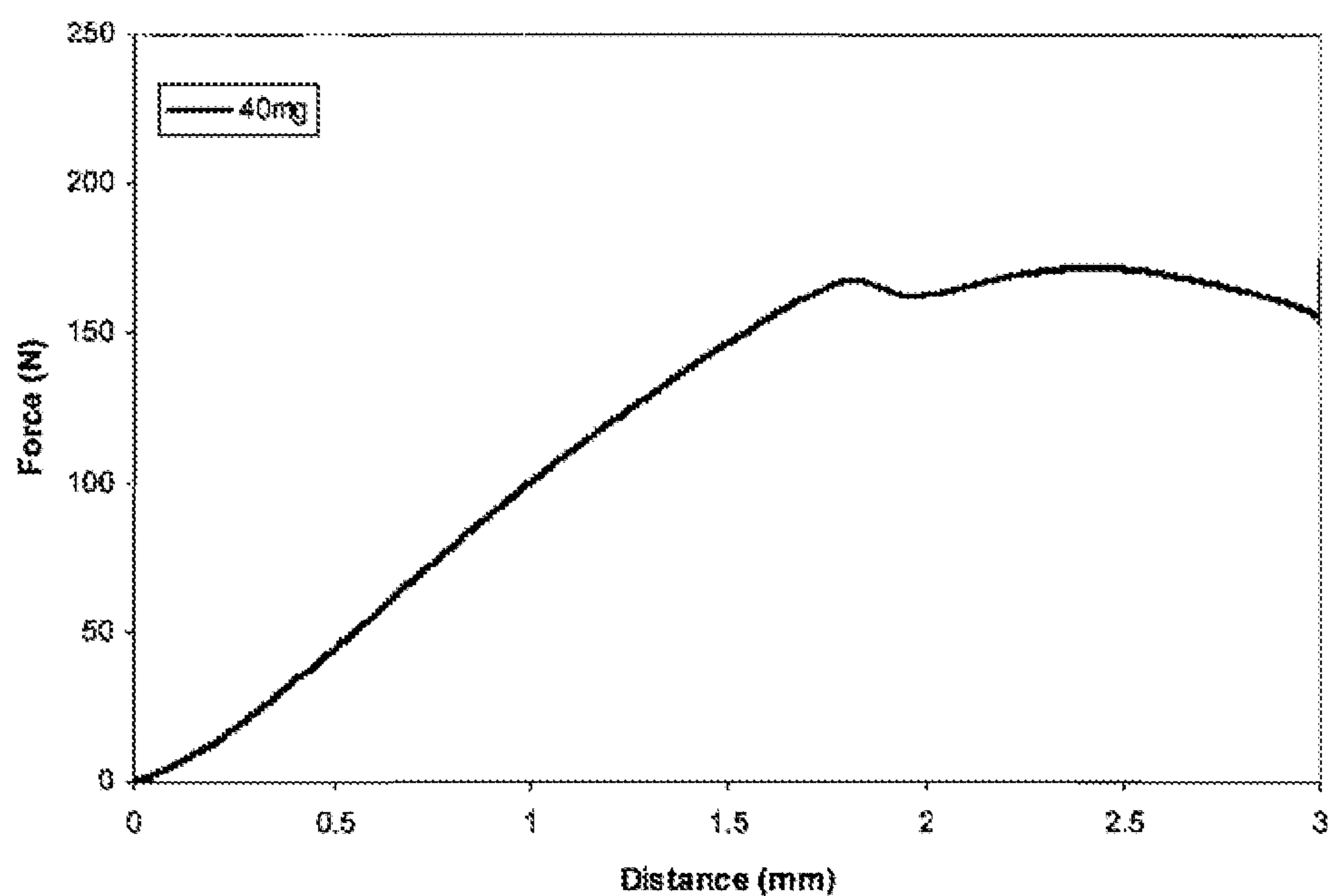
Example 20 Indentation Test of Example 13.5 tablet
