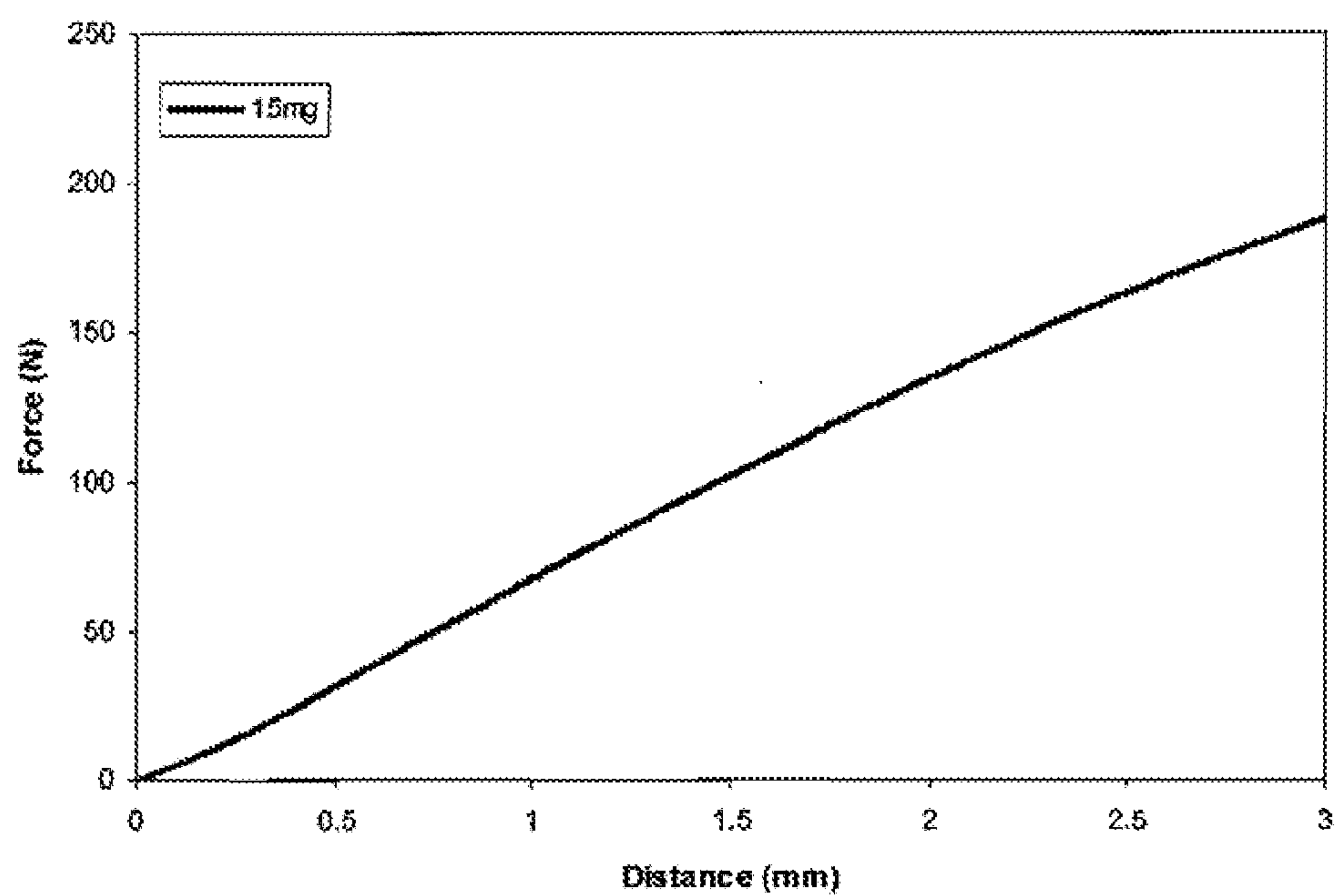
Example 20 Indentation Test of Example 13.2 tablet
