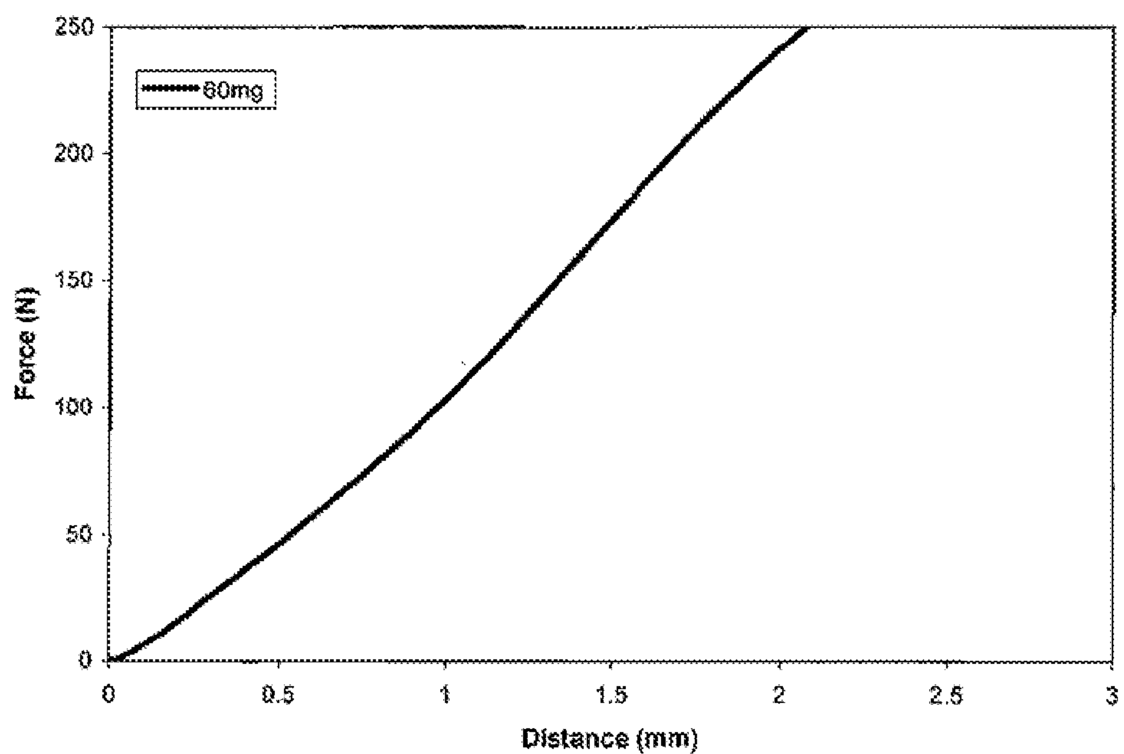
Example 20 Indentation Test of Example 17.1 tablet
