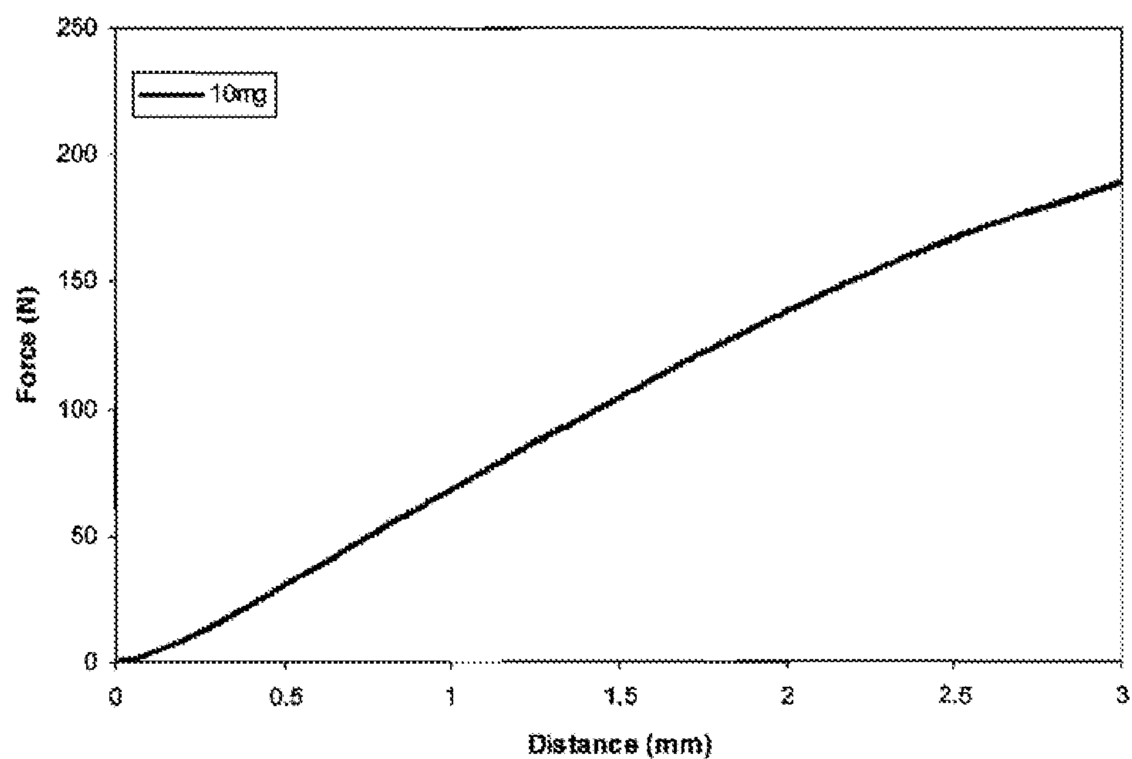
Example 20 Indentation Test of Example 13.1 tablet
