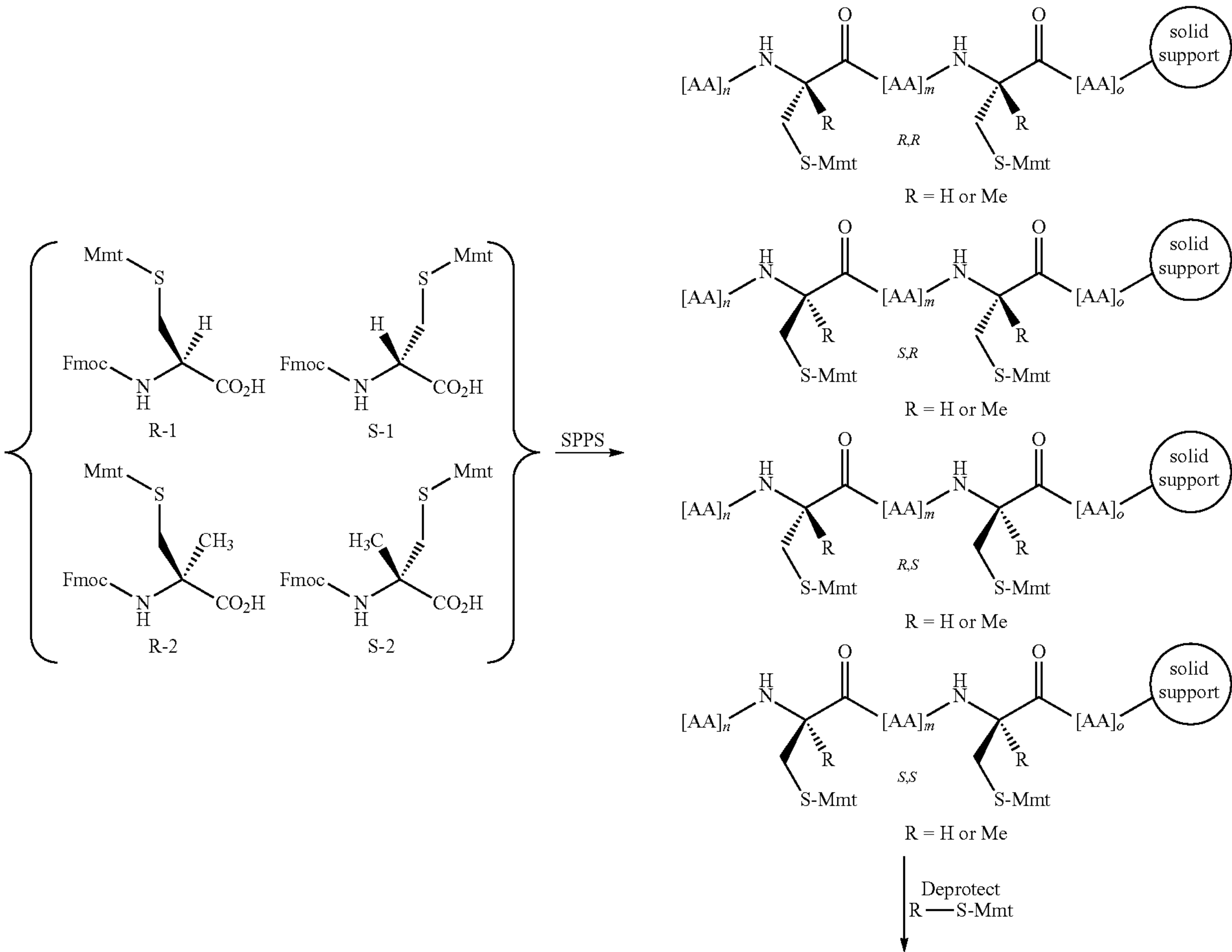
Synthetic Scheme 7:
