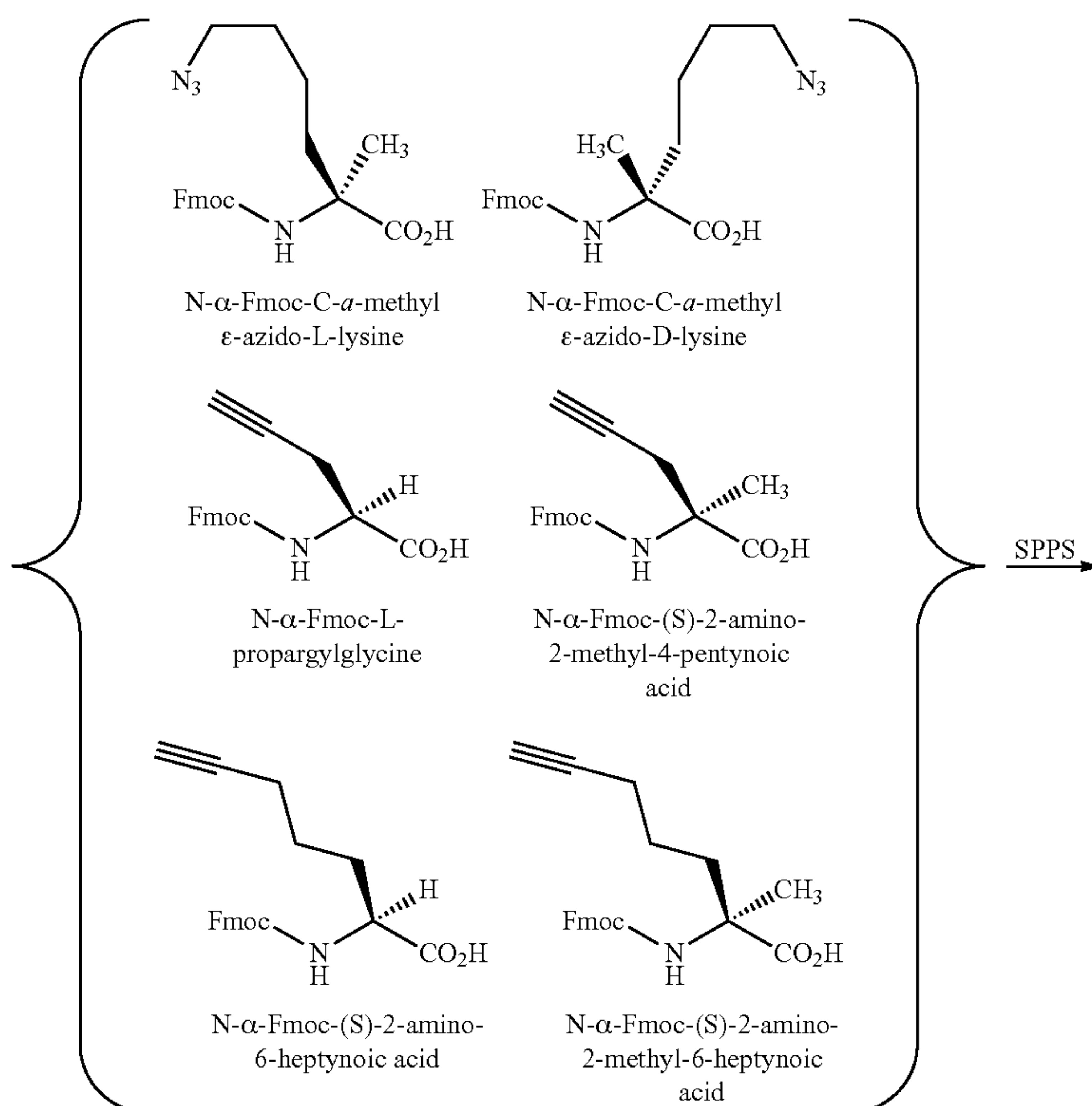
Synthetic Scheme 3:
