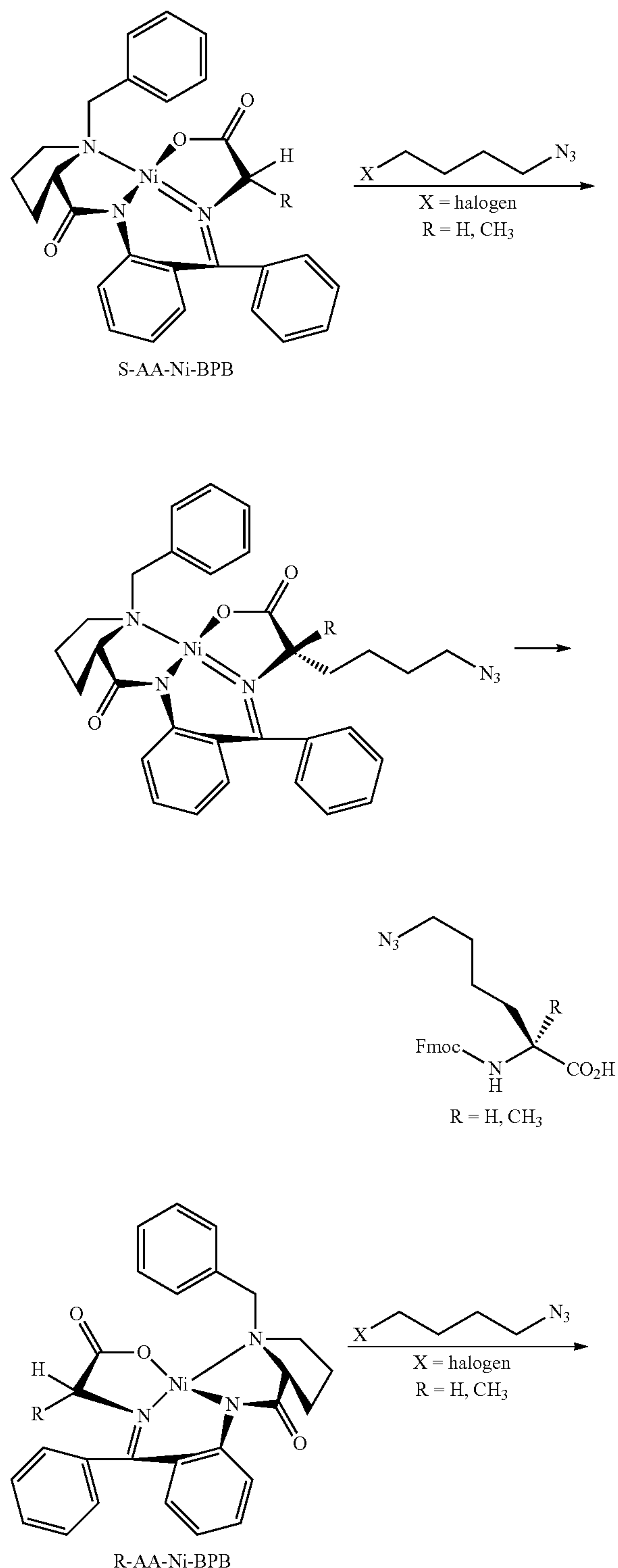
Synthetic Scheme 1:
