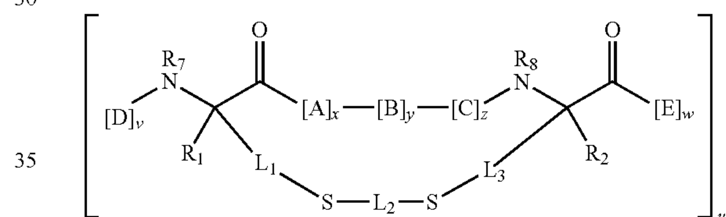
Formula (III)
