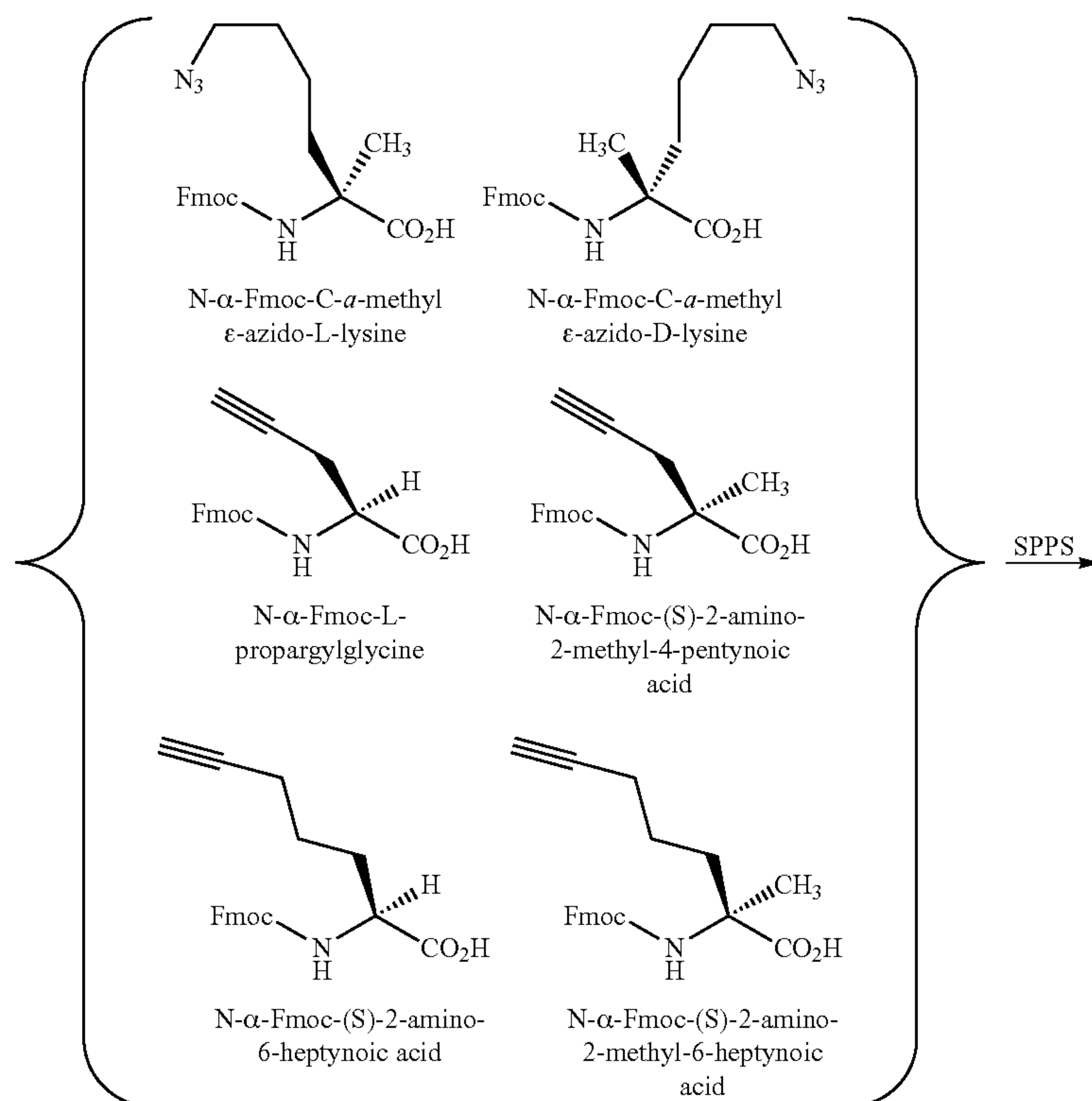
Synthetic Scheme 2:
