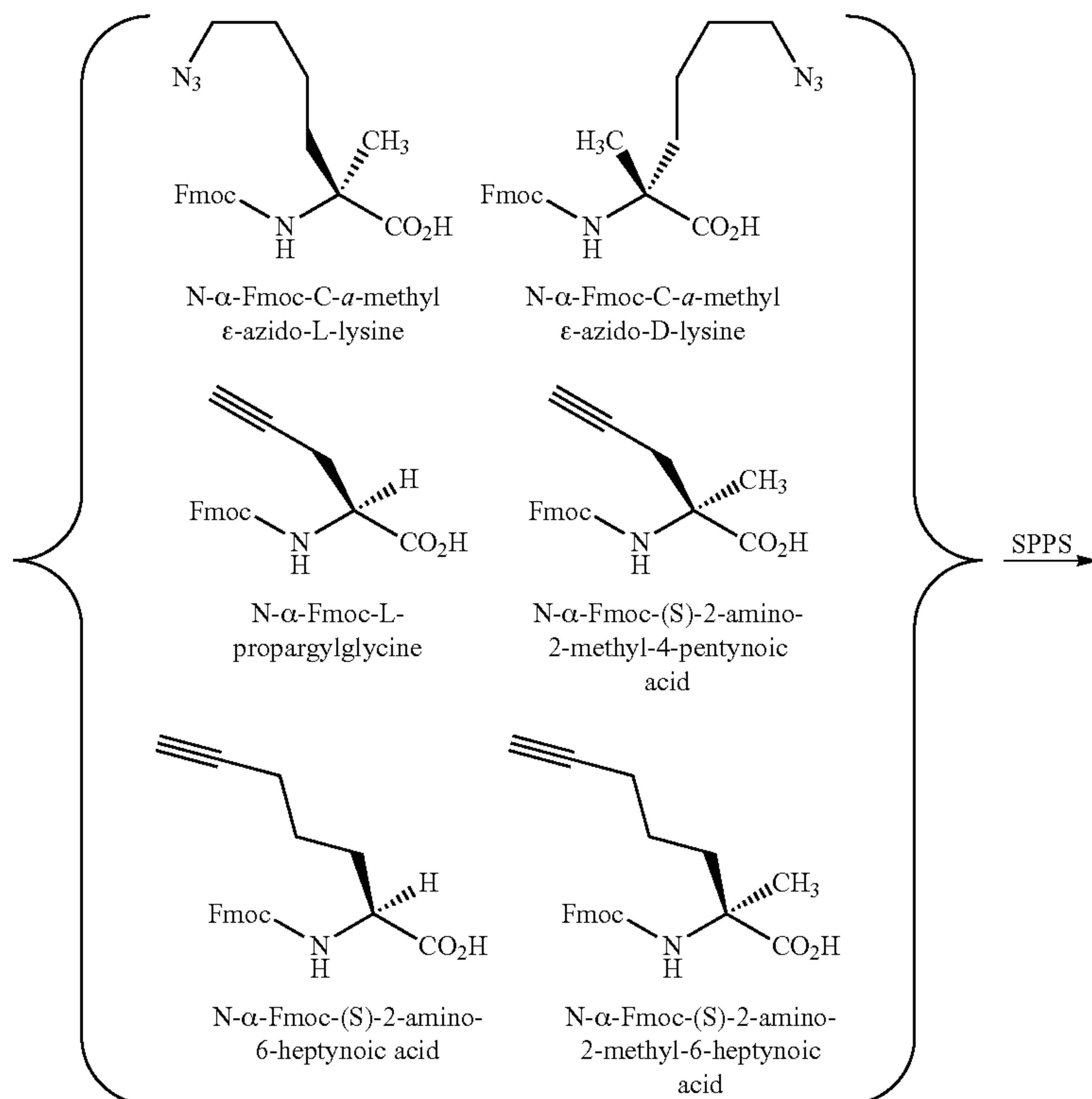
Synthetic Scheme 4:
