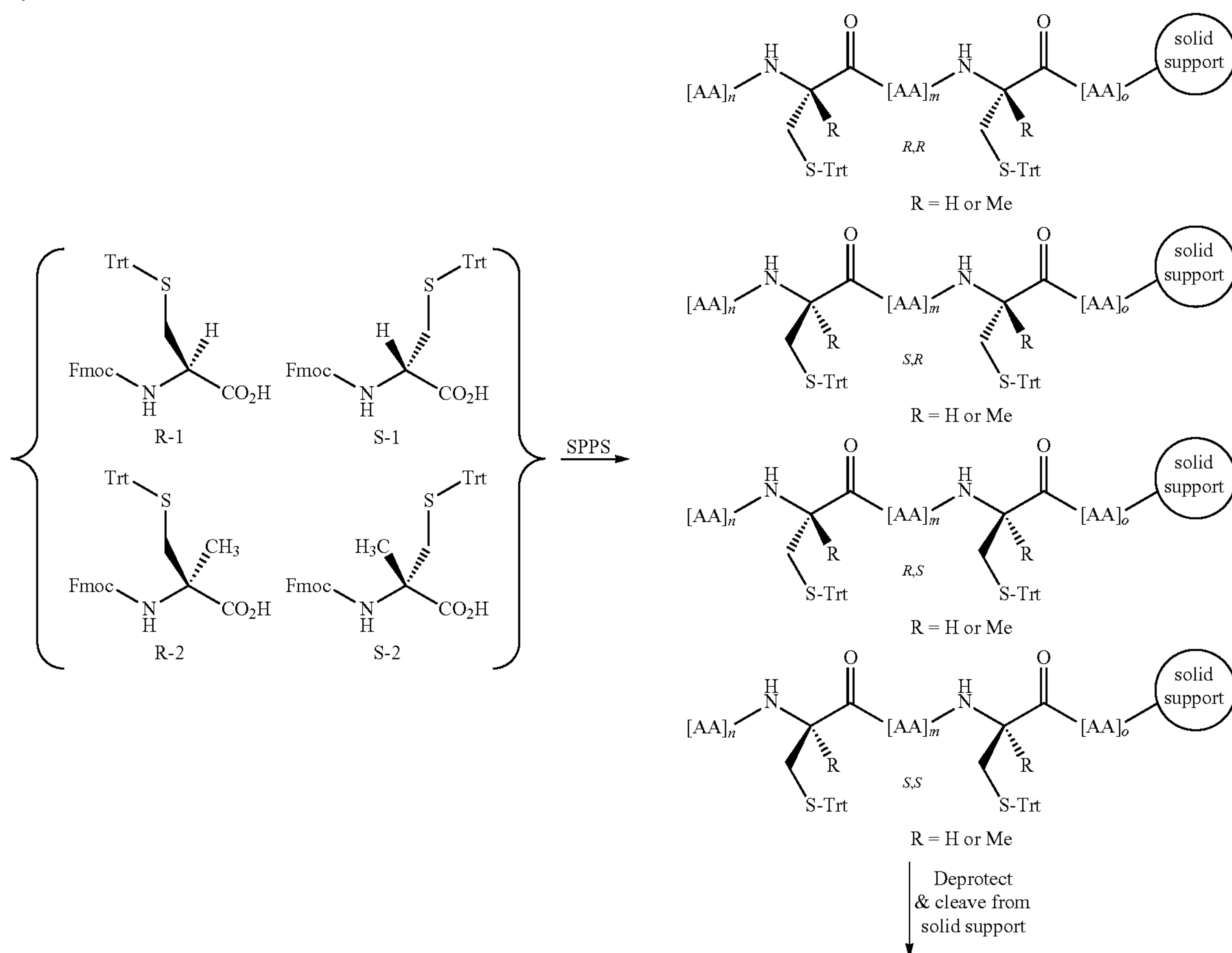
Synthetic Scheme 6:
