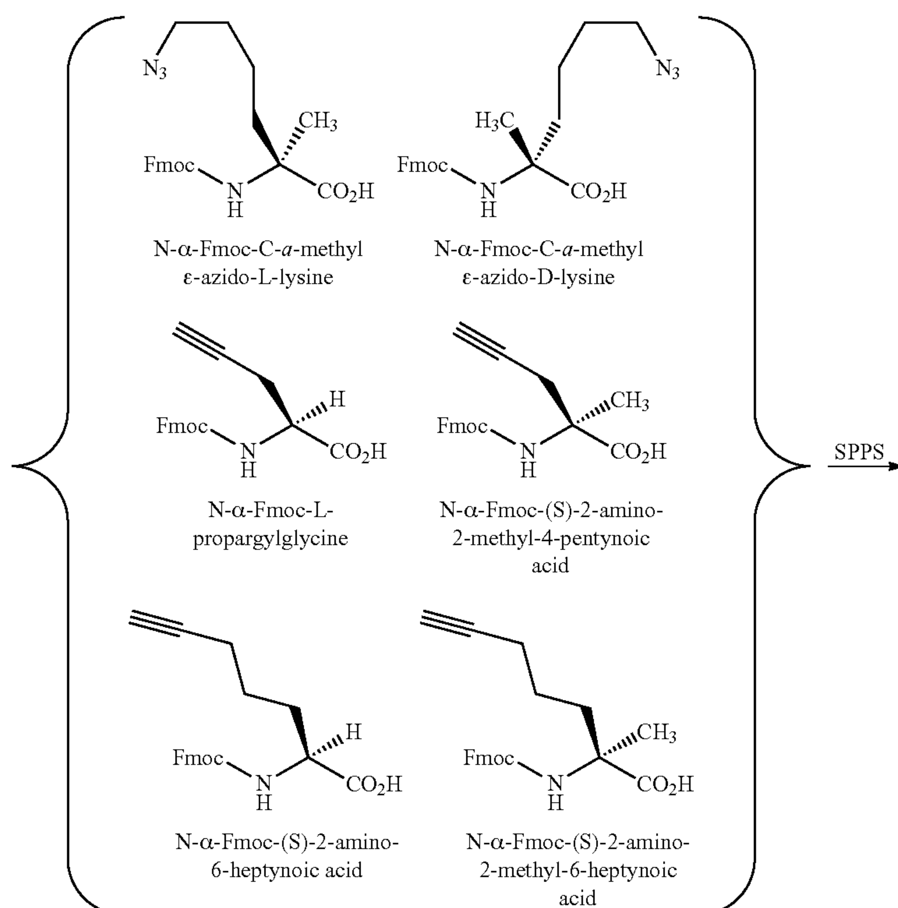
Synthetic Scheme 5:
