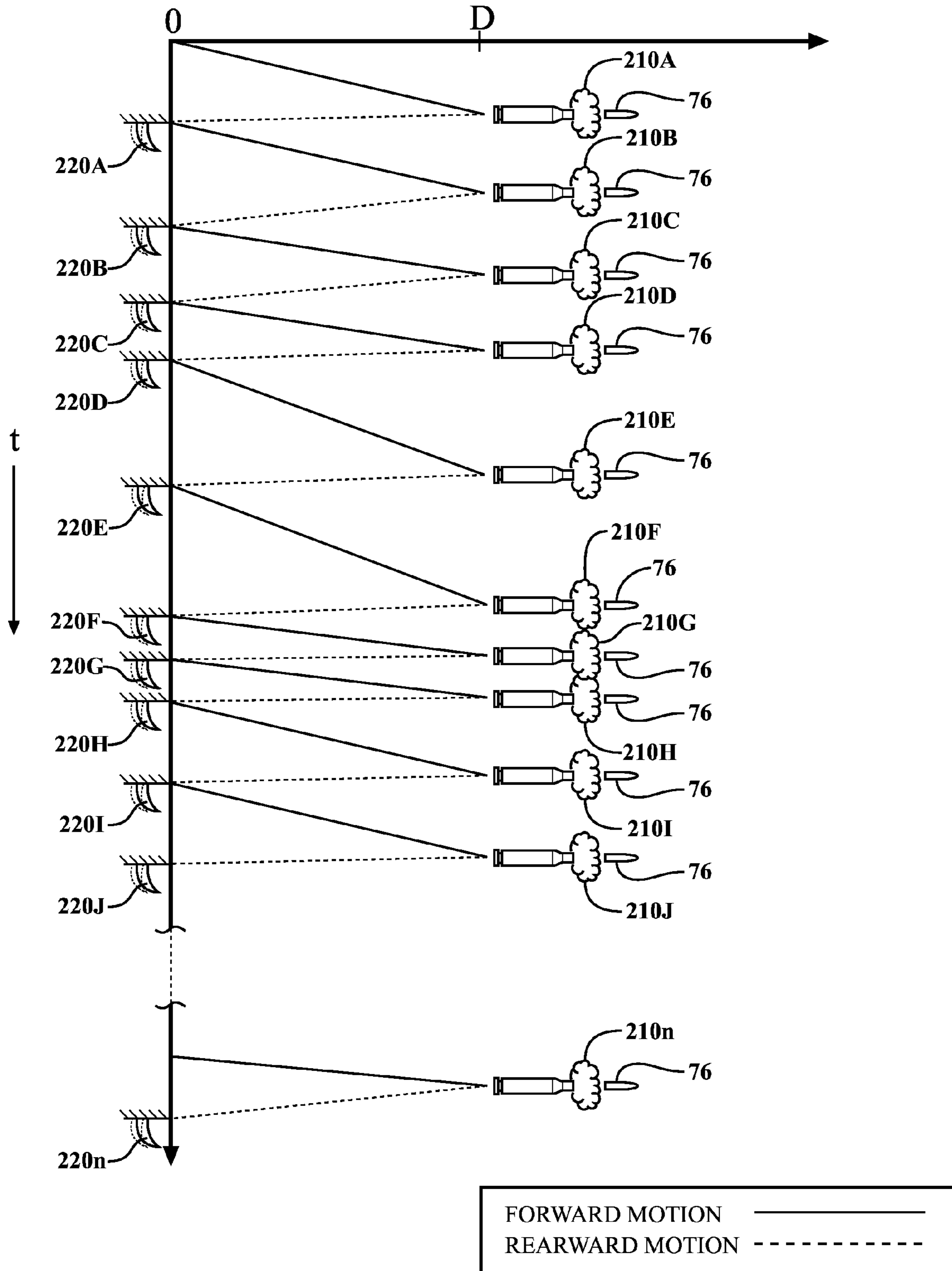
FIG. 27 FIRING UNIT DISPLACEMENT
