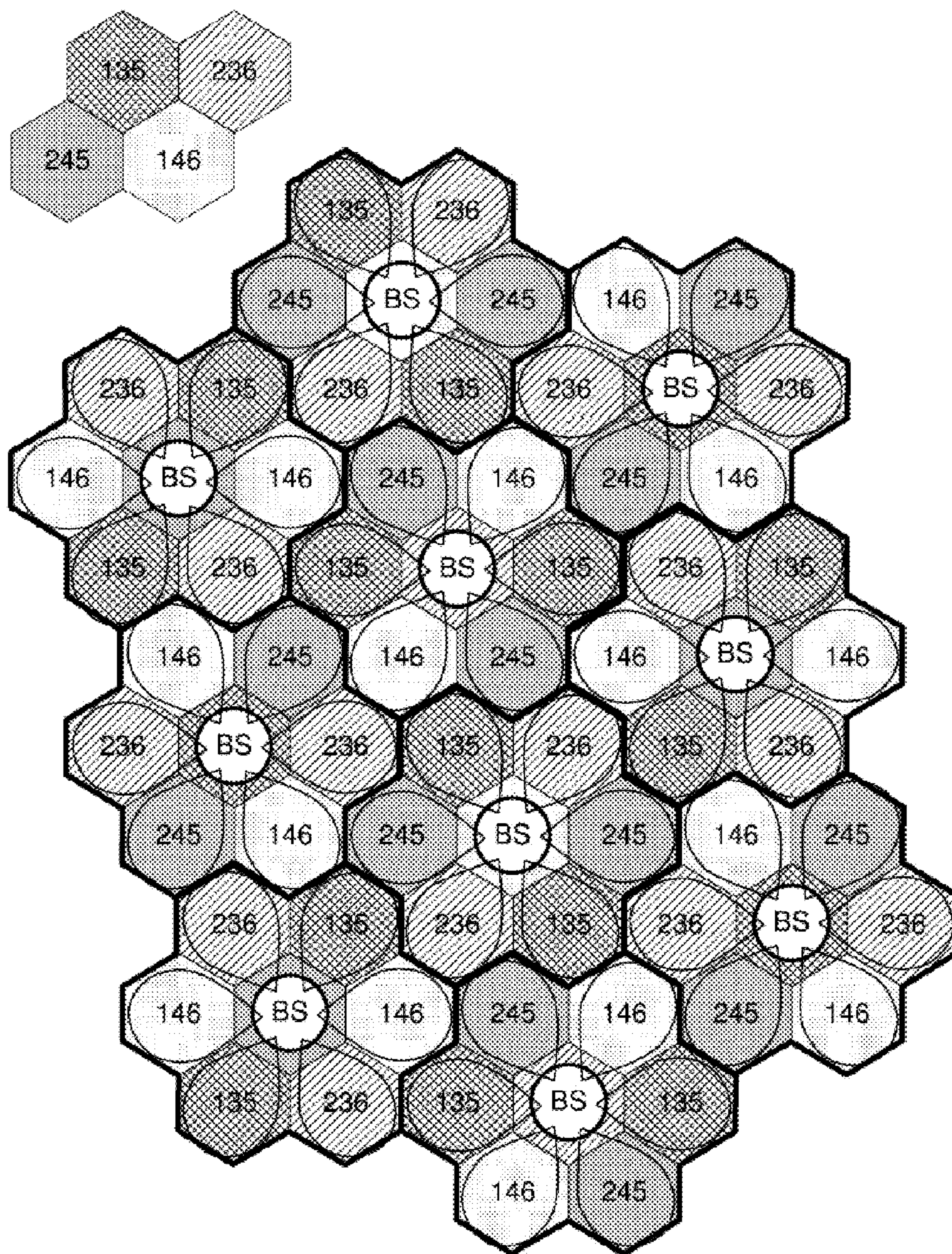
Figure 8 - Fractional Frequency Reuse 3 out of 6 resources in each sector Based on 1-2-1-2-1-2 coloring in three directions Applied to 6-sector deployment
