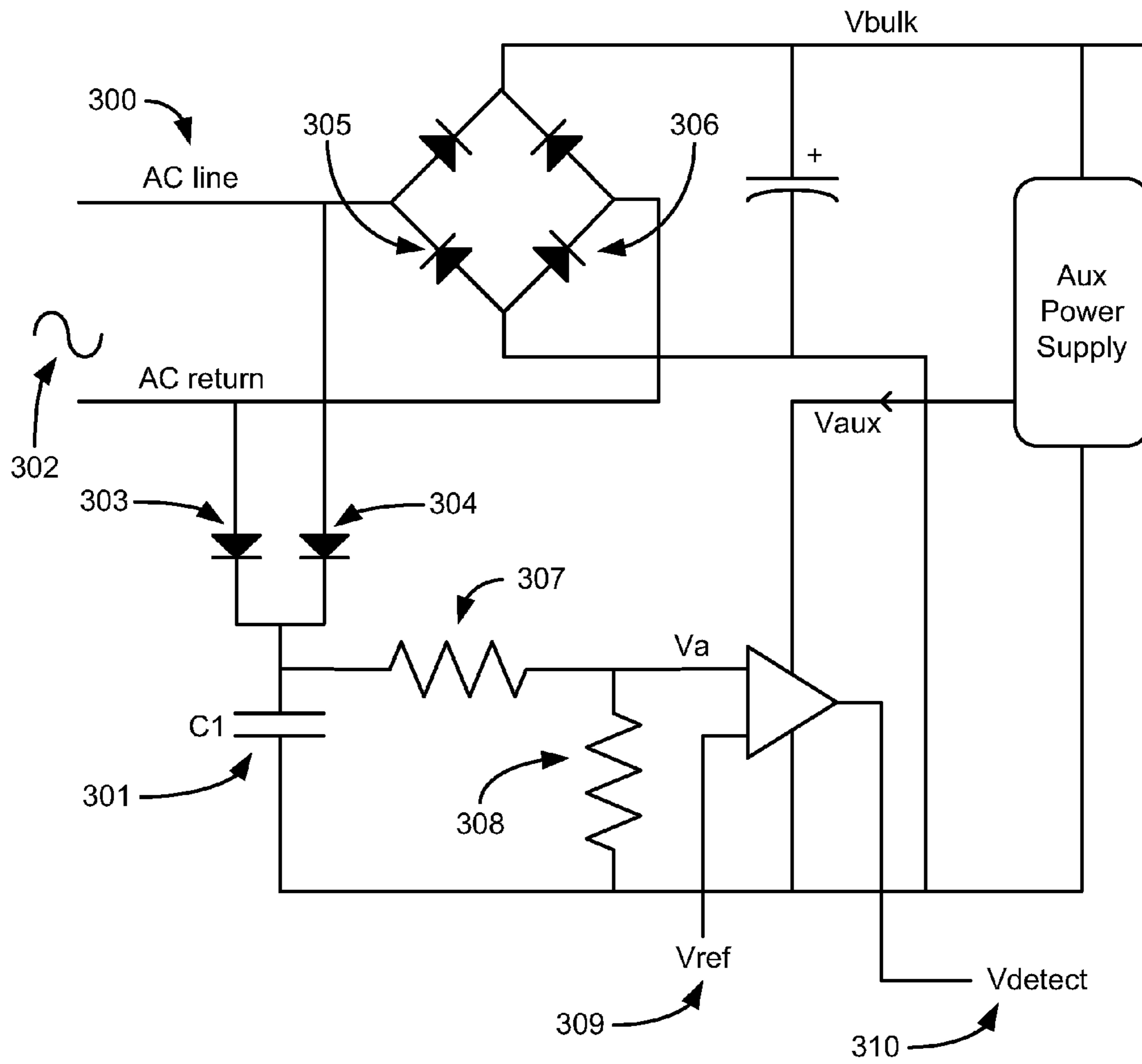
FIG. 8 Prior Art
