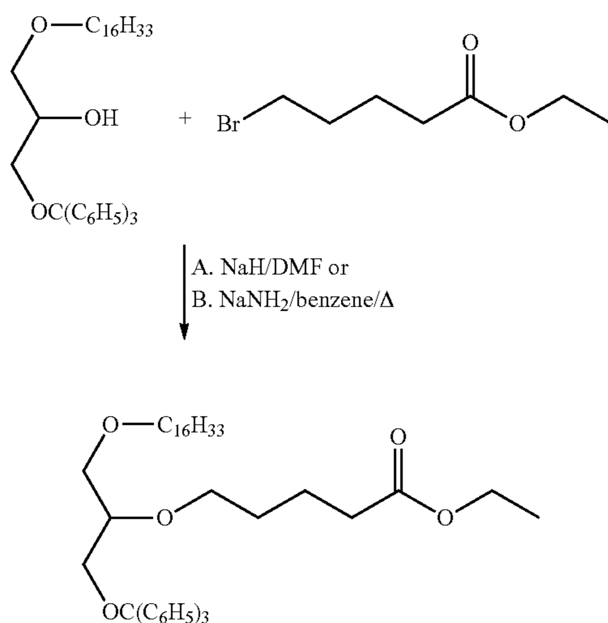
Scheme XI
