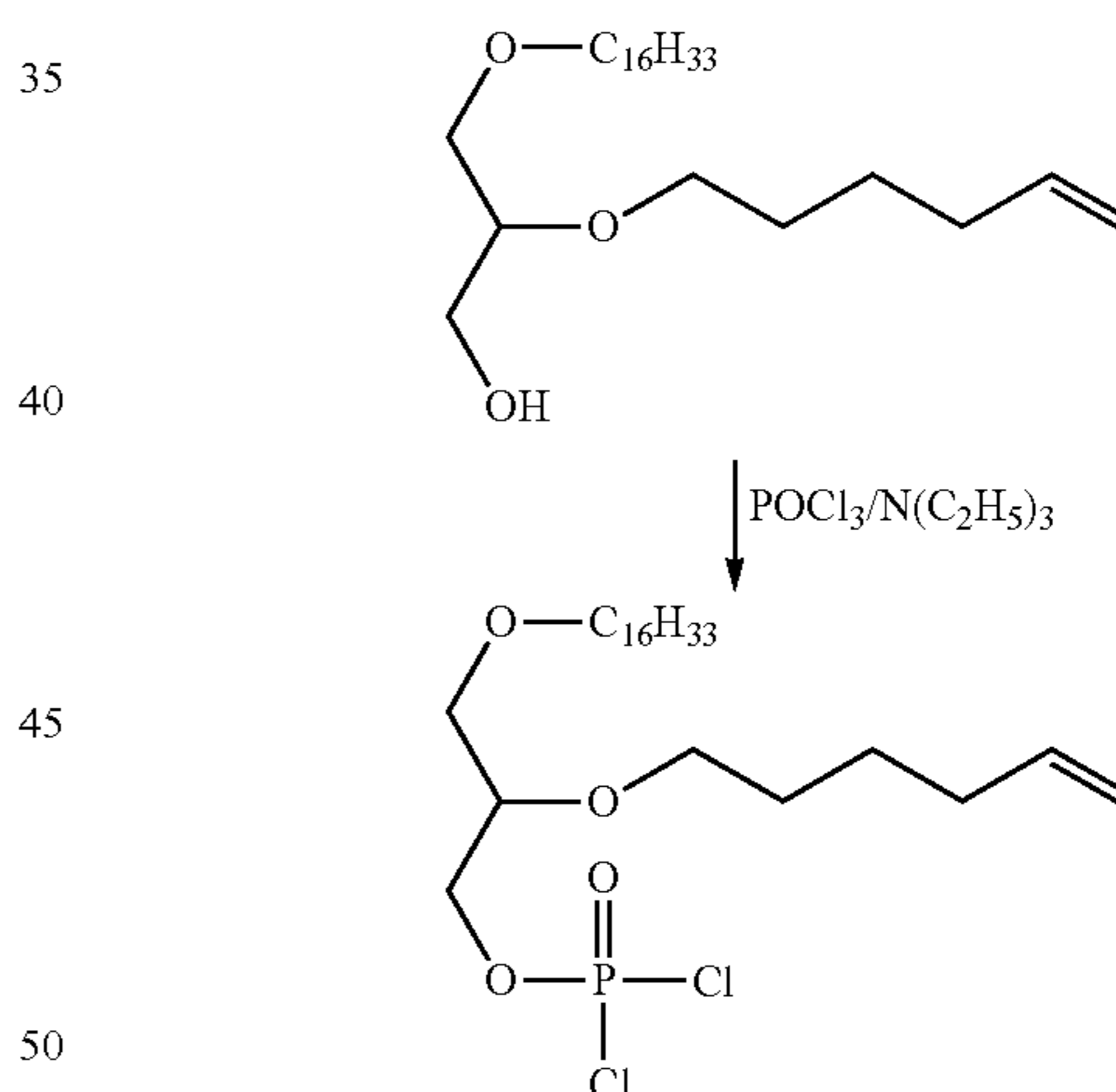
Scheme XII
