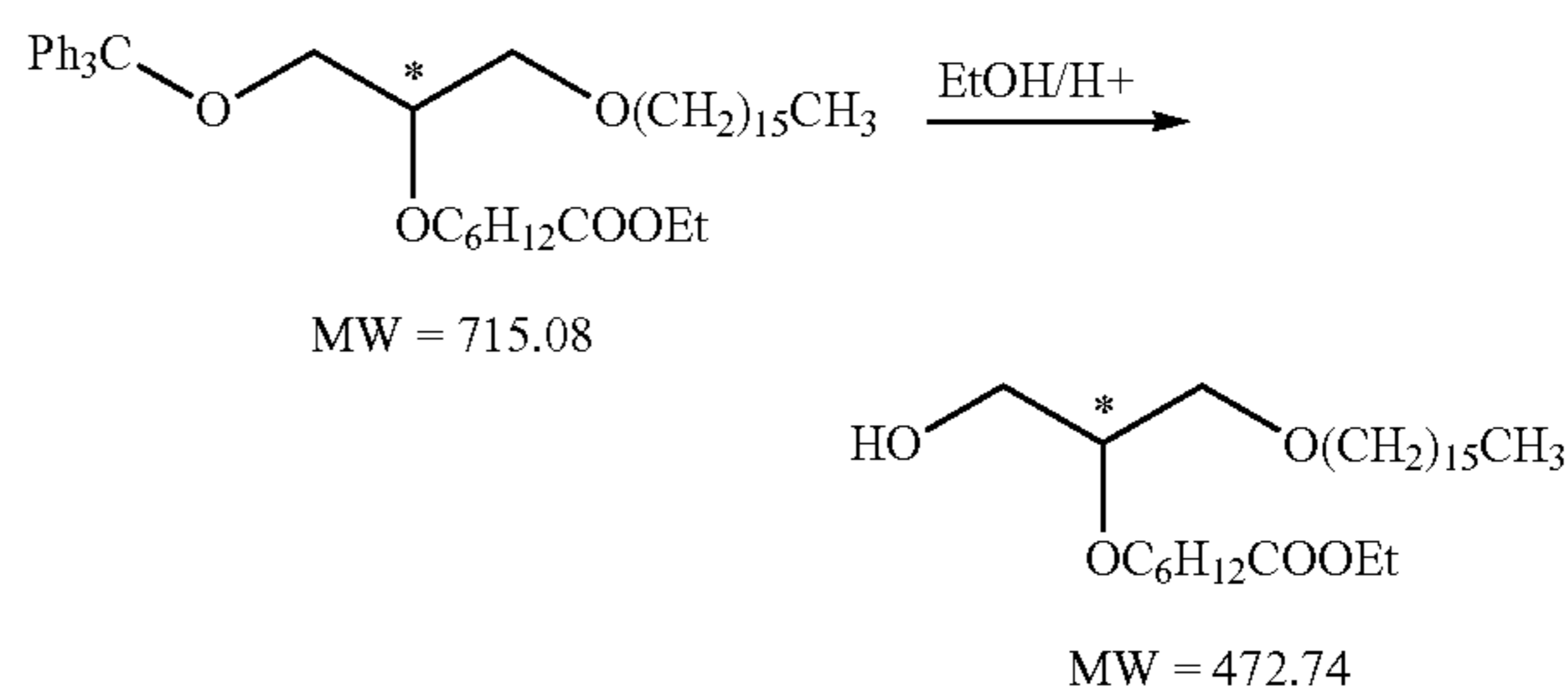
Scheme XVII
