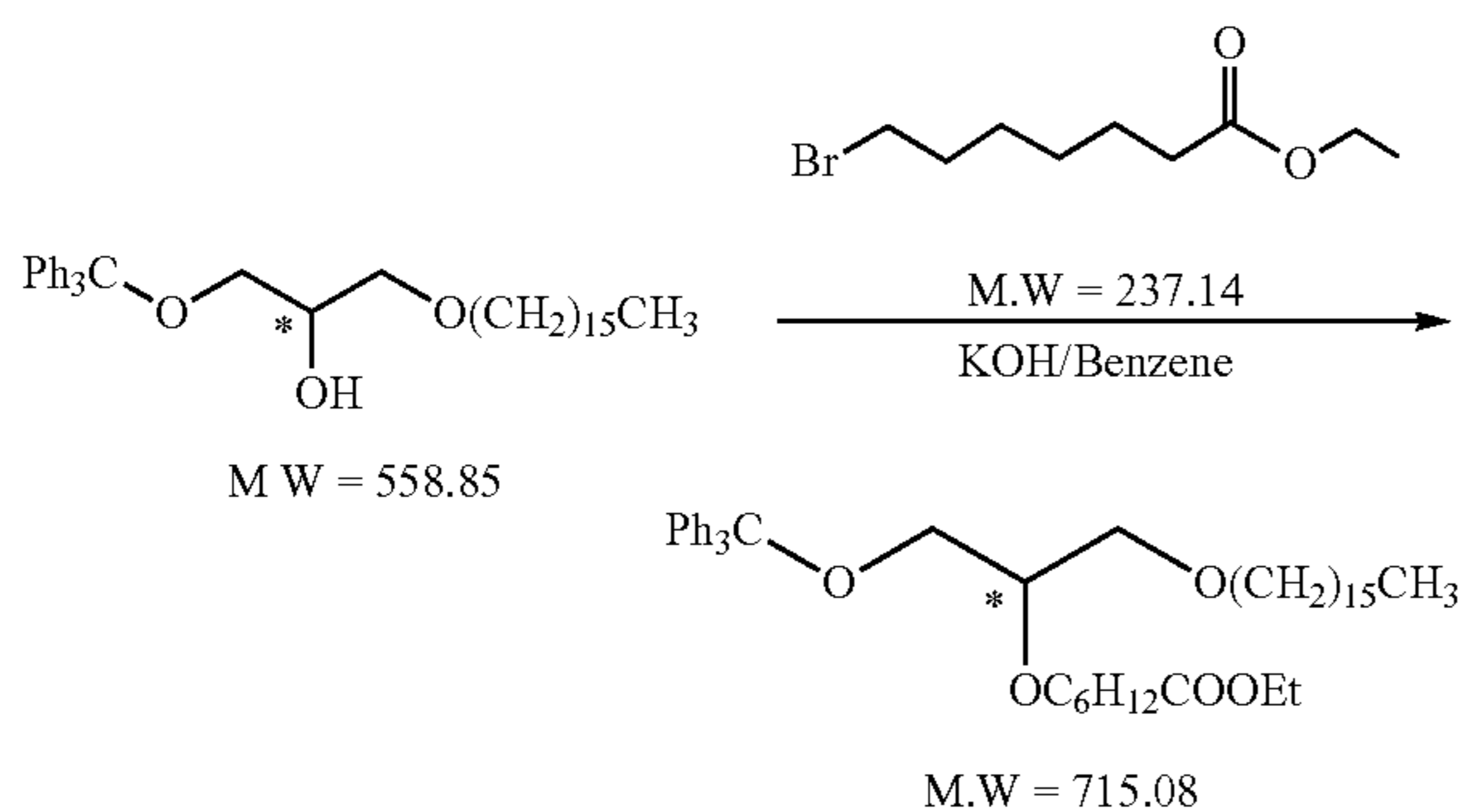
Scheme XVI
