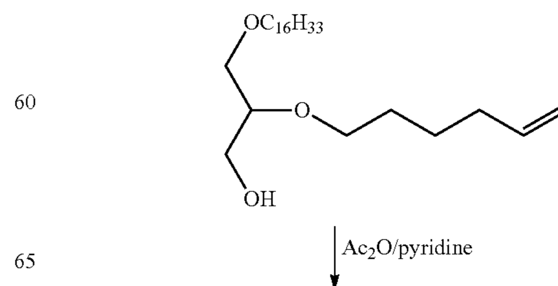
Scheme VII
