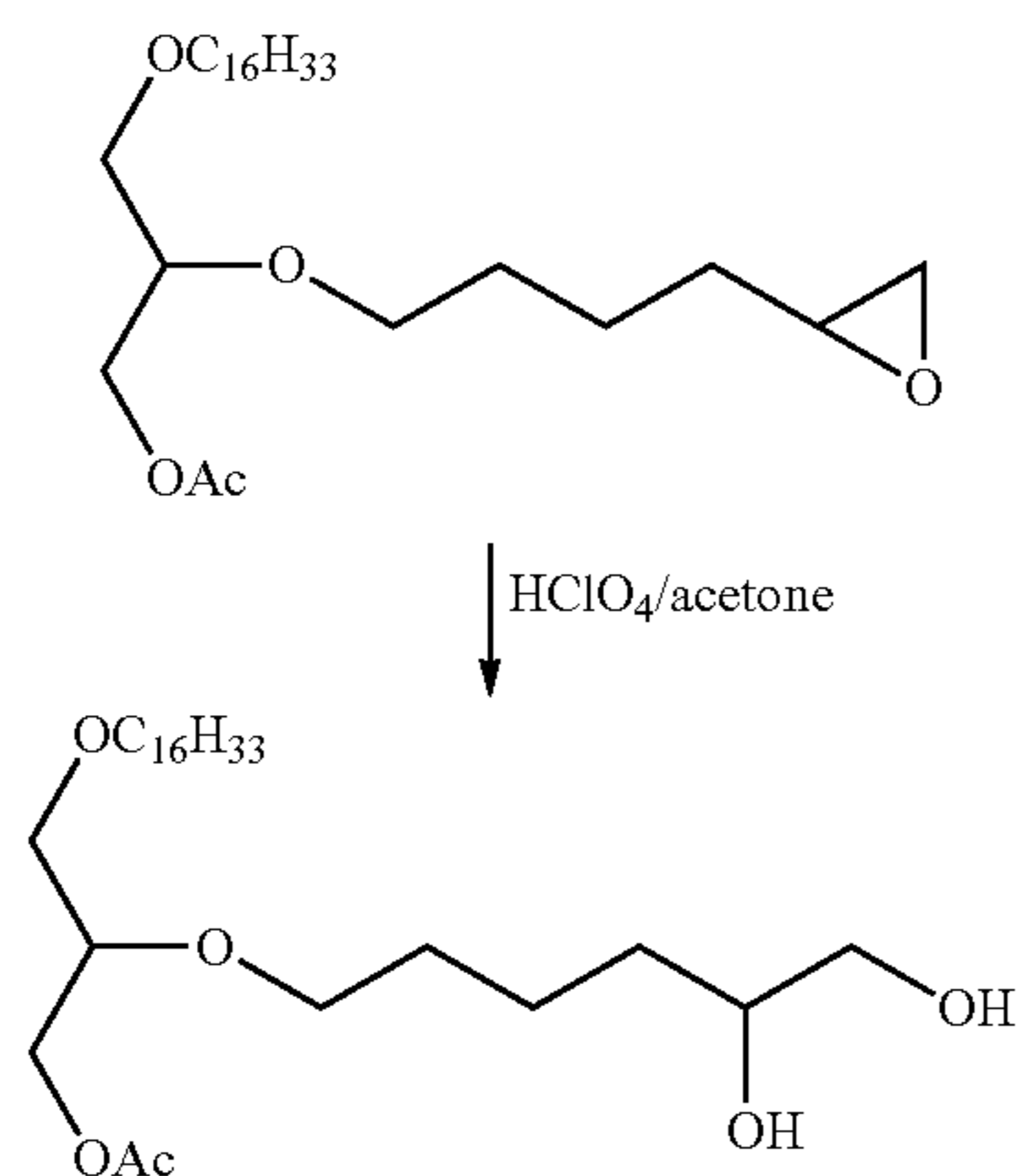
Scheme VIII
