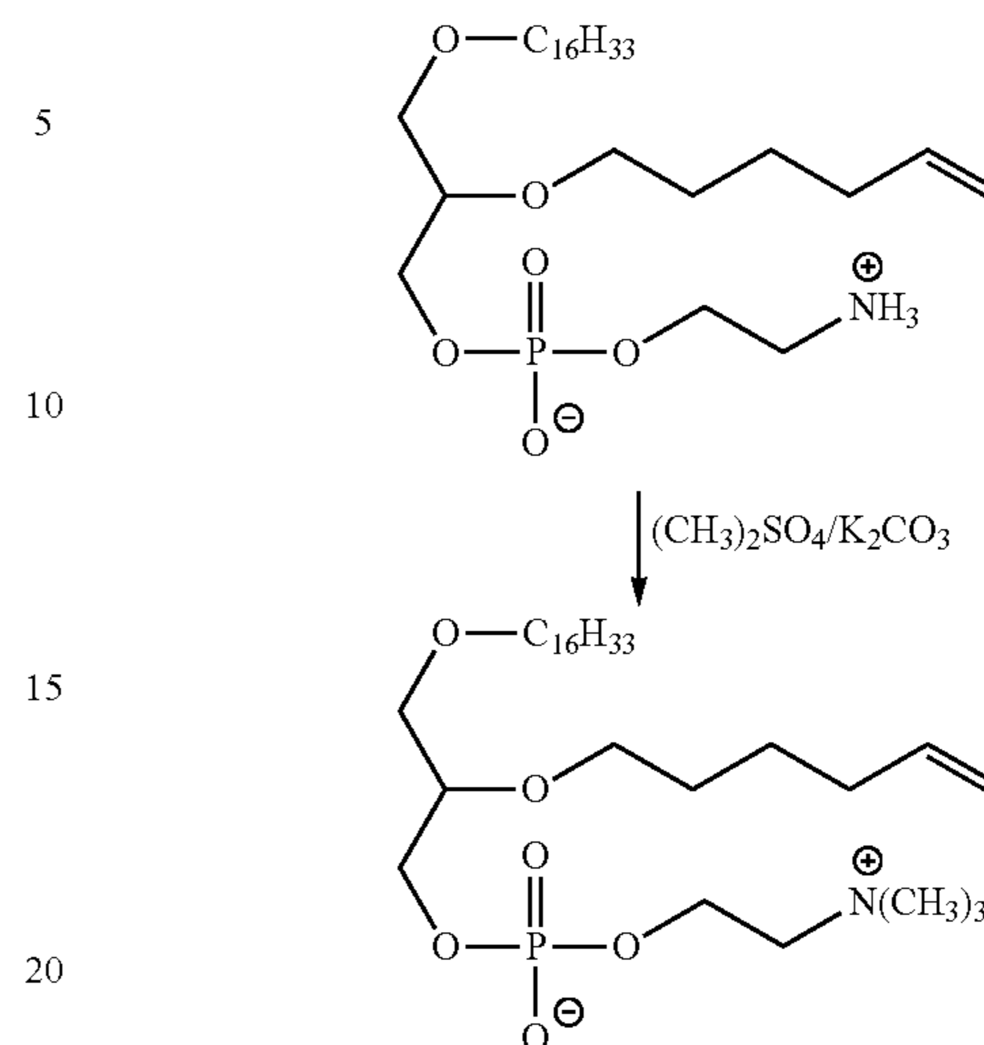
Scheme XIV
