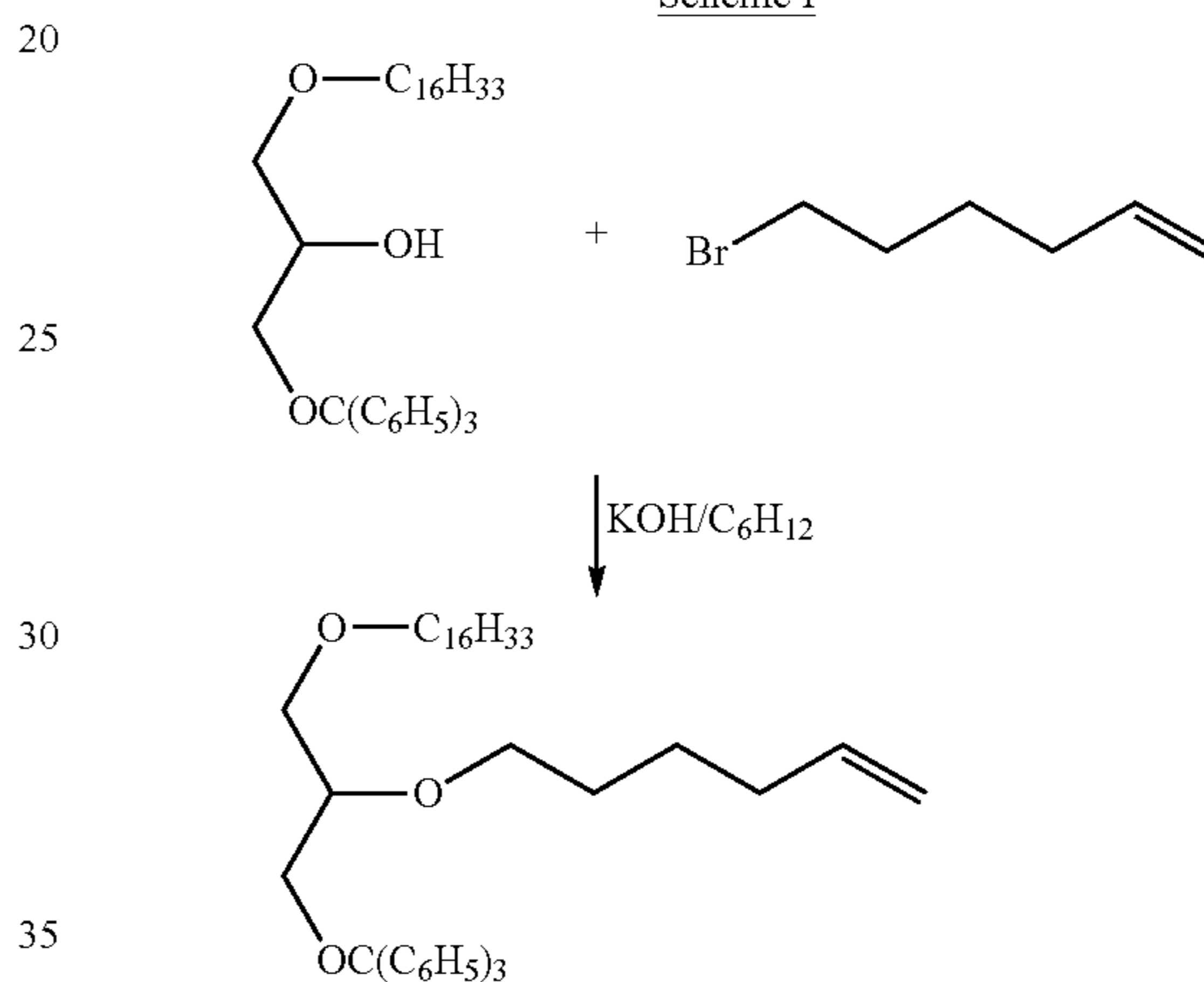
Scheme I
