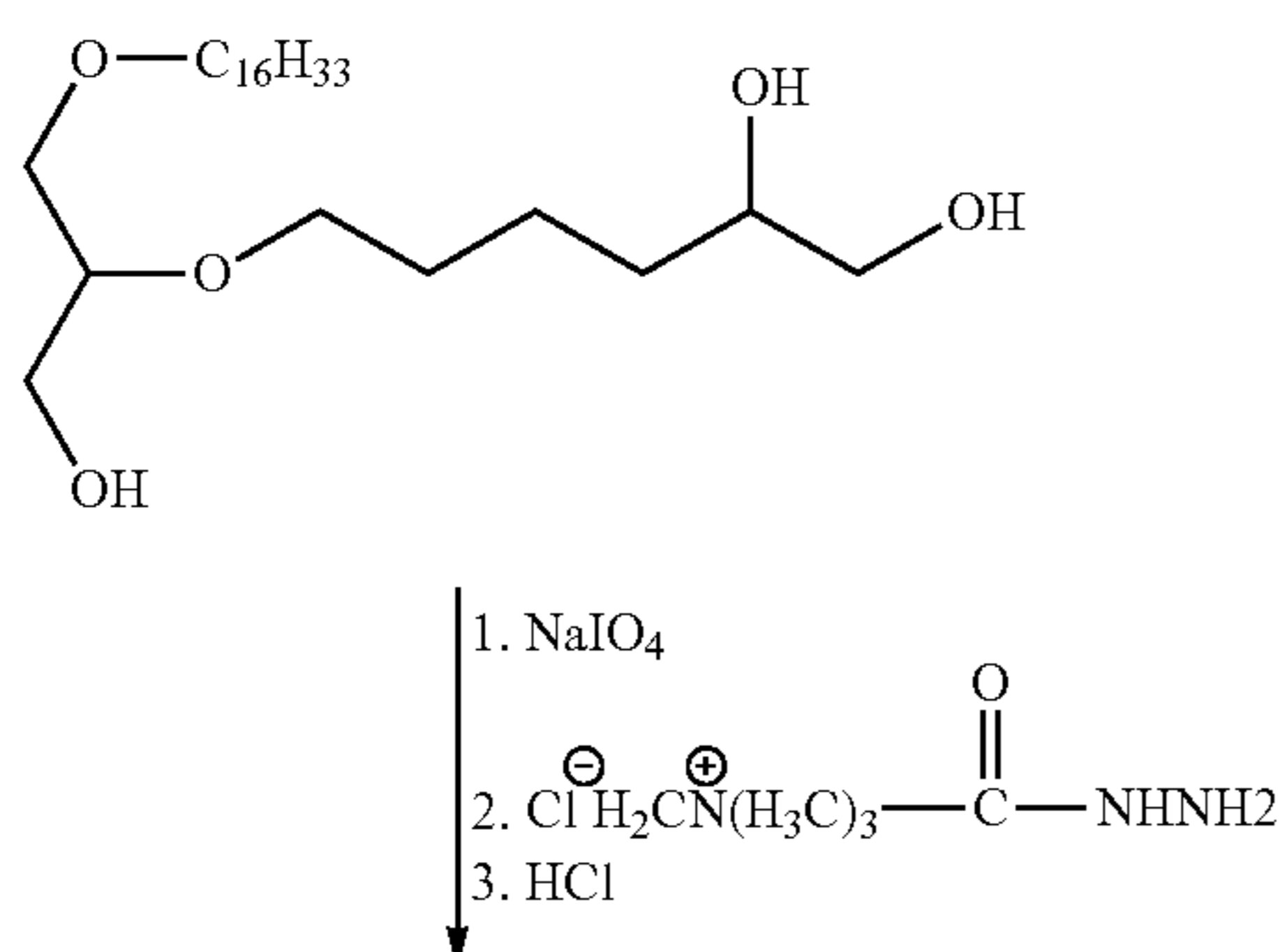
Scheme III
