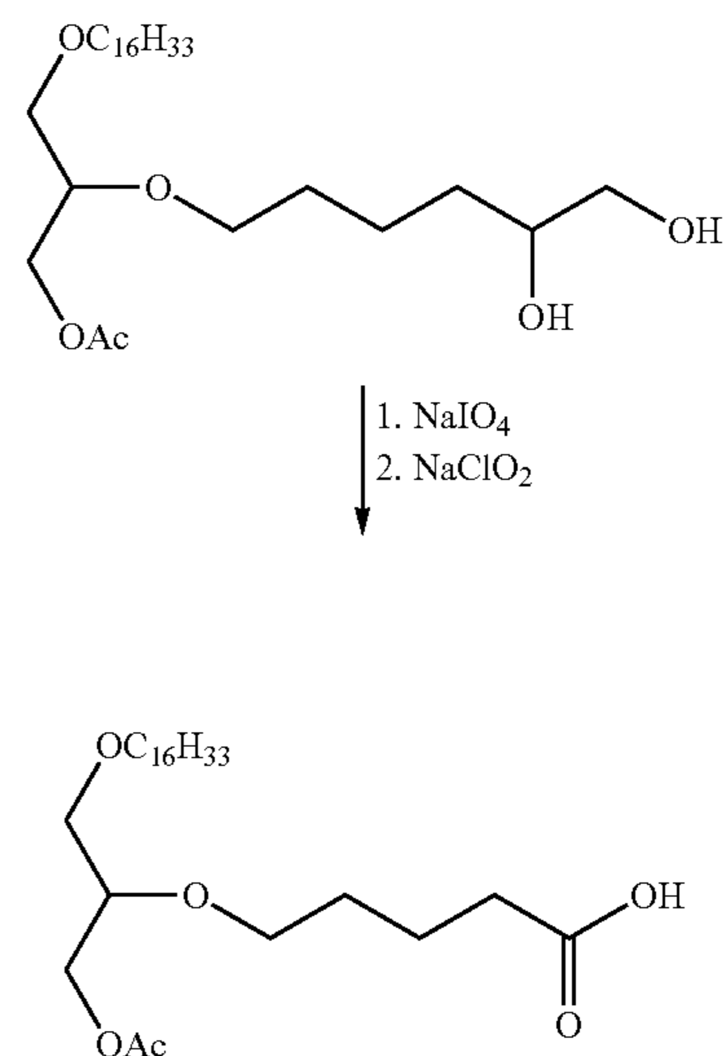
Scheme IX
