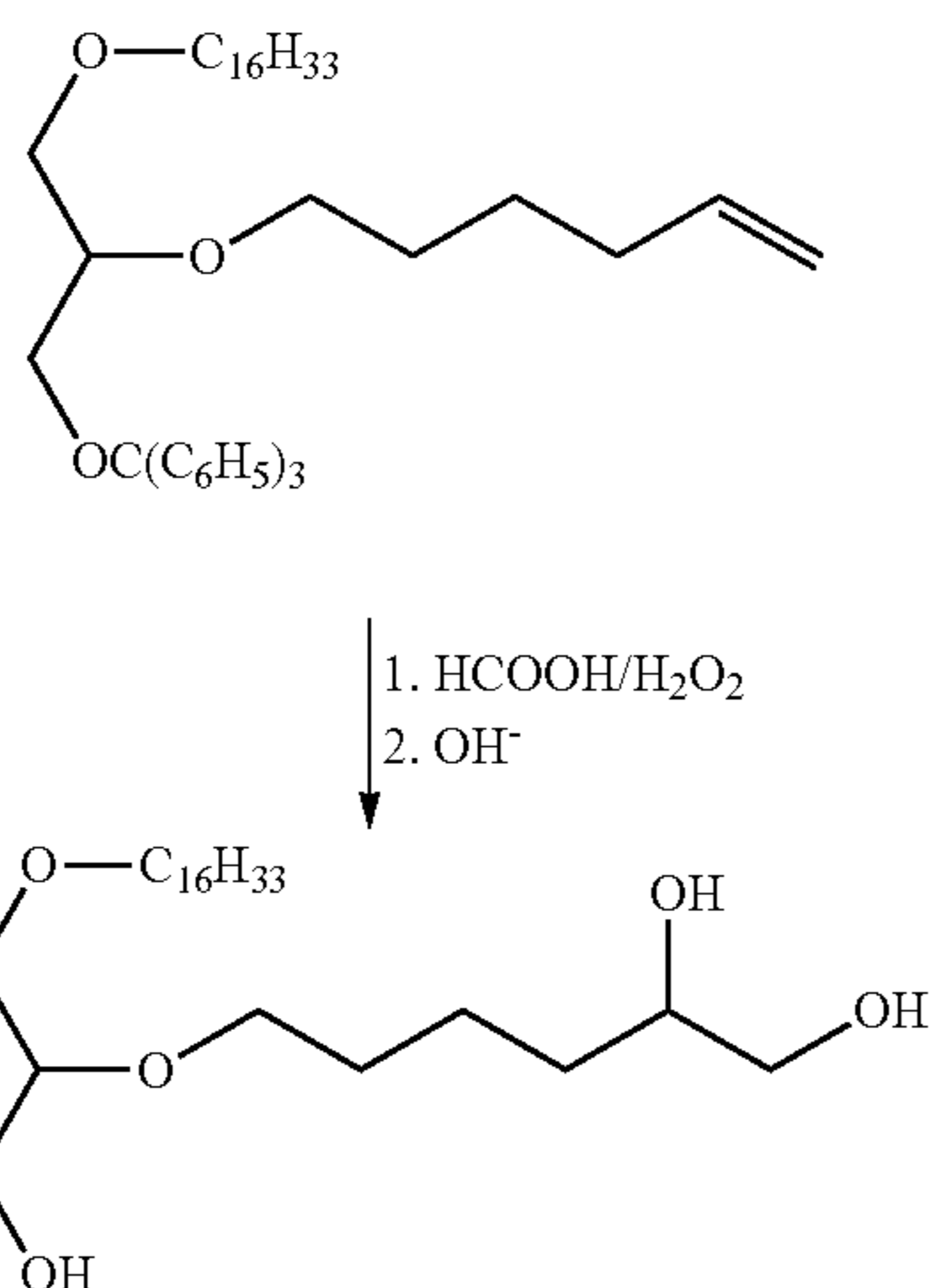
Scheme II
