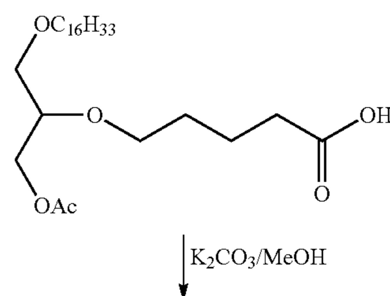
Scheme X
