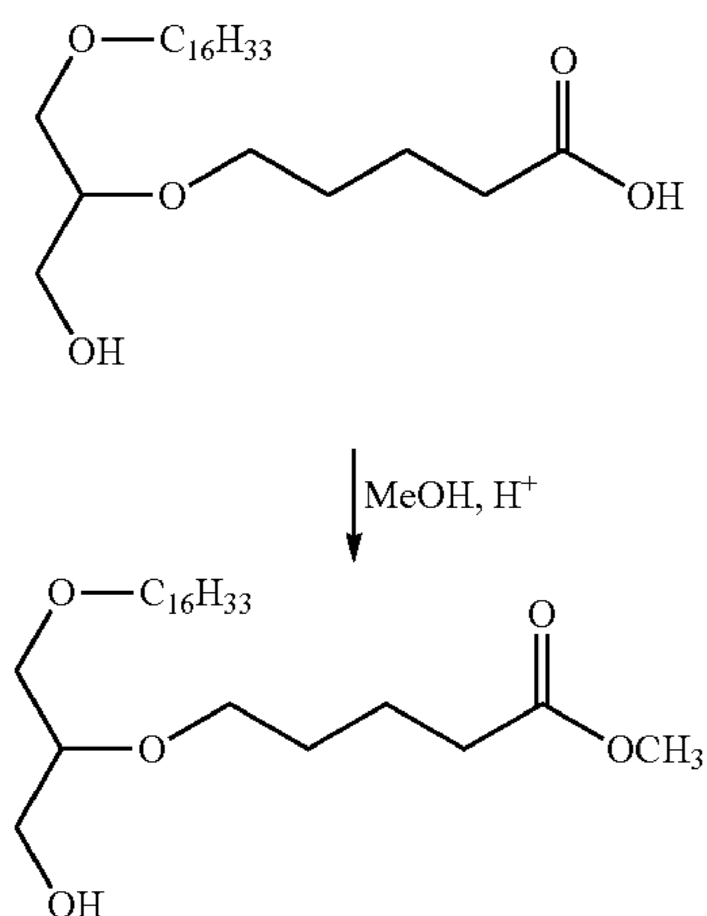
Scheme V
