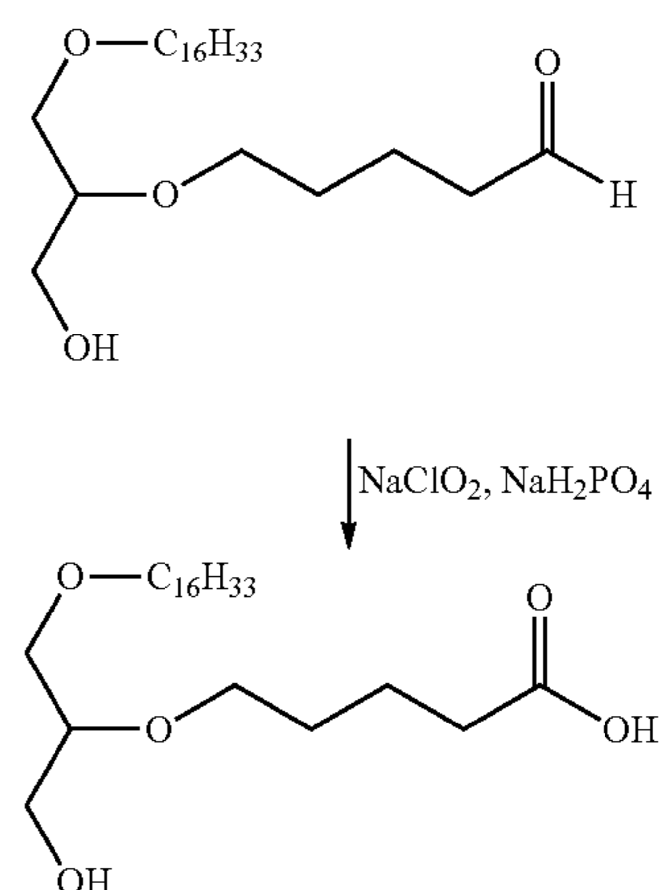
Scheme IV
