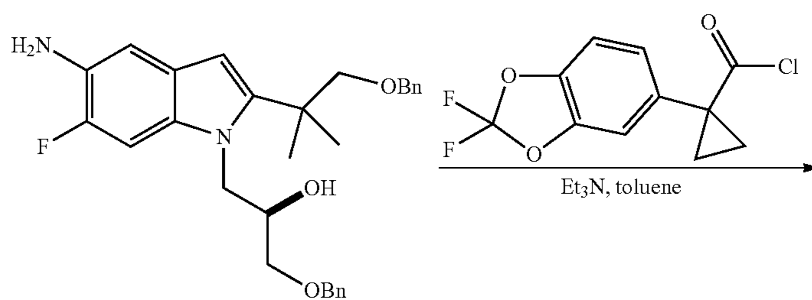
Scheme 4. Formation of Compound 1.
