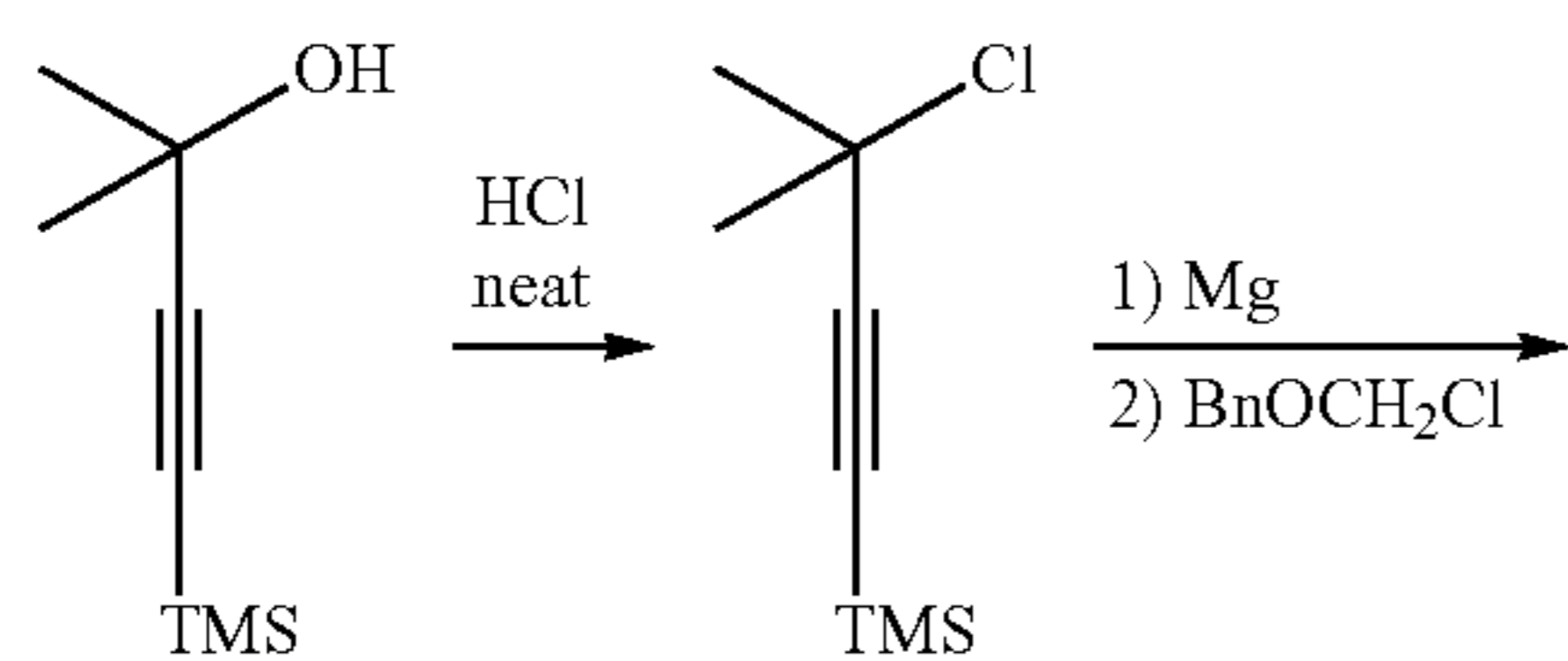
Scheme 3. Synthesis of the amine moiety.
