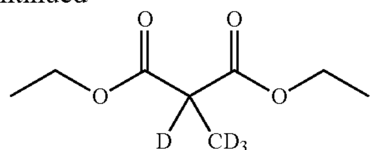
d 4 -Diethyl 2-methylmalonate
