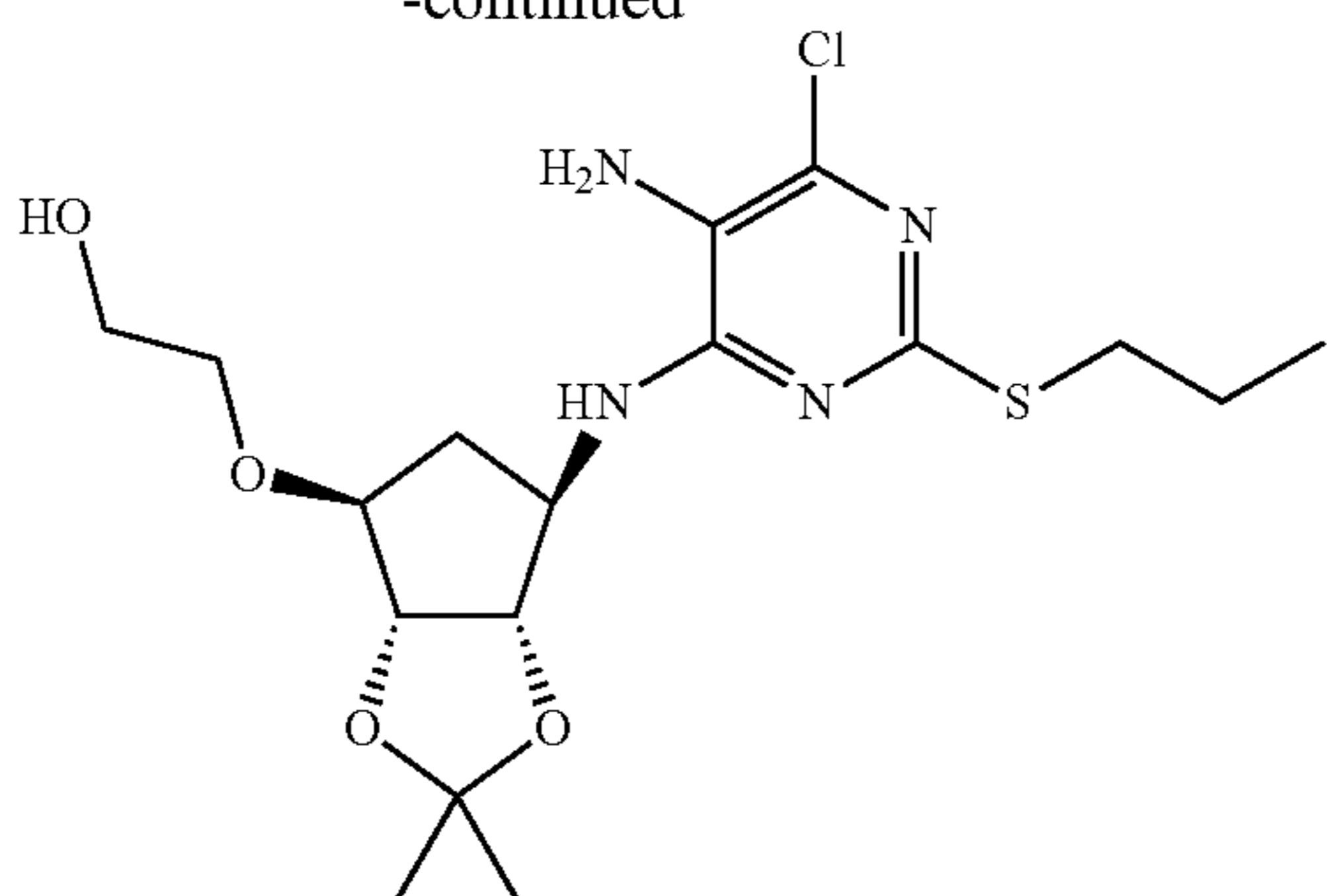
2-((3aR,4S,6R,6aS)-6-(5-Amino-6-chloro-2-(propylthio)pyrimidin-4-ylamino)-2,2-dimethyl-tetrahydro-3aH-cyclopenta[d][1,3]dioxol-4-yloxy)ethanol
