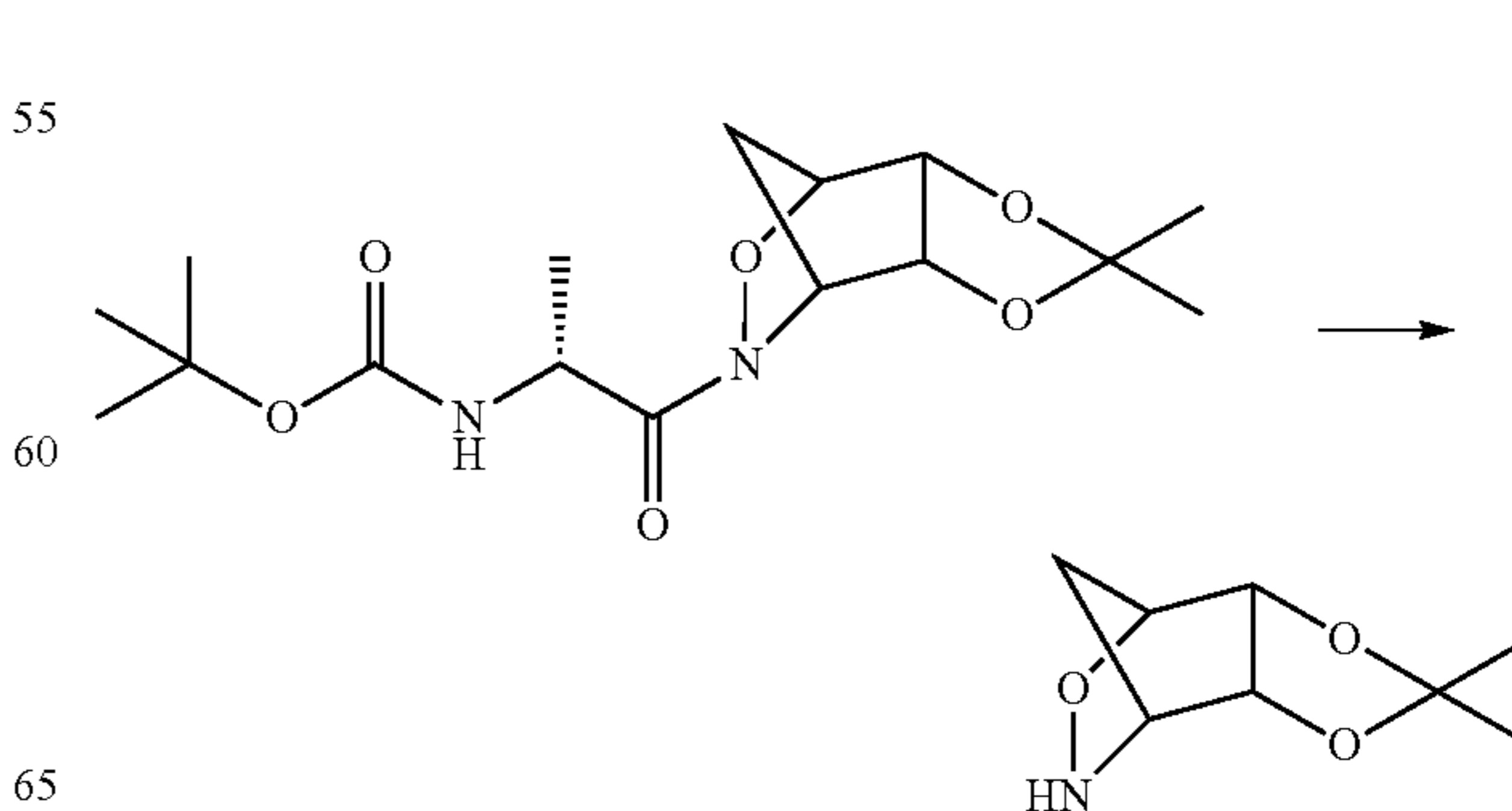
tert-Butyl(R)-1-(5,6-dihydroxy-3-oxa-2-aza-bicyclo[2.2.1]heptan-2-yl)-1-oxopropan-2-ylcarbamate
