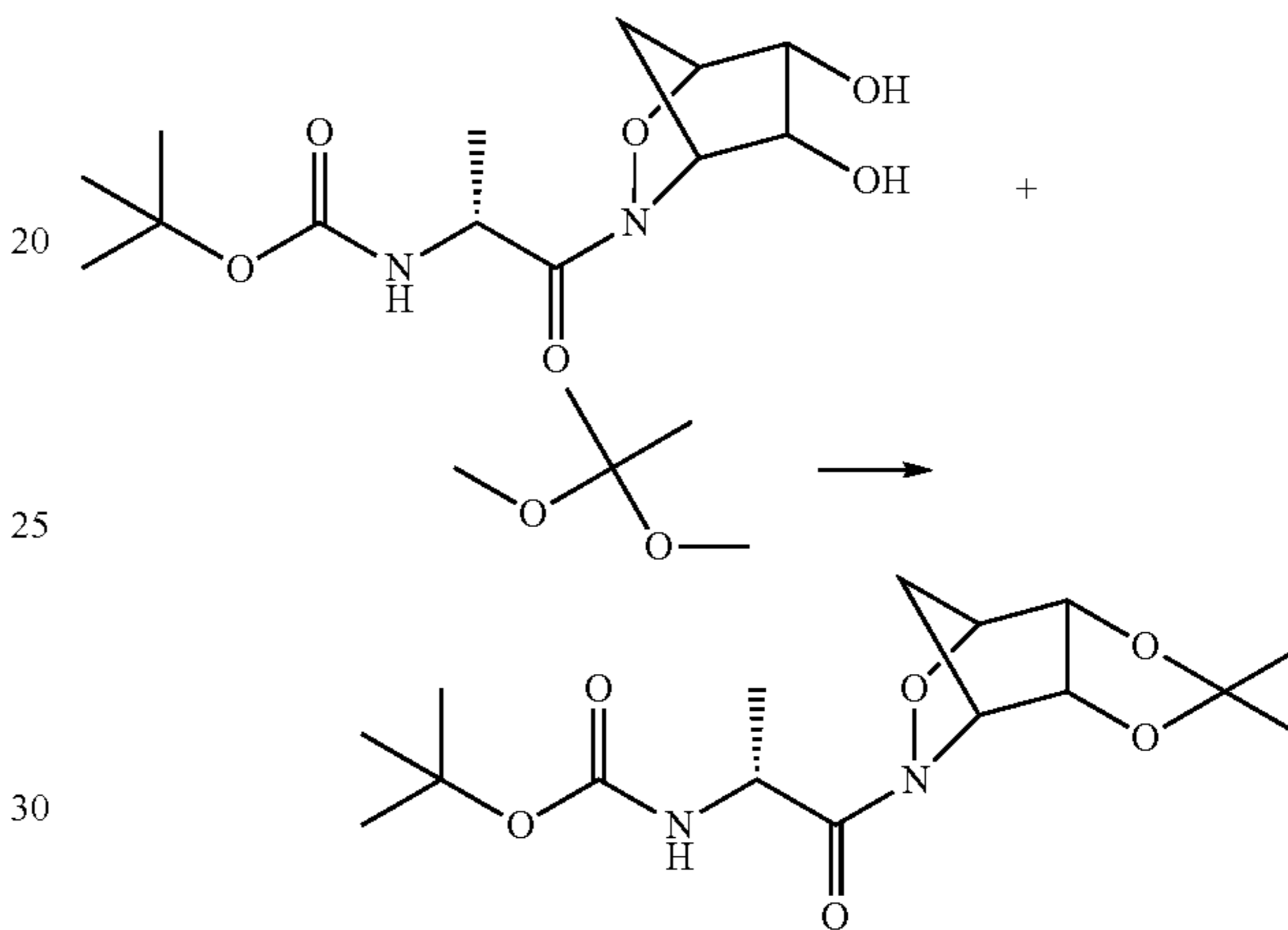
(2-(4,4-Dimethyl-3,5,8-trioxa-9-aza-tricyclo[5.2.1.0 2,6 ]dec-9-yl)-1-methyl-2-oxo-ethyl)-carbamate acid tert-butyl ester
