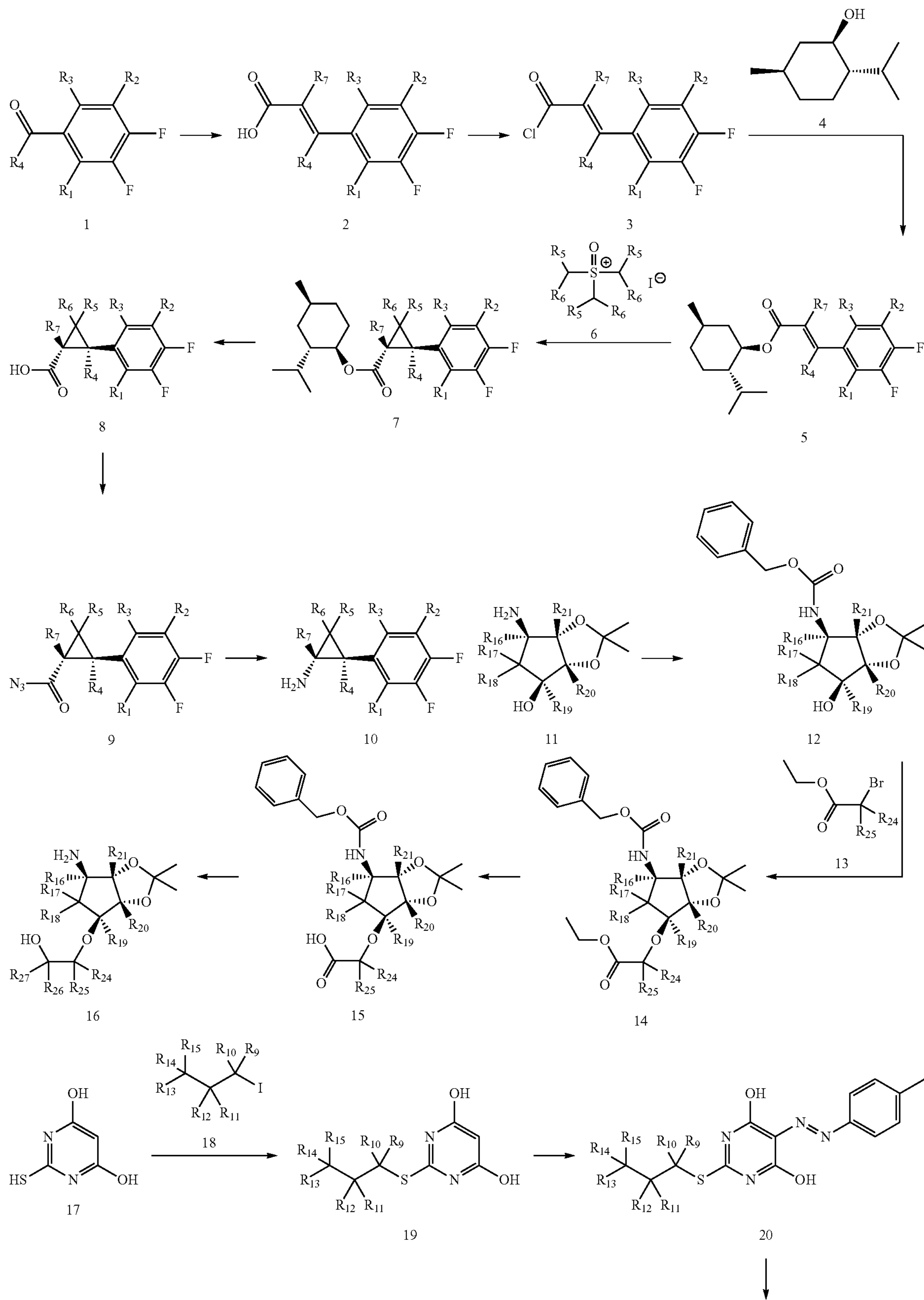
Scheme I
