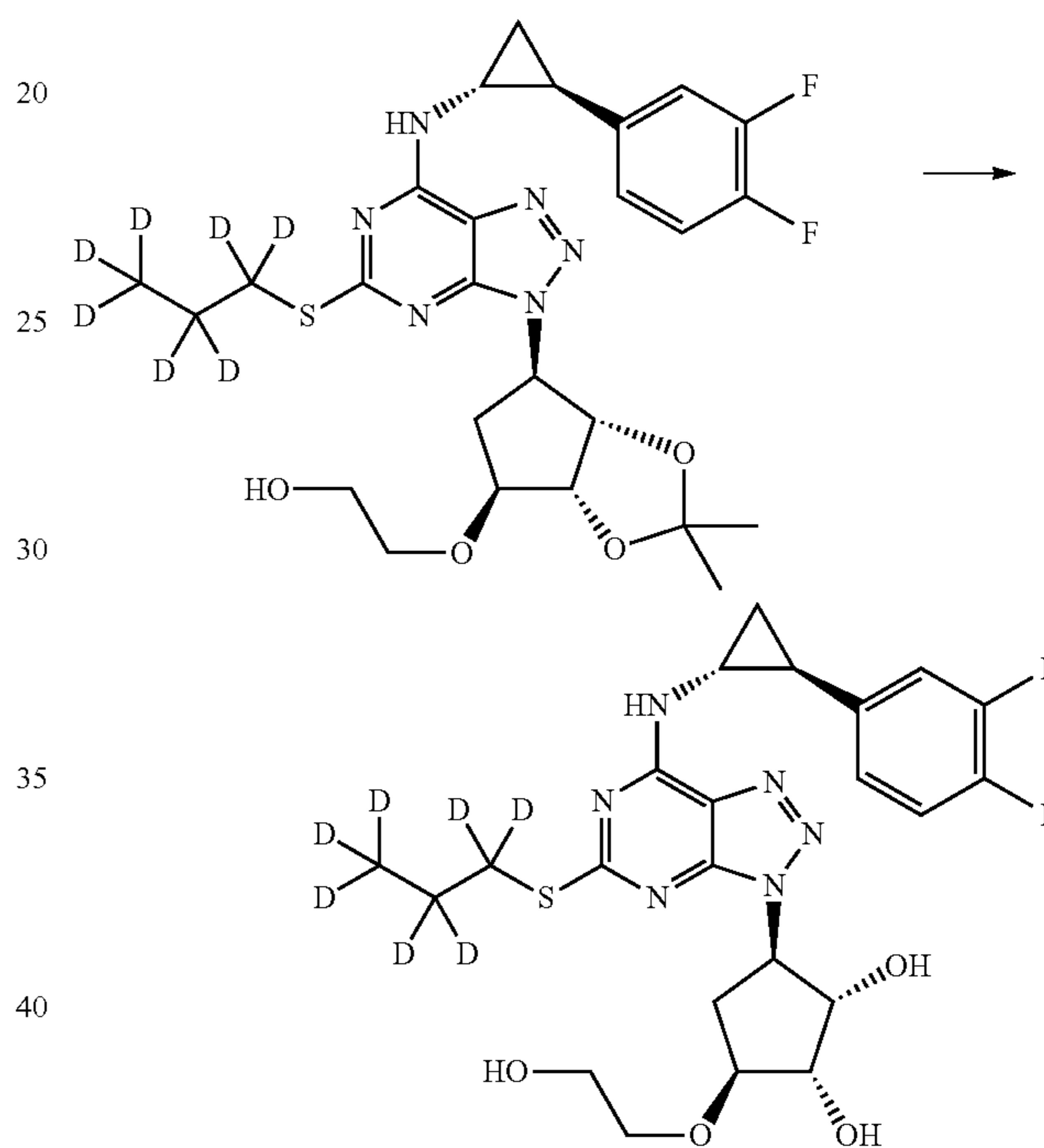
2-((3aR,4S,6R,6aS)-6-(7-Chloro-5-(d 7 -propylthio)-3H-[1,2,3]triazolo[4,5-d]pyrimidin-3-yl)-2,2-dimethyl-tetrahydro-3aH-cyclopenta[d][1,3]dioxol-4-yloxy)ethanol
