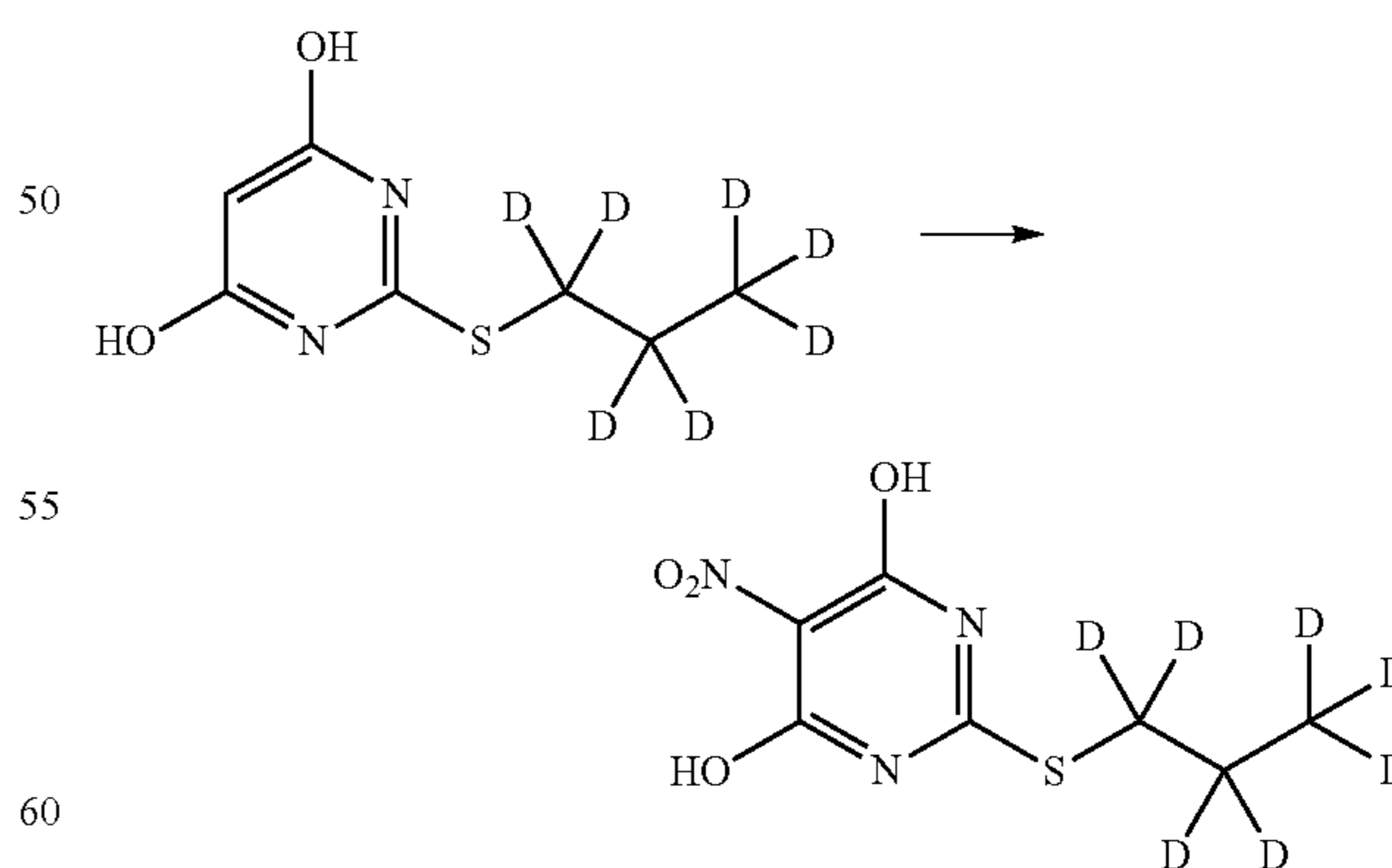
5-Nitro-2-(d 7 -propylthio)pyrimidine-4,6-diol
