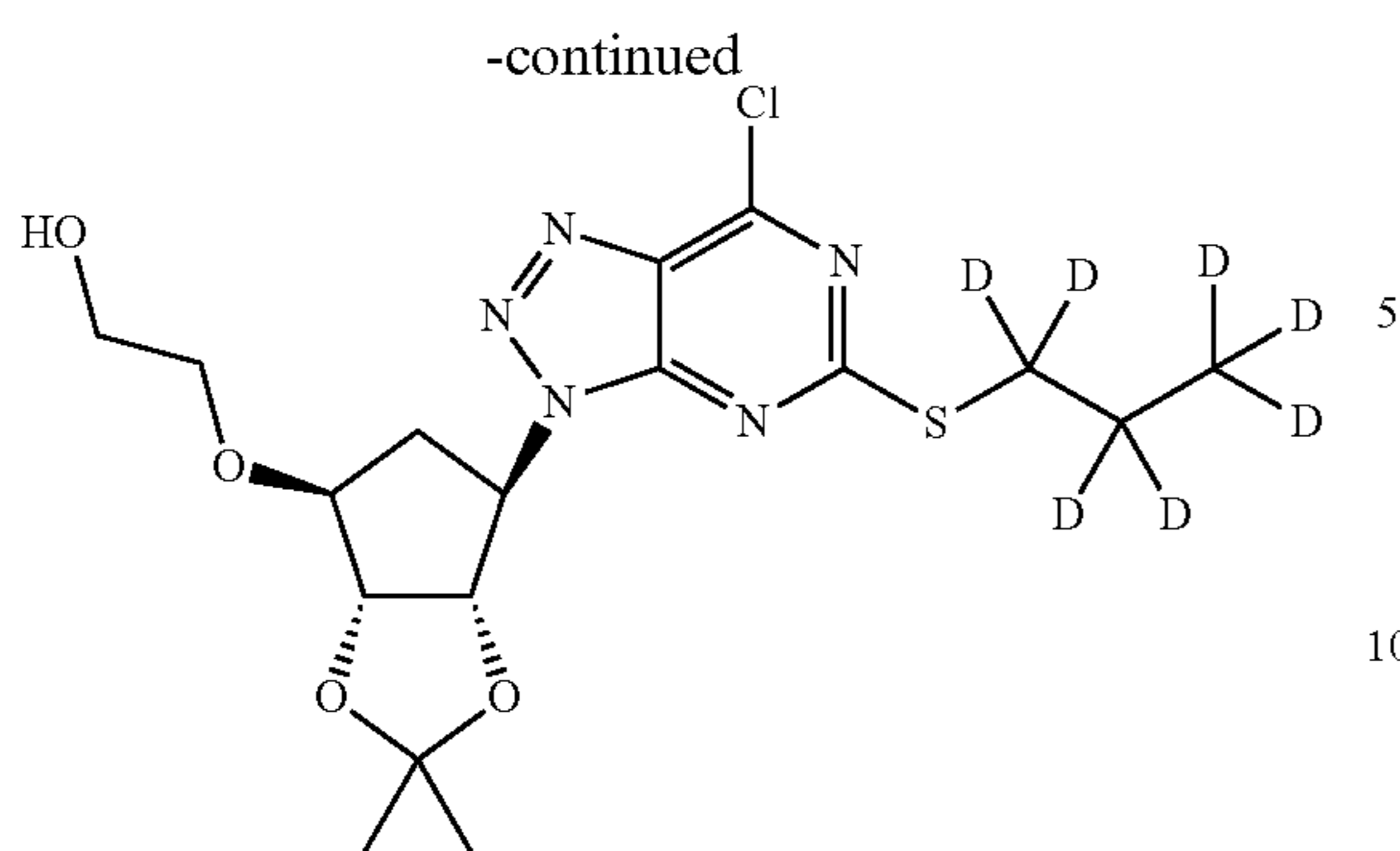
2-((3aR,4S,6R,6aS)-6-(7-((1R,2S)-2-(3,4-Difluorophenyl)cyclopropylamino)-5-(d 7 -propylthio)-3H-[1,2,3]triazolo[4,5-d]pyrimidin-3-yl)-2,2-dimethyl-tetrahydro-3aH-cyclopenta[d][1,3]dioxol-4-yloxy)ethanol
