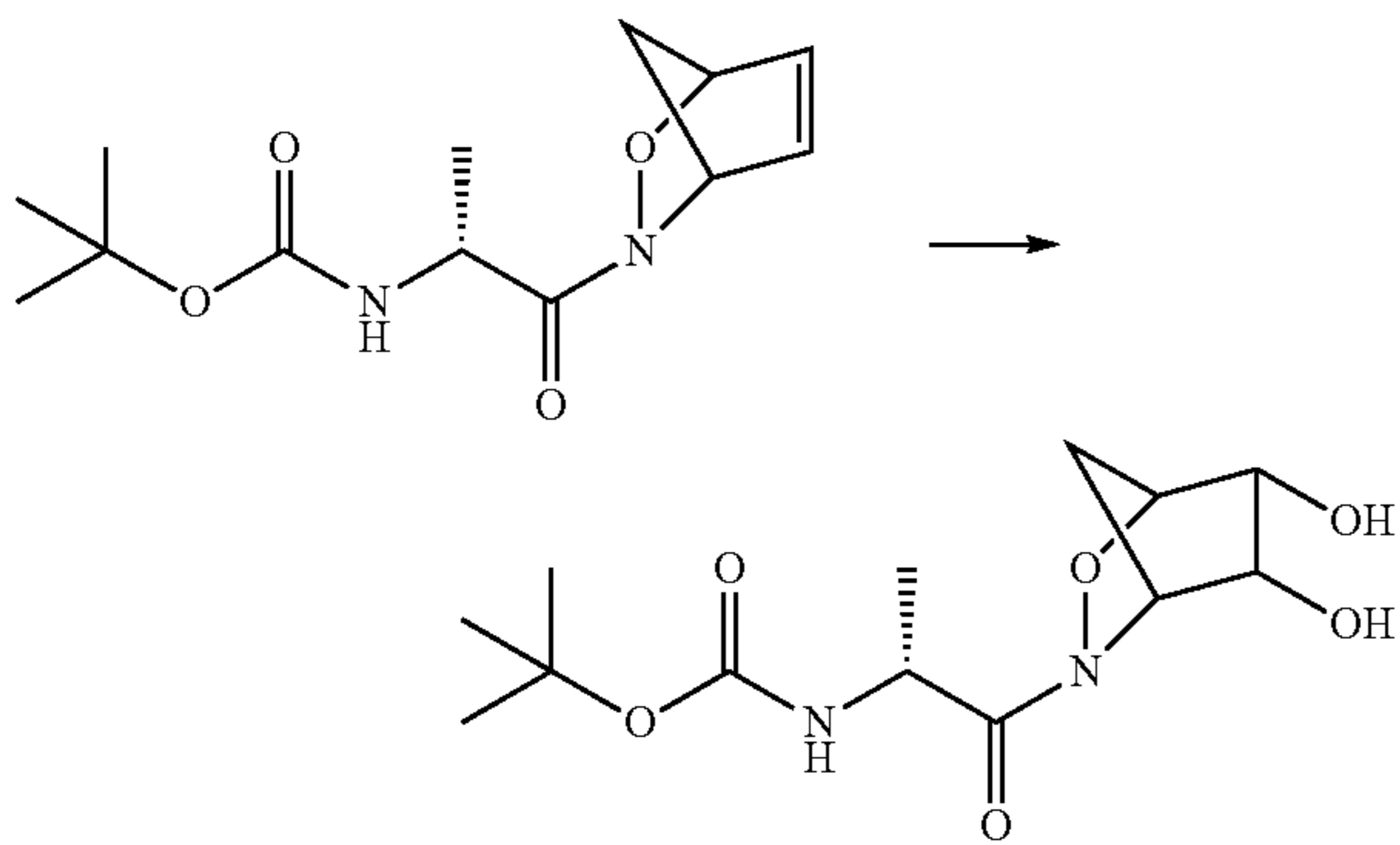
tert-Butyl(R)-1-(5,6-dihydroxy-3-oxa-2-aza-bicyclo[2.2.1]heptan-2-yl)-1-oxopropan-2-ylcarbamate
