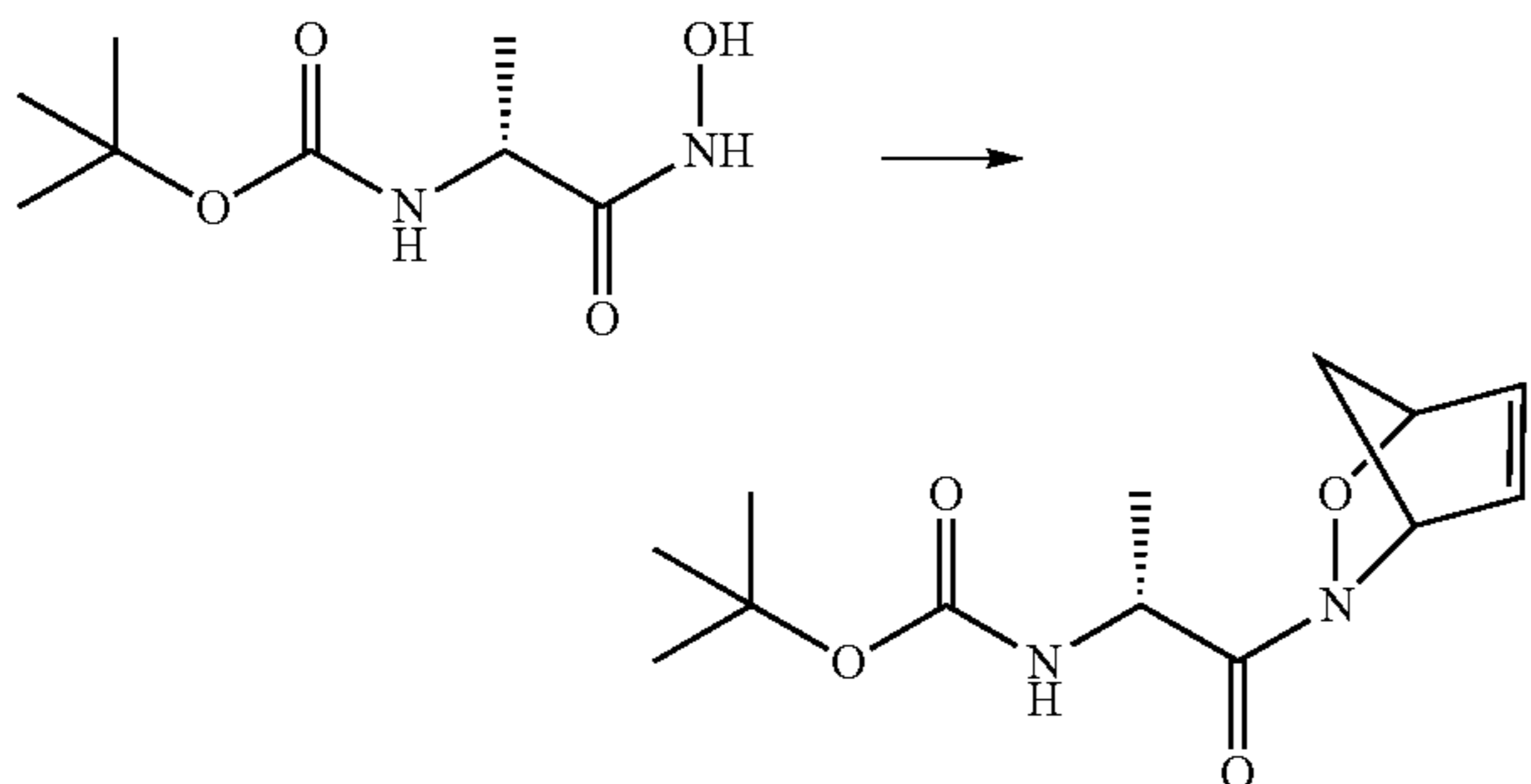
tert-Butyl-(R)-1-(3-oxa-2-aza-bicyclo[2.2.1]hept-5-en-2-yl)-1-oxopropan-2-ylcarbamate
