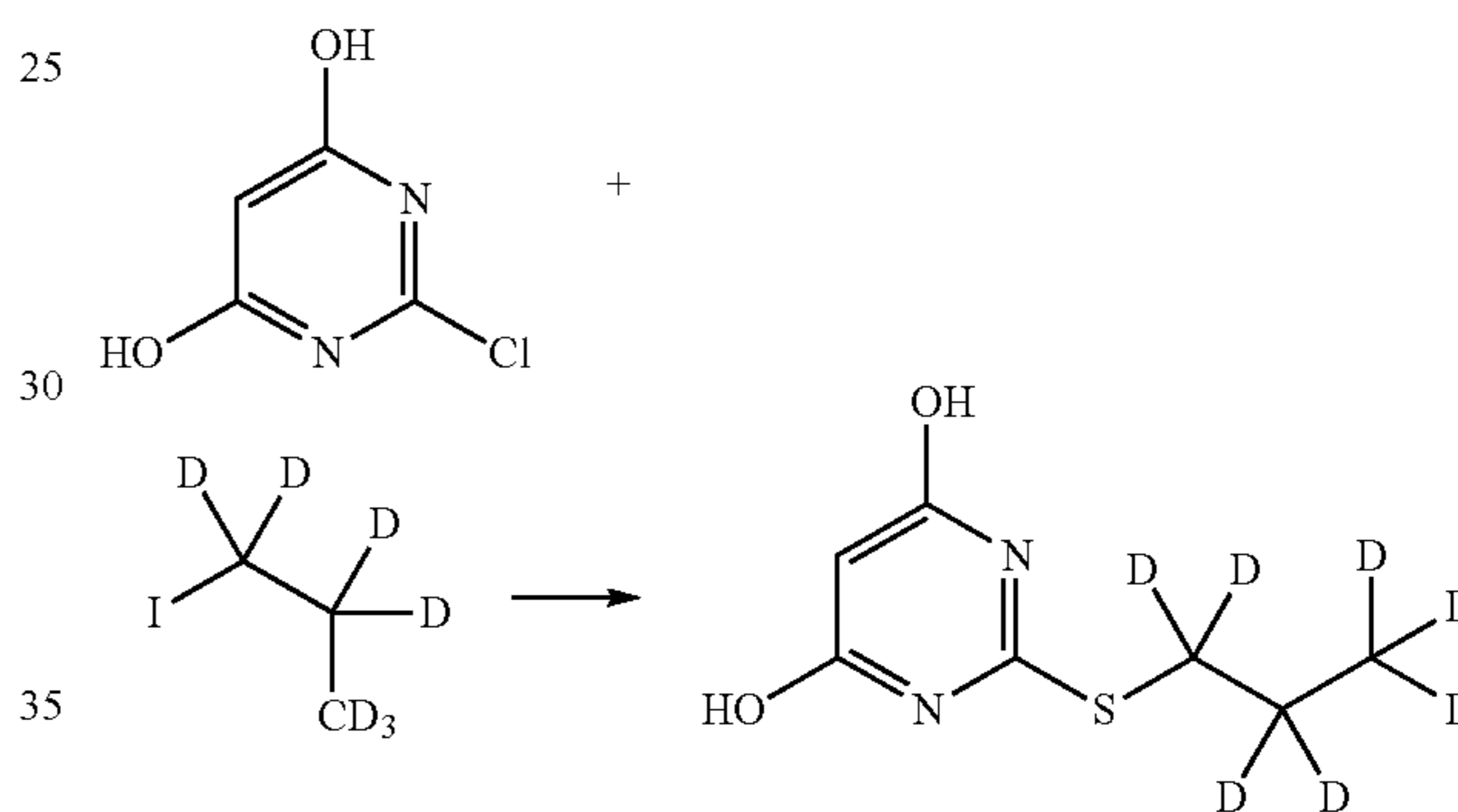
2-(d 7 -Propylthio)pyrimidine-4,6-diol
