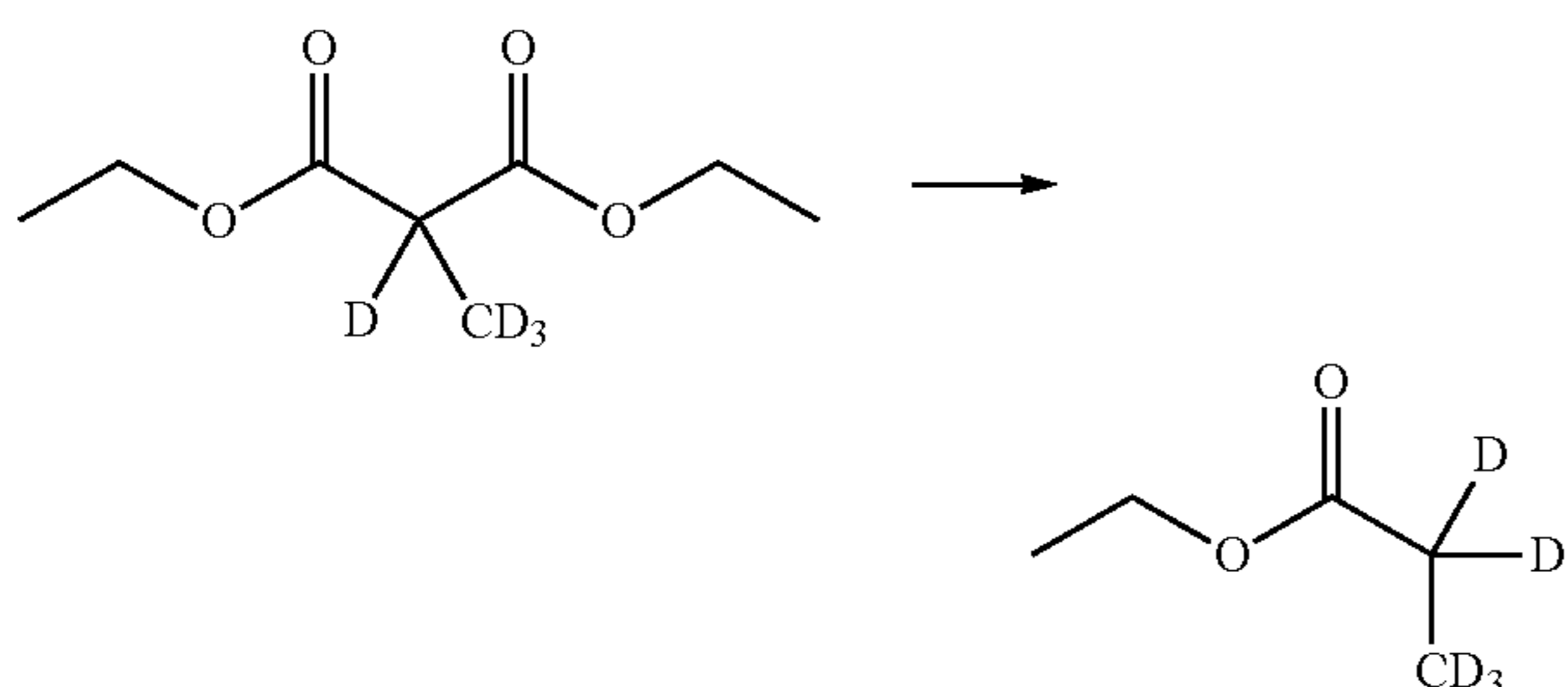
d 5 -Ethyl propionate
