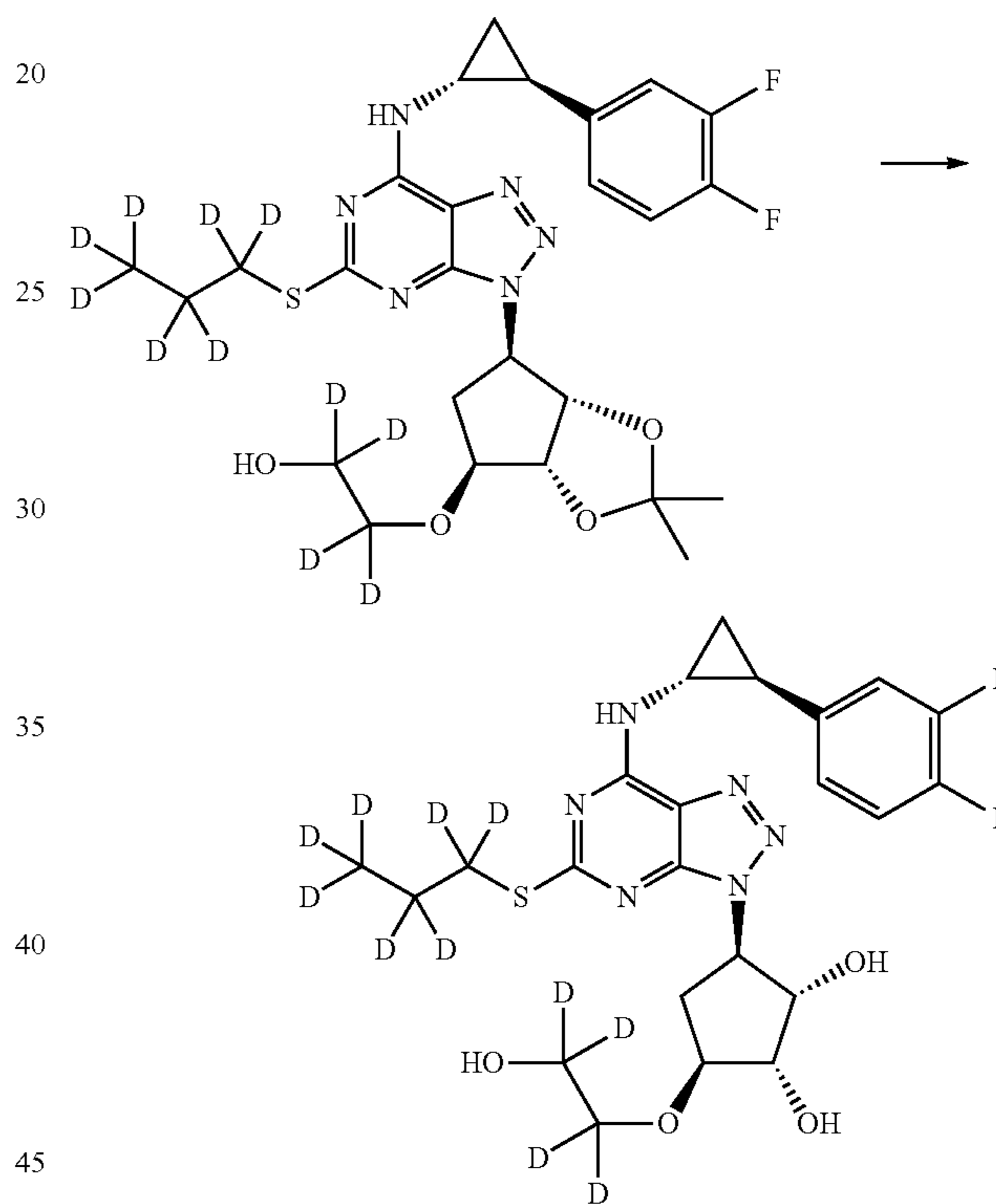
(1S,2S,3R,5S)-3-(7-((1R,2S)-2-(3,4-difluorophenyl)cyclopropylamino)-5-(propylthio)-3H-[1,2,3]triazolo[4,5-d]pyrimidin-3-yl)-5-(2-hydroxyethoxy)cyclopentane-1,2-diol (ticagrelor-d 11 )
