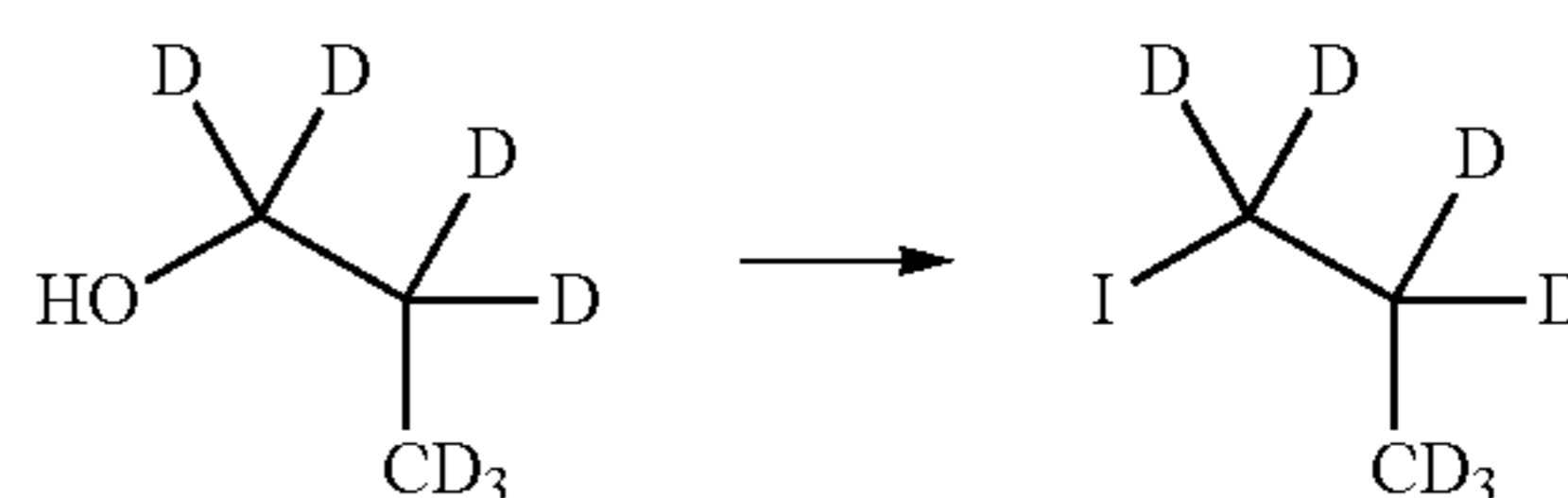
d 7 -1-Iodopropane
