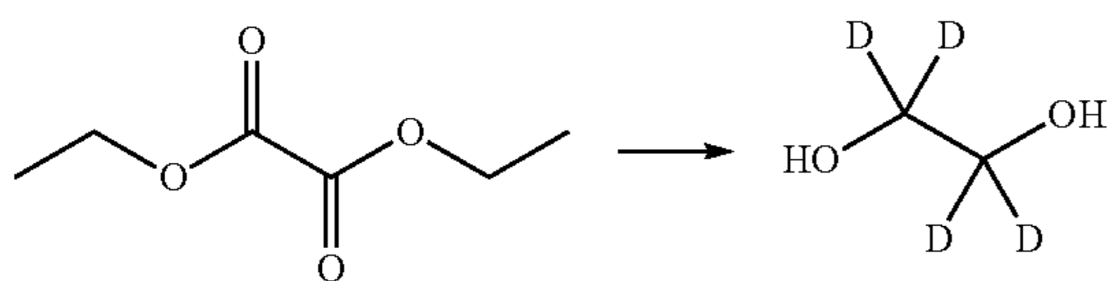
d 4 -Ethane-1,2-diol
