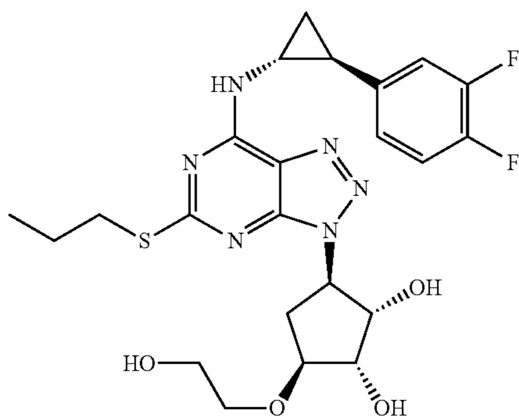
Ticagrelor
