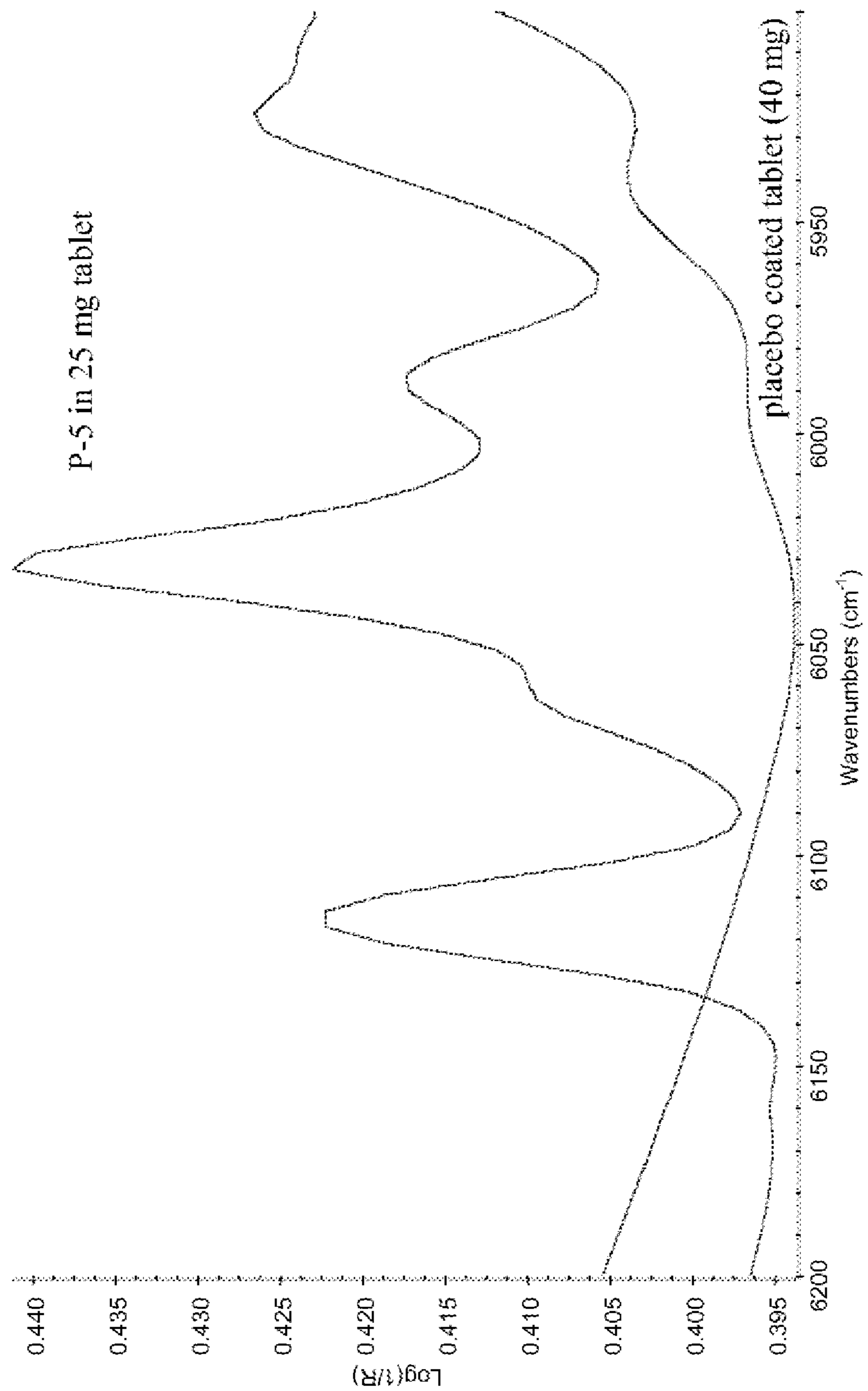
FIG. 30 Characteristic Region of FT-NIR Spectrum of HCl Salt Pattern P-5 in 25 mg Tablet
