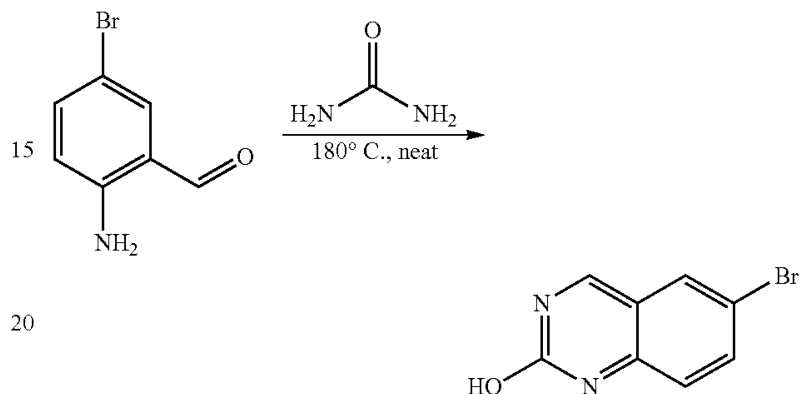
Step 3: Synthesis of 6-bromoquinazolin-2-ol
