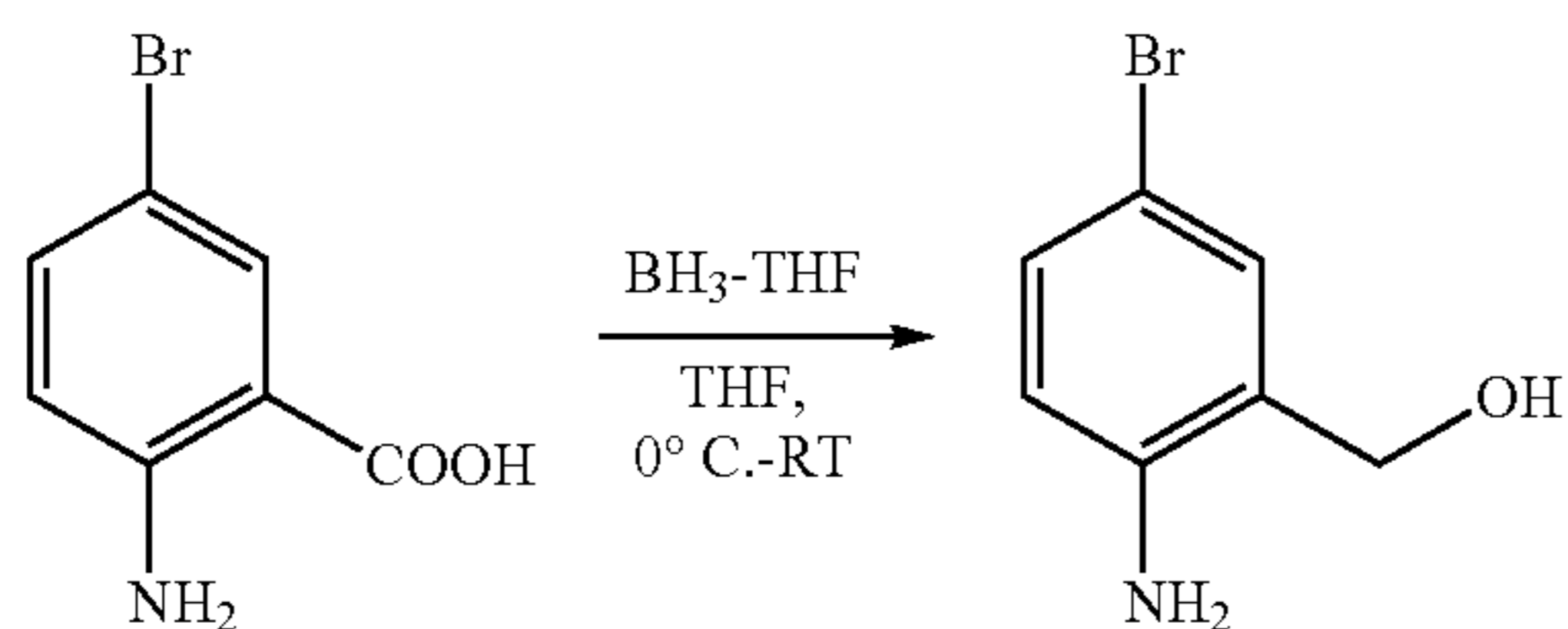
Step 1: Synthesis of (2-amino-5-bromophenyl)methanol
