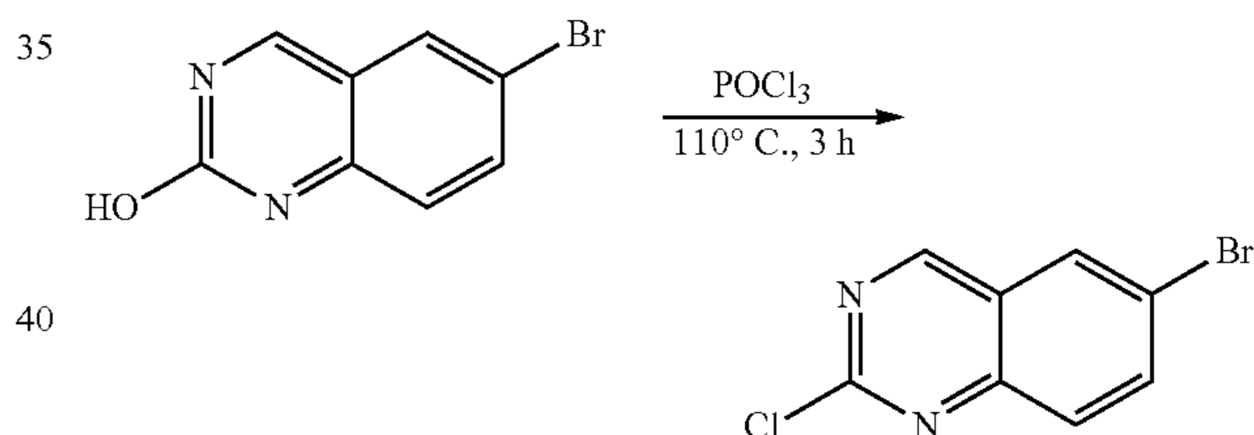
Step 4: Synthesis of 6-bromo-2-chloroquinazoline
