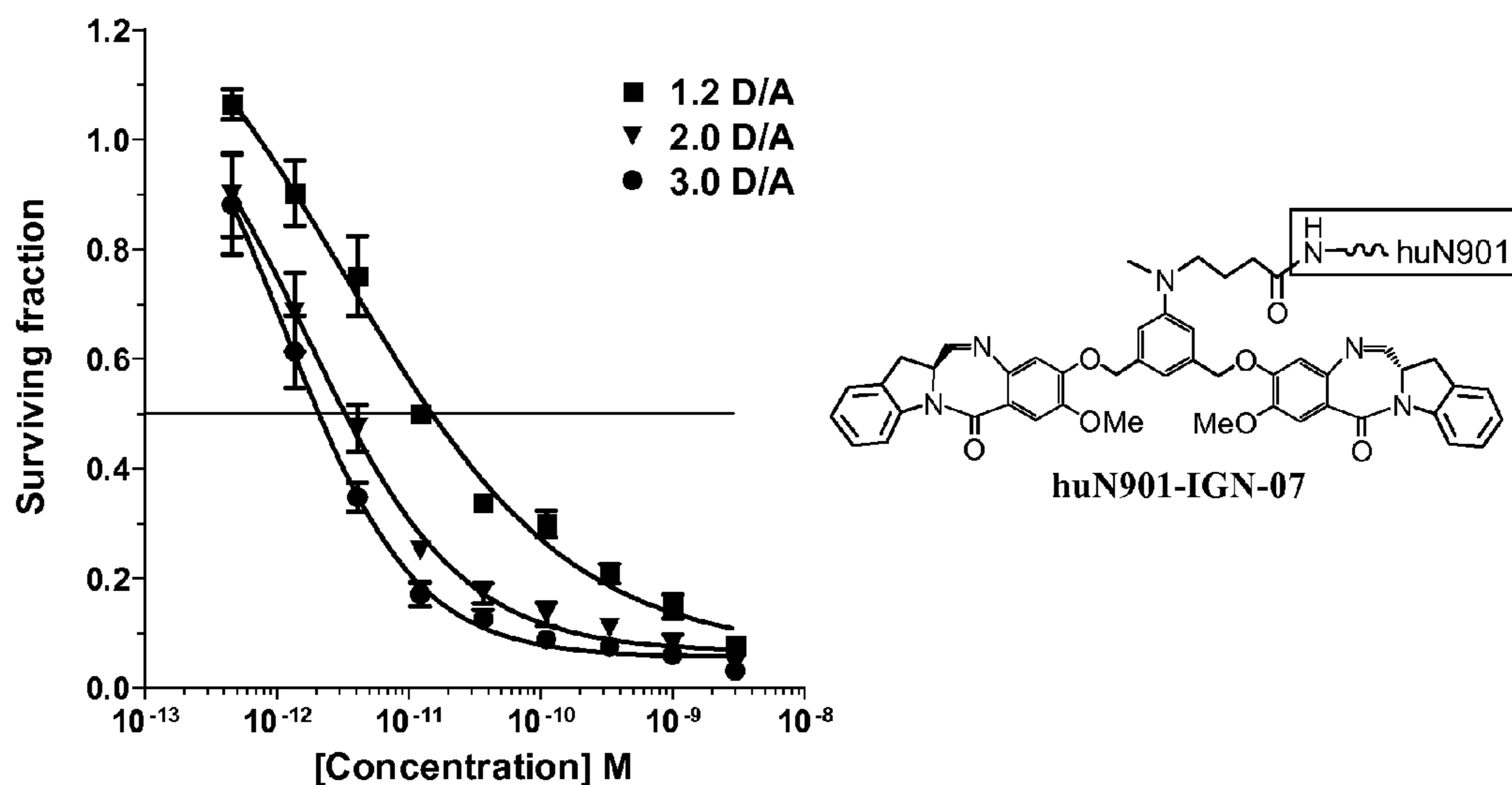
Figure 23. Antiproliferative activity of huN901-IGN-07 against RH-30 (Ag+) cells. Conjugates were tested at three different ratios of cytotoxic agent per antibody (D/A).
