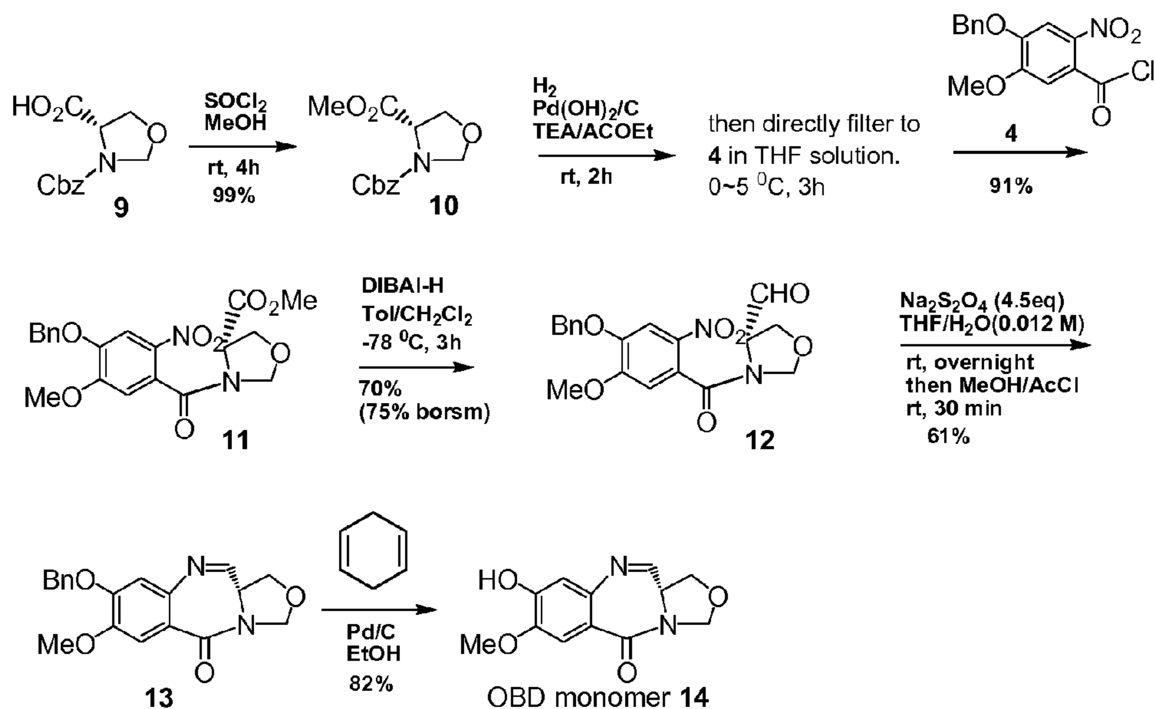
Figure 2. Synthetic scheme of OBD monomer 14
