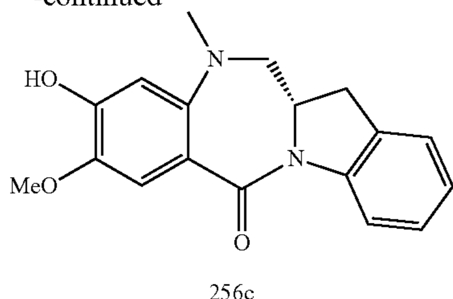
Compound 256c
