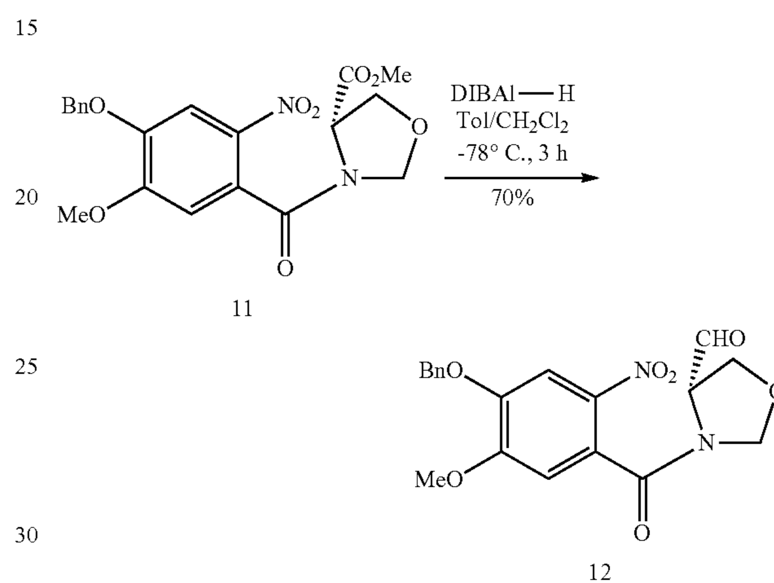
Aldehyde 12
