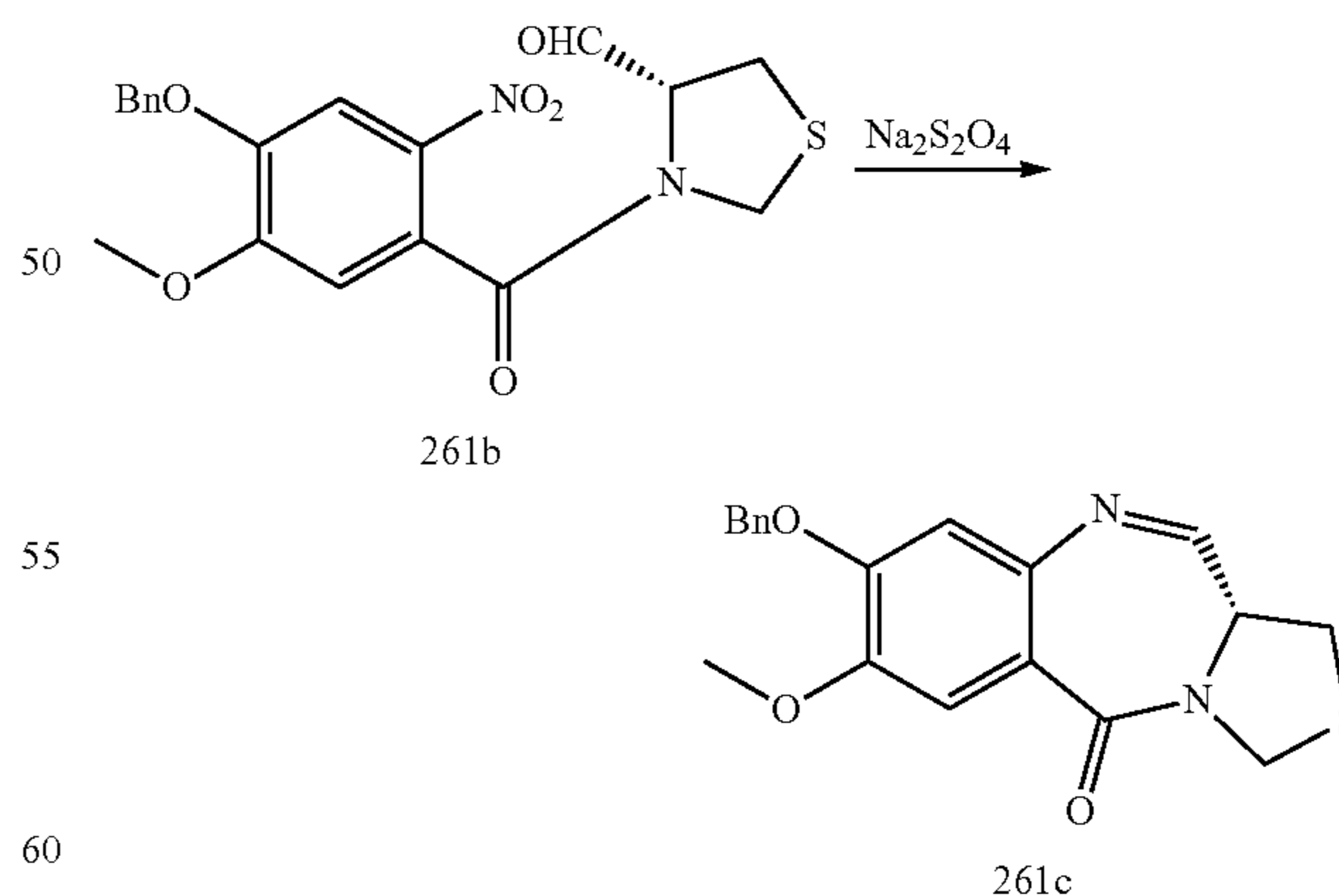
Compound 261c
