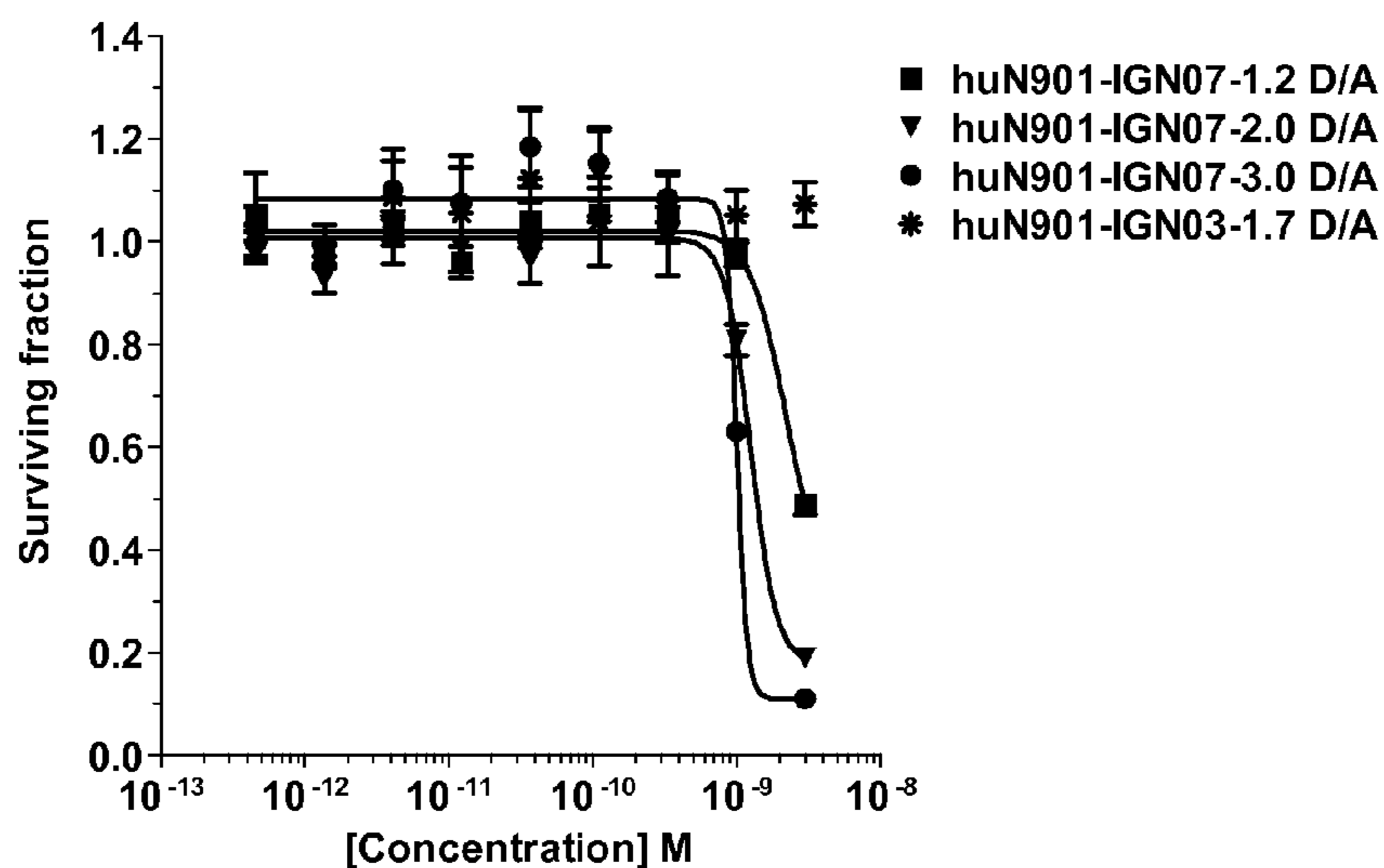
Figure 25. Antiproliferative activity of huN901-IGN-07 (1.2-3.0 D/A) and huN901-IGN-03 (1.7 D/A) against Namalwa (Ag-) cells.
