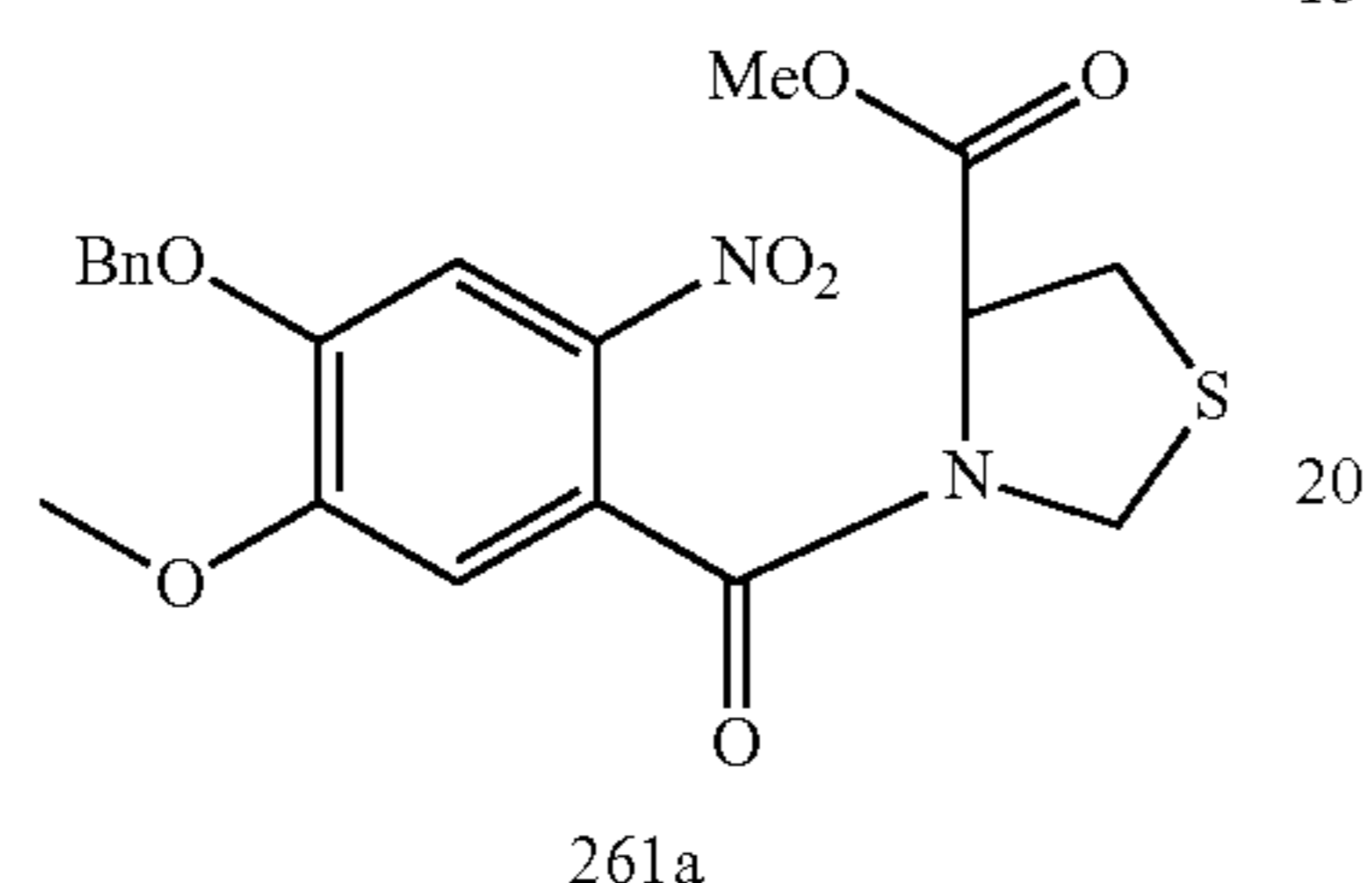
Compound 261a
