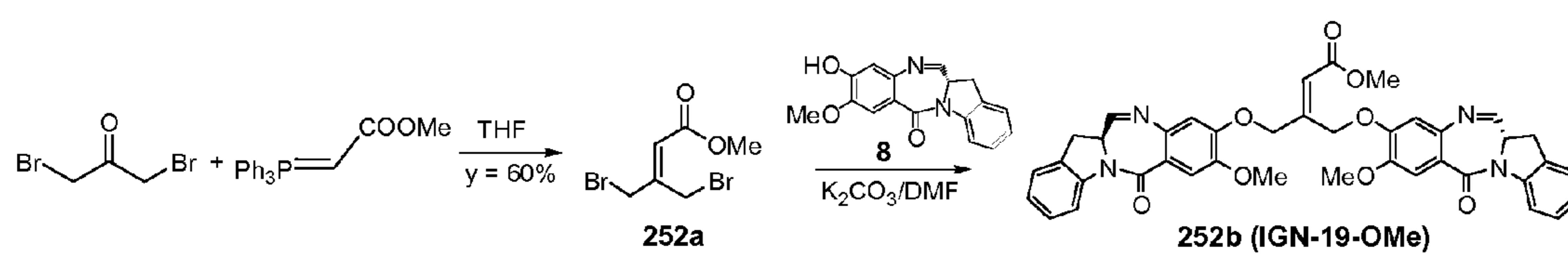
Figure 36. Synthetic scheme for dimer 252b (IGN-19-OMe) .
