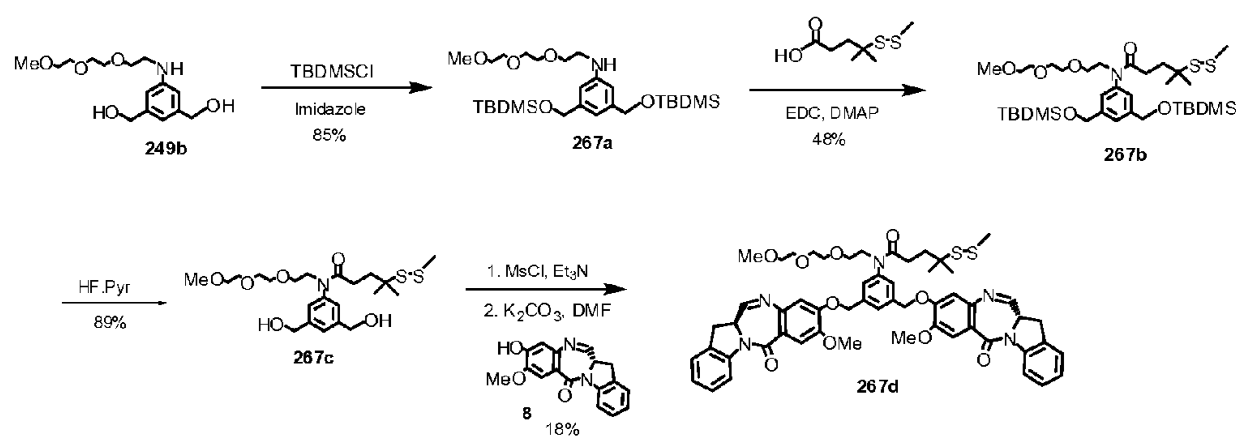
Figure 49. Synthetic scheme of dimer 267d (IGN-31-SMe).
