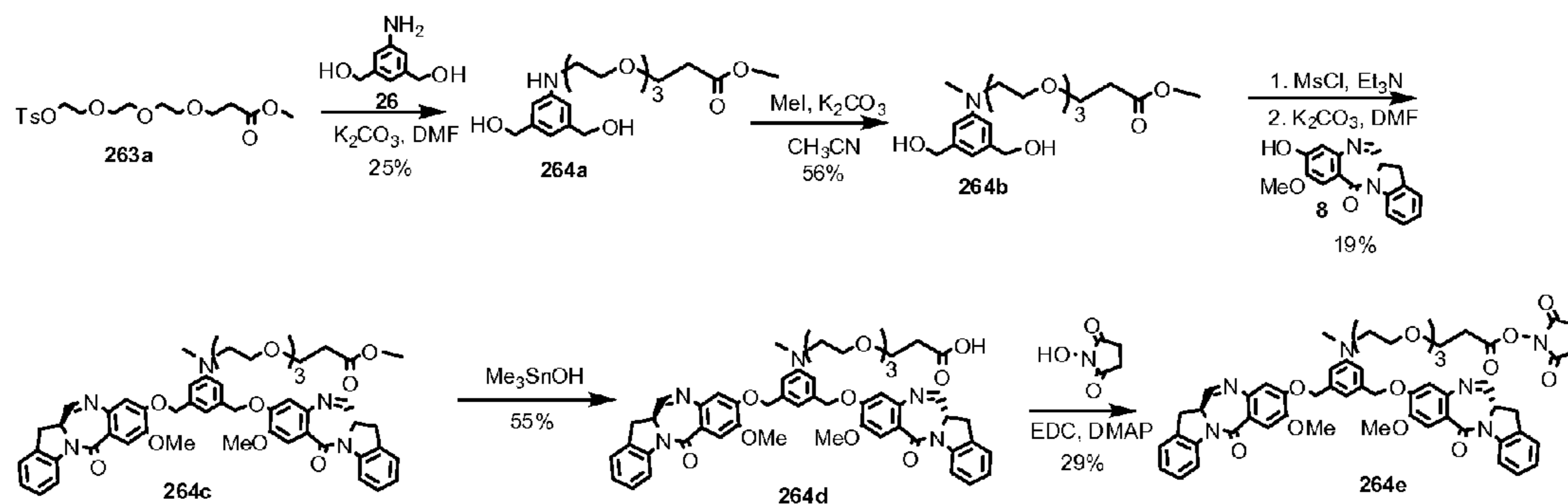
Figure 46. Synthetic scheme of dimer 264e (IGN-27-NHS).
