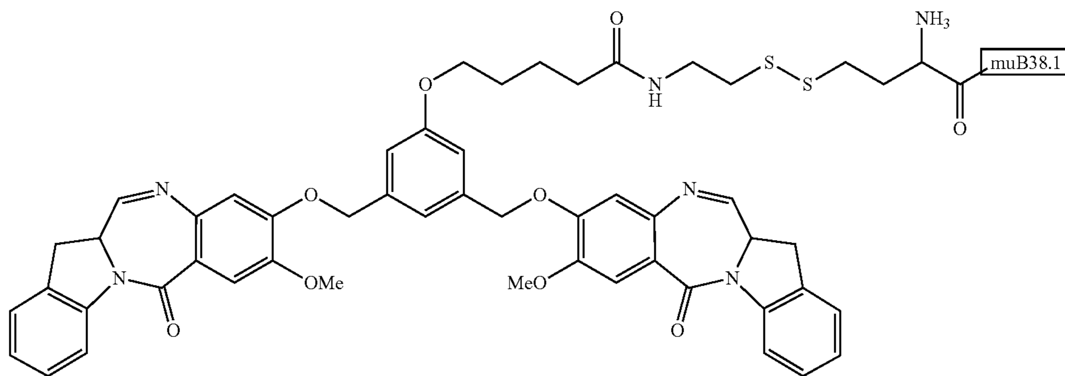
B38.1-IGN-10
