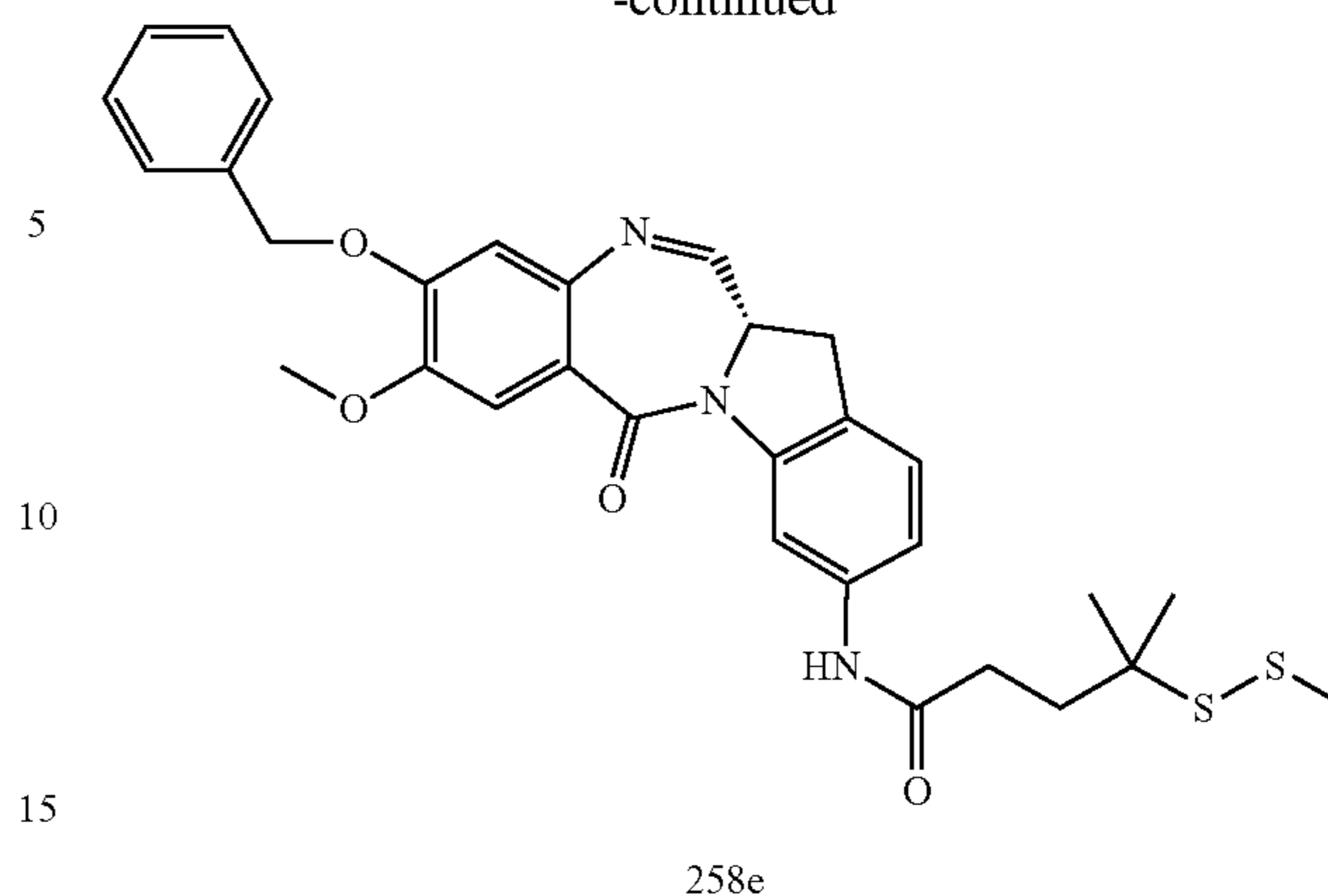
Compound 258e
