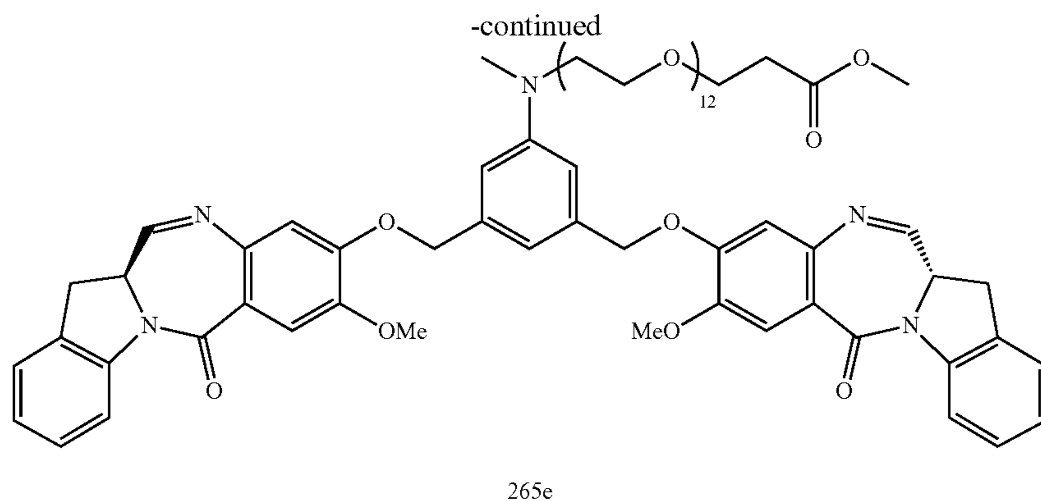
Compound 265e
