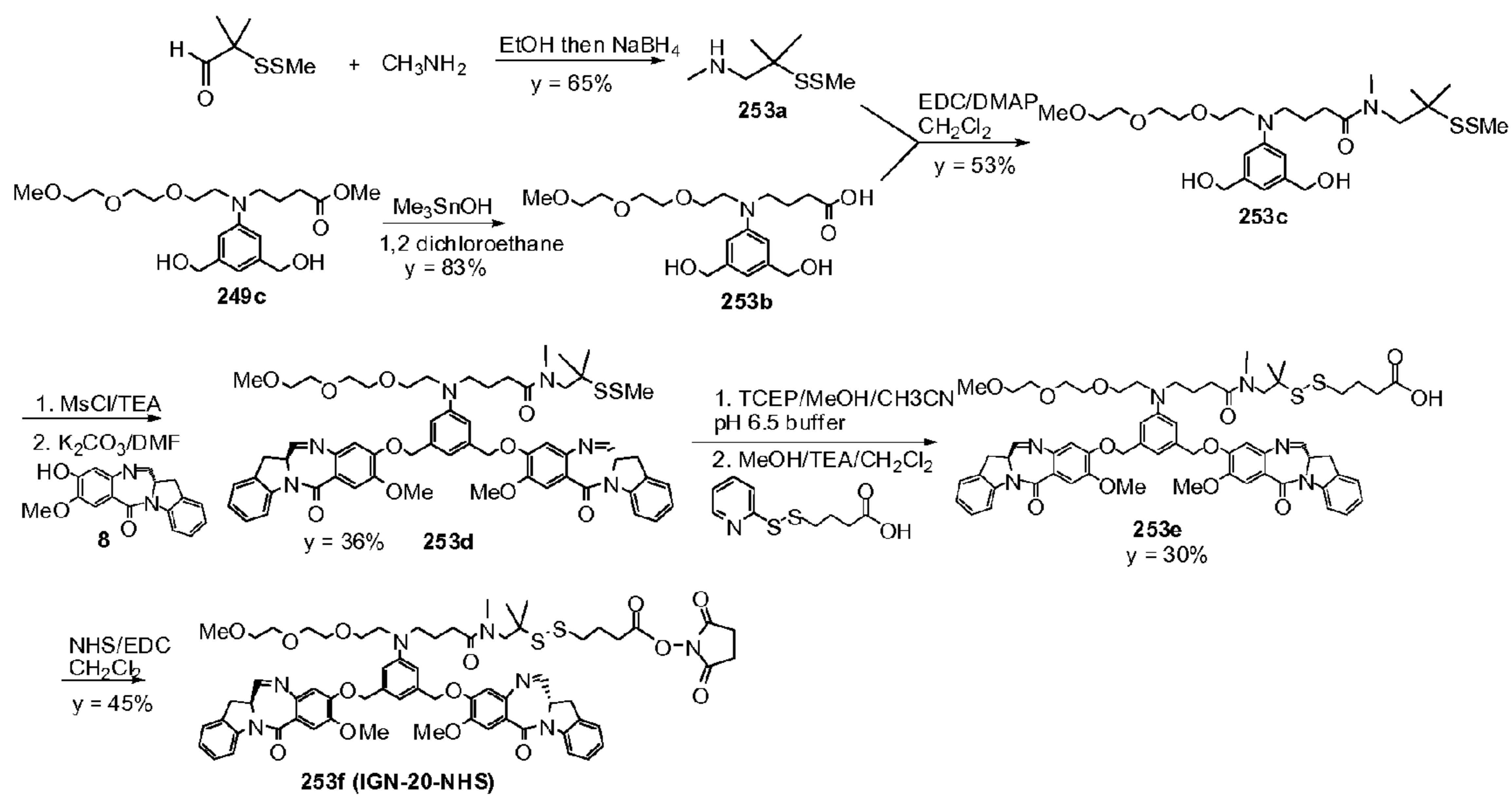
Figure 37. Synthetic scheme for linkable dimer
