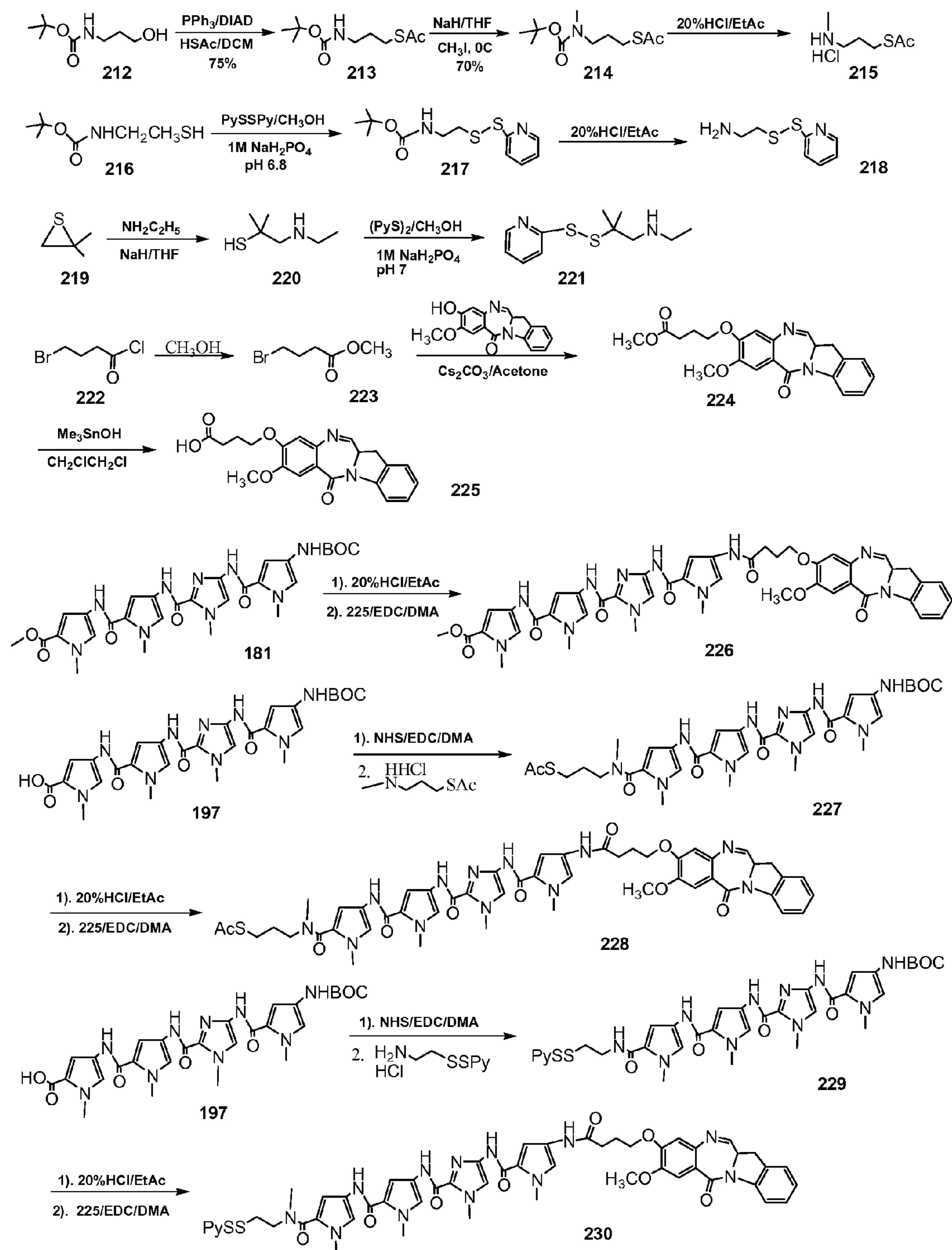
Figure 19. The synthesis of IBD-polypyrrole-imidazole analogs
