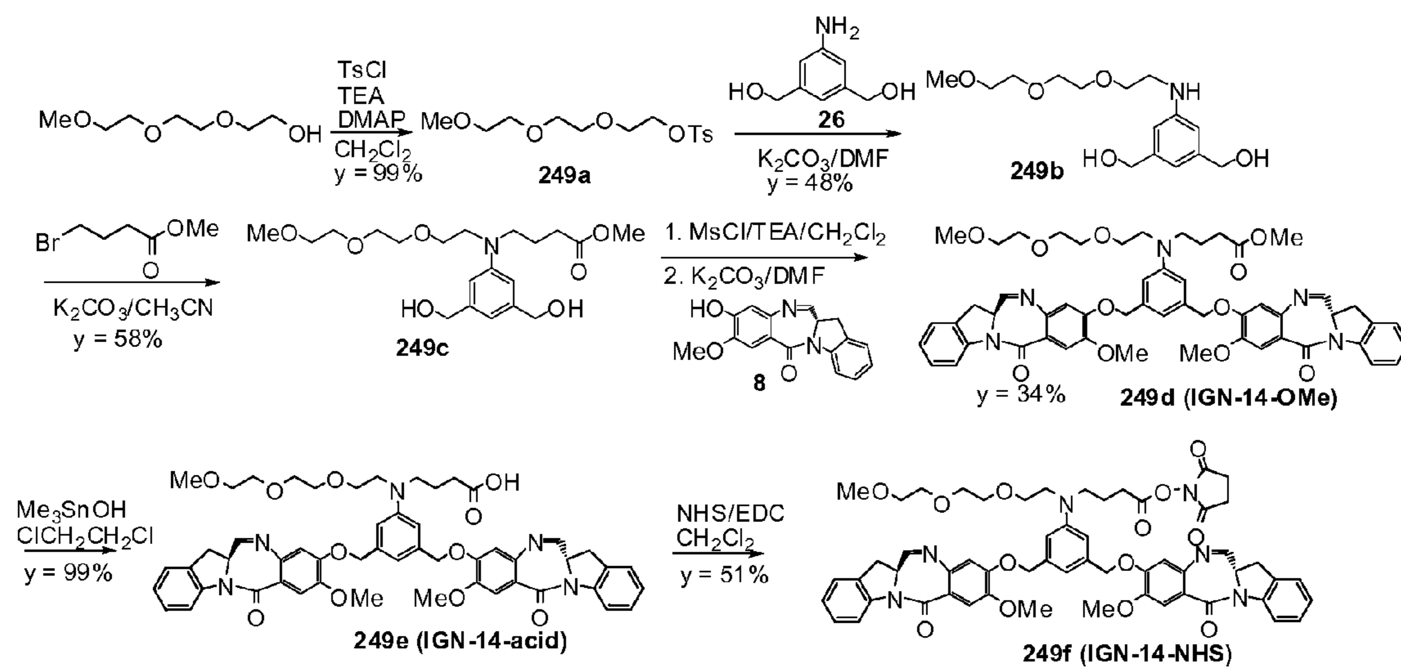
Figure 33. Synthetic scheme for indolinobenzodiazepine (IBD) dimers
