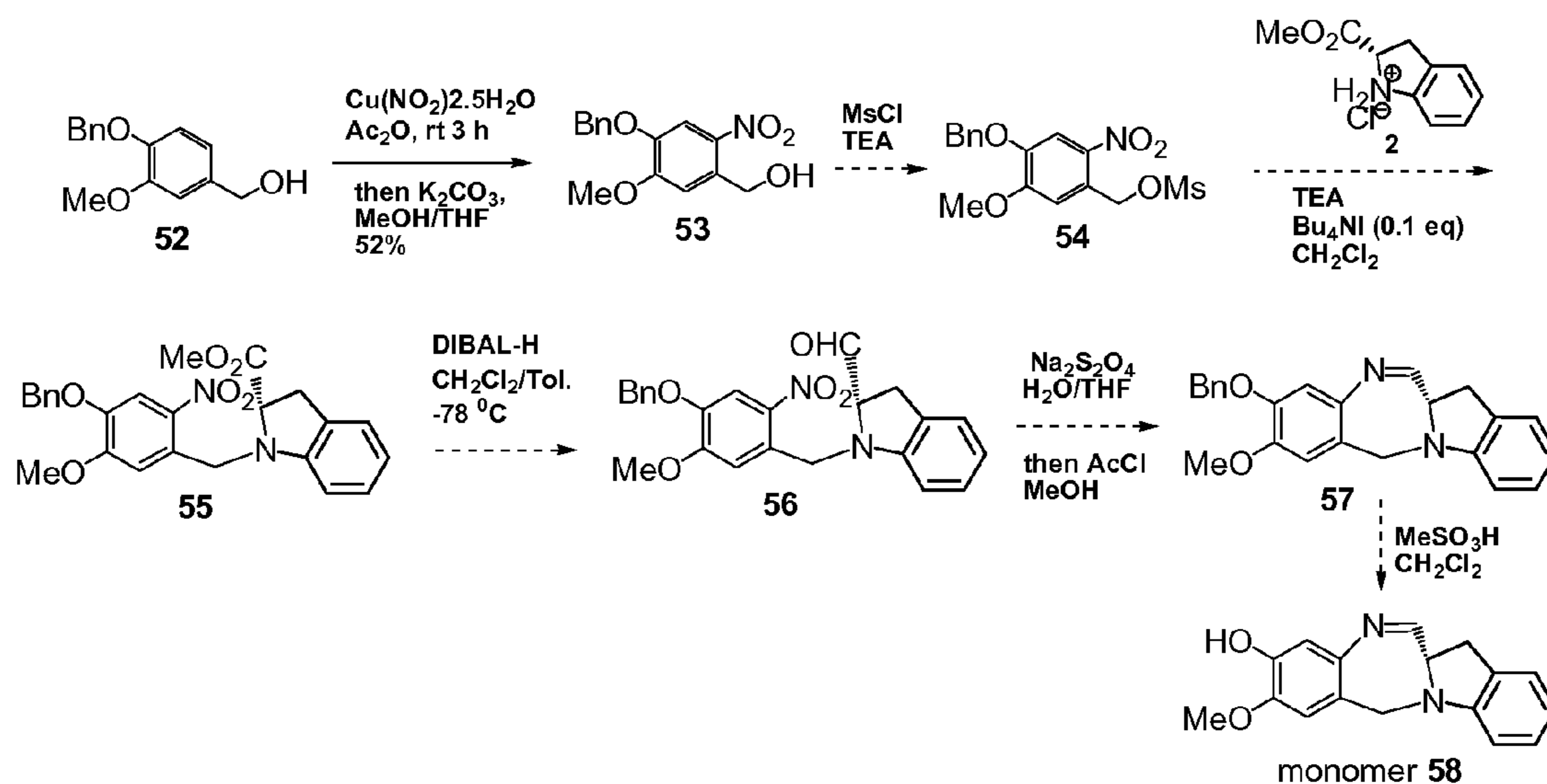
Figure 12. Synthetic scheme of isoindolinobenzodiazepine monomer 66
