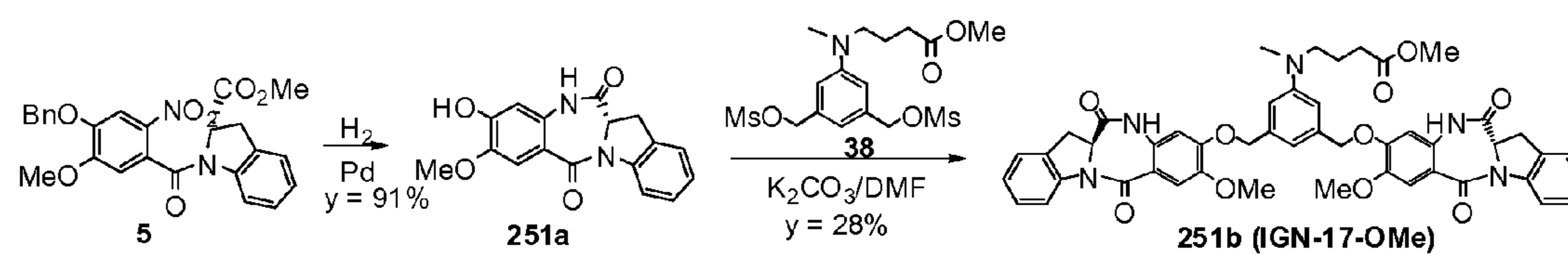
Figure 35. Synthetic scheme of dimer 251b (IGN-17-OMe) .
