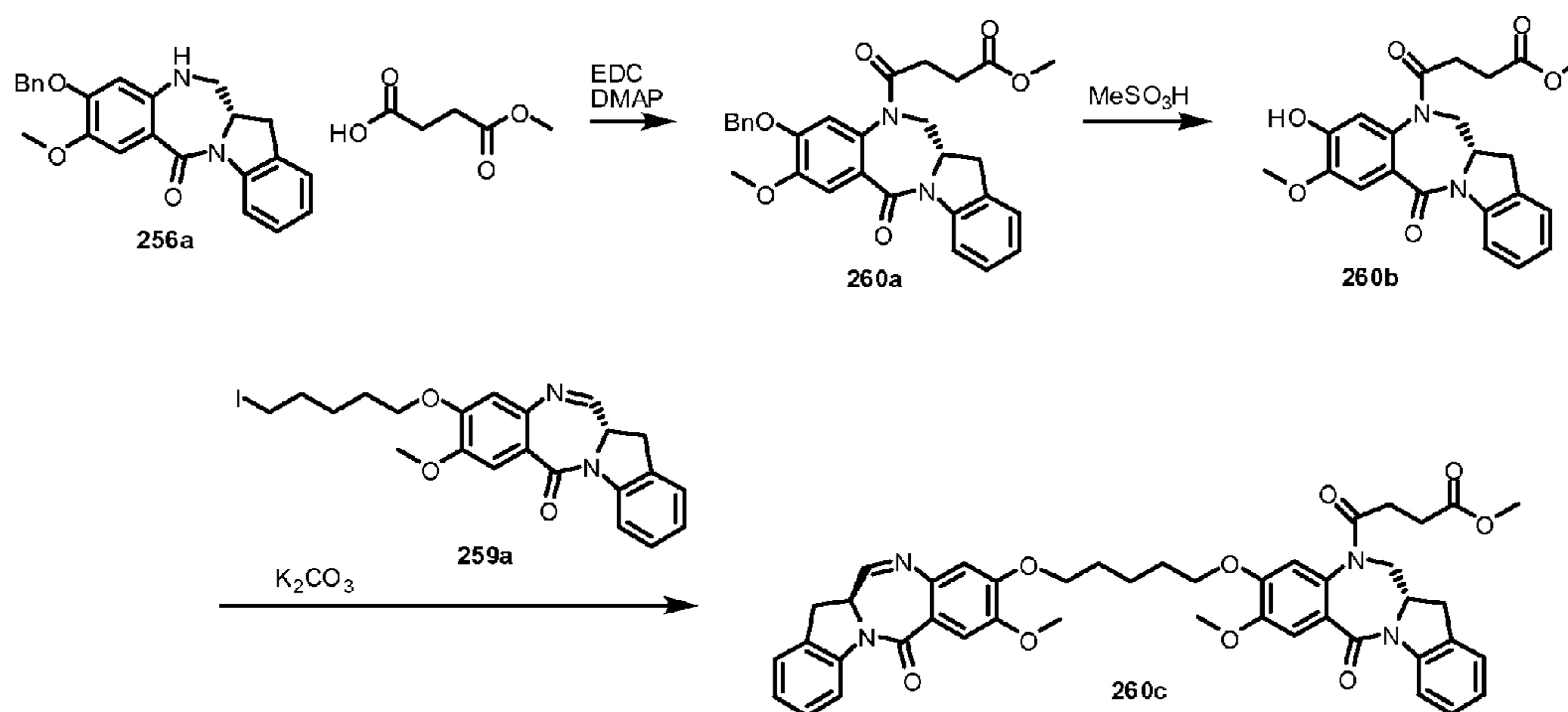
Figure 43. Synthetic scheme of compound 260c (IGN-25-OMe).
