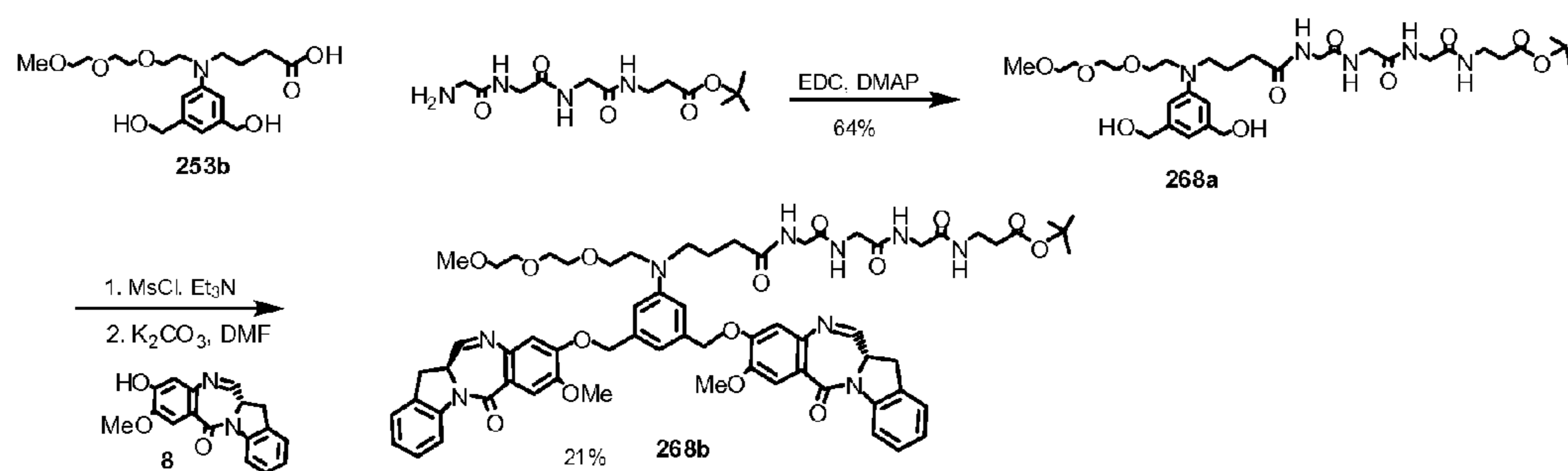
Figure 50. Synthetic scheme of dimer 268b (IGN-32-OtBu).
