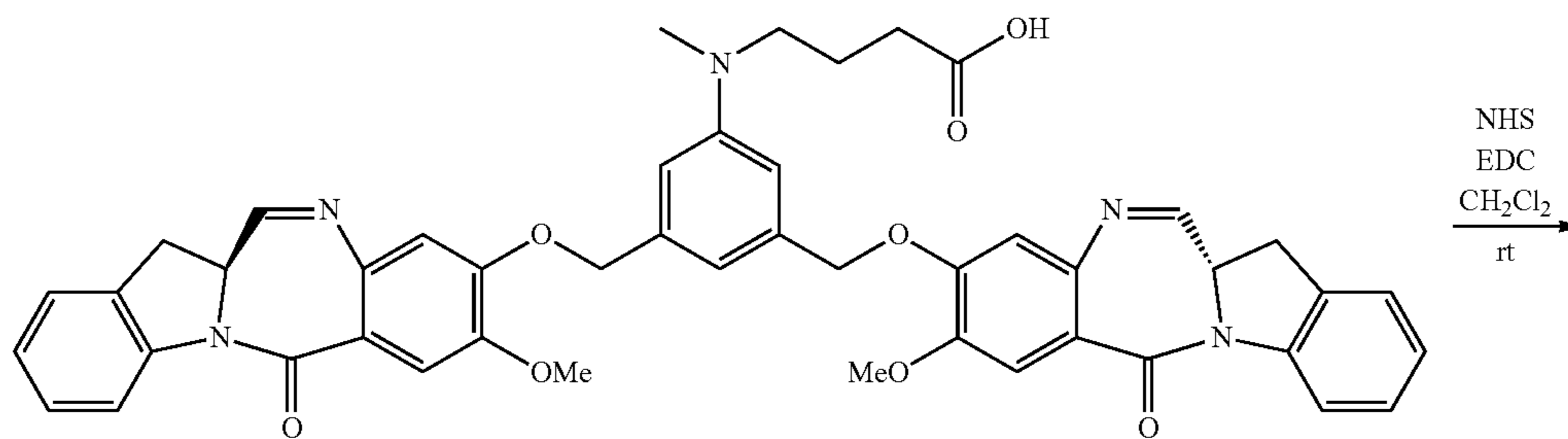
45 (IGN-07 acid)
