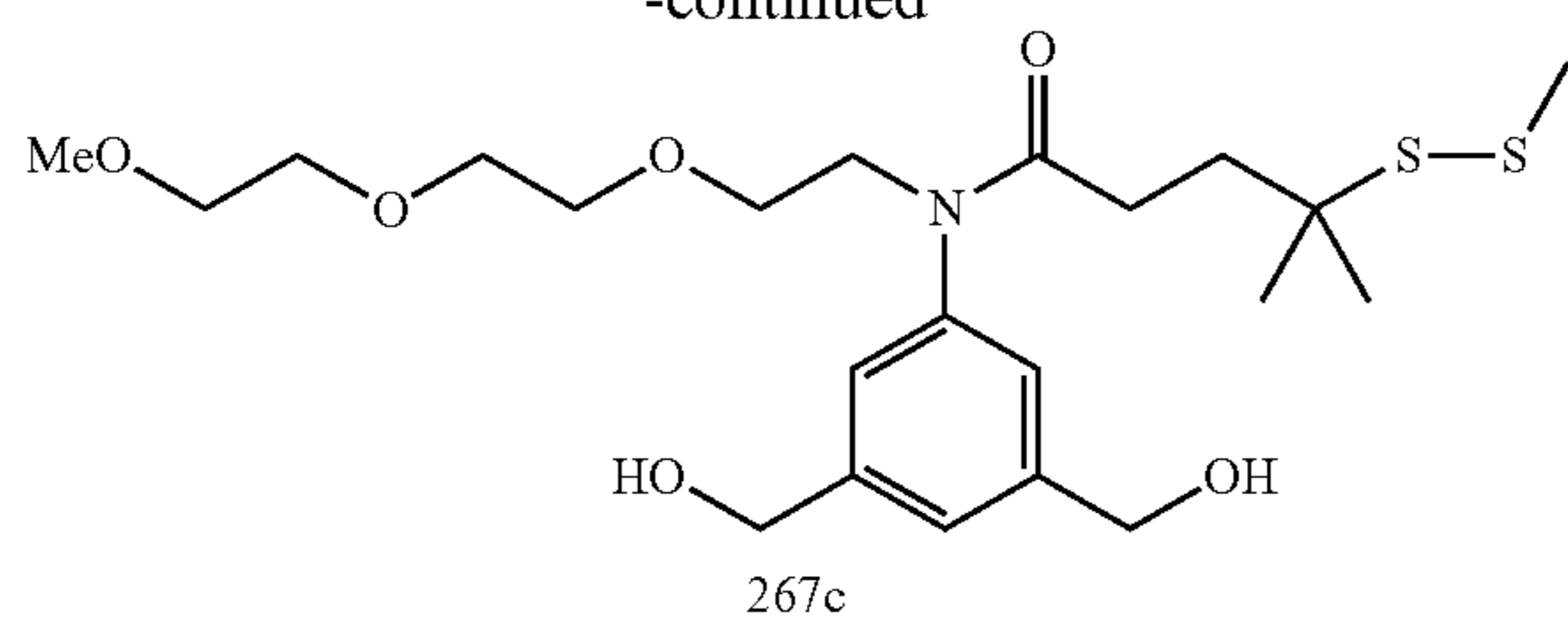
N-(3,5-bis(hydroxymethyl)phenyl)-N-(2-(2-(2-methoxyethoxy)ethoxy)ethyl)-4-methyl-4-(methylsulfanyl)pentanamide (267c)
