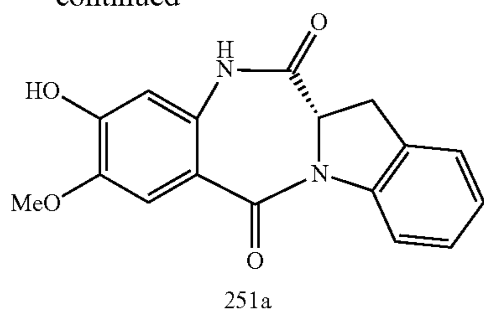
Compound 251a
