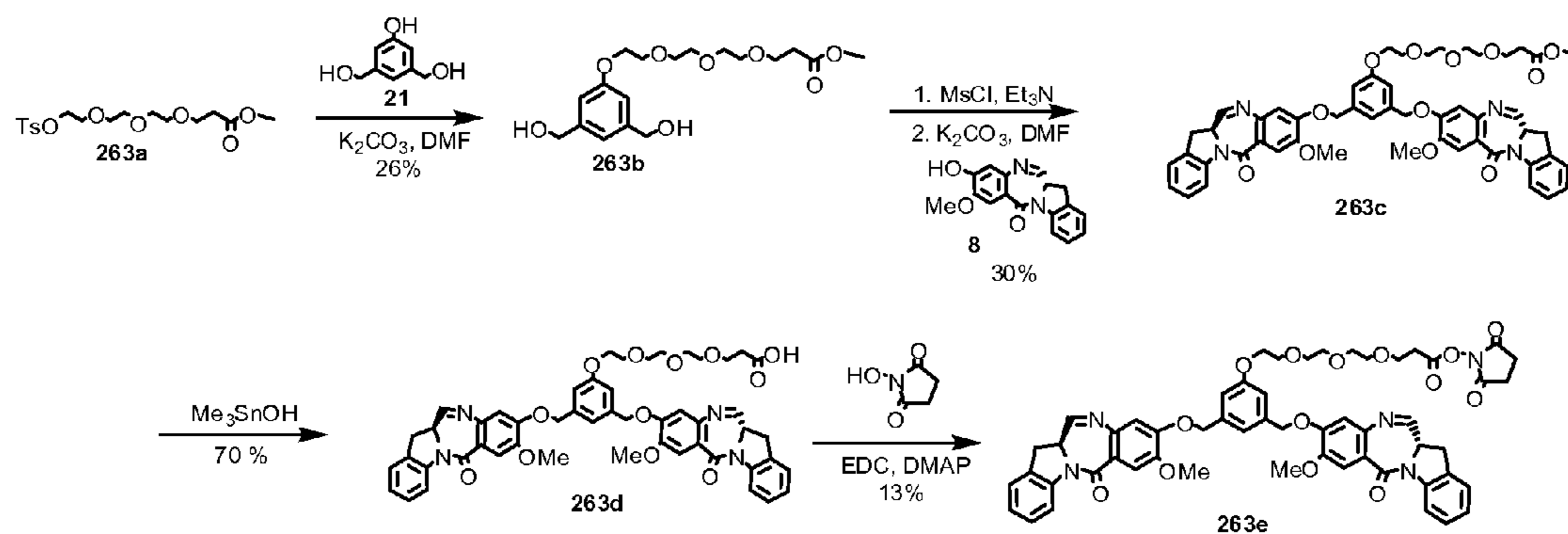
Figure 45. Synthetic scheme of dimer 263e (IGN-13-NHS).
