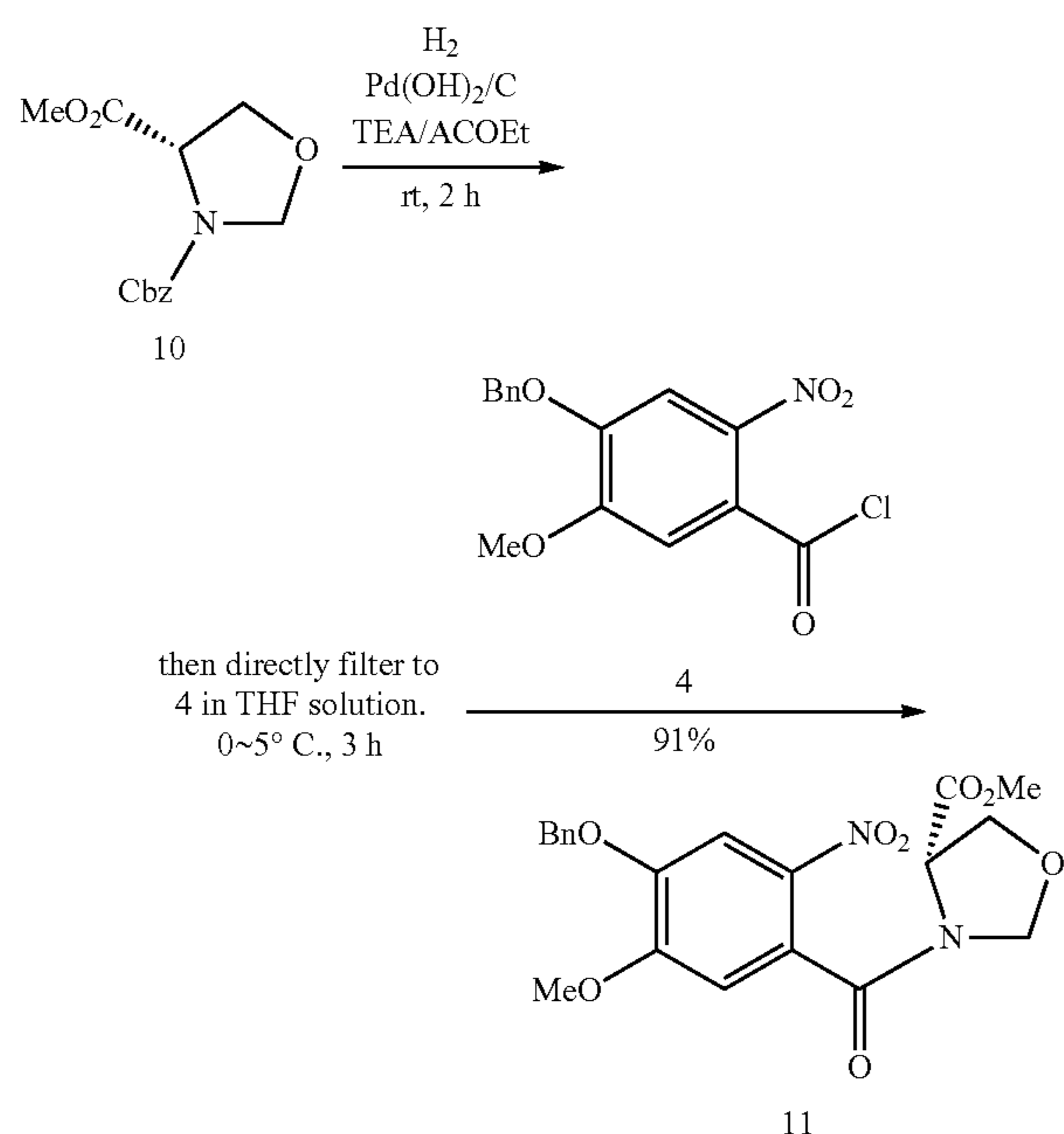
Compound 11
