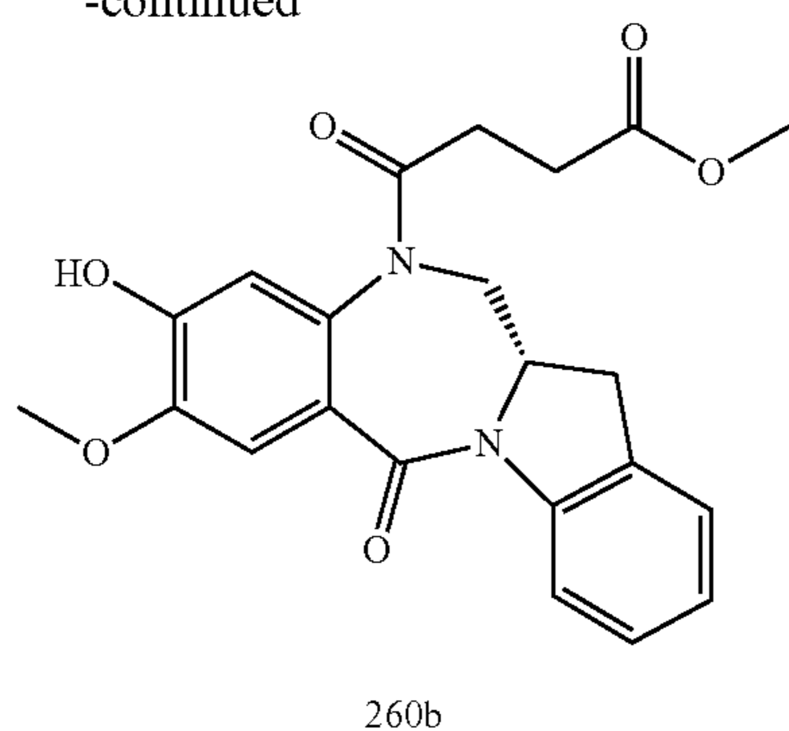
Compound 260b
