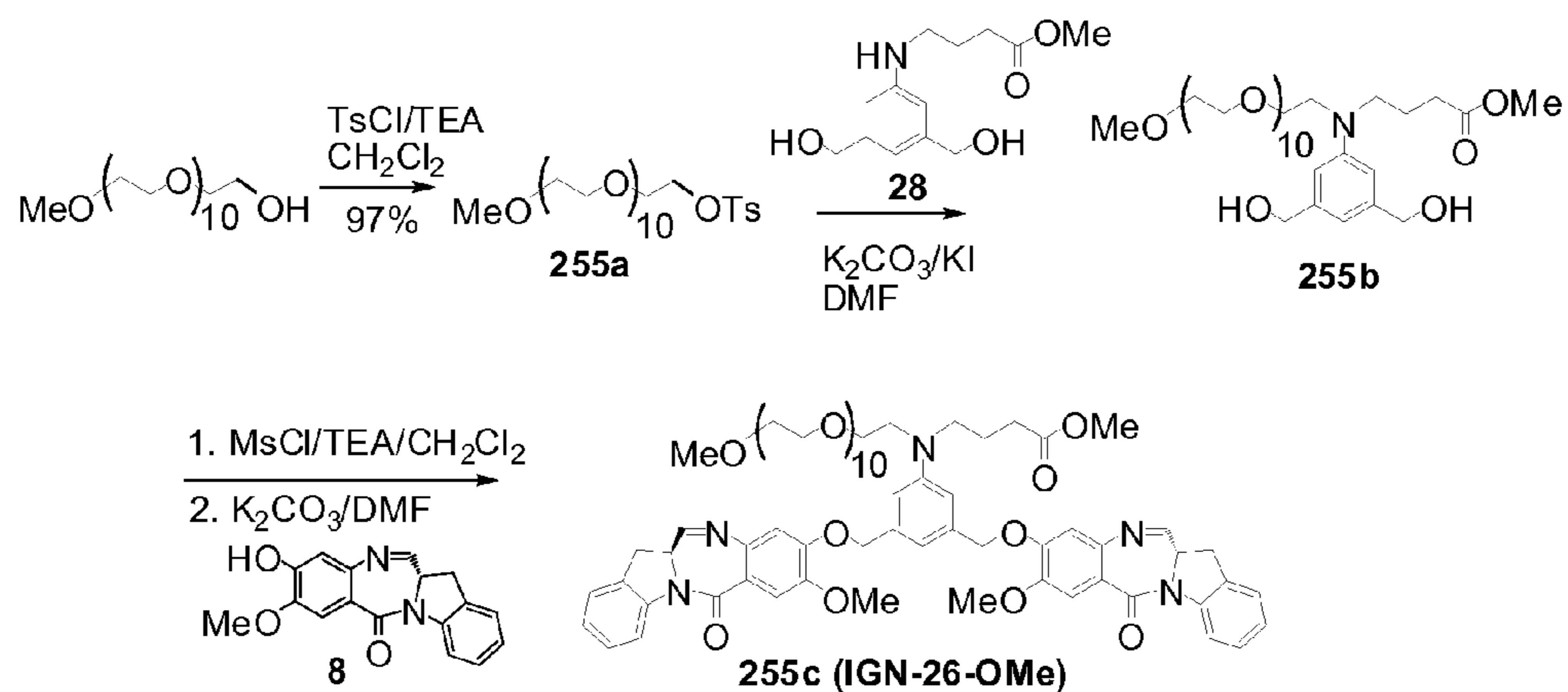
Figure 39. Synthetic scheme of IBD dimer 255c (IGN-26-OMe) .
