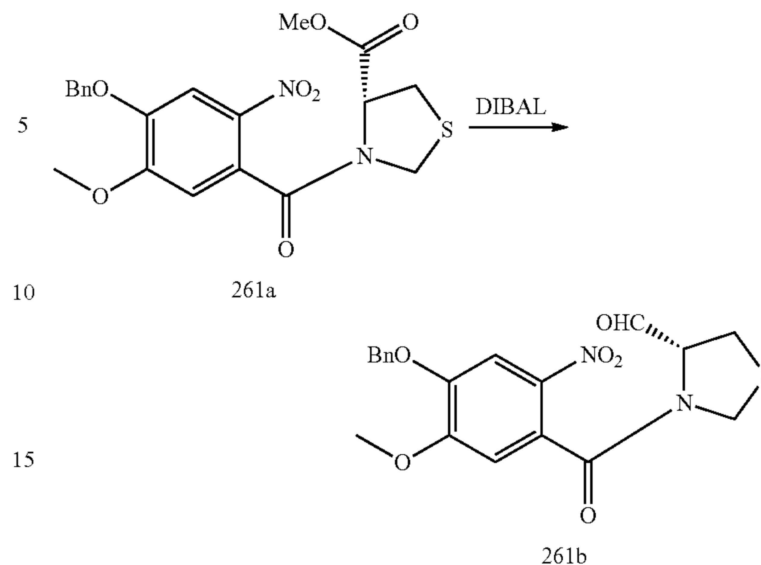
Compound 261b
