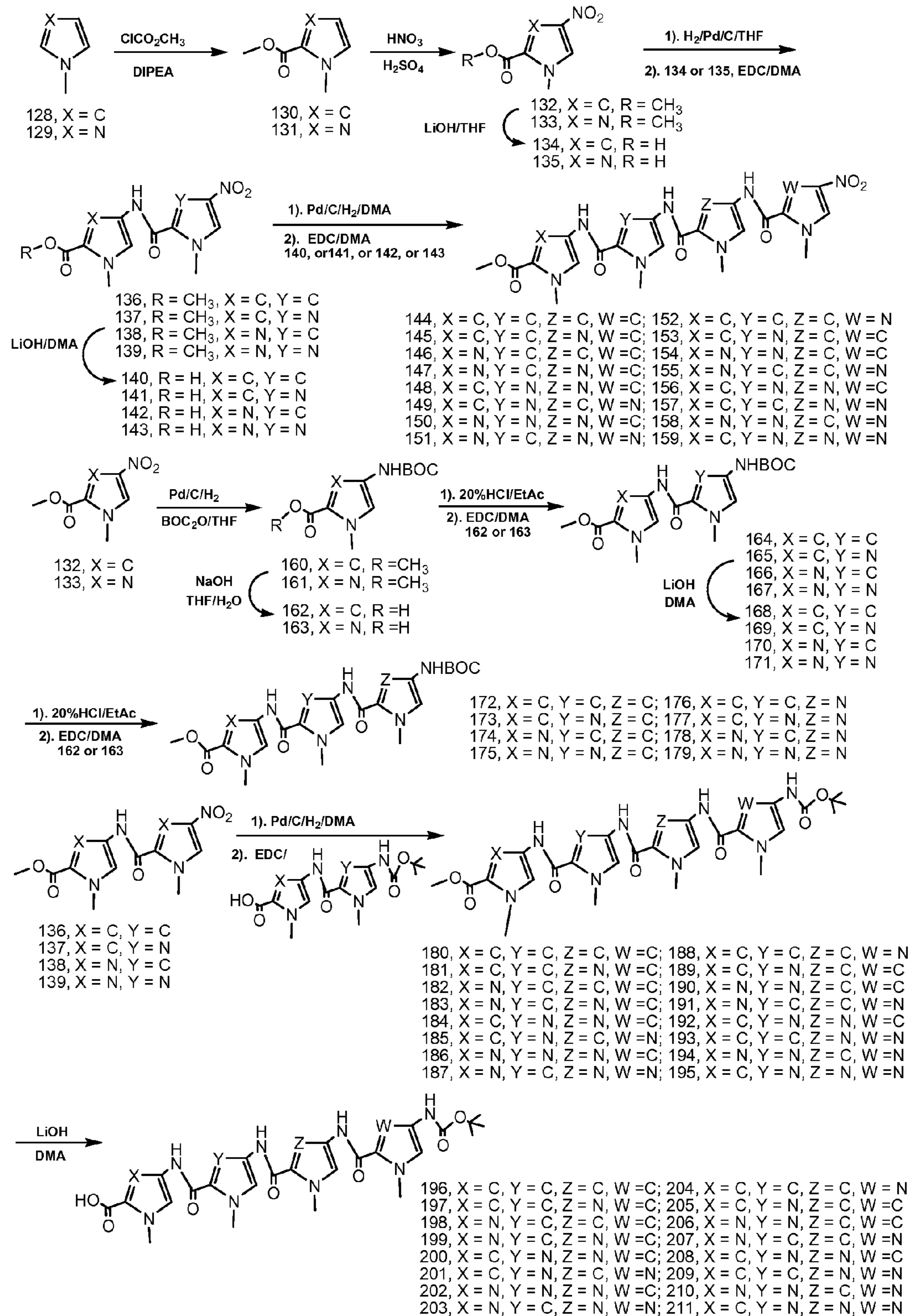
Figure 18. The assembling of polypyrroles/polyimidazoles
