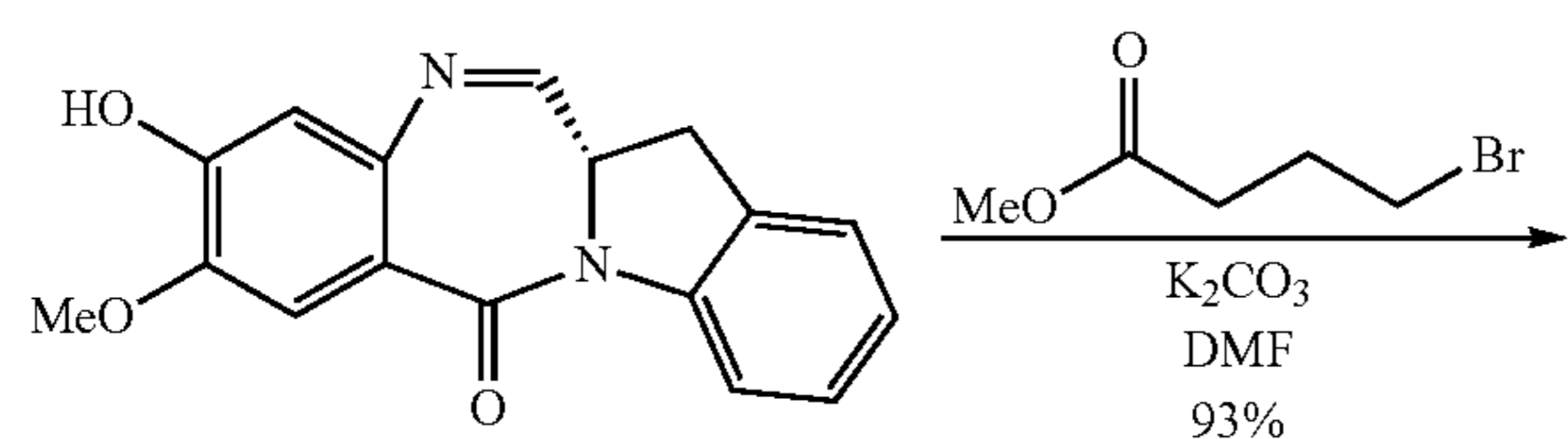
IBD monomer 8
