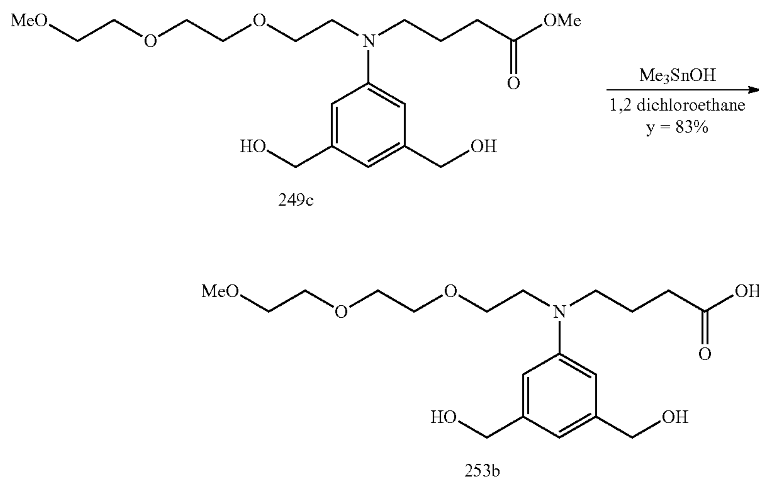
Compound 253b
