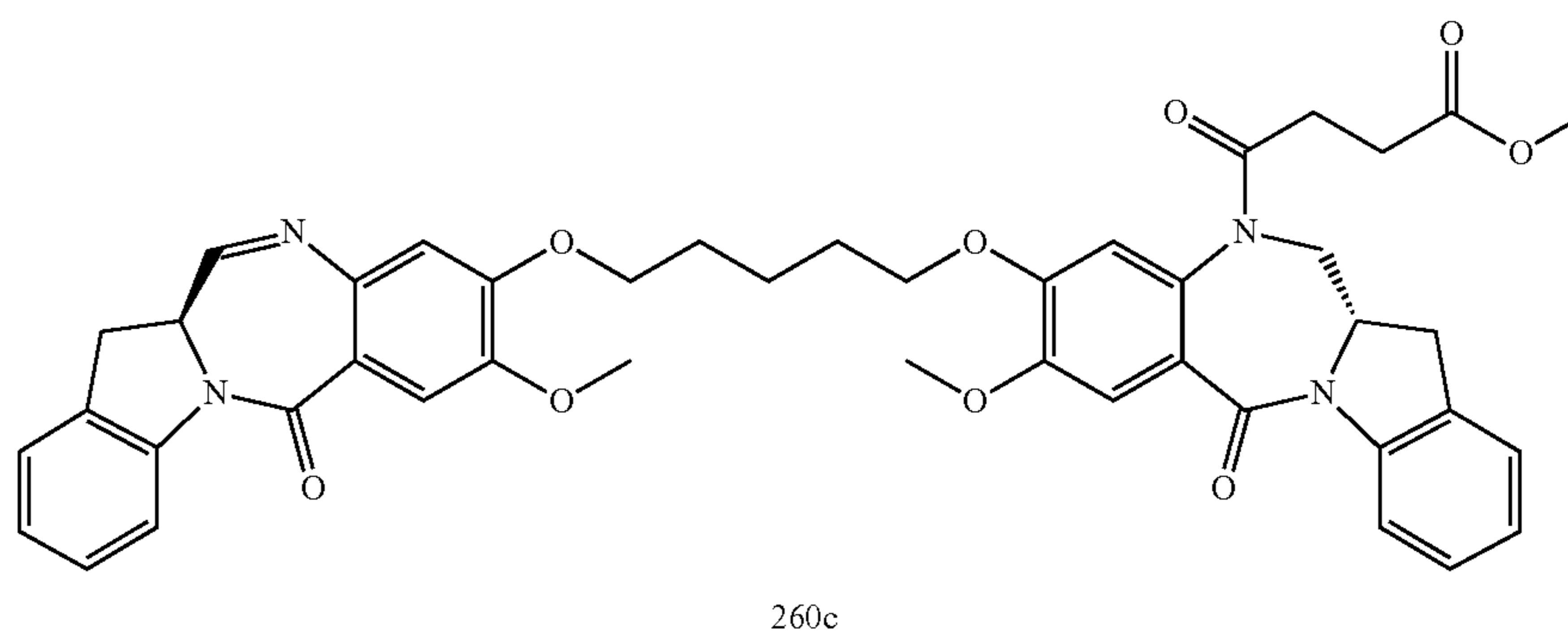
Compound 260c
