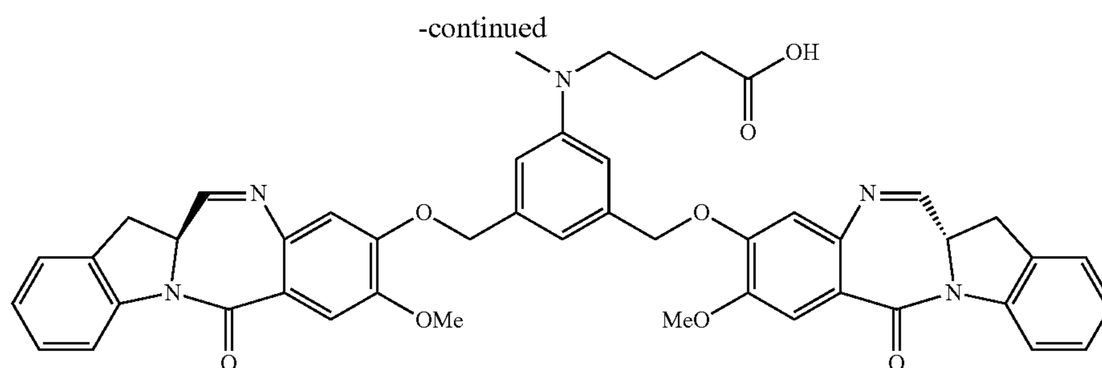
45 (IGN-07 acid)
