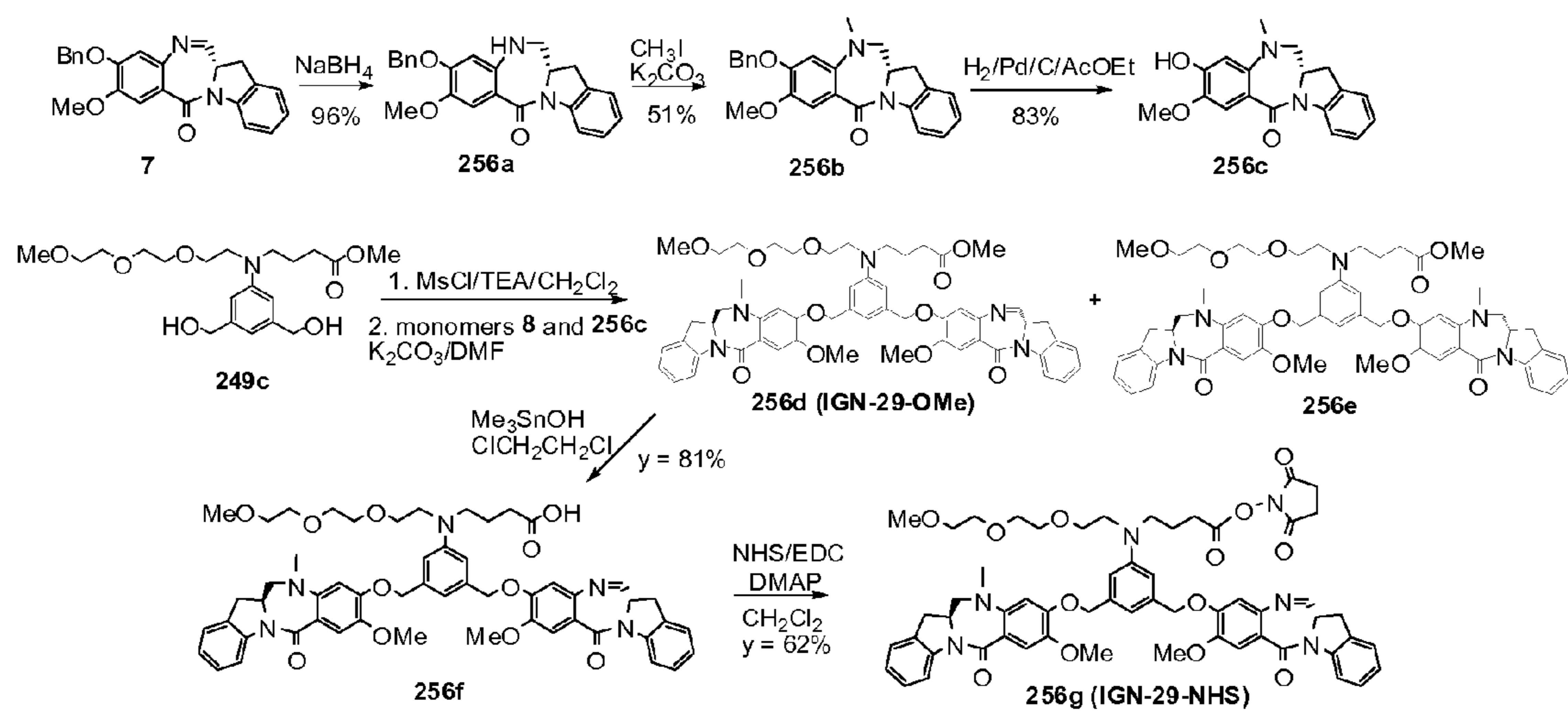
Figure 40. Synthetic scheme of compound 256g (IGN-29-NHS) .
