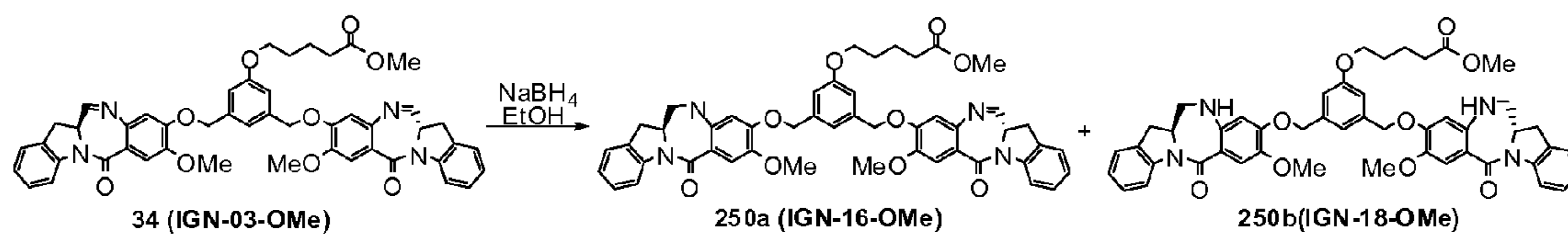
Figure 34. Synthetic scheme of esters of IBD dimers
