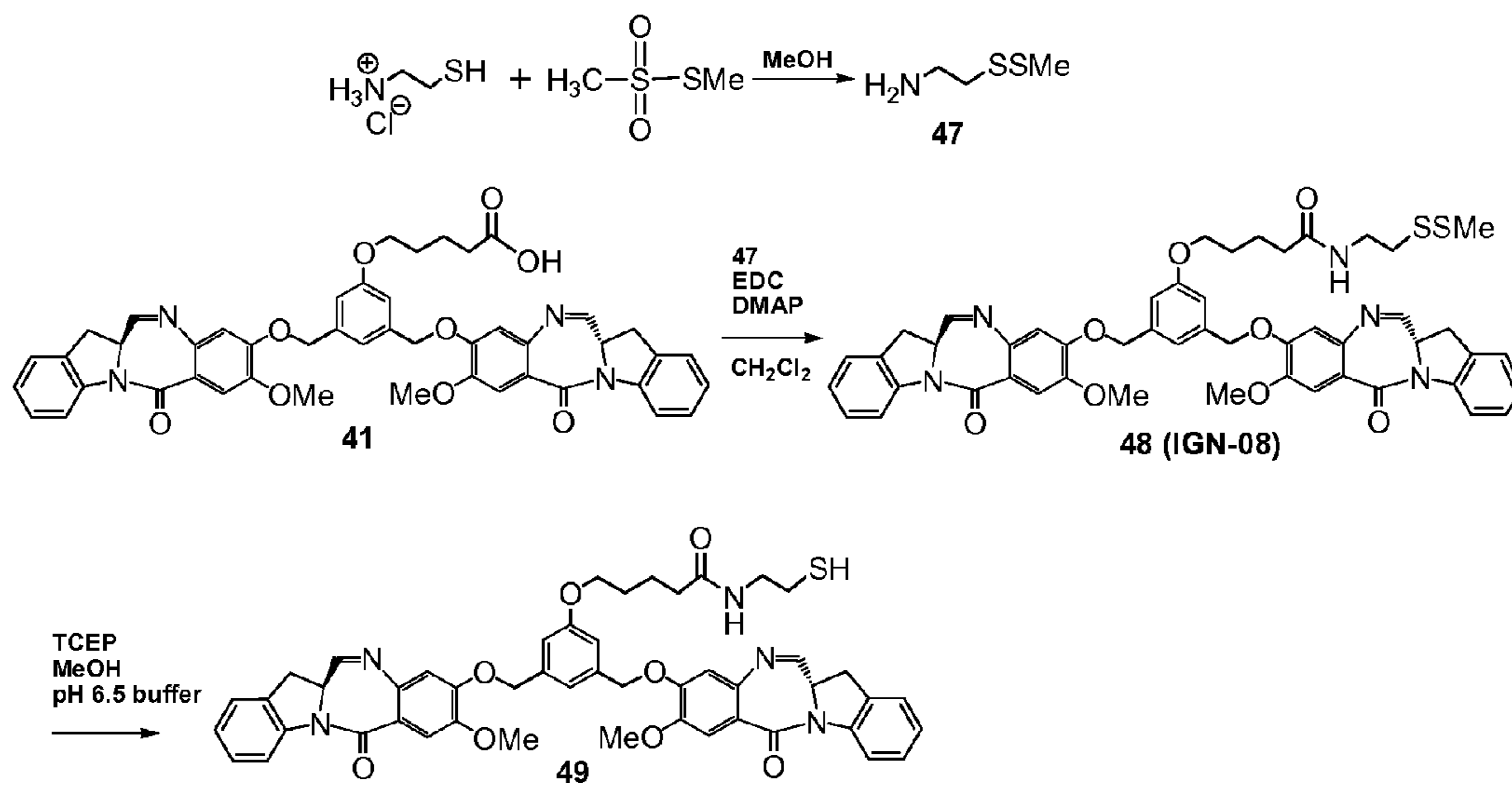
Figure 9. Synthetic scheme of thiol 49
