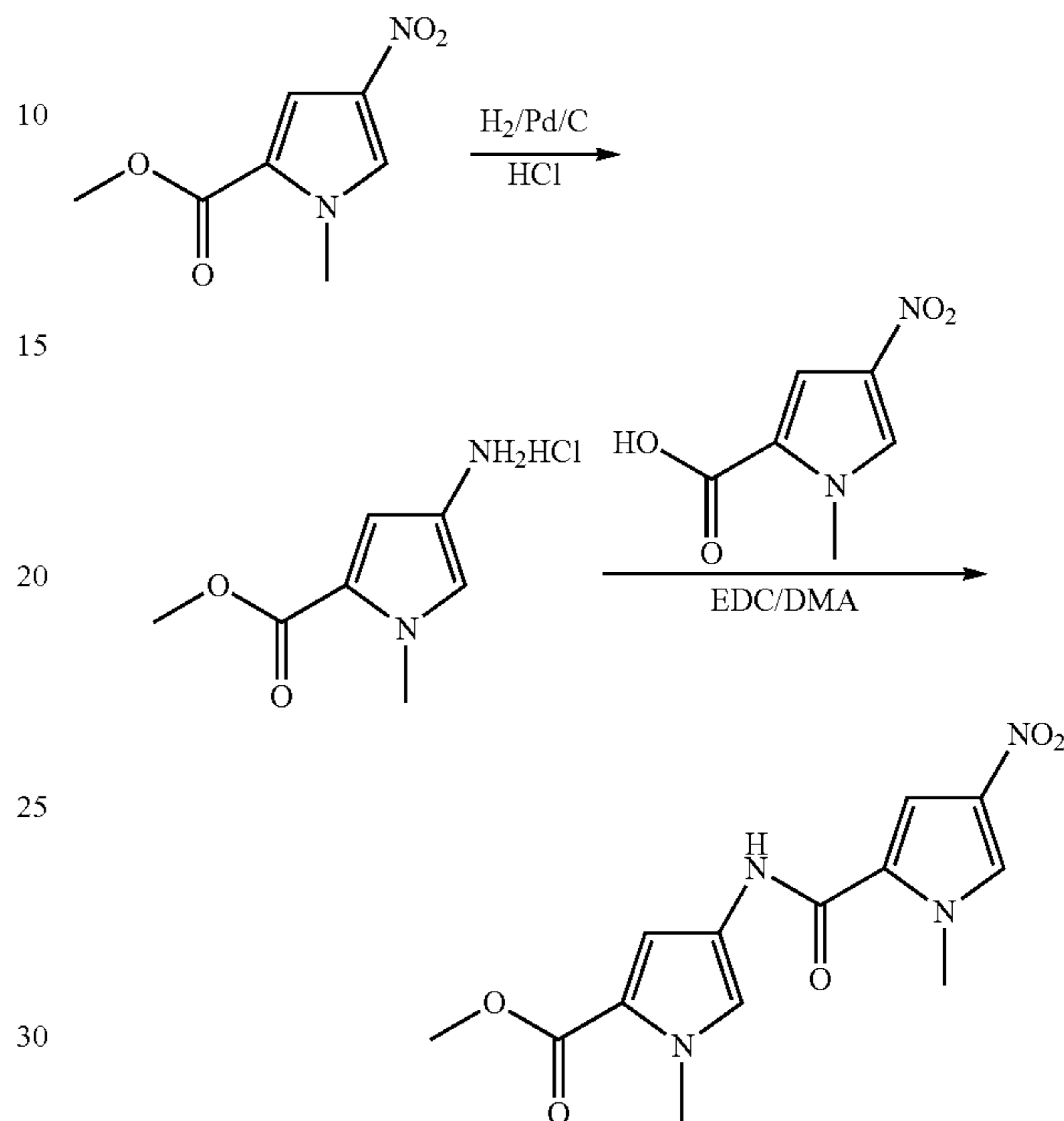
Methyl 1-methyl-4-(1-methyl-4-nitro-1H-pyrrole-2-carboxamido)-1H-pyrrole-2-carboxylate
