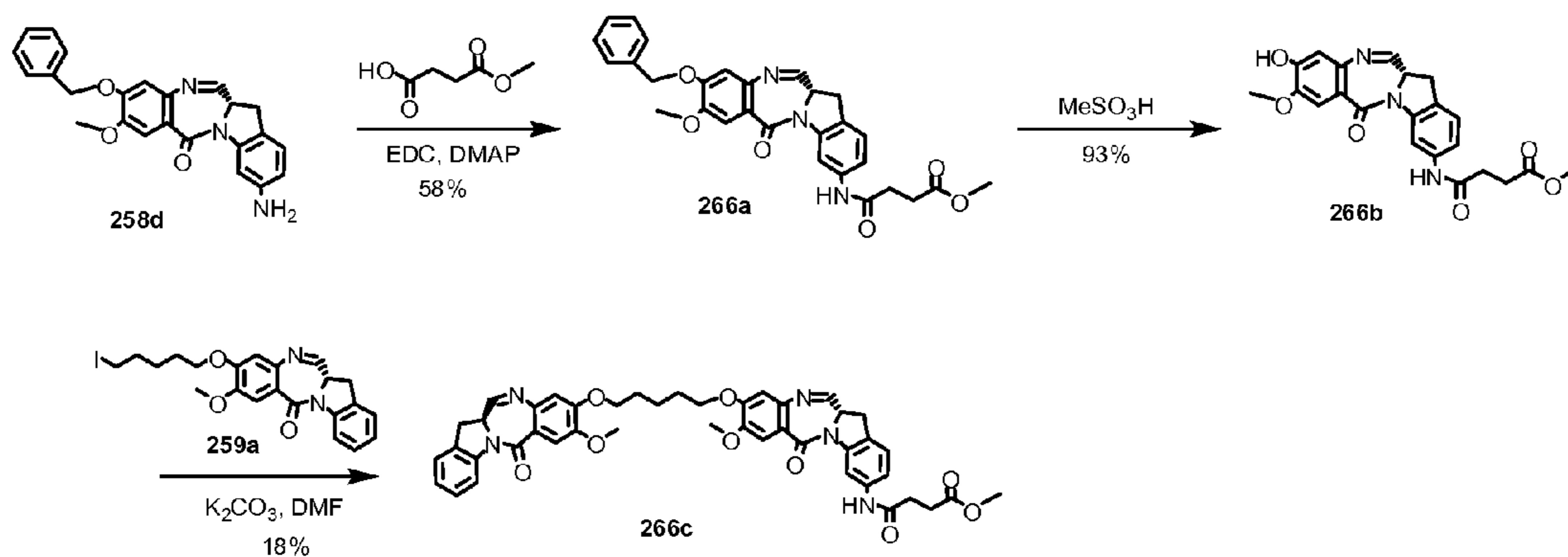
Figure 48. Synthetic scheme of dimer 266c (IGN-22-OMe).
