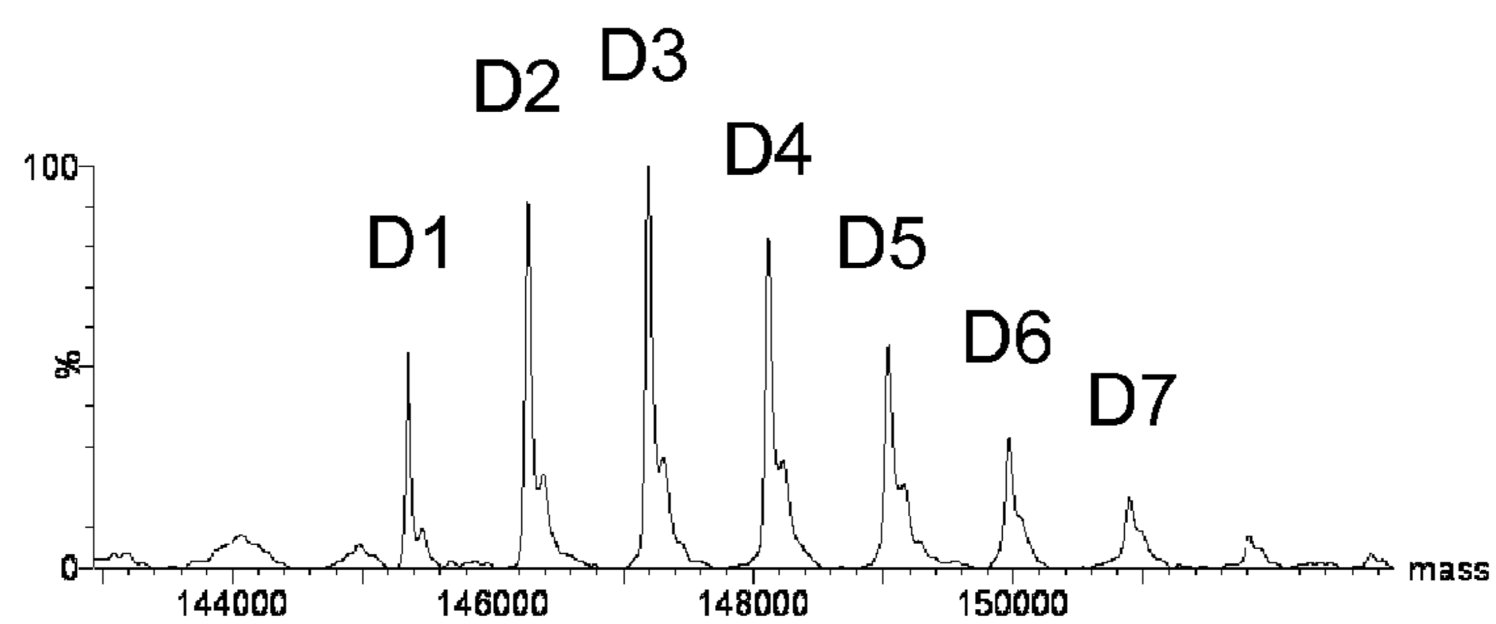
Figure 59. MS analysis of chB38.1-IGN14 conjugate
