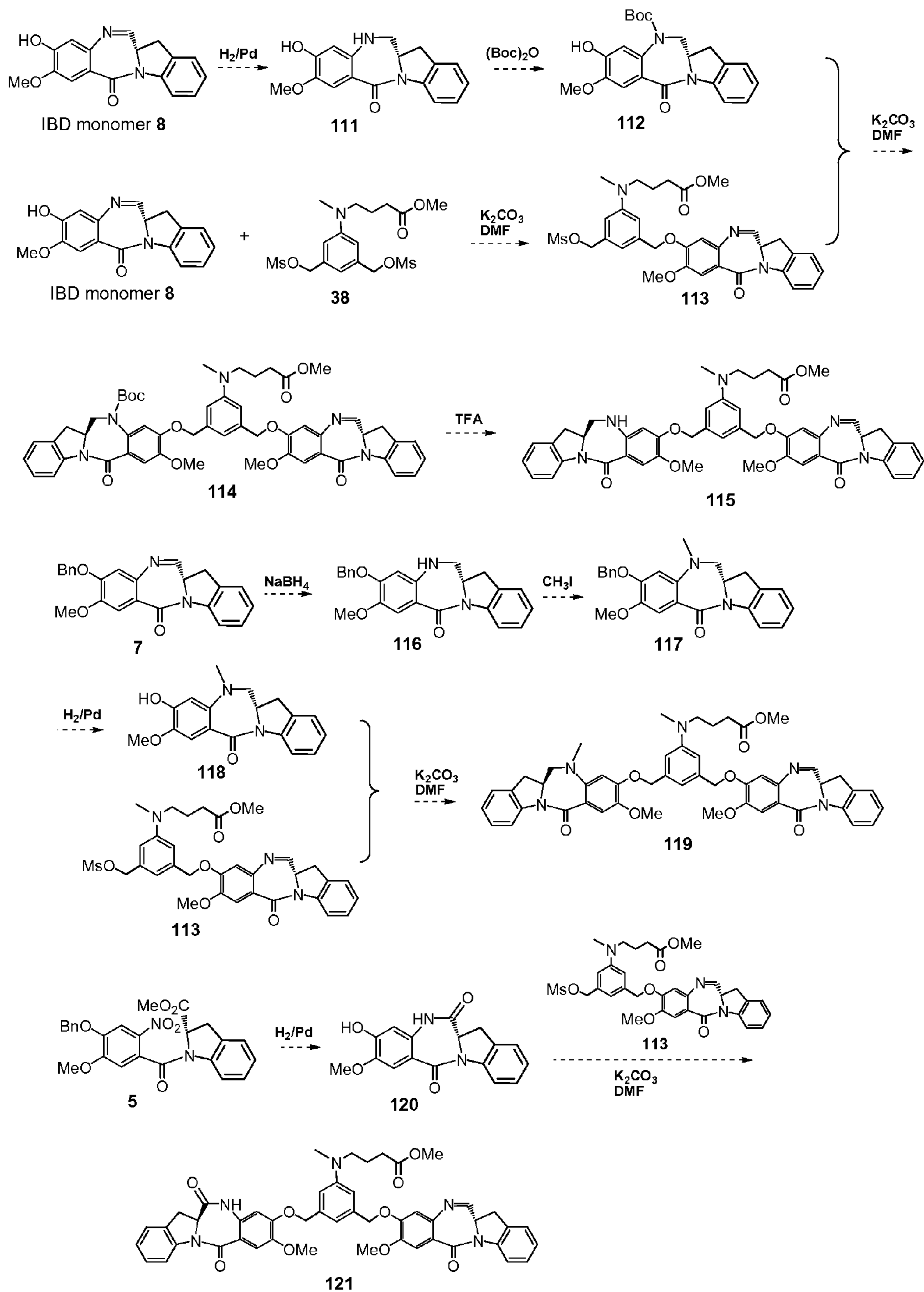
Figure 16. Synthetic schemes of compounds 115, 119 and 121
