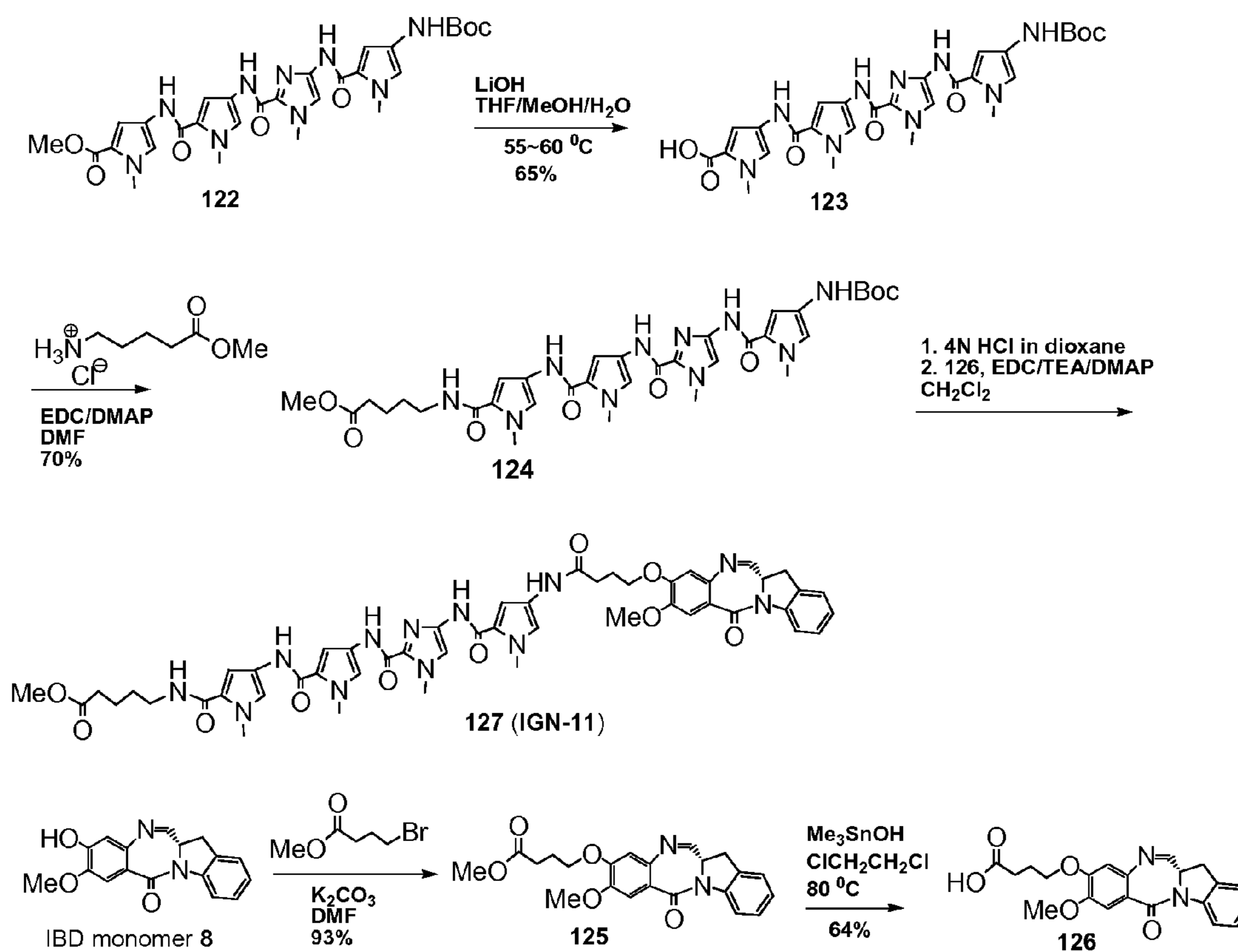
Figure 17. Synthetic scheme of compound 127 (IGN-11)
