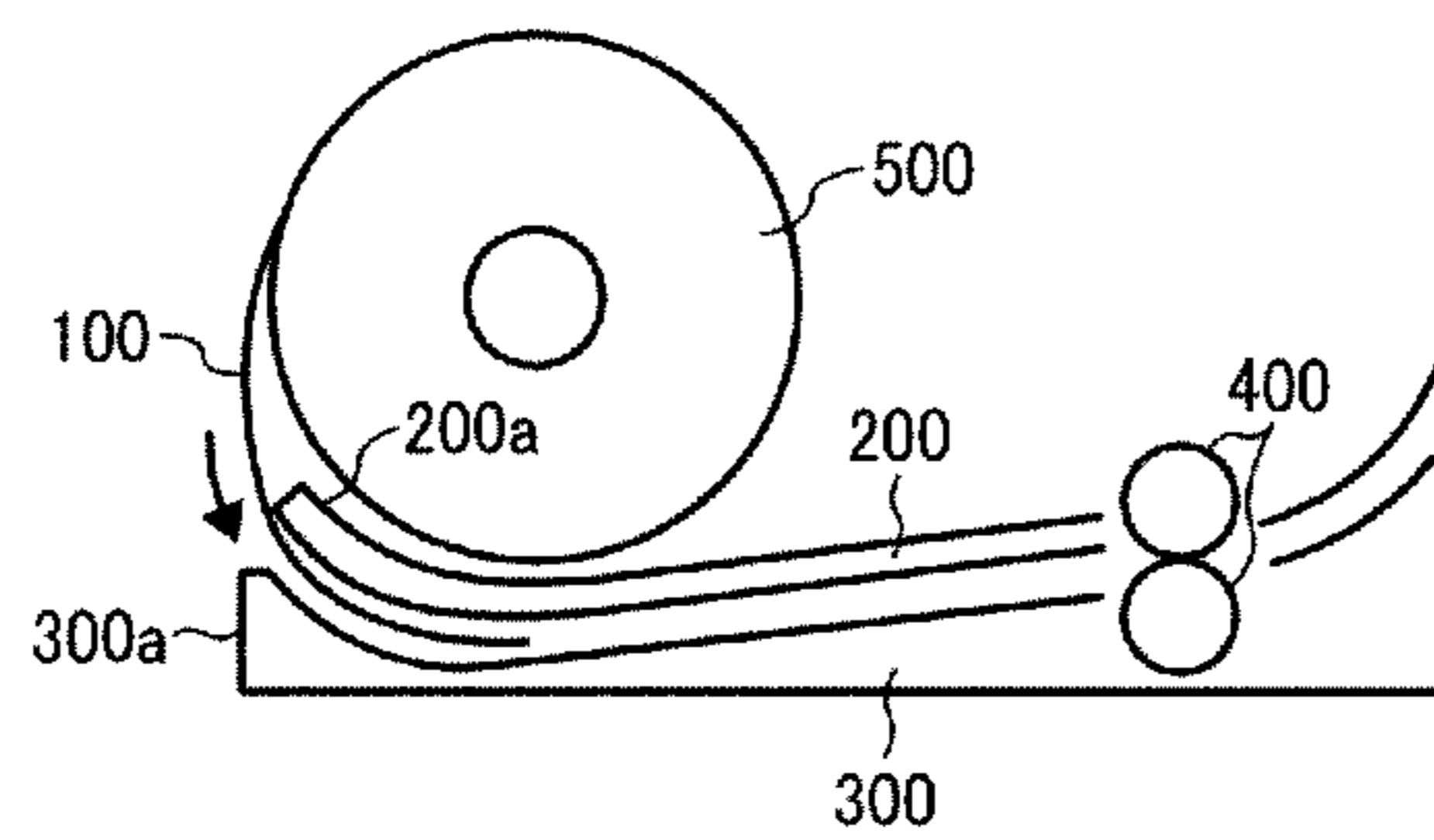
FIG. 20 RELATED ART
