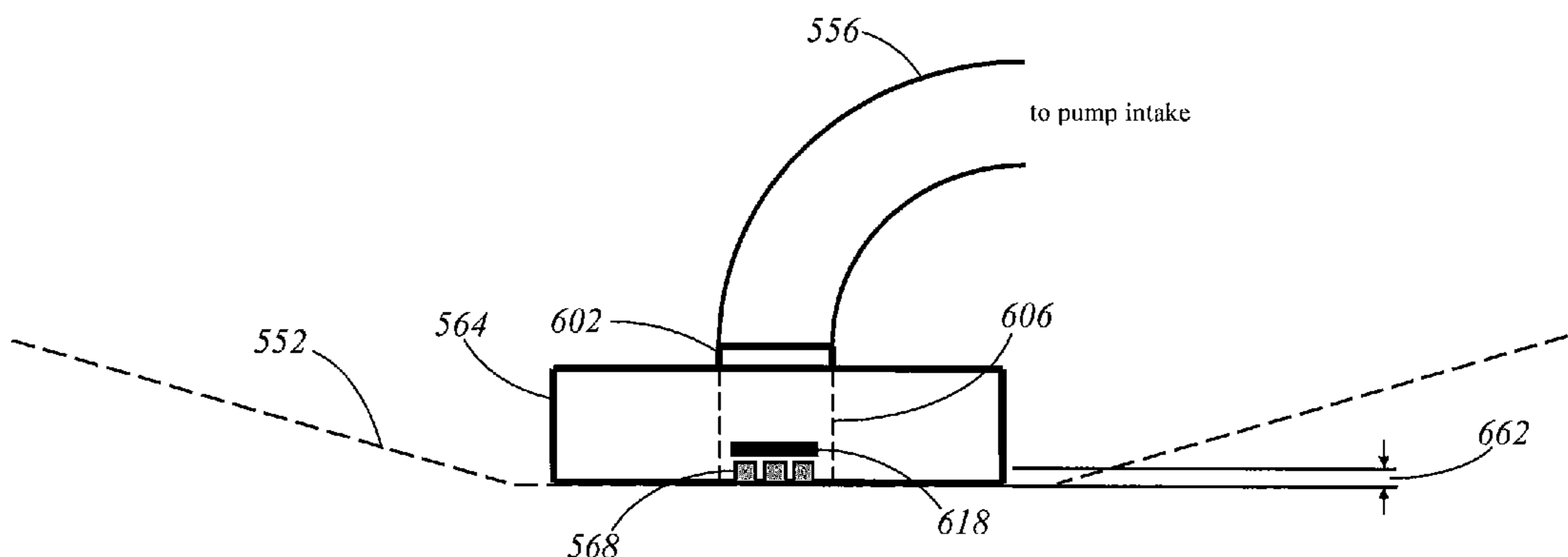
Figure 17a side view
