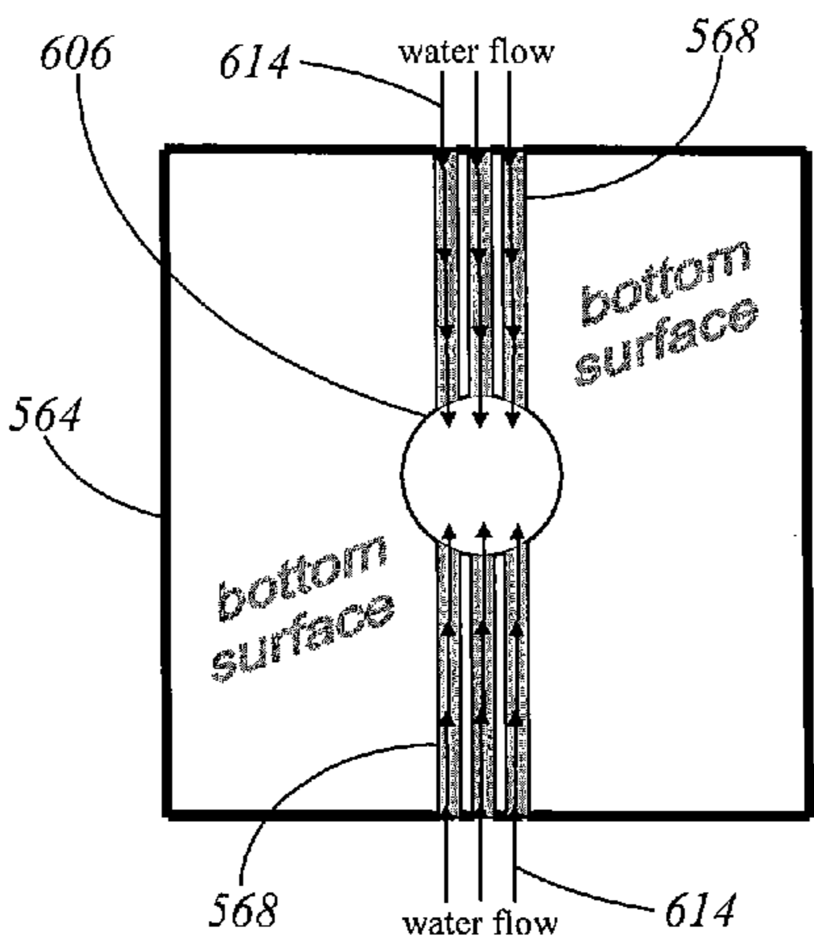
Figure 17b bottom view
