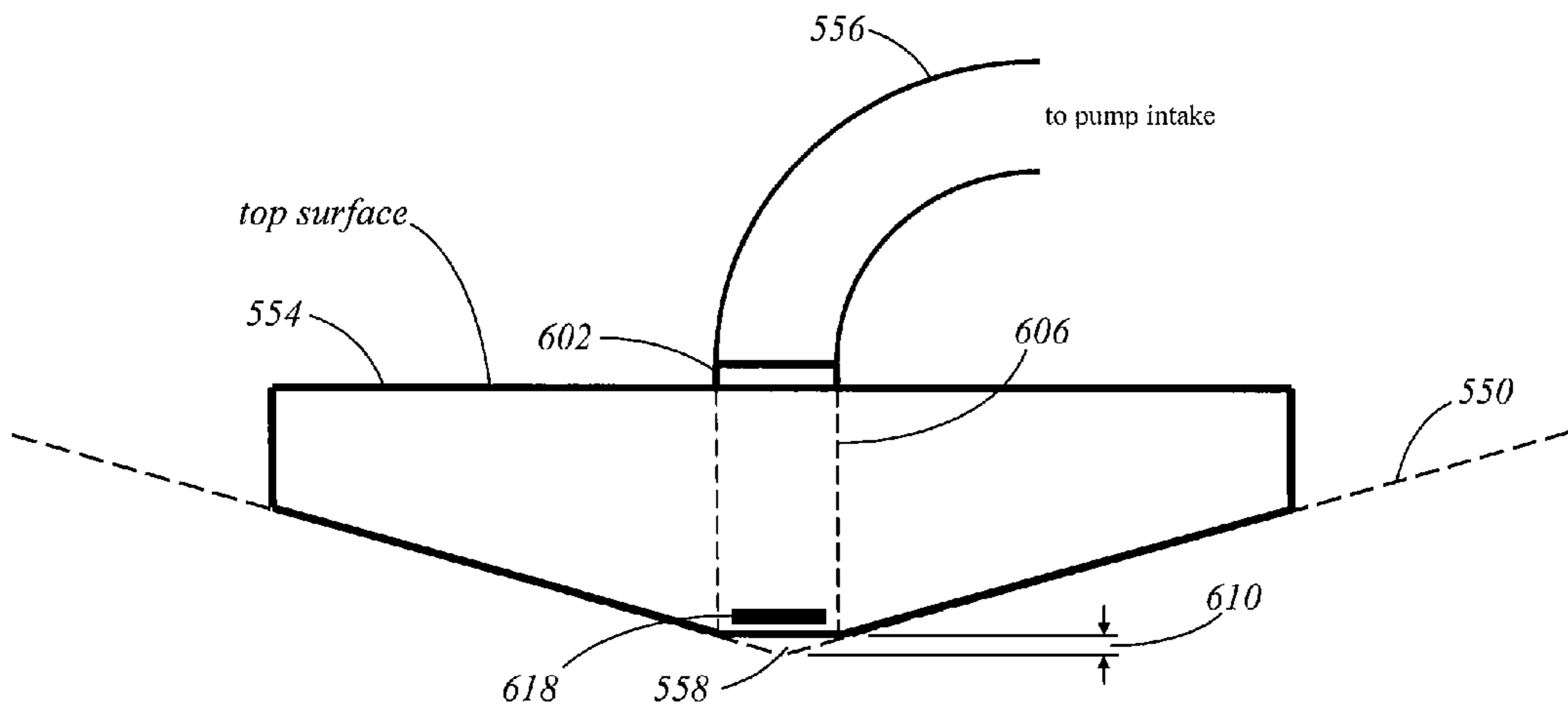
Figure 16a side view
